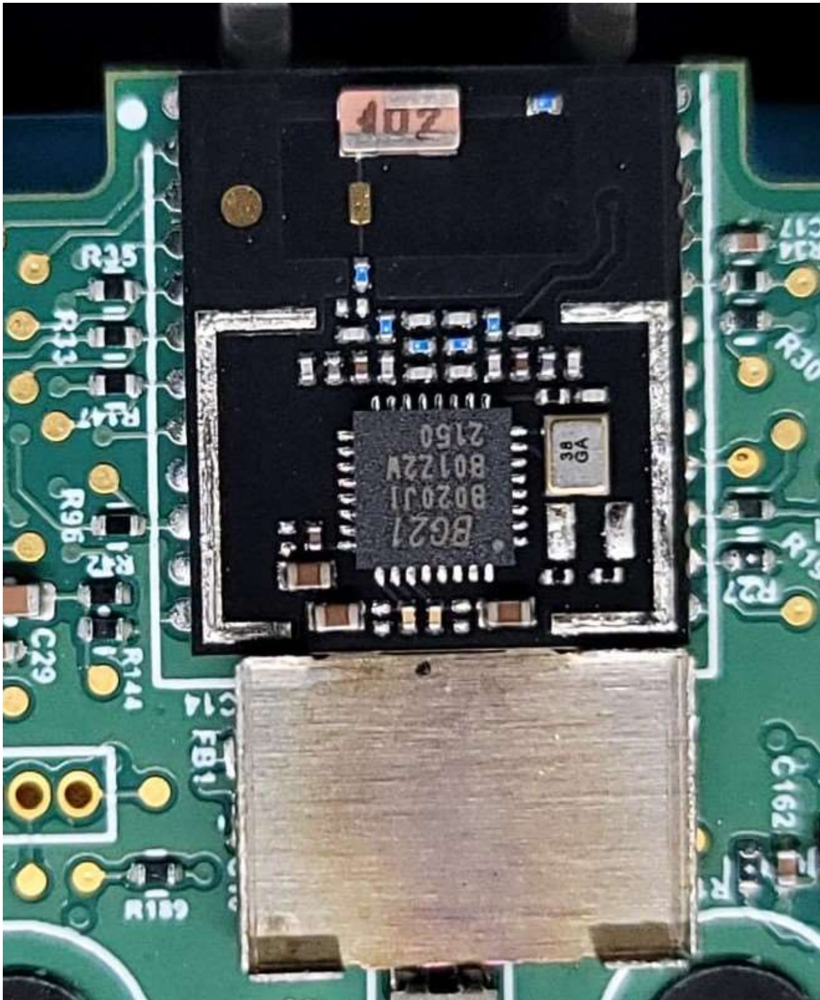
Closeup of the BLE module installed on the circuit board with the top cover (can) removed
