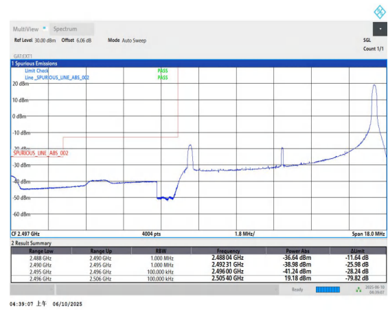
Band41-10MHz-QPSK-39700-1RB#49-PASS
