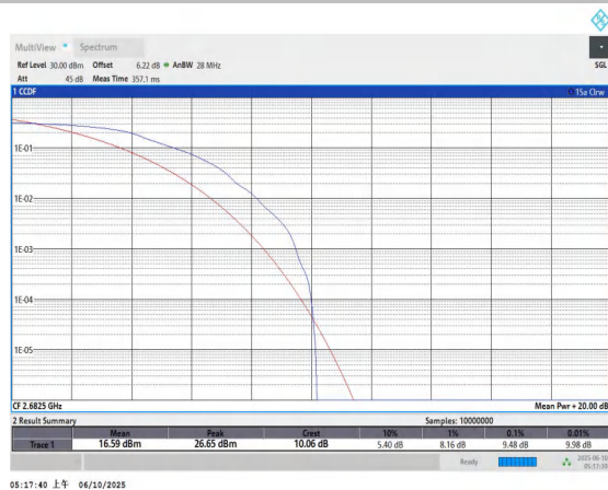
Band41-15MHz-QPSK-41515-1RB#0-PASS
