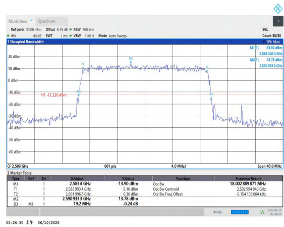
Band41-20MHz-QPSK-40620-100RB#0-PASS
