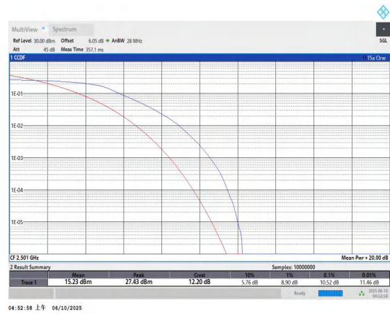
Band41-10MHz-QPSK-39700-50RB#0-PASS
