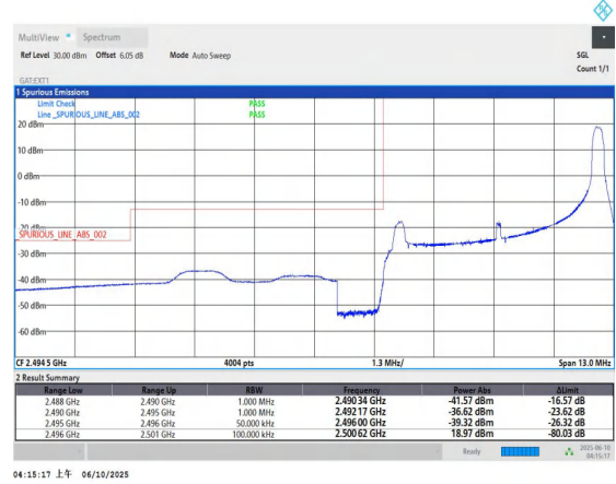
Band41-5MHz-QPSK-39675-1RB#24-PASS
