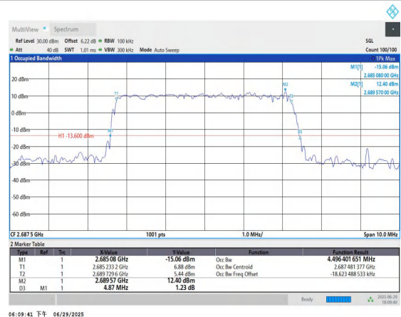
Band41-5MHz-16QAM-41565-25RB#0-PASS
