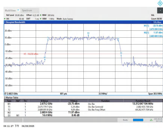
Band41-15MHz-16QAM-41515-75RB#0-PASS
