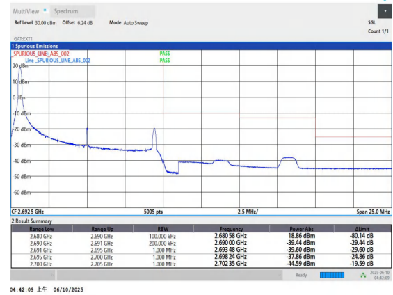
Band41-10MHz-QPSK-41540-1RB#0-PASS
