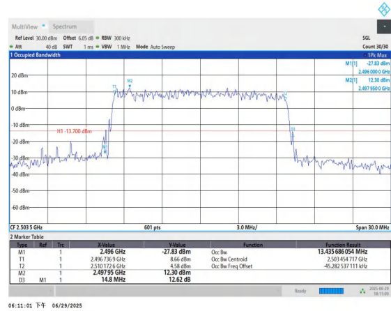
Band41-15MHz-16QAM-39725-75RB#0-PASS
