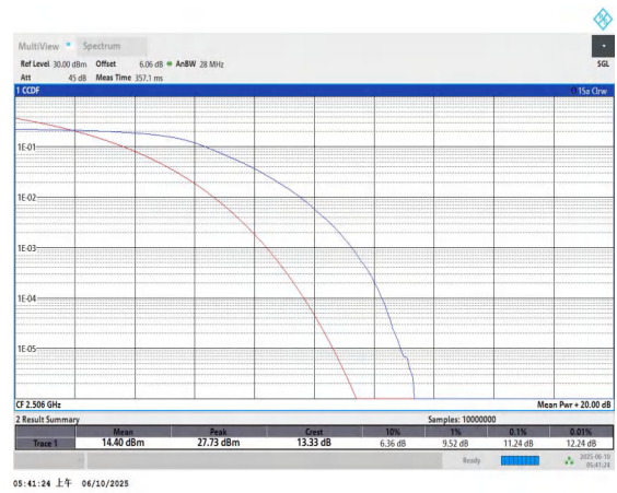
Band41-20MHz-QPSK-39750-100RB#0-PASS
