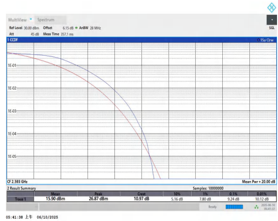
Band41-20MHz-QPSK-40620-100RB#0-PASS
