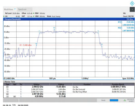
Band41-5MHz-16QAM-39675-25RB#0-PASS
