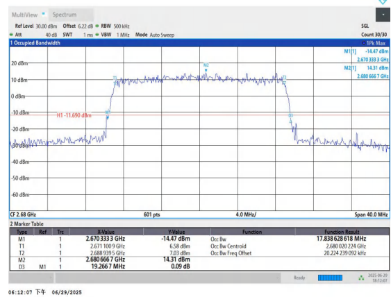
Band41-20MHz-16QAM-41490-100RB#0-PASS
