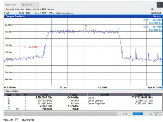
Band41-20MHz-16QAM-39750-100RB#0-PASS
