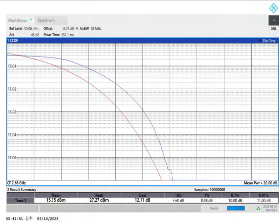
Band41-20MHz-QPSK-41490-100RB#0-PASS
