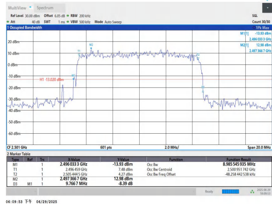
Band41-10MHz-16QAM-39700-50RB#0-PASS
