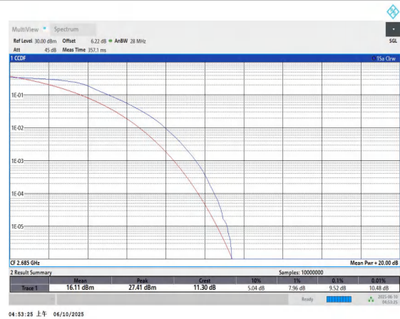
Band41-10MHz-QPSK-41540-50RB#0-PASS
