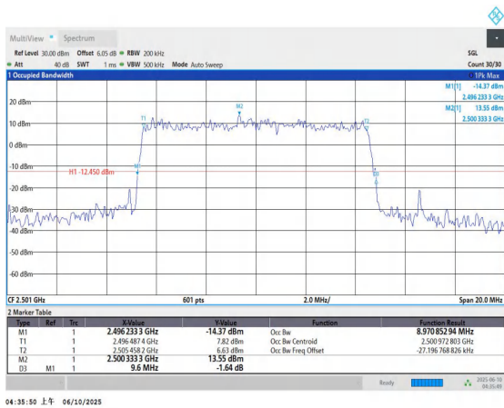
Band41-10MHz-QPSK-39700-50RB#0-PASS
