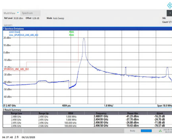
Band41-10MHz-QPSK-39700-1RB#0-PASS
