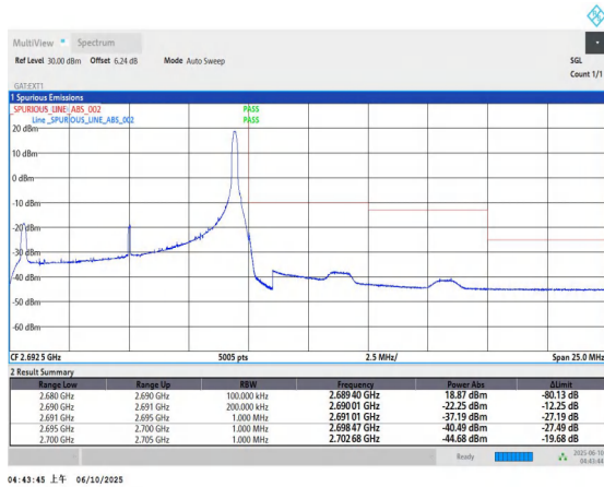
Band41-10MHz-QPSK-41540-1RB#49-PASS
