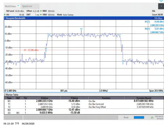
Band41-10MHz-16QAM-41540-50RB#0-PASS
