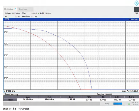
Band41-5MHz-QPSK-39675-25RB#0-PASS
