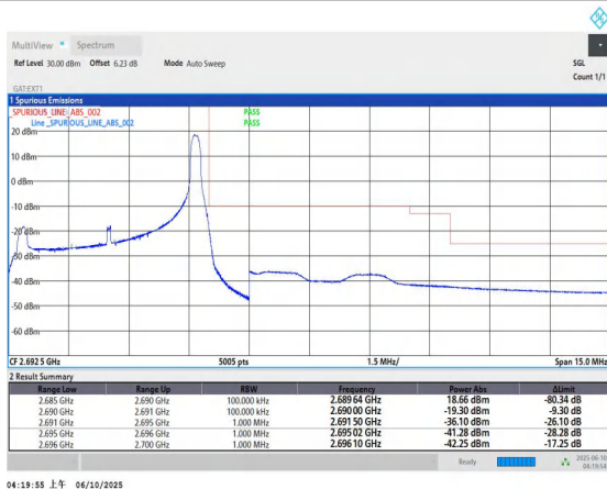
Band41-5MHz-QPSK-41565-1RB#24-PASS
