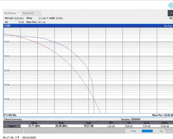
Band41-15MHz-QPSK-40620-1RB#0-PASS
