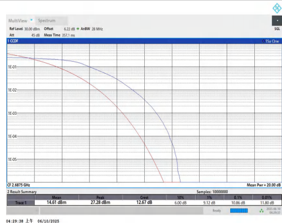
Band41-5MHz-QPSK-41565-25RB#0-PASS
