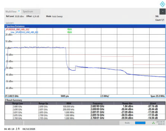
Band41-10MHz-QPSK-41540-50RB#0-PASS
