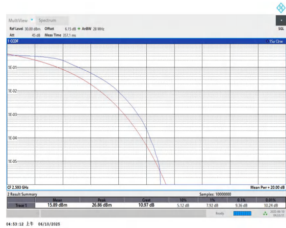
Band41-10MHz-QPSK-40620-50RB#0-PASS
