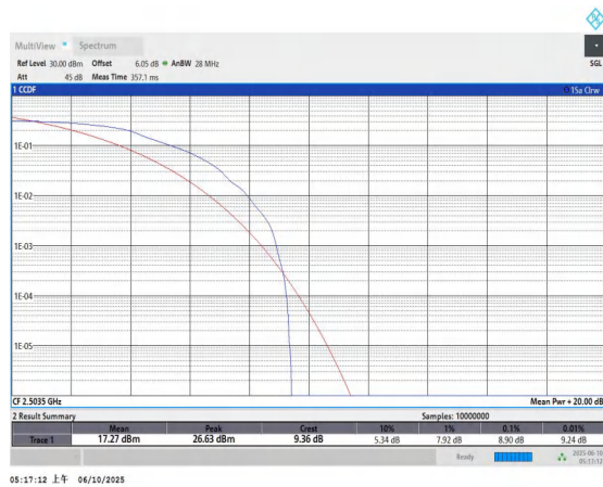
Band41-15MHz-QPSK-39725-1RB#0-PASS
