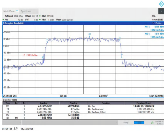
Band41-15MHz-QPSK-41515-75RB#0-PASS
