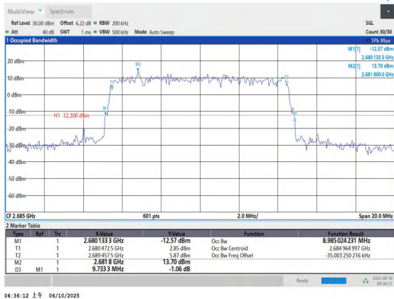
Band41-10MHz-QPSK-41540-50RB#0-PASS
