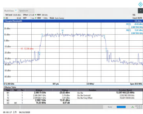
Band41-15MHz-QPSK-40620-75RB#0-PASS
