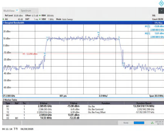
Band41-15MHz-16QAM-40620-75RB#0-PASS
