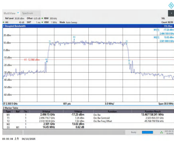
Band41-15MHz-QPSK-39725-75RB#0-PASS
