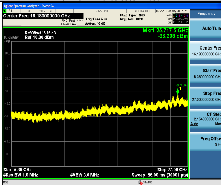
11N20SISO-Ant1-5200-30~5140-PASS
