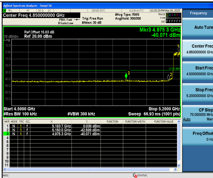
11AC40SISO-Ant1-5230-PASS
