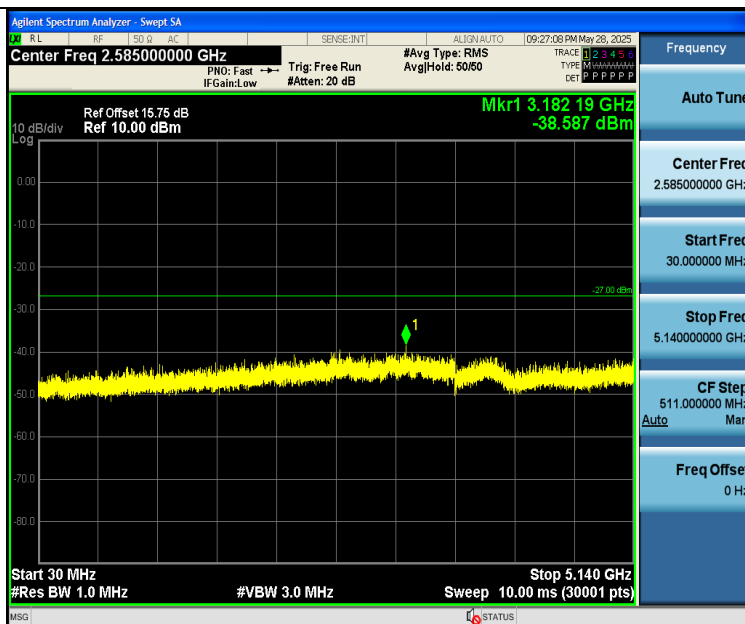
11N20SISO-Ant1-5180-5360~27000-PASS
