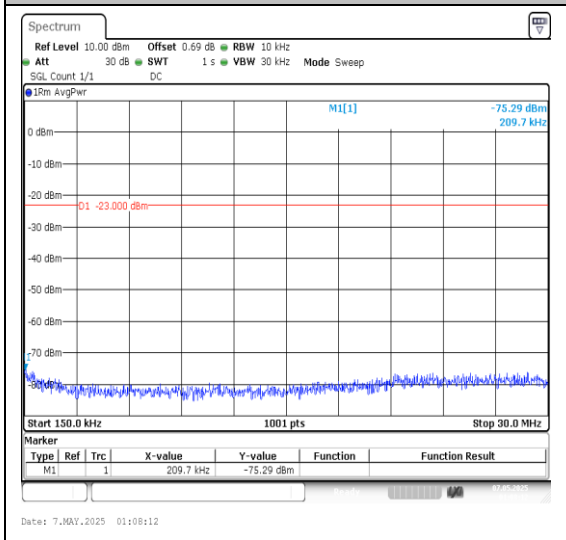
Band5-3MHz-16QAM-20415-1RB#0-0.15~30-PA SS
