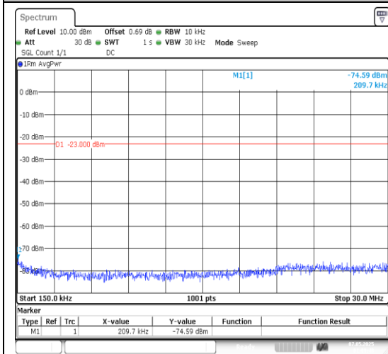
Band5-3MHz-QPSK-20525-1RB#0-3000~10000-PASS
