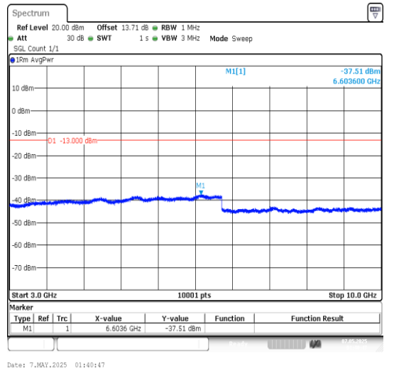
Band5-5MHz-16QAM-20525-1RB#0-30~100-PAS S
