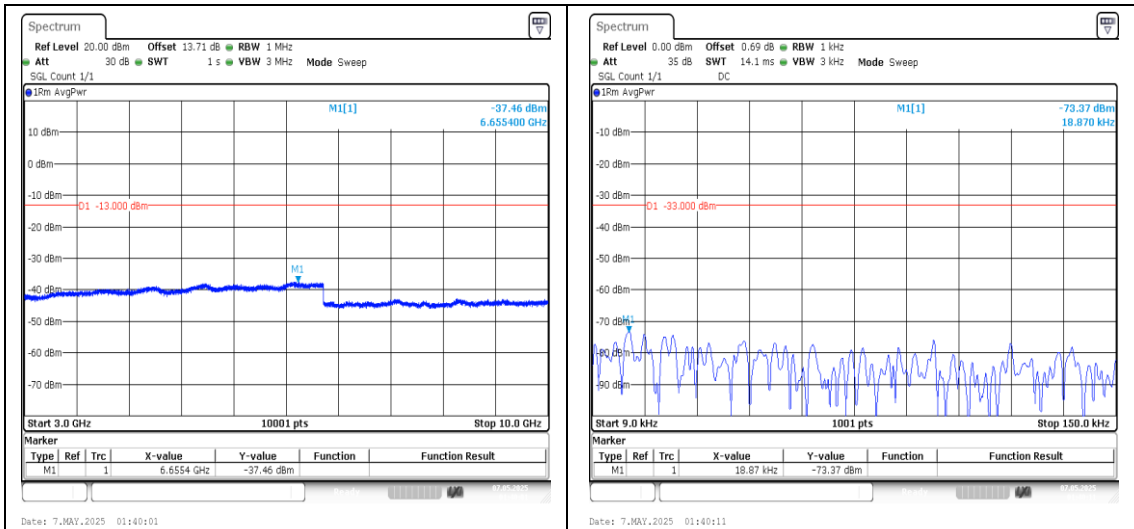
Band5-5MHz-QPSK-20525-1RB#0-3000~10000-PASS
