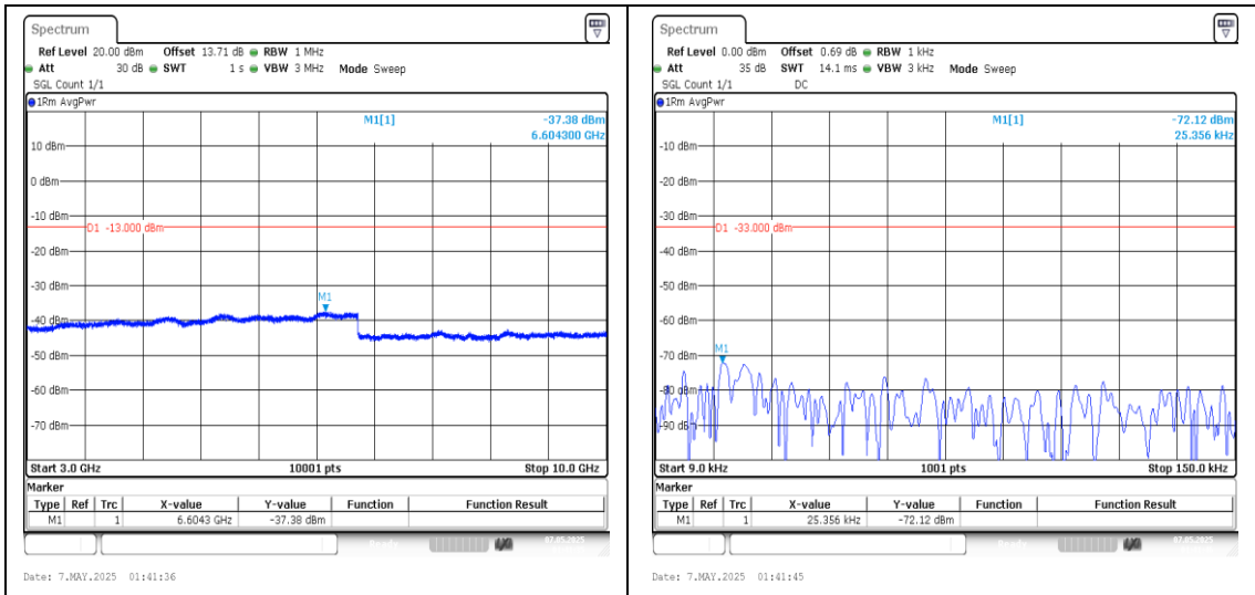
Band5-5MHz-QPSK-20625-1RB#0-3000~10000-PASS
