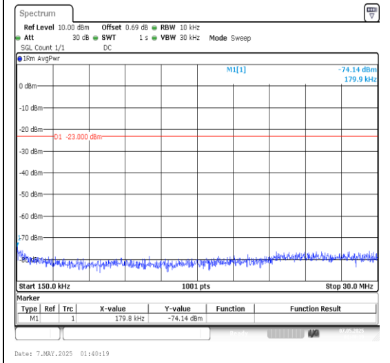
Band5-5MHz-16QAM-20525-1RB#0-0.15~30-PA SS
