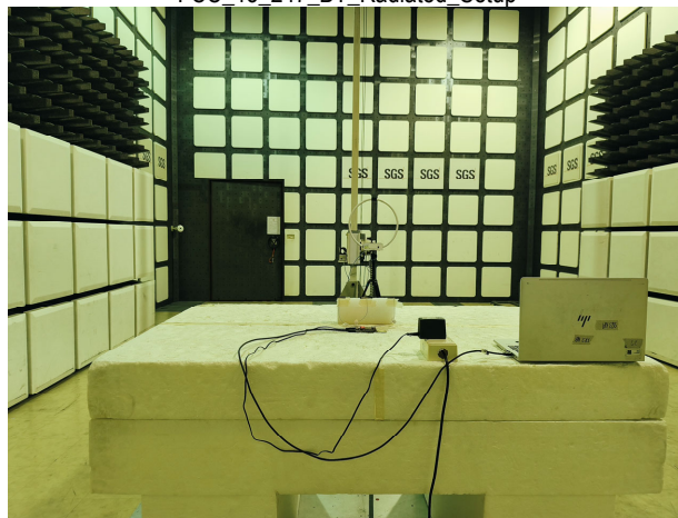
FCC 15 247 BT Radiated Setup
