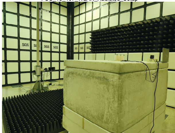
FCC 15 407 WLAN Radiated Setup
