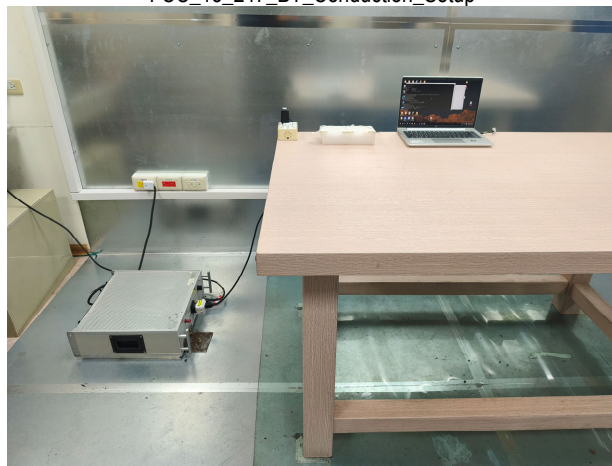
FCC_15_247_BT_Conduction_Setup
