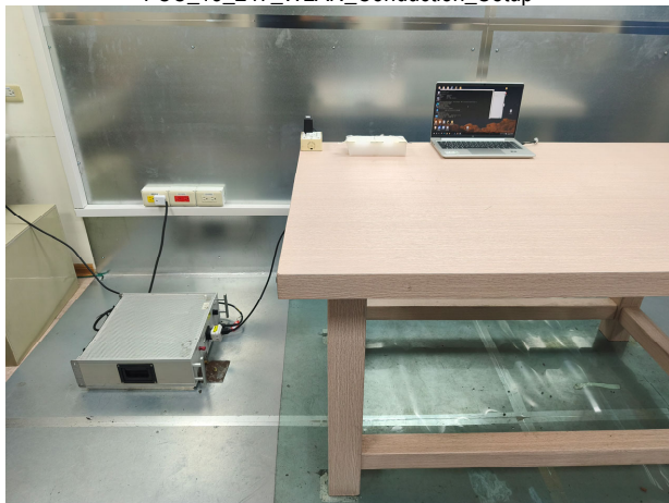
FCC_15_247_WLAN_Conduction_Setup
