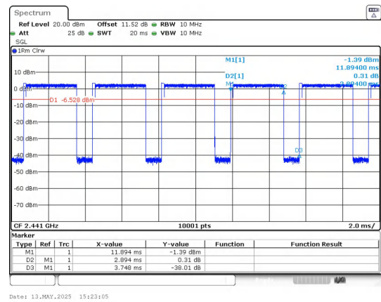
8DPSK(3-DH5)_Channel 39
