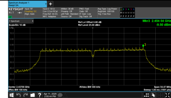
In-Band Reference Level IEEE 802.11n Channel 6 40MHz Antenna 0
