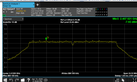
In-Band Reference Level IEEE 802.11g Channel 1 20MHz Antenna 0
