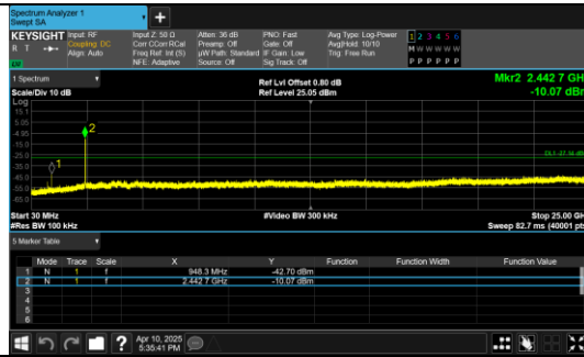
30.0 MHz - 25000.0 MHz IEEE 802.11n Channel 6 20MHz Antenna 0
