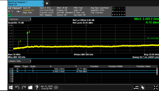
30.0 MHz - 25000.0 MHz IEEE 802.11n Channel 11 20MHz Antenna 0
