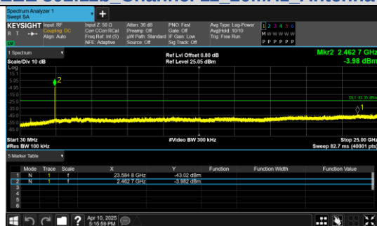
30.0 MHz - 25000.0 MHz IEEE 802.11b Channel 11 20MHz Antenna 0
