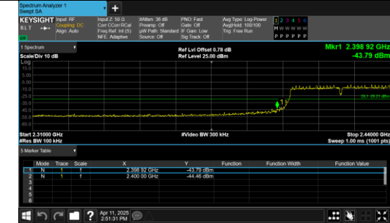
Out Of Band Emission IEEE 802.11n Channel 3 40MHz Antenna 0
