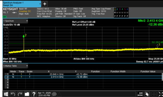
30.0 MHz - 25000.0 MHz IEEE 802.11n Channel 3 40MHz Antenna 0
