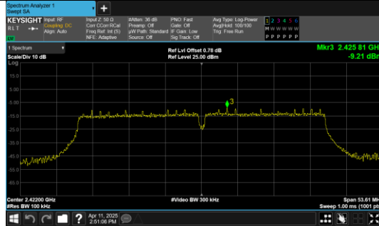
In-Band Reference Level IEEE 802.11n Channel 3 40MHz Antenna 0
