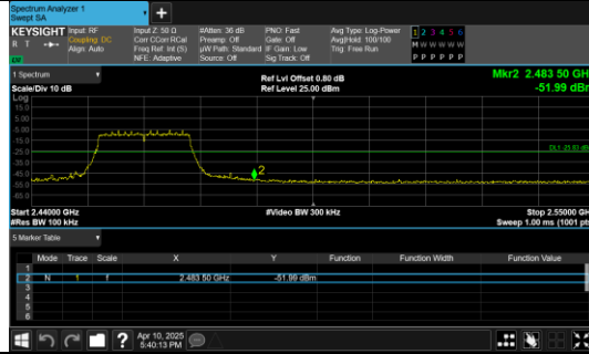
Out Of Band Emission IEEE 802.11n Channel 11 20MHz Antenna 0
