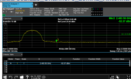
Out Of Band Emission
