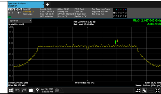
In-Band Reference Level IEEE 802.11n Channel 11 20MHz Antenna 0
