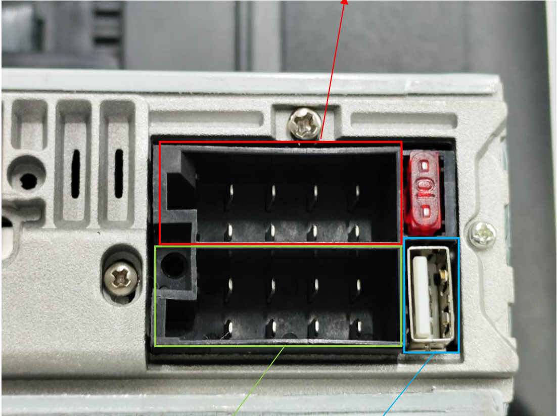
Power Interface
