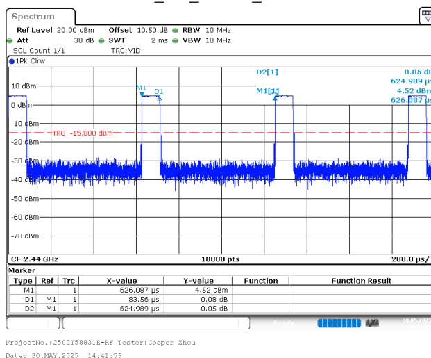
BLE_1M_Middle_Channel
