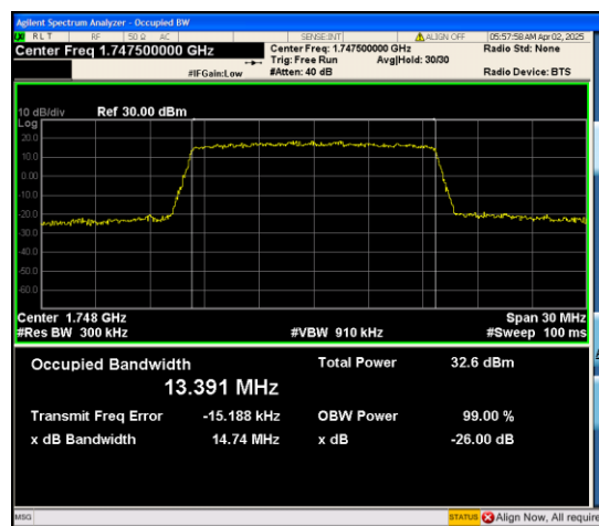
Band4-15MHz-QPSK-20325-75RB#0-PASS
