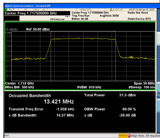
Band4-15MHz-16QAM-20025-75RB#0-PASS
