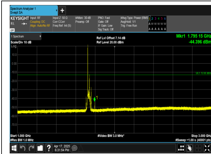
Band4-20MHz-QPSK-20175-1RB#0-1000~3000-PASS
