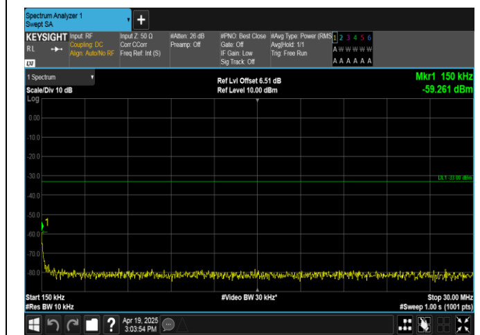
Band4-15MHz-16QAM-20175-75RB#0-0.15~30-PASS
