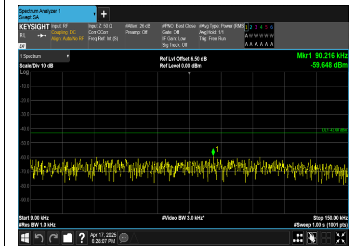
Band4-20MHz-16QAM-20050-1RB#0-0.009~0.15-PASS
