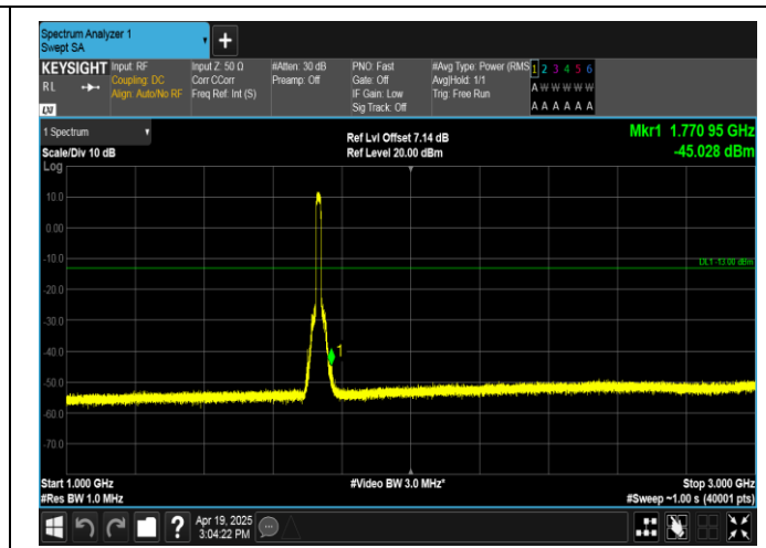
Band4-15MHz-16QAM-20175-75RB#0-1000~3000-PASS
