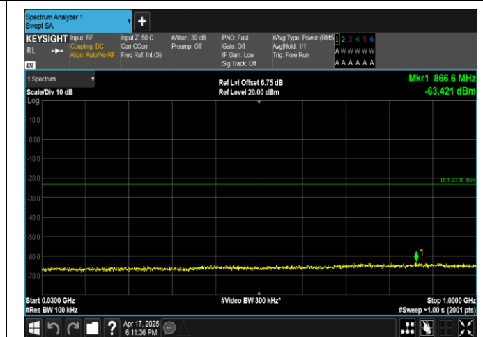
Band4-15MHz-16QAM-20325-1RB#0-30~1000-PASS
