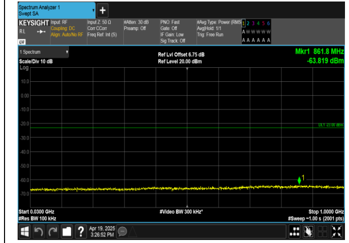
Band4-20MHz-QPSK-20175-100RB#0-30~1000-PASS
