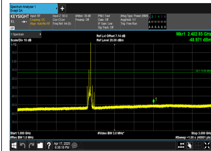
Band4-20MHz-QPSK-20300-1RB#99-1000~3000-PASS
