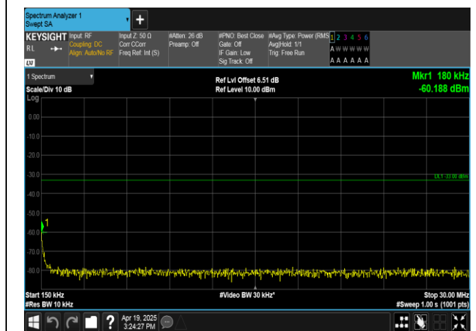
Band4-20MHz-QPSK-20050-100RB#0-0.15~30-PASS
