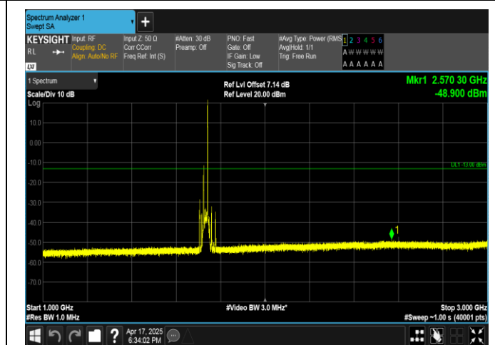
Band4-20MHz-QPSK-20175-1RB#99-1000~3000-PASS
