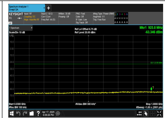
Band4-15MHz-16QAM-20175-1RB#74-30~1000-PASS
