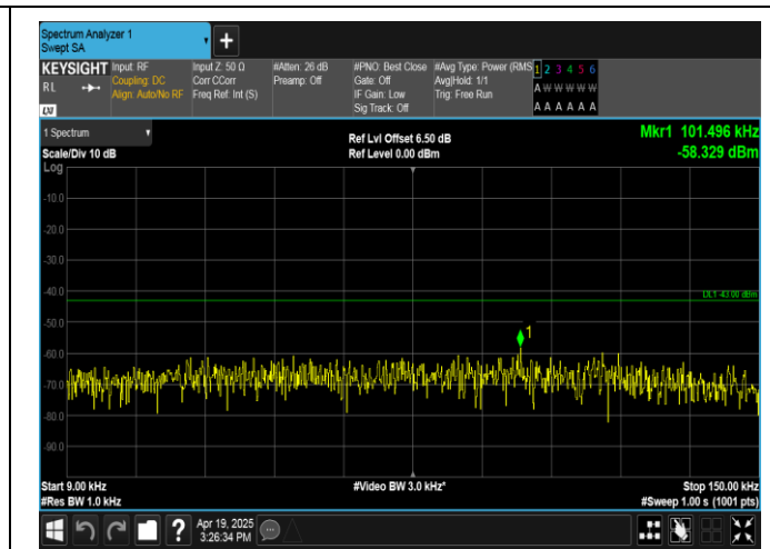
Band4-20MHz-QPSK-20175-100RB#0-0.009~0.15-PASS
