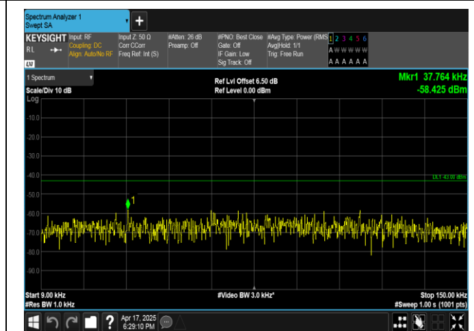
Band4-20MHz-QPSK-20050-1RB#99-0.009~0.15-PASS
