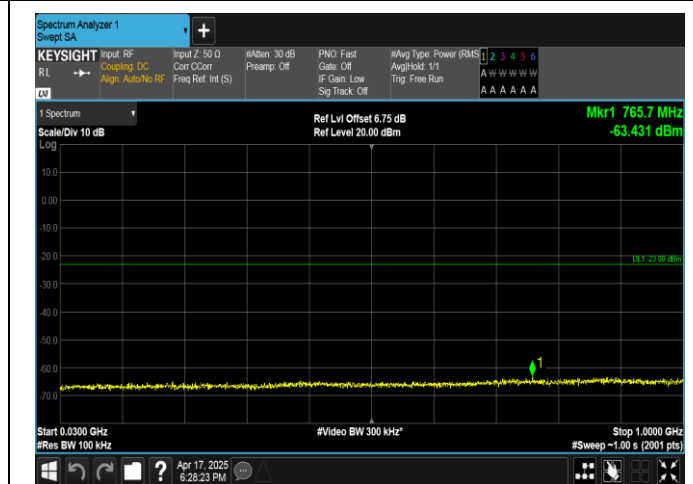
Band4-20MHz-16QAM-20050-1RB#0-30~1000-PASS
