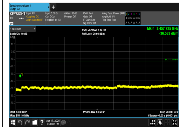
Band4-20MHz-QPSK-20050-1RB#99-3000~20000-PASS
