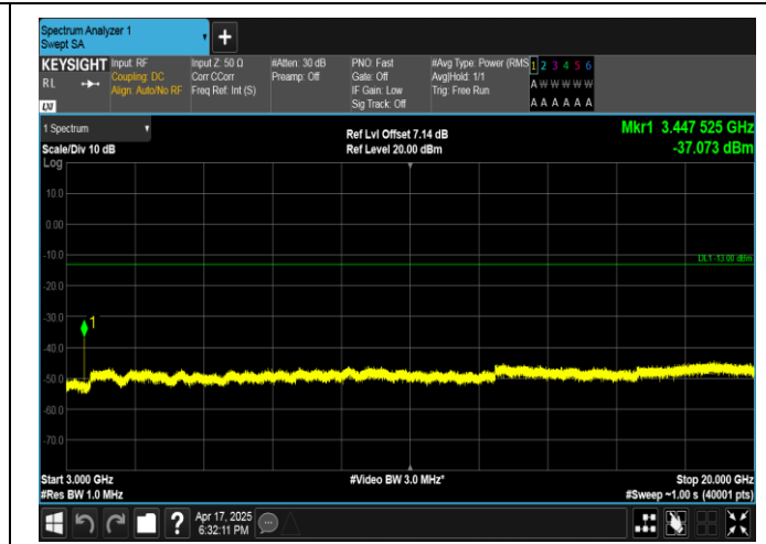
Band4-20MHz-QPSK-20175-1RB#0-3000~20000-PASS
