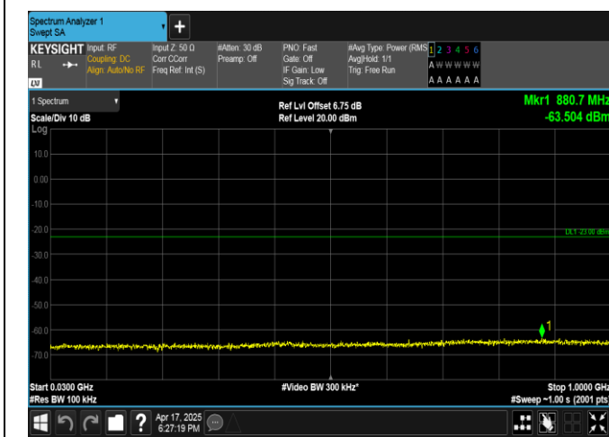
Band4-20MHz-QPSK-20050-1RB#0-30~1000-PASS
