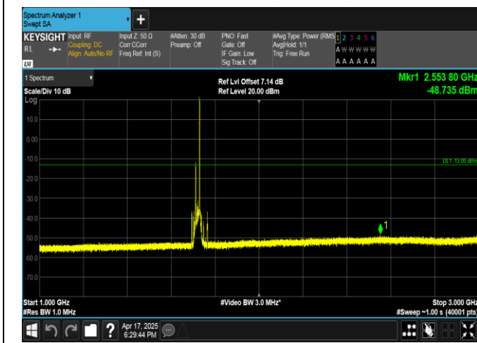
Band4-20MHz-QPSK-20050-1RB#99-1000~3000-PASS
