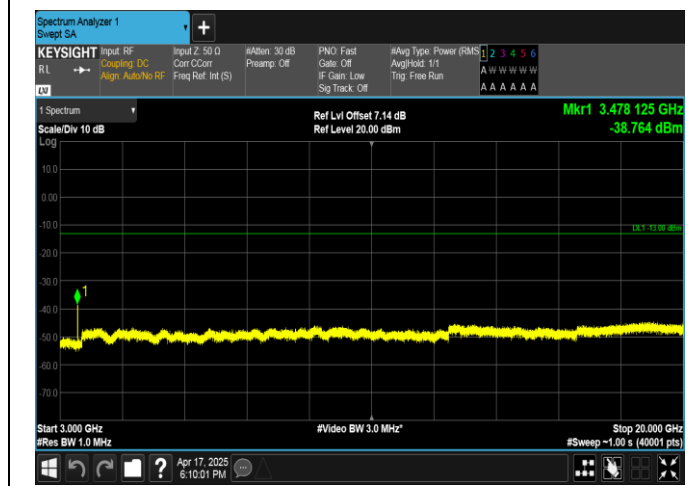
Band4-15MHz-16QAM-20175-1RB#74-3000~20000-PASS
