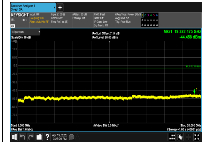
Band4-20MHz-QPSK-20175-100RB#0-3000~20000-PASS
