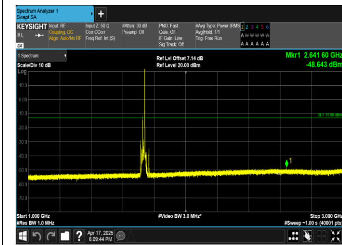
Band4-15MHz-16QAM-20175-1RB#74-1000~3000-PASS
