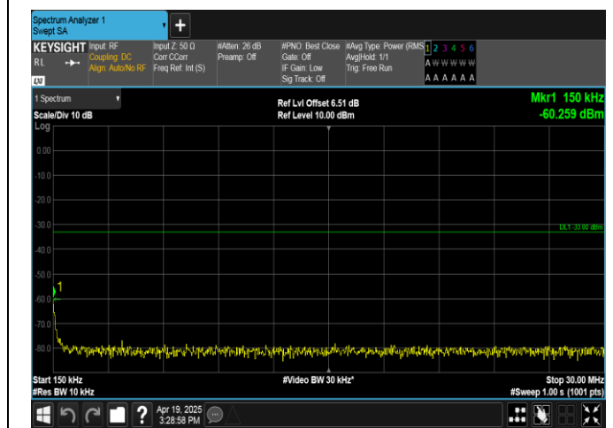
Band4-20MHz-QPSK-20300-100RB#0-0.15~30-PASS
