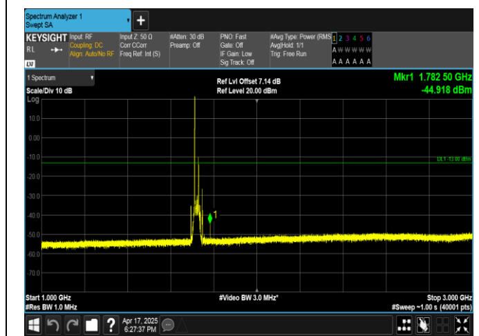
Band4-20MHz-QPSK-20050-1RB#0-1000~3000-PASS
