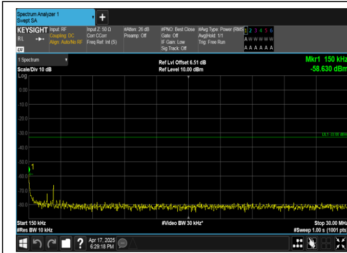
Band4-20MHz-QPSK-20050-1RB#99-0.15~30-PASS
