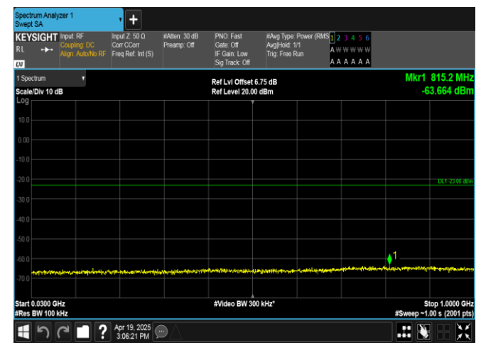
Band4-15MHz-16QAM-20325-75RB#0-30~1000-PASS
