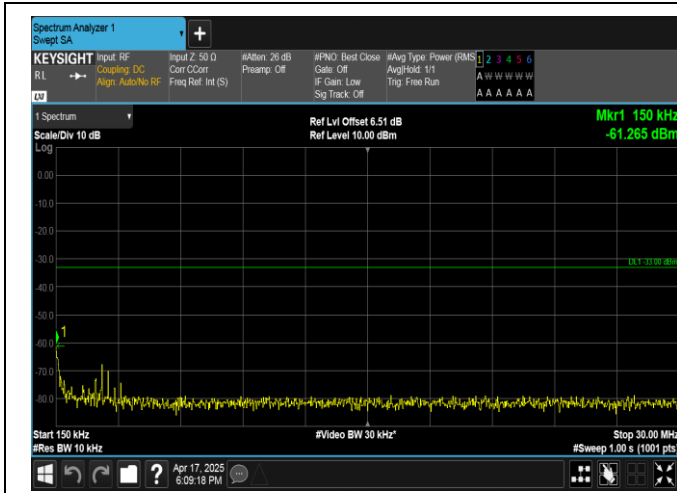
Band4-15MHz-16QAM-20175-1RB#74-0.15~30-PASS
