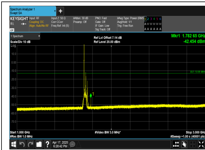
Band4-20MHz-16QAM-20050-1RB#0-1000~3000-PASS
