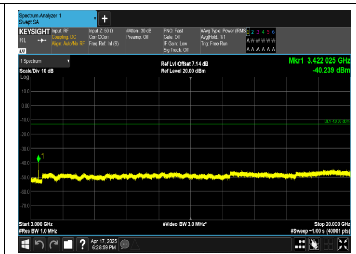
Band4-20MHz-16QAM-20050-1RB#0-3000~20000-PASS
