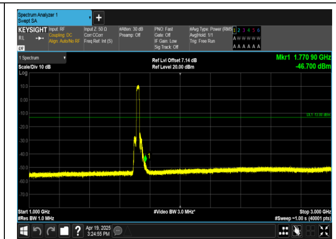
Band4-20MHz-QPSK-20050-100RB#0-1000~3000-PASS
