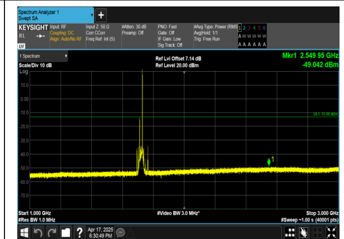
Band4-20MHz-16QAM-20050-1RB#99-1000~3000-PASS
