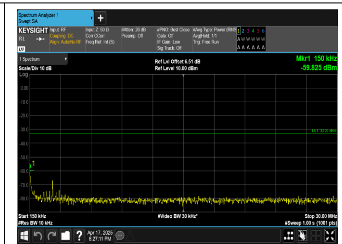
Band4-20MHz-QPSK-20050-1RB#0-0.15~30-PASS
