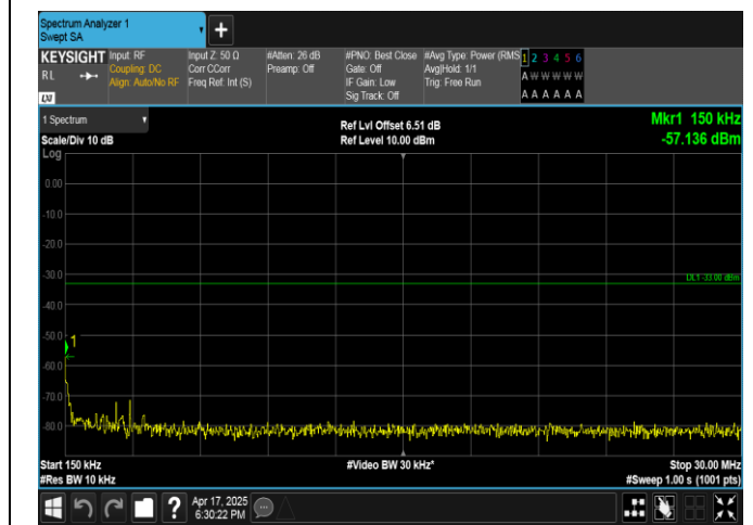
Band4-20MHz-16QAM-20050-1RB#99-0.15~30-PASS
