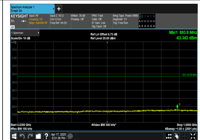
Band4-20MHz-QPSK-20175-1RB#0-30~1000-PASS
