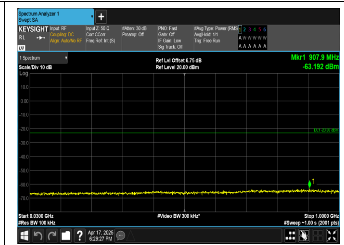
Band4-20MHz-QPSK-20050-1RB#99-30~1000-PASS
