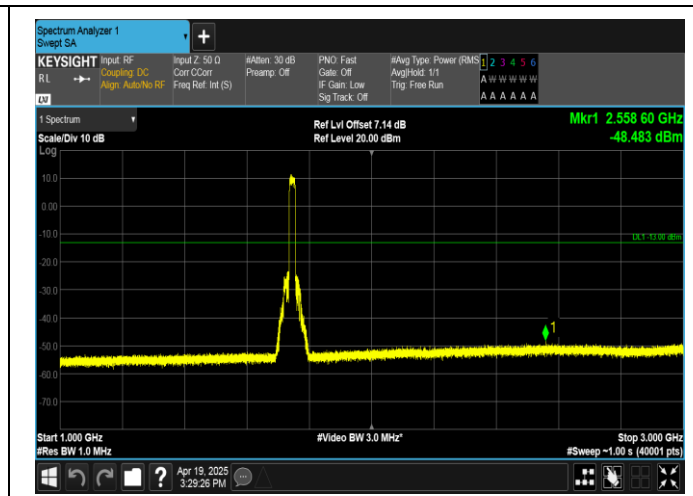
Band4-20MHz-QPSK-20300-100RB#0-1000~3000-PASS
