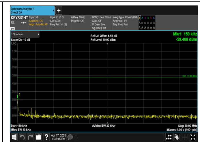
Band4-20MHz-QPSK-20300-1RB#0-0.15~30-PASS
