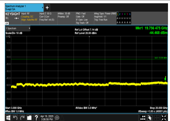
Band4-15MHz-16QAM-20325-75RB#0-3000~20000-PASS
