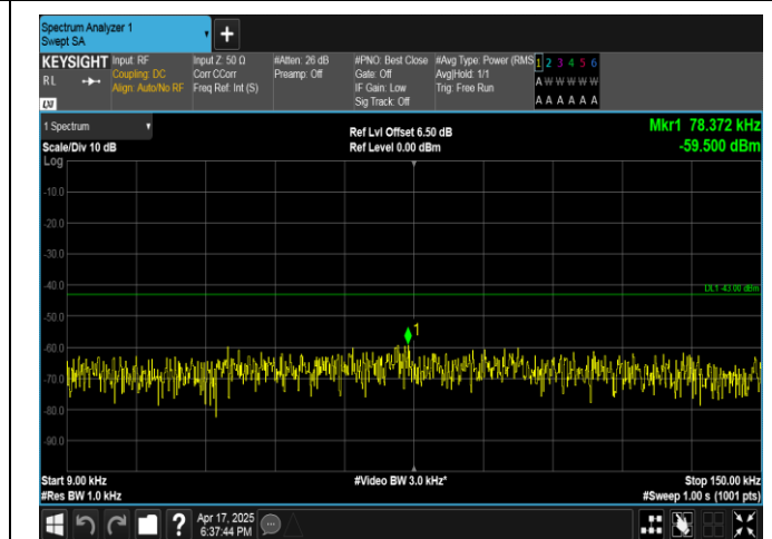
Band4-20MHz-QPSK-20300-1RB#99-0.009~0.15-PASS
