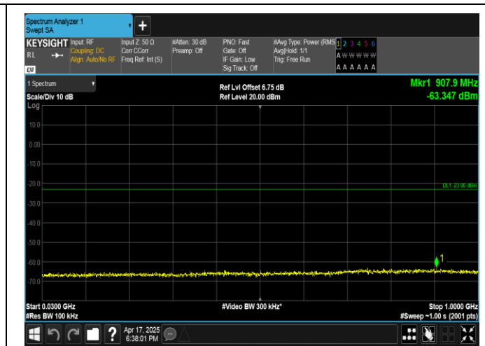
Band4-20MHz-QPSK-20300-1RB#99-30~1000-PASS
