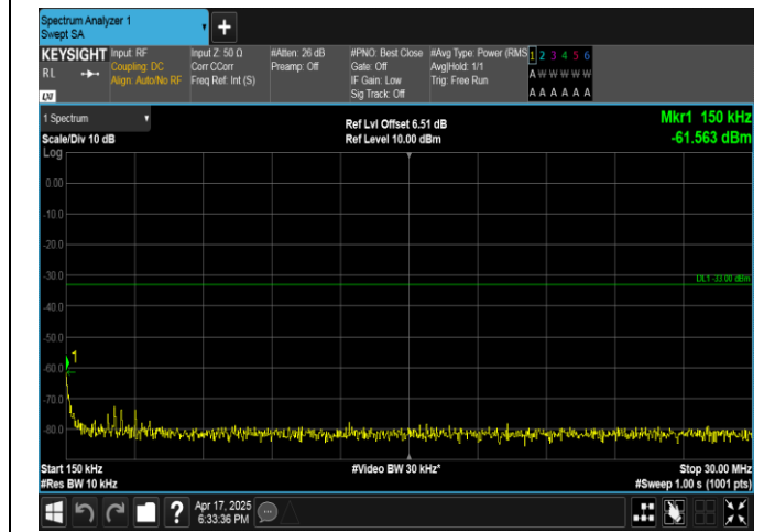
Band4-20MHz-QPSK-20175-1RB#99-0.15~30-PASS
