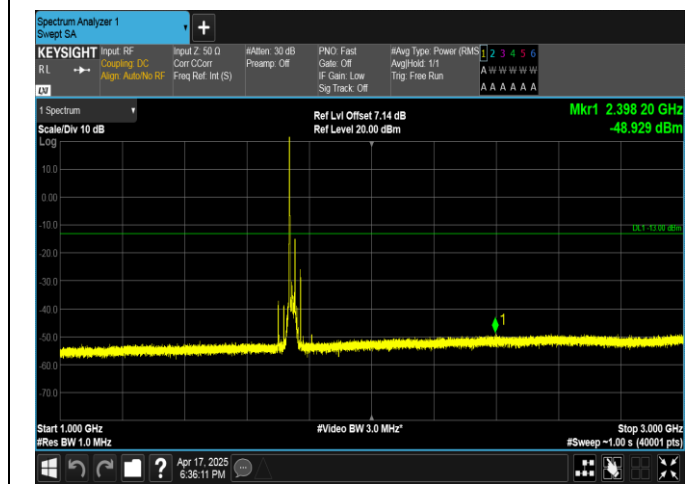
Band4-20MHz-QPSK-20300-1RB#0-1000~3000-PASS
