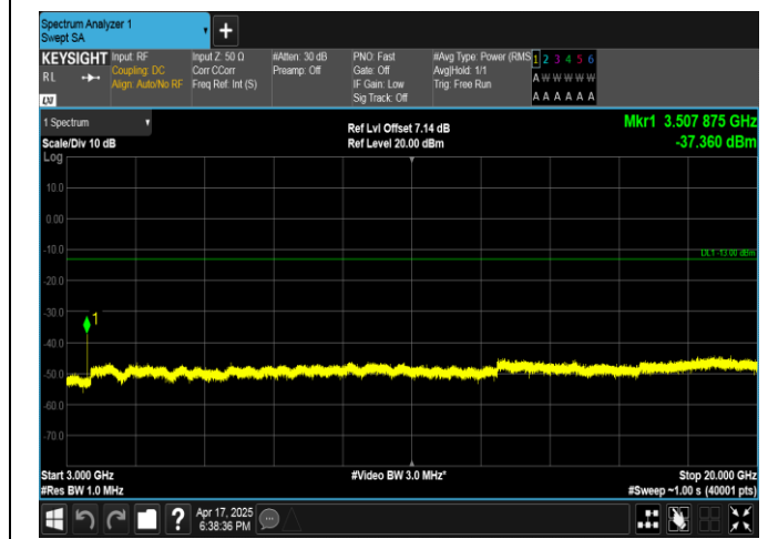
Band4-20MHz-QPSK-20300-1RB#99-3000~20000-PASS
