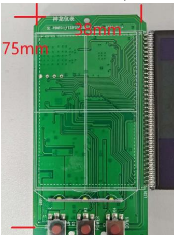
Antenna View (75mm*38mm)
