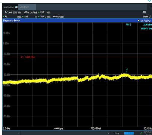
Band12-10MHz-QPSK-23095-1RB#0-3000~100 00-PASS
