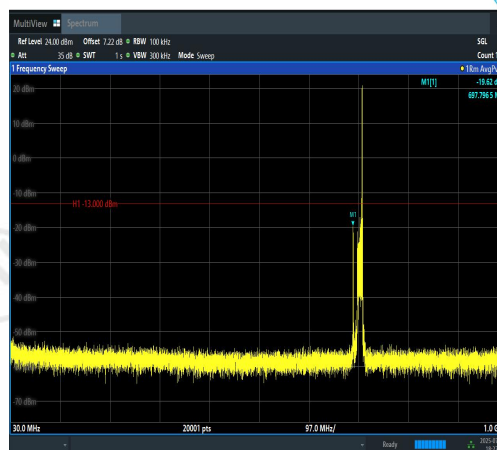
Band12-10MHz-QPSK-23130-1RB#49-30~1000- PASS
