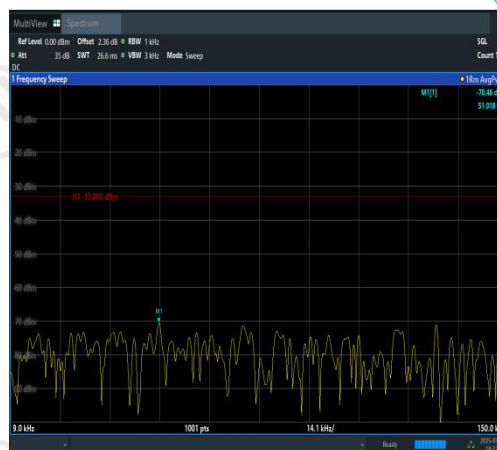
Band12-10MHz-QPSK-23130-1RB#49-0.009~0. 15-PASS
