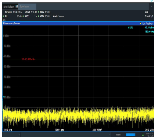
Band12-10MHz-QPSK-23095-1RB#49-0.15~30- PASS
