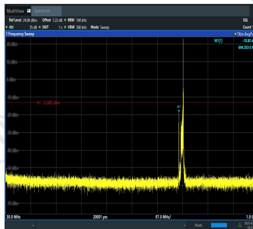
Band12-10MHz-QPSK-23095-1RB#49-30~1000- PASS
