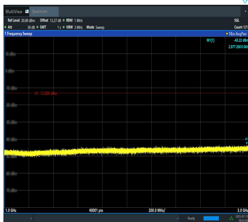
Band12-10MHz-16QAM-23095-1RB#0-1000~3000-PASS
