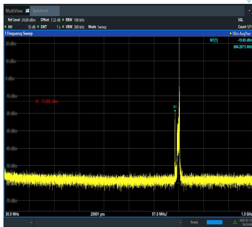
Band12-10MHz-16QAM-23095-1RB#49-30~1000-PASS
