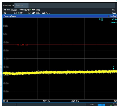
Band12-10MHz-QPSK-23095-1RB#0-1000~300 0-PASS
