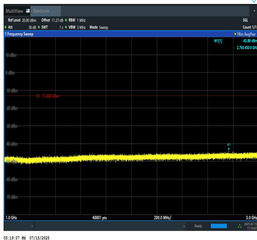
Band12-10MHz-16QAM-23095-50RB#0-1000~3 000-PASS
