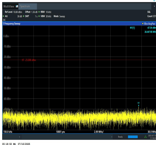
Band12-10MHz-16QAM-23095-50RB#0-0.15~30 -PASS
