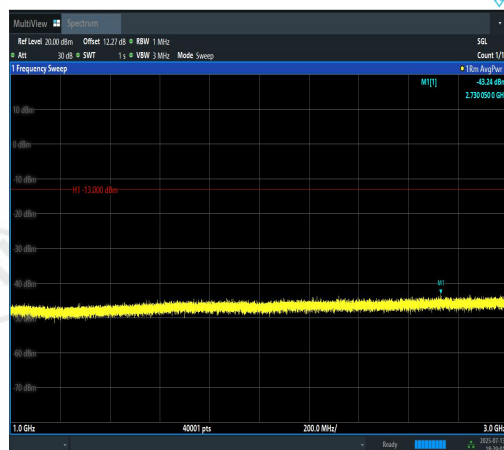
Band12-10MHz-QPSK-23130-50RB#0-1000~30 00-PASS
