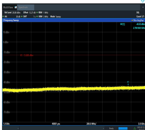
Band12-10MHz-QPSK-23095-1RB#49-1000~30 00-PASS
