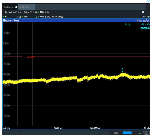
Band12-10MHz-16QAM-23095-1RB#49-3000~10000-PASS
