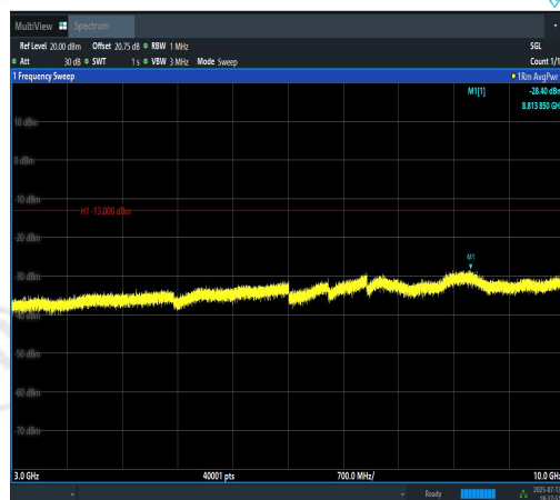
Band12-10MHz-QPSK-23130-1RB#49-3000~10 000-PASS
