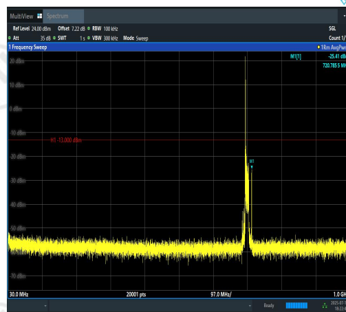
Band12-10MHz-16QAM-23095-1RB#0-30~1000-PASS
