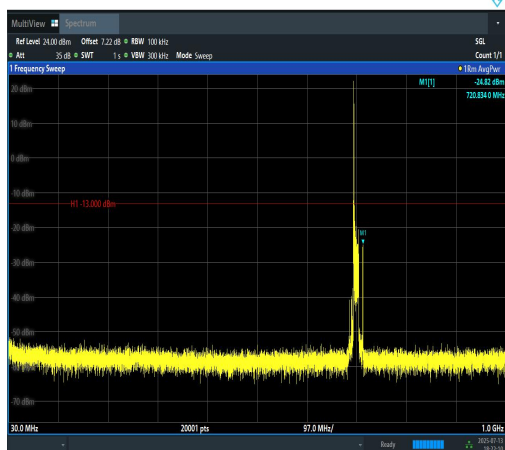
Band12-10MHz-QPSK-23095-1RB#0-30~1000-P ASS
