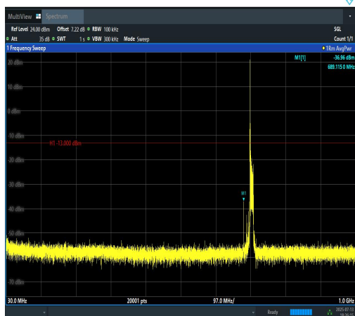
Band12-10MHz-QPSK-23130-1RB#0-30~1000-P ASS
