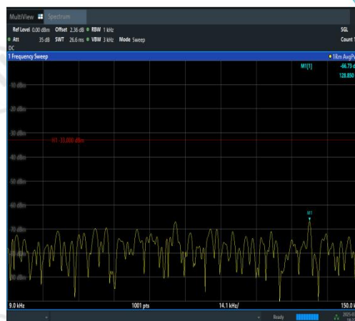
Band12-10MHz-QPSK-23095-1RB#49-0.009~0. 15-PASS
