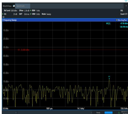
Band12-10MHz-QPSK-23130-50RB#0-0.009~0.15 15-PASS
