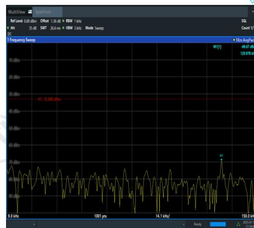
Band12-10MHz-16QAM-23095-50RB#0-0.009~0.15-PASS
