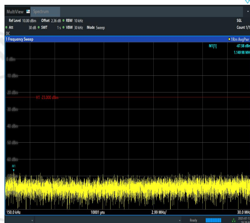
Band12-10MHz-QPSK-23130-50RB#0-0.15~30 PASS
