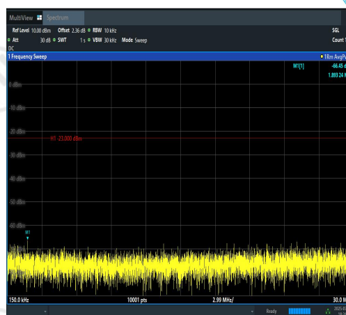
Band12-10MHz-QPSK-23095-50RB#0-0.15~30 PASS
