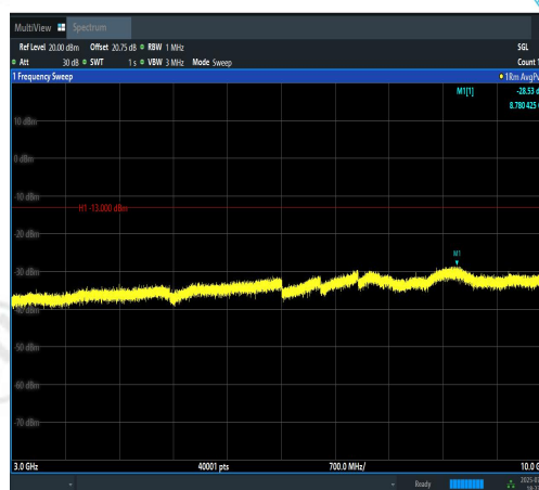
Band12-10MHz-QPSK-23095-1RB#49-3000~10 000-PASS
