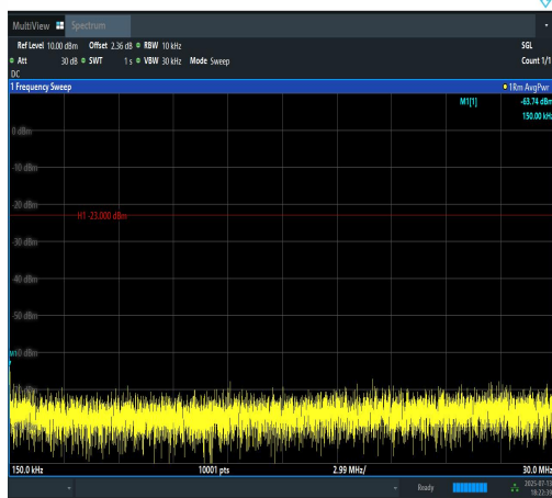
Band12-10MHz-16QAM-23095-1RB#0-0.15~30-PASS
