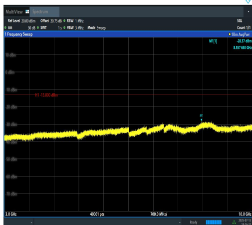
Band12-10MHz-QPSK-23130-1RB#0-3000~100 00-PASS
