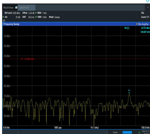
Band12-10MHz-QPSK-23095-50RB#0-0.009~0.15 15-PASS
