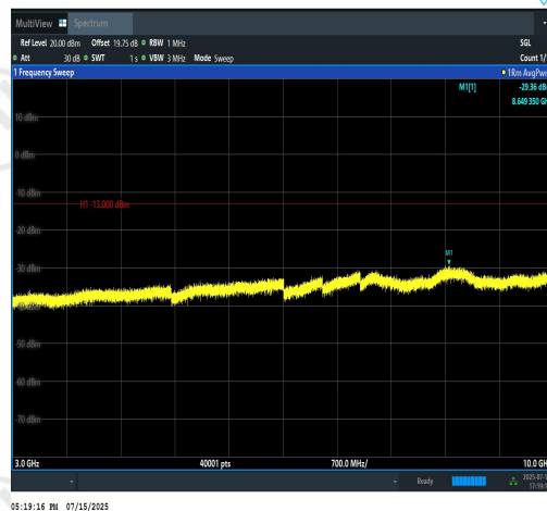
Band12-10MHz-16QAM-23095-50RB#0-3000~1 0000-PASS
