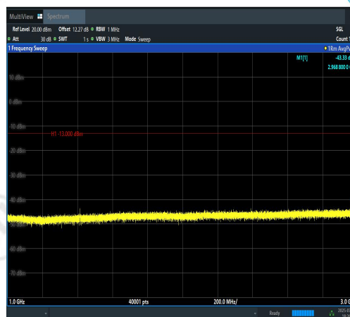
Band12-10MHz-QPSK-23130-1RB#0-1000~300 0-PASS
