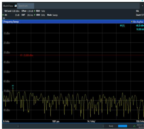
Band12-10MHz-16QAM-23095-1RB#49-0.009~0.15-PASS
