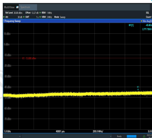
Band12-10MHz-QPSK-23095-50RB#0-1000~30 00-PASS
