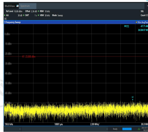
Band12-10MHz-16QAM-23095-1RB#49-0.15~30-PASS
