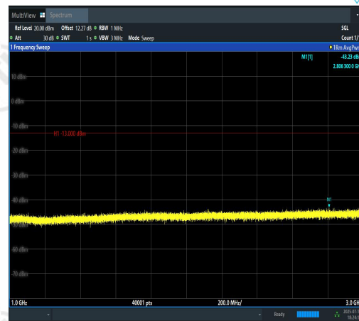
Band12-10MHz-16QAM-23095-1RB#49-1000~3000-PASS
