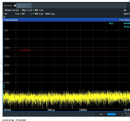
Band12-10MHz-QPSK-23130-1RB#0-0.15~30-P ASS
