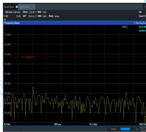
Band12-10MHz-16QAM-23095-1RB#0-0.009~0.15-PASS
