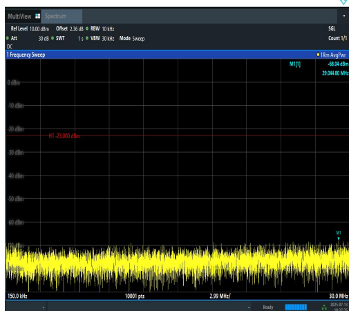
Band12-10MHz-QPSK-23130-1RB#49-0.15~30- PASS
