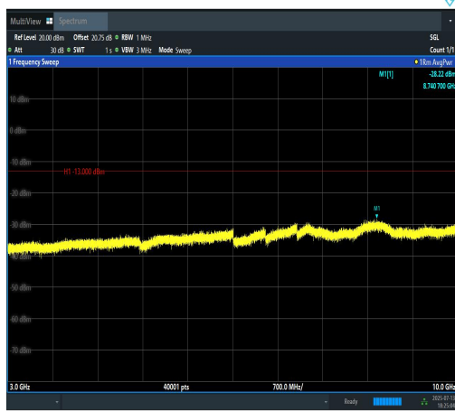
Band12-10MHz-QPSK-23095-50RB#0-3000~10000-PASS
