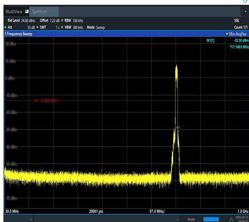
Band12-10MHz-QPSK-23130-50RB#0-30~1000 PASS
