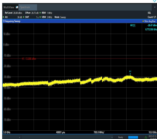
Band5-1.4MHz-QPSK-20407-6RB#0-3000~1000 0-PASS
