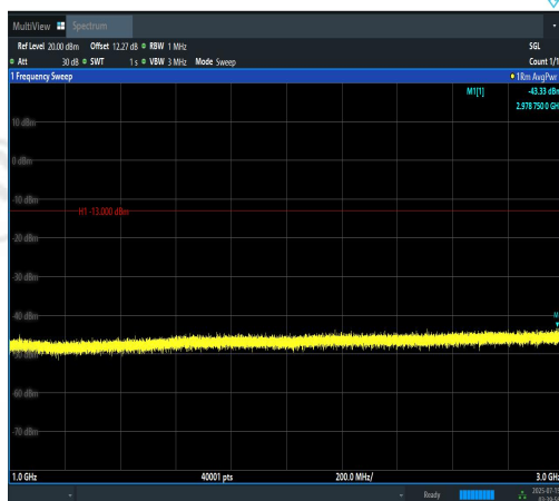
Band5-1.4MHz-QPSK-20407-6RB#0-1000~3000 -PASS
