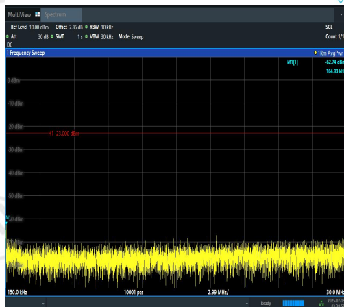
Band5-1.4MHz-16QAM-20407-1RB#5-0.15~30-P ASS
