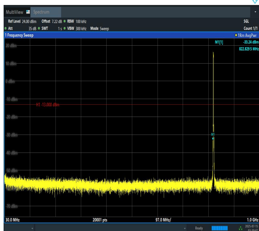
Band5-1.4MHz-QPSK-20407-6RB#0-30~1000-P ASS
