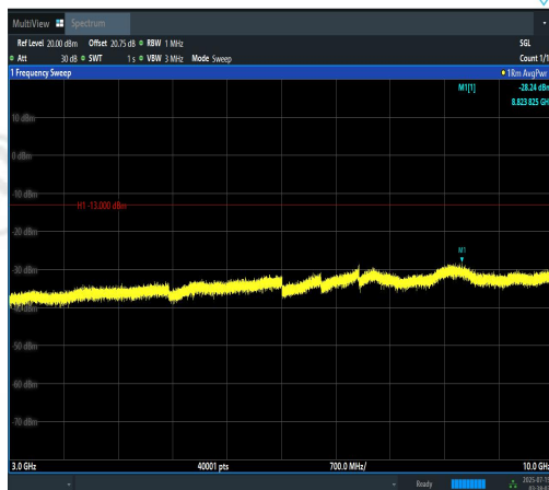
Band5-1.4MHz-16QAM-20407-1RB#0-3000~100 00-PASS
