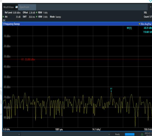
Band5-1.4MHz-16QAM-20407-1RB#0-0.009~0.1 5-PASS
