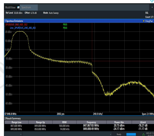
Band5-1.4MHz-16QAM-20643-1RB#0-PASS
