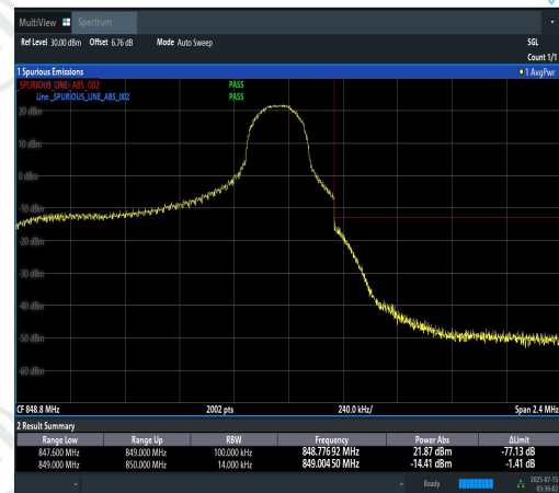
Band5-1.4MHz-QPSK-20643-1RB#5-PASS
