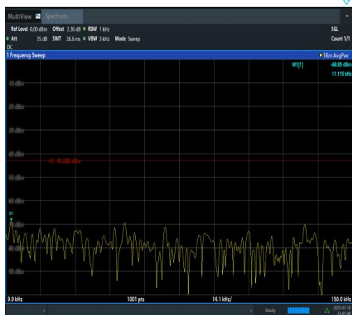
Band4-10MHz-16QAM-20000-1RB#49-0.009~0.15-PASS
