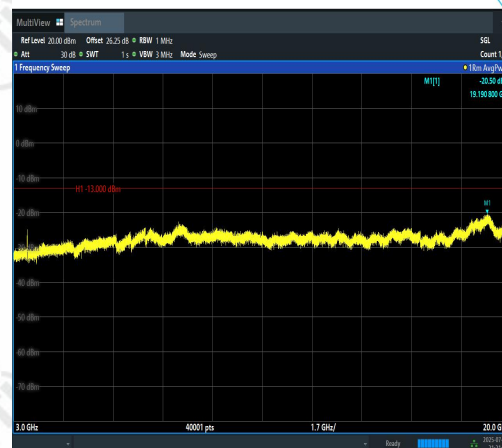
Band4-10MHz-16QAM-20175-50RB#0-3000~20000-PASS
