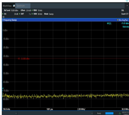
Band4-10MHz-16QAM-20000-1RB#0-0.15~30-P ASS
