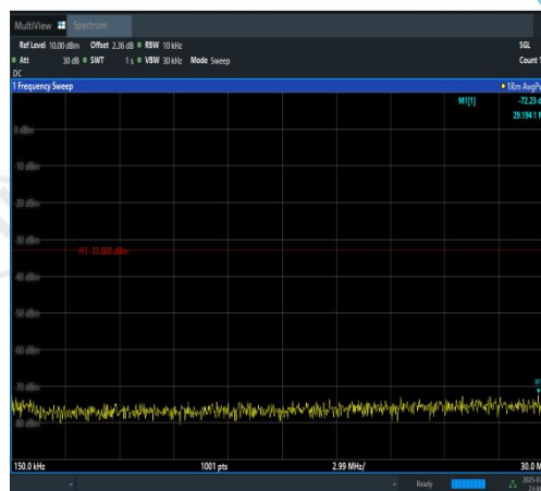
Band4-10MHz-QPSK-20175-1RB#0-0.15~30-PA SS
