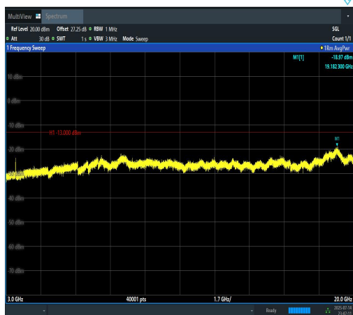
Band4-10MHz-QPSK-20175-50RB#0-3000~200 00-PASS
