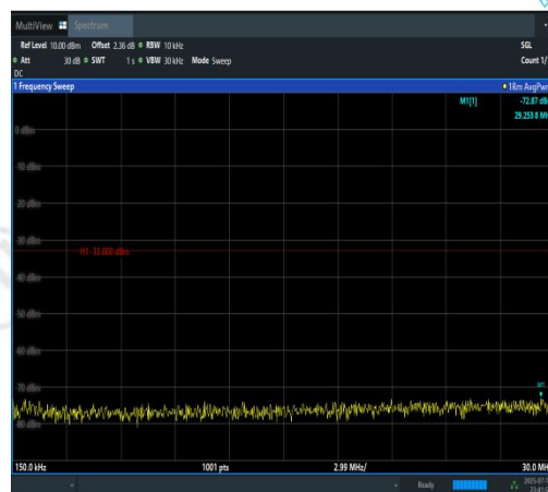
Band4-10MHz-16QAM-20000-1RB#49-0.15~30-PASS
