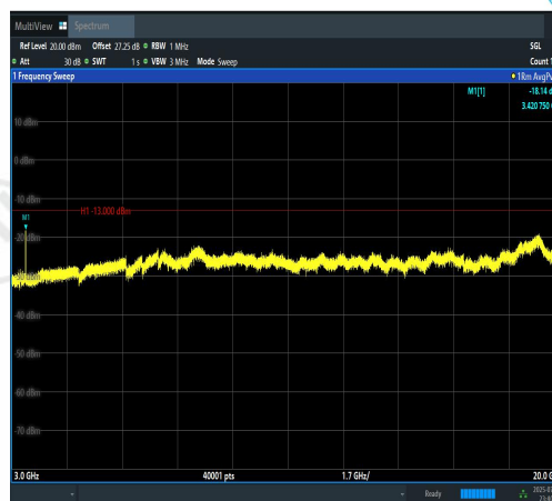
Band4-10MHz-16QAM-20000-1RB#0-3000~200 00-PASS
