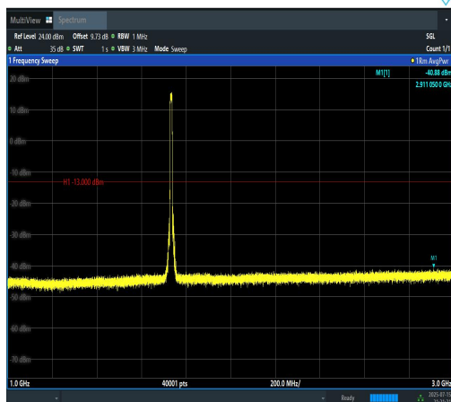
Band4-10MHz-16QAM-20175-50RB#0-1000~3000-PASS
