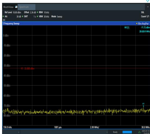
Band4-10MHz-16QAM-20000-50RB#0-0.15~30- PASS
