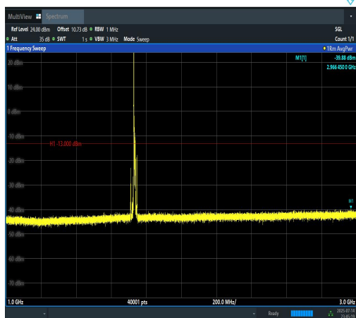
Band4-10MHz-16QAM-20175-1RB#0-1000~300 0-PASS
