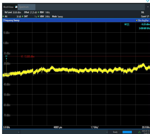
Band4-10MHz-16QAM-20000-1RB#49-3000~20000-PASS
