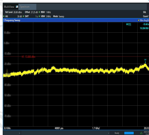
Band4-10MHz-16QAM-20000-50RB#0-3000~20 000-PASS
