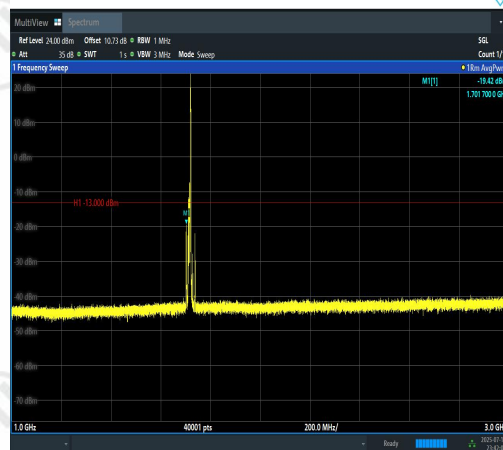
Band4-10MHz-16QAM-20000-1RB#49-1000~3000-PASS
