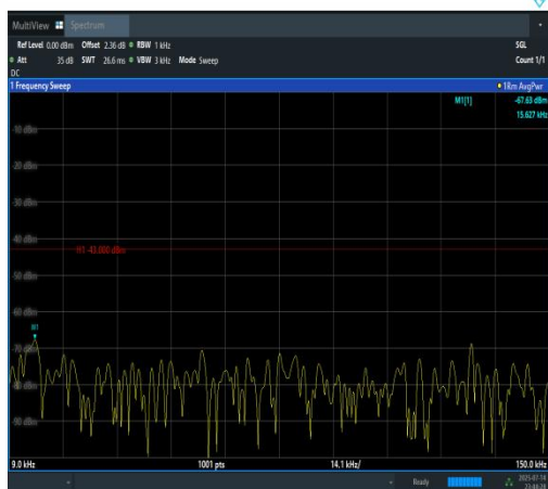
Band4-10MHz-QPSK-20175-1RB#0-0.009~0.15- PASS
