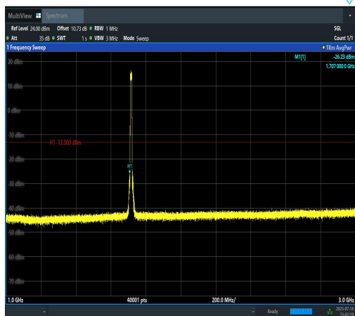
Band4-10MHz-16QAM-20000-50RB#0-1000~30 00-PASS
