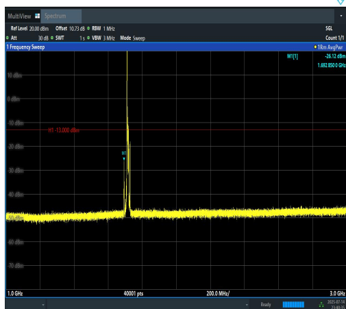
Band4-10MHz-16QAM-20000-1RB#0-1000~300 0-PASS
