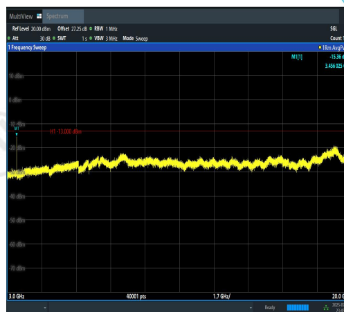
Band4-10MHz-16QAM-20175-1RB#0-3000~200 00-PASS
