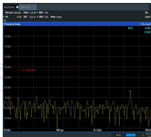
Band4-10MHz-16QAM-20175-1RB#0-0.009~0.1 5-PASS
