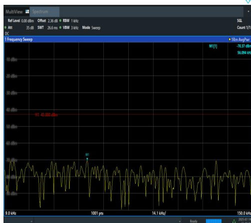
Band4-10MHz-QPSK-20350-1RB#0-0.009~0.15-PASS
