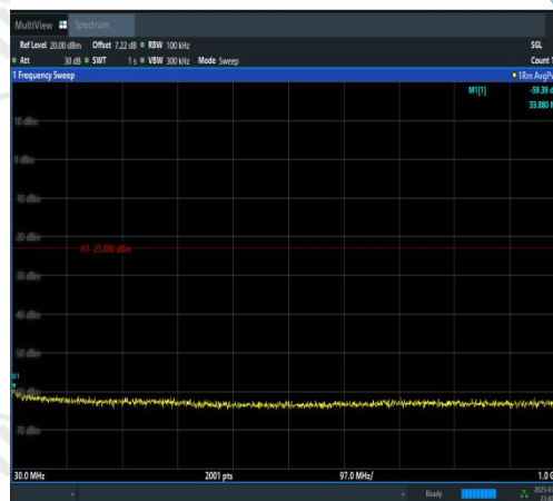
Band4-10MHz-16QAM-20000-1RB#0-30~1000-P ASS
