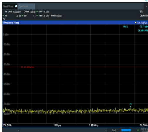
Band4-10MHz-16QAM-20175-50RB#0-0.15~30-PASS
