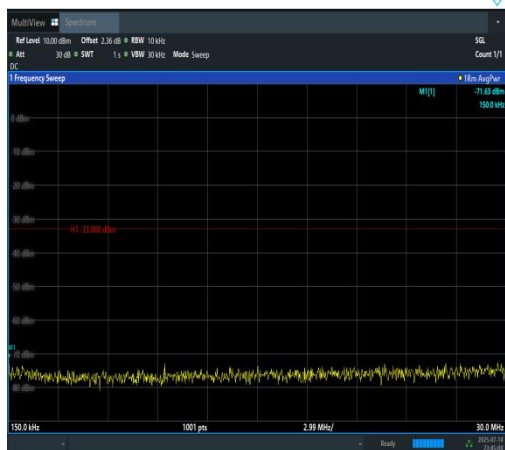
Band4-10MHz-16QAM-20175-1RB#0-0.15~30-P ASS
