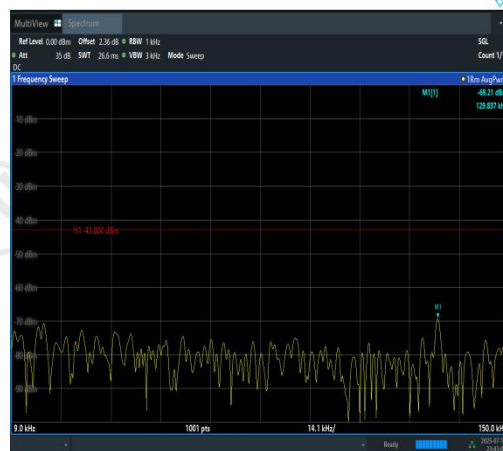
Band4-10MHz-16QAM-20000-50RB#0-0.009~0.15-PASS
