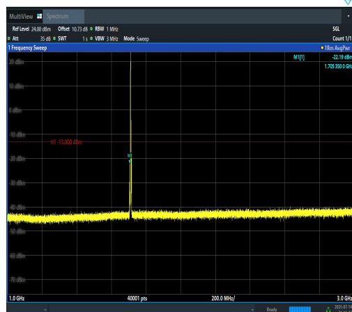
Band4-3MHz-16QAM-19965-1RB#0-1000~3000- PASS
