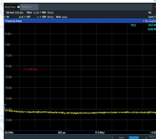
Band4-3MHz-16QAM-19965-1RB#0-30~1000-P ASS
