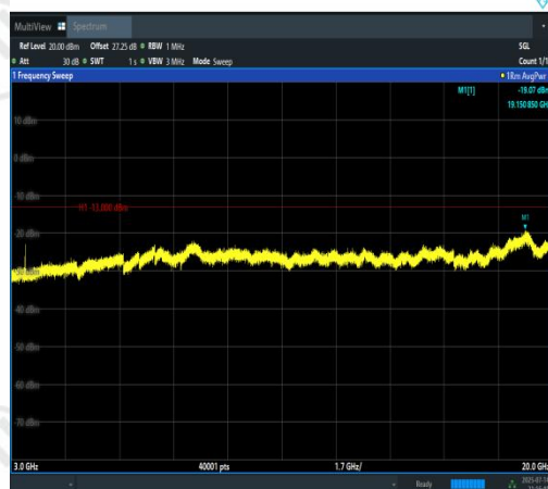
Band4-3MHz-16QAM-19965-15RB#0-3000~200 00-PASS
