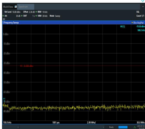
Band4-1.4MHz-16QAM-20175-6RB#0-0.15~30-P ASS
