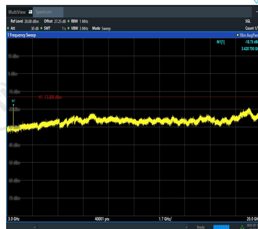
Band4-3MHz-16QAM-19965-1RB#0-3000~2000 0-PASS
