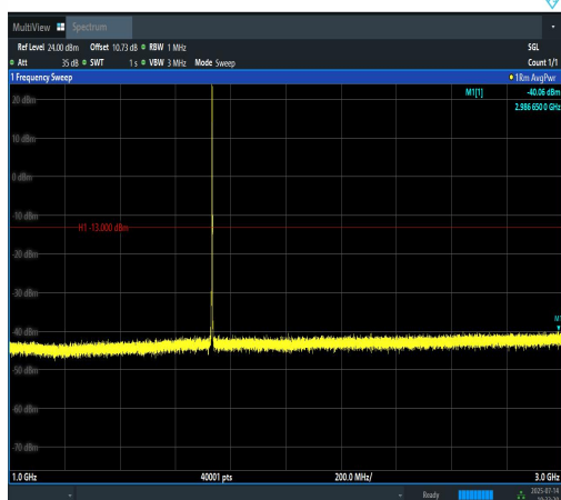
Band4-1.4MHz-16QAM-20175-6RB#0-1000~3000 0-PASS
