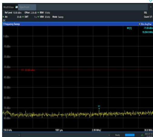
Band4-3MHz-16QAM-19965-15RB#0-0.15~30-P ASS
