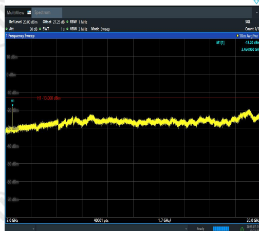
Band4-1.4MHz-16QAM-20175-6RB#0-3000~200 00-PASS
