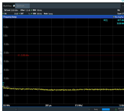
Band4-3MHz-16QAM-19965-15RB#0-30~1000-P ASS
