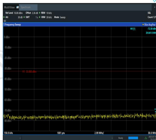
Band4-1.4MHz-QPSK-20393-1RB#0-0.15~30-P ASS
