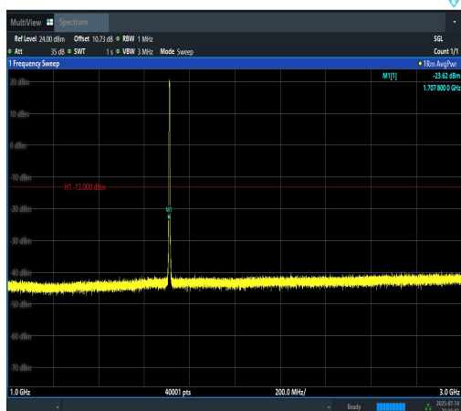
Band4-3MHz-16QAM-19965-15RB#0-1000~300 0-PASS
