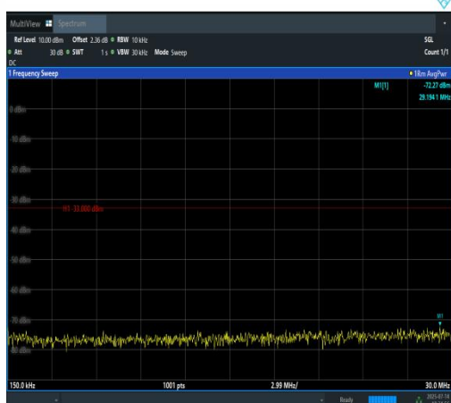
Band4-1.4MHz-QPSK-20393-1RB#5-0.15~30-P ASS
