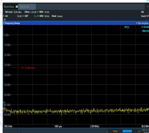
Band4-1.4MHz-QPSK-20393-6RB#0-0.15~30-P ASS
