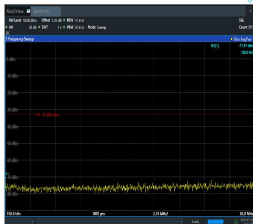
Band4-3MHz-16QAM-19965-1RB#0-0.15~30-PA SS
