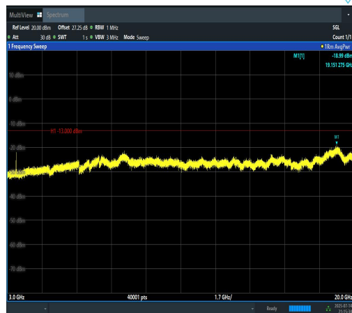
Band4-3MHz-QPSK-19965-15RB#0-3000~2000 0-PASS
