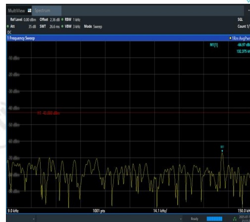
Band4-3MHz-16QAM-19965-1RB#0-0.009~0.15- PASS
