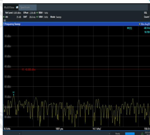
Band4-1.4MHz-QPSK-20393-1RB#5-0.009~0.15 -PASS
