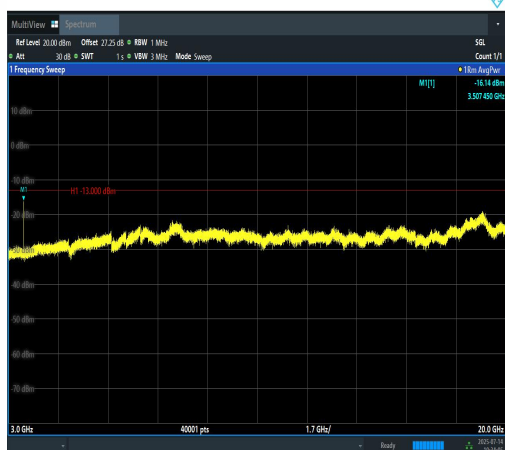
Band4-1.4MHz-QPSK-20393-1RB#0-3000~2000 0-PASS
