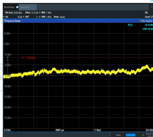
Band4-1.4MHz-QPSK-20393-1RB#5-3000~2000 0-PASS
