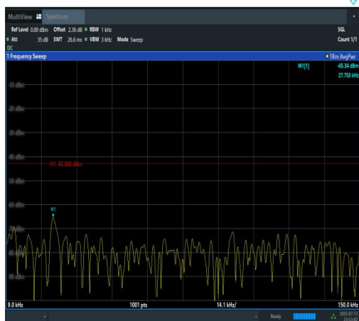
Band2-20MHz-QPSK-19100-1RB#0-0.009~0.15-PASS
