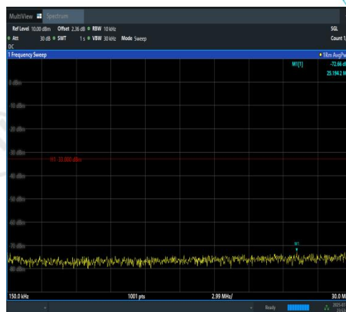
Band2-20MHz-QPSK-19100-1RB#0-0.15~30-PASS
