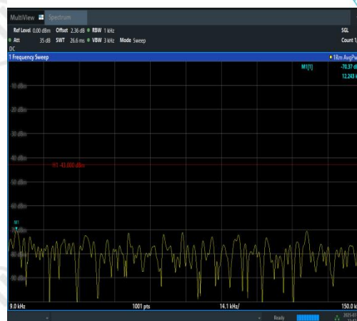
Band2-20MHz-QPSK-18900-1RB#99-0.009~0.1 5-PASS
