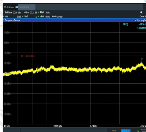
Band2-20MHz-16QAM-18900-100RB#0-3000~20000-PASS
