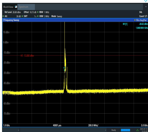
Band2-20MHz-16QAM-18700-1RB#0-1000~3000-PASS
