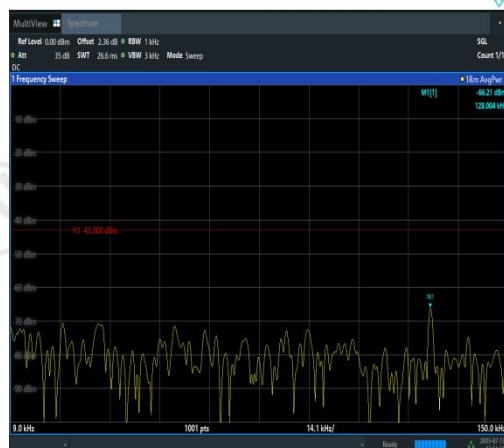
Band2-20MHz-16QAM-18900-100RB#0-0.009~0.15-PASS
