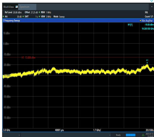
Band2-20MHz-QPSK-19100-1RB#0-3000~2000 0-PASS
