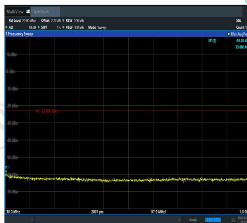
Band2-20MHz-16QAM-18900-100RB#0-30~100 0-PASS
