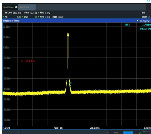
Band2-20MHz-16QAM-18900-100RB#0-1000~3000-PASS
