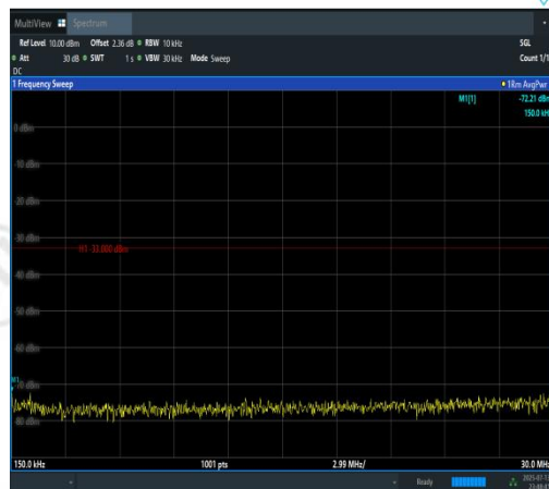
Band2-20MHz-16QAM-18900-1RB#99-0.15~30-PASS
