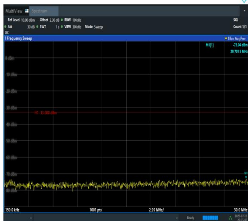
Band2-20MHz-16QAM-18700-1RB#0-0.15~30-PASS
