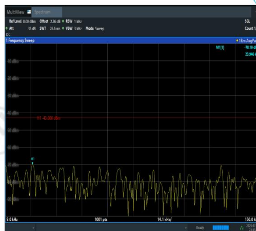
Band2-20MHz-16QAM-18700-1RB#0-0.009~0.15-PASS
