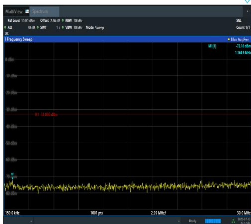
Band2-20MHz-16QAM-18900-100RB#0-0.15~30 -PASS
