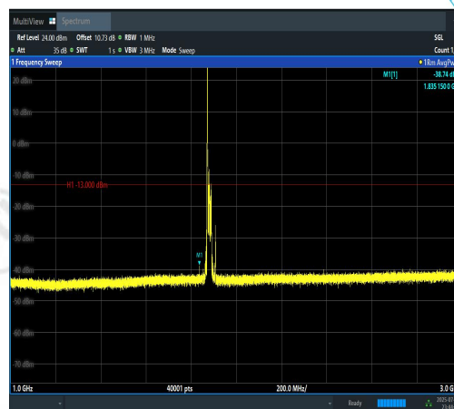
Band2-20MHz-QPSK-18900-1RB#0-1000~3000-P PASS
