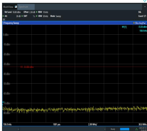
Band2-20MHz-QPSK-19100-1RB#99-0.15~30-P ASS
