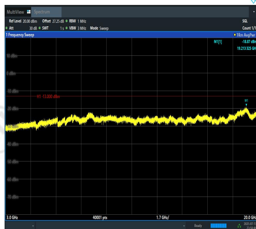
Band2-20MHz-QPSK-19100-1RB#99-3000~200 00-PASS
