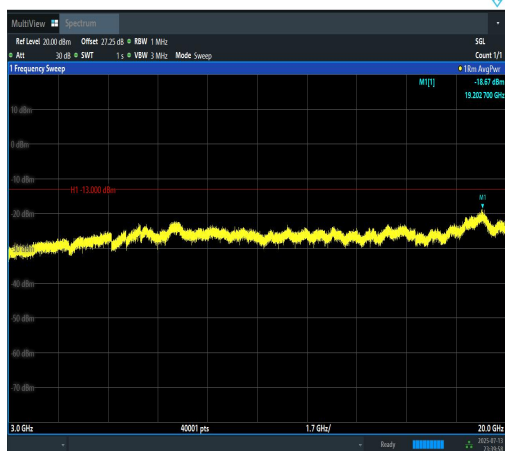
Band2-20MHz-QPSK-18700-100RB#0-3000~20000-PASS
