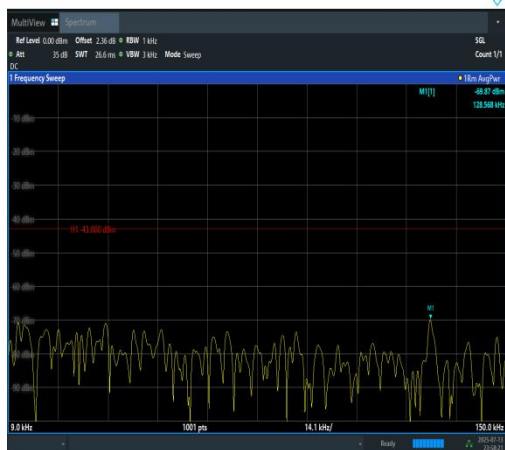
Band2-20MHz-QPSK-19100-100RB#0-0.009~0.15-PASS 15-PASS
