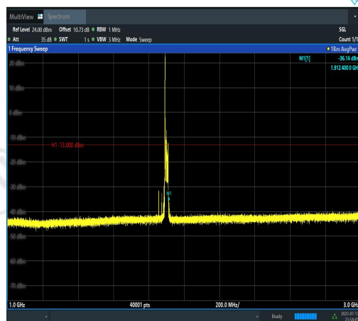
Band2-20MHz-QPSK-19100-1RB#0-1000~3000- PASS
