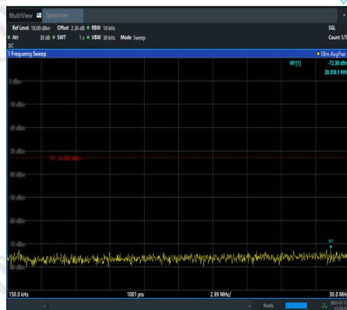
Band2-20MHz-QPSK-19100-100RB#0-0.15~30-PASS PASS
