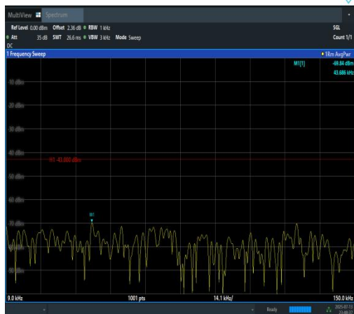
Band2-20MHz-16QAM-18900-1RB#99-0.009~0.15-PASS
