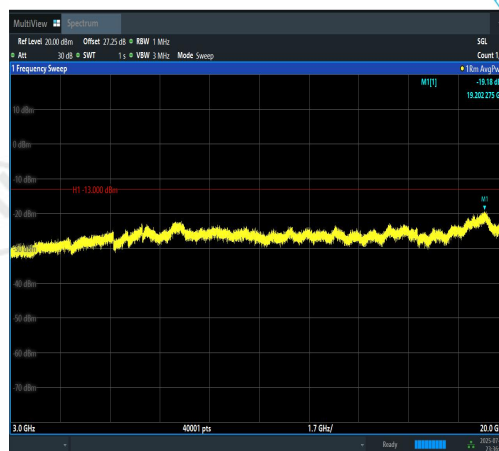
Band2-20MHz-16QAM-18700-1RB#0-3000~20000-PASS
