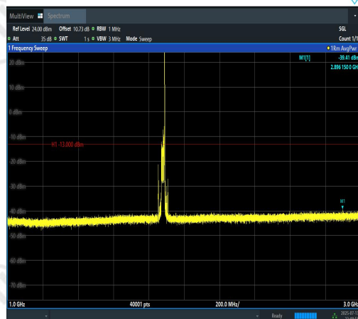
Band2-20MHz-16QAM-18900-1RB#99-1000~3000-PASS
