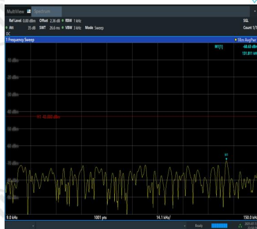
Band2-20MHz-QPSK-19100-1RB#99-0.009~0.1 5-PASS
