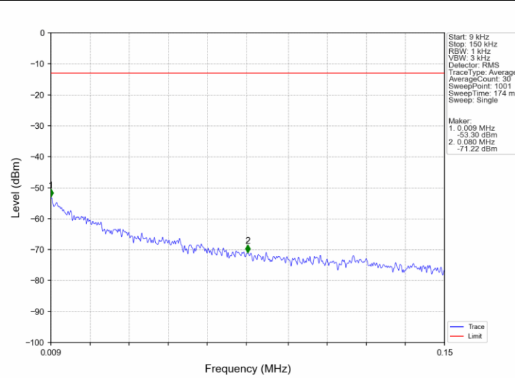
Band66_20MHz_16QAM_HCH_1770MHz_RB_1_0_NTNV
