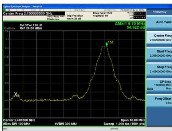
GFSK Band Edge(Ch. 0)
