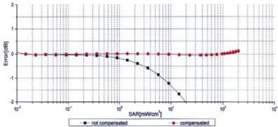
Uncertainty of Linearity Assessment: ±0.9% (k=2)
