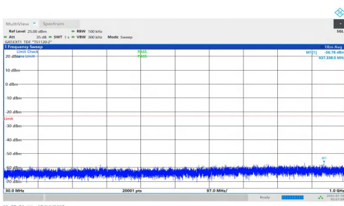
NTNV-n78(3700-3800)-PC1.5-30-100-L-DFT-BPSK-Inner_1RB_Left-30-1000-PASS
