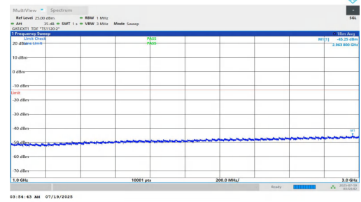
NTNV-n78(3700-3800)-PC1.5-30-90-H-DFT-QPSK-Inner_1RB_Left-10 00-3000-PASS
