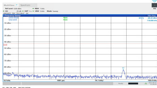
NTNV-n78(3700-3800)-PC1.5-30-90-H-DFT-BPSK-Inner_1RB_Left-0.009-0.15-PASS
