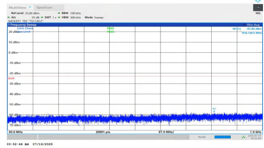
NTNV-n78(3700-3800)-PC1.5-30-90-H-DFT-BPSK-Inner_1RB_Right-3 0-1000-PASS
