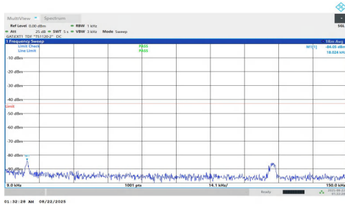
NTNV-n78(3700-3800)-PC1.5-30-100-L-DFT-QPSK-Inner_1RB_Left- 0.009-0.15-PASS
