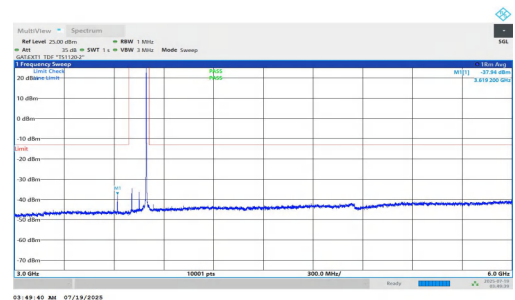
NTNV-n78(3700-3800)-PC1.5-30-90-M-DFT-QPSK-Inner_1RB_Right- 3000-6000-PASS
