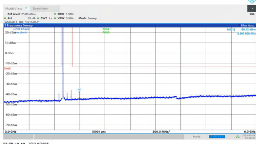
NTNV-n78(3700-3800)-PC1.5-30-100-L-DFT-BPSK-Inner_1RB_Left-3 000-6000-PASS
