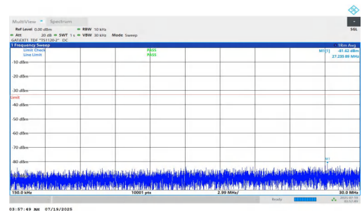
NTNV-n78(3700-3800)-PC1.5-30-100-L-DFT-BPSK-Inner_1RB_Left-0.15-30-PASS
