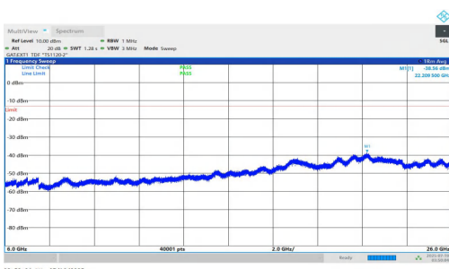
NTNV-n78(3700-3800)-PC1.5-30-90-M-DFT-QPSK-Inner_1RB_Right- 6000-26000-PASS
