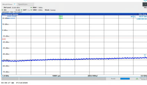
NTNV-n78(3700-3800)-PC1.5-30-90-H-DFT-QPSK-Inner_1RB_Right-1000-3000-PASS
