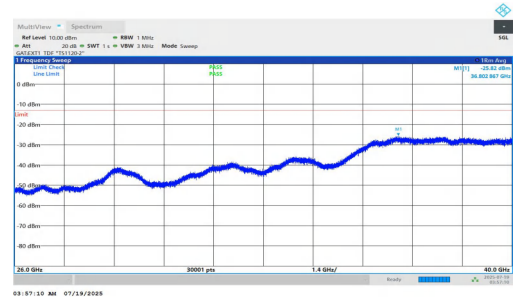
NTNV-n78(3700-3800)-PC1.5-30-90-H-DFT-QPSK-Inner_1RB_Right-26000-40000-PASS
