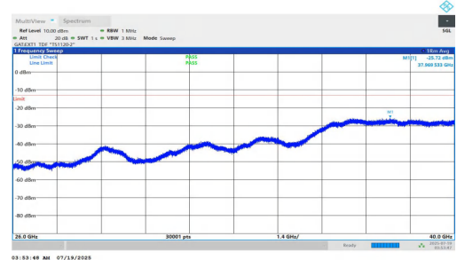
NTNV-n78(3700-3800)-PC1.5-30-90-H-DFT-BPSK-Inner_1RB_Right-2 6000-40000-PASS
