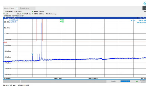
NTNV-n78(3700-3800)-PC1.5-30-100-L-DFT-QPSK-Inner_1RB_Right-3000-6000-PASS
