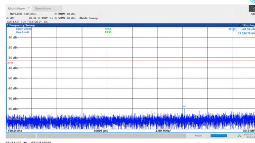
NTNV-n78(3700-3800)-PC1.5-30-90-H-DFT-BPSK-Inner_1RB_Left-0.15-30-PASS
