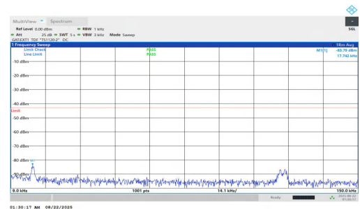
NTNV-n78(3700-3800)-PC1.5-30-90-H-DFT-QPSK-Inner_1RB_Right-0 .009-0.15-PASS
