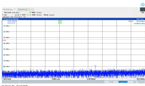
NTNV-n78(3700-3800)-PC1.5-30-100-L-DFT-BPSK-Inner_1RB_Right -0.15-30-PASS
