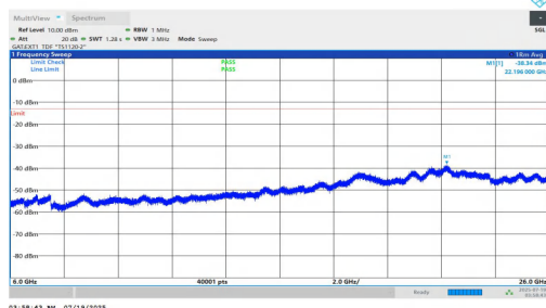
NTNV-n78(3700-3800)-PC1.5-30-100-L-DFT-BPSK-Inner_1RB_Left-6 000-26000-PASS
