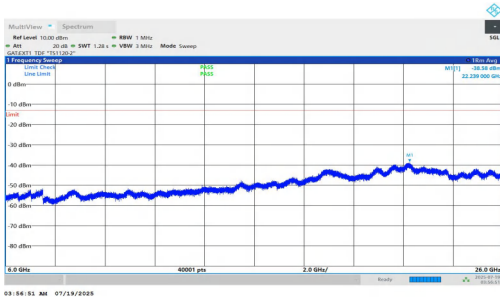
NTNV-n78(3700-3800)-PC1.5-30-90-H-DFT-QPSK-Inner_1RB_Right-6000-26000-PASS
