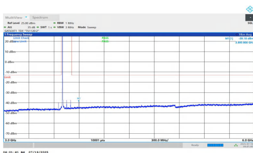
NTNV-n78(3700-3800)-PC1.5-30-100-L-DFT-QPSK-Inner_1RB_Left- 3000-6000-PASS
