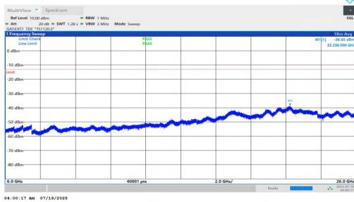
NTNV-n78(3700-3800)-PC1.5-30-100-L-DFT-BPSK-Inner_1RB_Right -6000-26000-PASS
