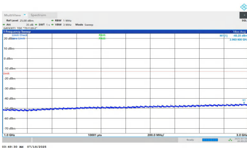
NTNV-n78(3700-3800)-PC1.5-30-90-M-DFT-QPSK-Inner_1RB_Right- 1000-3000-PASS
