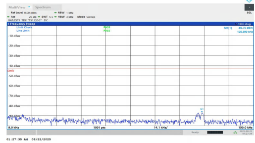
NTNV-n78(3700-3800)-PC1.5-30-90-M-DFT-QPSK-Inner_1RB_Right- 0.009-0.15-PASS
