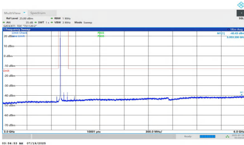
NTNV-n78(3700-3800)-PC1.5-30-90-H-DFT-QPSK-Inner_1RB_Left-3 000-6000-PASS
