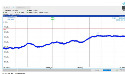
NTNV-n78(3700-3800)-PC1.5-30-100-L-DFT-QPSK-Inner_1RB_Right-26000-40000-PASS
