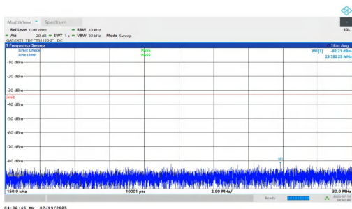
NTNV-n78(3700-3800)-PC1.5-30-100-L-DFT-QPSK-Inner_1RB_Right-0.15-30-PASS
