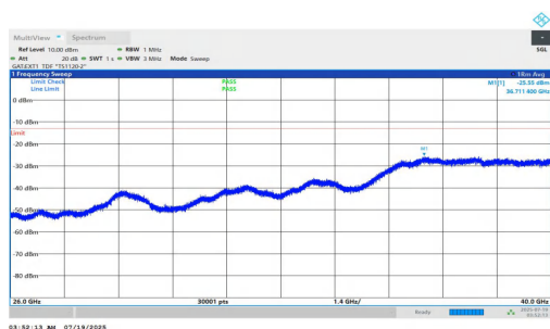
NTNV-n78(3700-3800)-PC1.5-30-90-H-DFT-BPSK-Inner_1RB_Left-26000-40000-PASS
