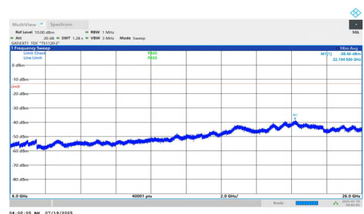
NTNV-n78(3700-3800)-PC1.5-30-100-L-DFT-QPSK-Inner_1RB_Left-6 000-26000-PASS
