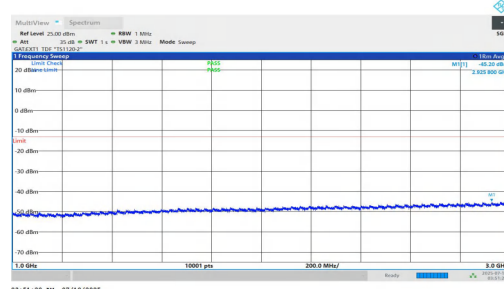
NTNV-n78(3700-3800)-PC1.5-30-90-H-DFT-BPSK-Inner_1RB_Left-1000-3000-PASS
