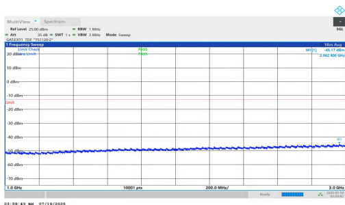
NTNV-n78(3700-3800)-PC1.5-30-100-L-DFT-BPSK-Inner_1RB_Right -1000-3000-PASS
