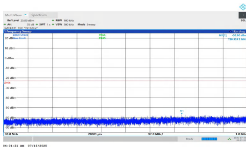
NTNV-n78(3700-3800)-PC1.5-30-100-L-DFT-QPSK-Inner_1RB_Left- 30-1000-PASS
