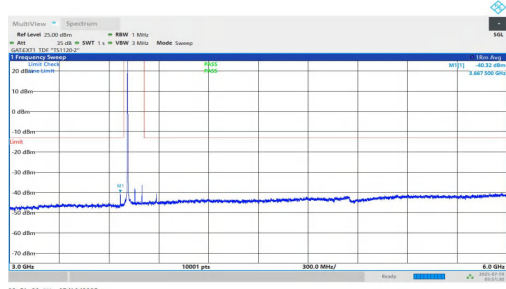
NTNV-n78(3700-3800)-PC1.5-30-90-H-DFT-BPSK-Inner_1RB_Left-3000-6000-PASS
