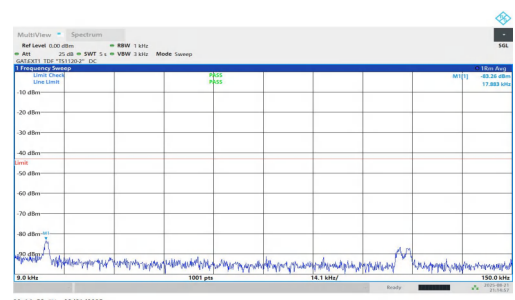
NTNV-n77(3700-3980)-PC1.5-30-25-M-DFT-BPSK-Inner_1RB_Right-0.009-0.15-PASS
