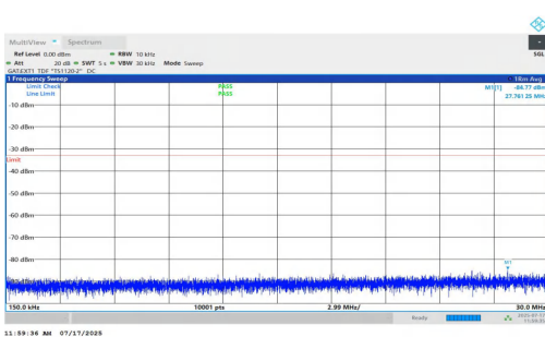
NTNV-n77(3700-3980)-PC1.5-30-20-H-DFT-QPSK-Inner_1RB_Right- 0.15-30-PASS
