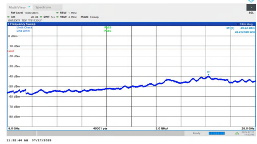
NTNV-n77(3700-3980)-PC1.5-30-20-M-DFT-BPSK-Inner_1RB_Left-60 00-26000-PASS
