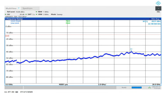
NTNV-n77(3700-3980)-PC1.5-30-20-H-DFT-QPSK-Inner_1RB_Left-60 00-26000-PASS
