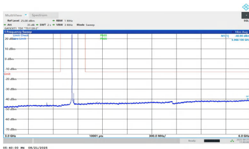
NTNV-n77(3700-3980)-PC1.5-30-25-M-DFT-BPSK-Inner_1RB_Left-3000-6000-PASS
