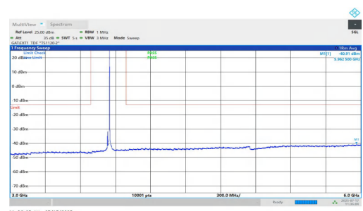
NTNV-n77(3700-3980)-PC1.5-30-20-M-DFT-BPSK-Inner_1RB_Right-3 000-6000-PASS
