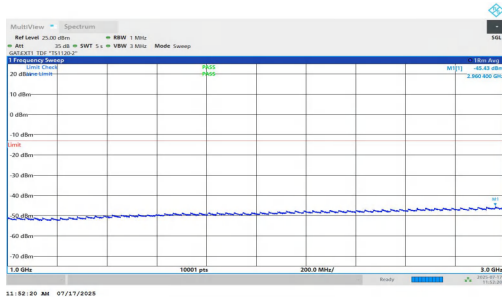
NTNV-n77(3700-3980)-PC1.5-30-20-H-DFT-BPSK-Inner_1RB_Right-1000-3000-PASS
