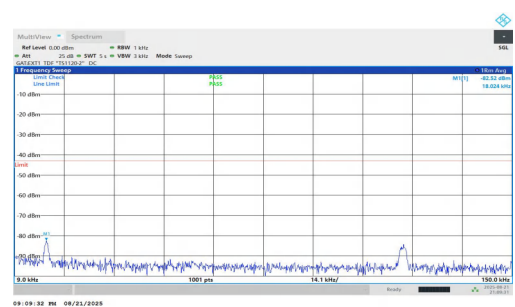
NTNV-n77(3700-3980)-PC1.5-30-20-H-DFT-BPSK-Inner_1RB_Right-0.009-0.15-PASS
