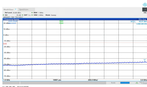
NTNV-n77(3700-3980)-PC1.5-30-20-M-DFT-QPSK-Inner_1RB_Left-1000-3000-PASS
