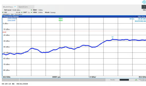
NTNV-n77(3700-3980)-PC1.5-30-25-L-DFT-QPSK-Inner_1RB_Left-2 6000-40000-PASS
