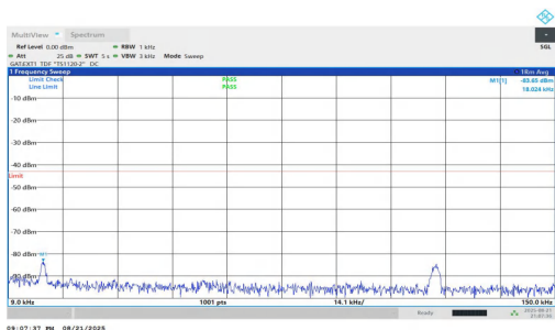
NTNV-n77(3700-3980)-PC1.5-30-20-M-DFT-QPSK-Inner_1RB_Left-0.009-0.15-PASS
