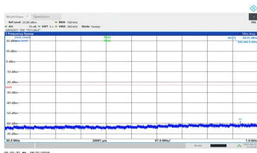
NTNV-n77(3700-3980)-PC1.5-30-25-L-DFT-BPSK-Inner_1RB_Right-3 0-1000-PASS
