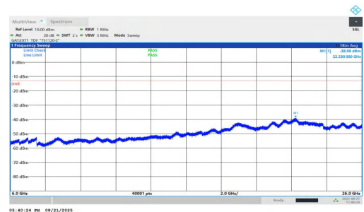
NTNV-n77(3700-3980)-PC1.5-30-25-M-DFT-BPSK-Inner_1RB_Left-6000-26000-PASS
