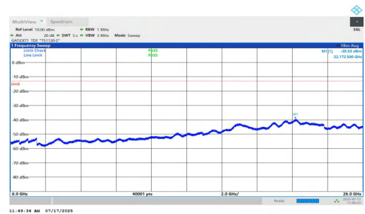
NTNV-n77(3700-3980)-PC1.5-30-20-H-DFT-BPSK-Inner_1RB_Left-6000-26000-PASS
