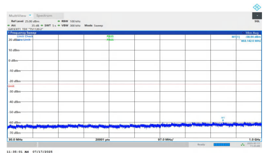
NTNV-n77(3700-3980)-PC1.5-30-20-M-DFT-BPSK-Inner_1RB_Right-3 0-1000-PASS
