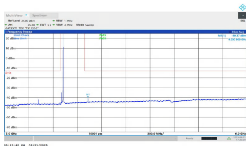
NTNV-n77(3700-3980)-PC1.5-30-25-L-DFT-BPSK-Inner_1RB_Right-3 000-6000-PASS
