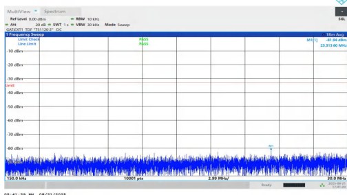
NTNV-n77(3700-3980)-PC1.5-30-25-M-DFT-BPSK-Inner_1RB_Right-0.15-30-PASS
