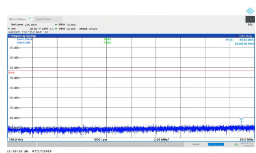
NTNV-n77(3700-3980)-PC1.5-30-20-H-DFT-QPSK-Inner_1RB_Left-0.15-30-PASS
