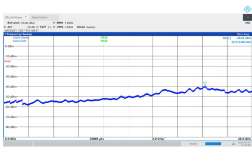
NTNV-n77(3700-3980)-PC1.5-30-20-M-DFT-QPSK-Inner_1RB_Right- 6000-26000-PASS
