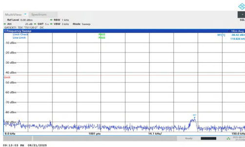
NTVN-n77(3700-3980)-PC1.5-30-25-L-DFT-QPSK-Inner_1RB_Left-0.009-0.15-PASS
