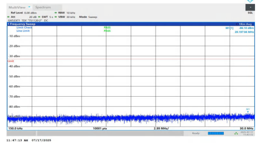
NTNV-n77(3700-3980)-PC1.5-30-20-H-DFT-BPSK-Inner_1RB_Left-0.15-30-PASS
