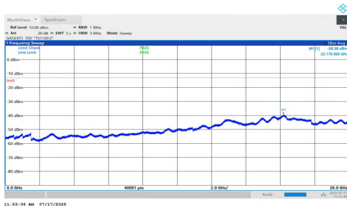
NTNV-n77(3700-3980)-PC1.5-30-20-H-DFT-BPSK-Inner_1RB_Right-6000-26000-PASS
