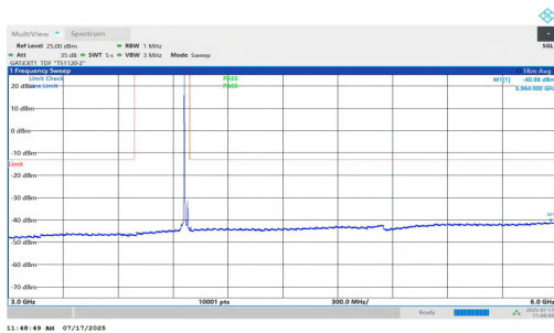
NTNV-n77(3700-3980)-PC1.5-30-20-H-DFT-BPSK-Inner_1RB_Left-3000-6000-PASS
