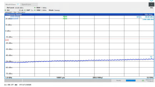
NTNV-n77(3700-3980)-PC1.5-30-20-H-DFT-QPSK-Inner_1RB_Left-10 00-3000-PASS
