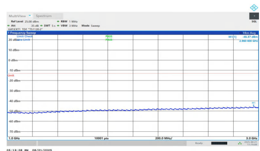
NTNV-n77(3700-3980)-PC1.5-30-25-L-DFT-BPSK-Inner_1RB_Left-1000-3000-PASS
