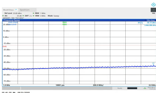
NTNV-n77(3700-3980)-PC1.5-30-25-M-DFT-BPSK-Inner_1RB_Right-1000-3000-PASS
