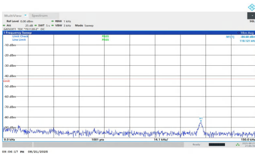
NTNV-n77(3700-3980)-PC1.5-30-20-M-DFT-BPSK-Inner_1RB_Left-0.009-0.15-PASS
