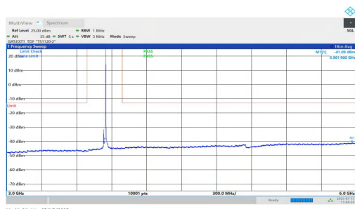
NTNV-n77(3700-3980)-PC1.5-30-20-M-DFT-QPSK-Inner_1RB_Right- 3000-6000-PASS
