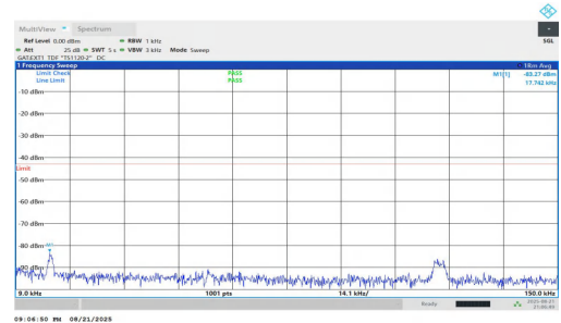
NTNV-n77(3700-3980)-PC1.5-30-20-M-DFT-BPSK-Inner_1RB_Right-0 .009-0.15-PASS
