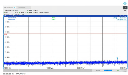
NTNV-n77(3700-3980)-PC1.5-30-20-M-DFT-BPSK-Inner_1RB_Left-0.15-30-PASS
