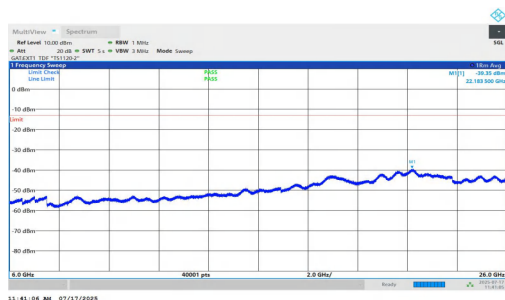
NTNV-n77(3700-3980)-PC1.5-30-20-M-DFT-QPSK-Inner_1RB_Left-6000-26000-PASS
