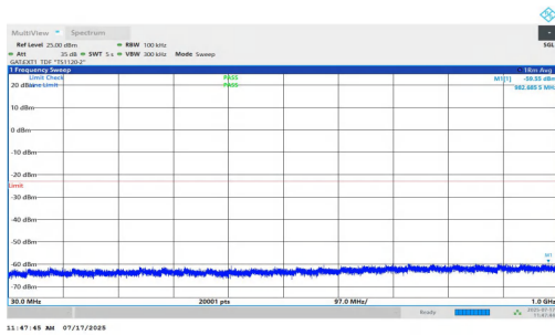
NTNV-n77(3700-3980)-PC1.5-30-20-H-DFT-BPSK-Inner_1RB_Left-300-1000-PASS
