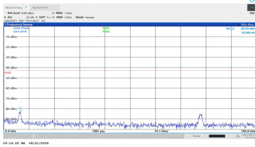
NTNV-n77(3700-3980)-PC1.5-30-25-M-DFT-BPSK-Inner_1RB_Left-0.009-0.15-PASS
