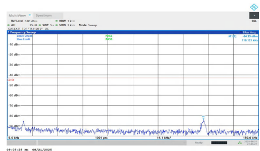
NTNV-n77(3700-3980)-PC1.5-30-20-L-DFT-QPSK-Inner_1RB_Right-0 .009-0.15-PASS
