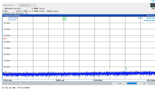
NTNV-n77(3700-3980)-PC1.5-30-20-H-DFT-BPSK-Inner_1RB_Right-0.15-30-PASS
