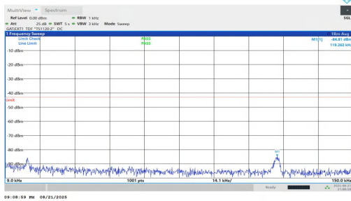
NTNV-n77(3700-3980)-PC1.5-30-20-H-DFT-BPSK-Inner_1RB_Left-0.009-0.15-PASS
