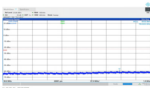
NTNV-n77(3700-3980)-PC1.5-30-20-M-DFT-QPSK-Inner_1RB_Right- 30-1000-PASS
