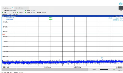
NTNV-n77(3700-3980)-PC1.5-30-25-L-DFT-BPSK-Inner_1RB_Right- 0.15-30-PASS
