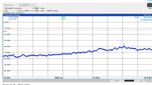
NTNV-n77(3700-3980)-PC1.5-30-25-L-DFT-BPSK-Inner_1RB_Left-60 00-26000-PASS
