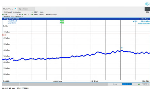
NTNV-n77(3700-3980)-PC1.5-30-20-M-DFT-BPSK-Inner_1RB_Right-6000-26000-PASS
