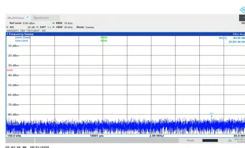
NTNV-n77(3700-3980)-PC1.5-30-25-M-DFT-QPSK-Inner_1RB_Left-0.15-30-PASS
