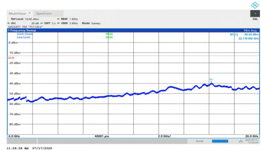
NTNV-n77(3700-3980)-PC1.5-30-20-L-DFT-QPSK-Inner_1RB_Left-60 00-26000-PASS
