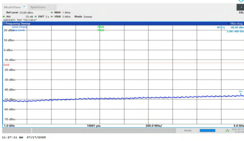
NTNV-n77(3700-3980)-PC1.5-30-20-L-DFT-QPSK-Inner_1RB_Right-1000-3000-PASS
