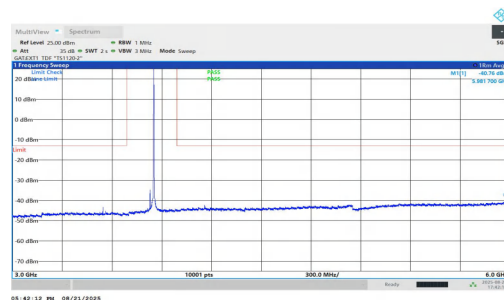
NTNV-n77(3700-3980)-PC1.5-30-25-M-DFT-BPSK-Inner_1RB_Right-3 000-6000-PASS
