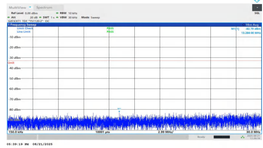
NTNV-n77(3700-3980)-PC1.5-30-25-M-DFT-BPSK-Inner_1RB_Left-0.15-30-PASS
