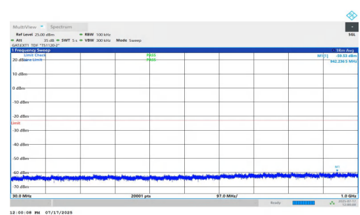
NTNV-n77(3700-3980)-PC1.5-30-20-H-DFT-QPSK-Inner_1RB_Right-3 0-1000-PASS
