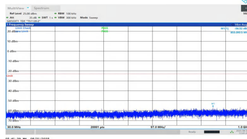
NTNV-n77(3700-3980)-PC1.5-30-25-M-DFT-BPSK-Inner_1RB_Right-3 0-1000-PASS
