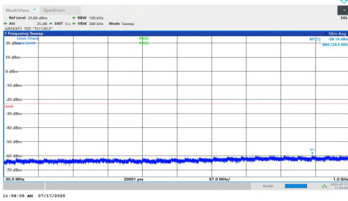
NTNV-n77(3700-3980)-PC1.5-30-20-H-DFT-QPSK-Inner_1RB_Left-3 0-1000-PASS
