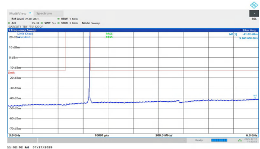
NTNV-n77(3700-3980)-PC1.5-30-20-H-DFT-BPSK-Inner_1RB_Right-3 000-6000-PASS
