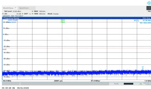
NTNV-n77(3700-3980)-PC1.5-30-25-M-DFT-BPSK-Inner_1RB_Left-30-1000-PASS
