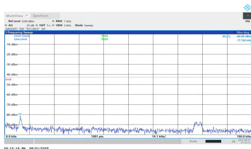
NTNV-n77(3700-3980)-PC1.5-30-25-L-DFT-BPSK-Inner_1RB_Right-0. 009-0.15-PASS
