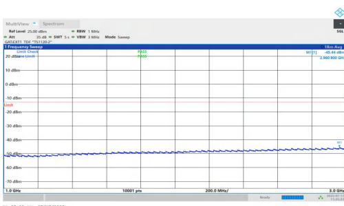
NTNV-n77(3700-3980)-PC1.5-30-20-M-DFT-BPSK-Inner_1RB_Right- 1000-3000-PASS
