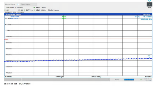
NTNV-n77(3700-3980)-PC1.5-30-20-L-DFT-QPSK-Inner_1RB_Left-10 00-3000-PASS
