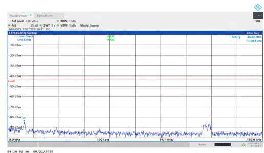
NTNV-n77(3700-3980)-PC1.5-30-20-H-DFT-QPSK-Inner_1RB_Right-0 .009-0.15-PASS
