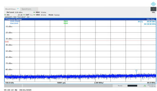
NTVN-n77(3700-3980)-PC1.5-30-25-L-DFT-QPSK-Inner_1RB_Left-0.15-0.30-PASS
