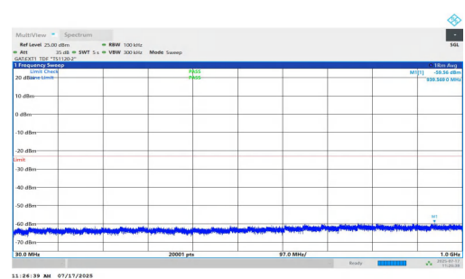
NTNV-n77(3700-3980)-PC1.5-30-20-L-DFT-QPSK-Inner_1RB_Right-3 0-1000-PASS
