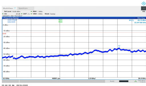
NTNV-n77(3700-3980)-PC1.5-30-25-M-DFT-BPSK-Inner_1RB_Right-6000-26000-PASS
