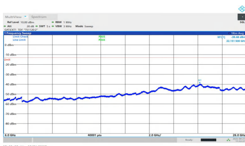
NTNV-n77(3700-3980)-PC1.5-30-25-L-DFT-QPSK-Inner_1RB_Right- 6000-26000-PASS
