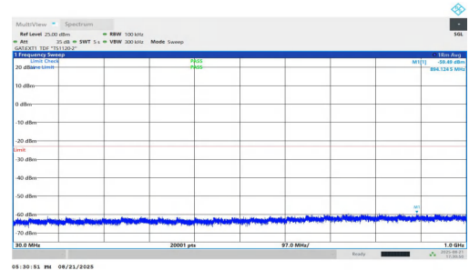
NTNV-n77(3700-3980)-PC1.5-30-25-L-DFT-QPSK-Inner_1RB_Right-3 0-1000-PASS
