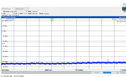
NTNV-n77(3700-3980)-PC1.5-30-20-M-DFT-BPSK-Inner_1RB_Left-30-1000-PASS
