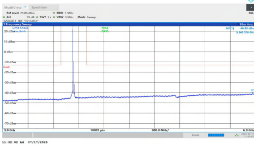
NTNV-n77(3700-3980)-PC1.5-30-20-M-DFT-BPSK-Inner_1RB_Left-3 000-6000-PASS
