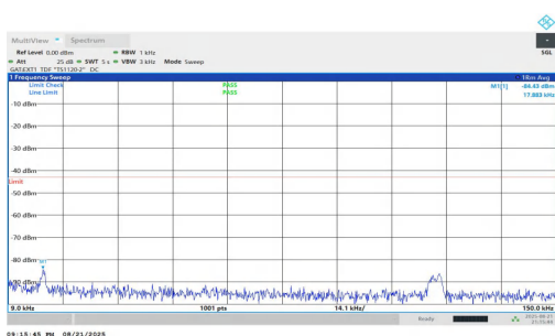
NTNV-n77(3700-3980)-PC1.5-30-25-M-DFT-QPSK-Inner_1RB_Left-0.009-0.15-PASS
