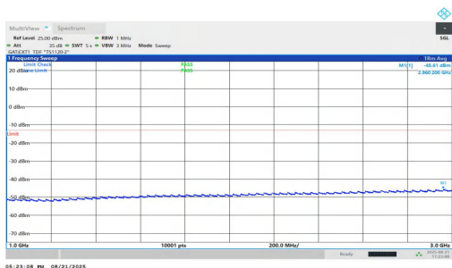
NTNV-n77(3700-3980)-PC1.5-30-25-L-DFT-BPSK-Inner_1RB_Right- 1000-3000-PASS
