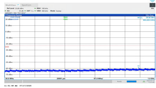
NTNV-n77(3700-3980)-PC1.5-30-20-H-DFT-BPSK-Inner_1RB_Right-3 0-1000-PASS
