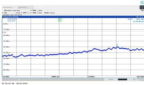
NTVN-n77(3700-3980)-PC1.5-30-25-L-DFT-BPSK-Inner_1RB_Right-6000-26000-PASS
