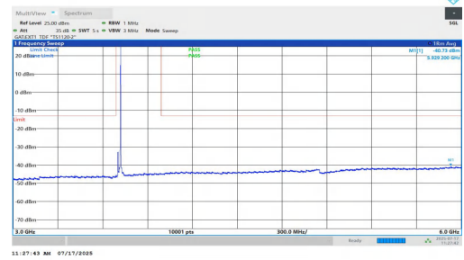
NTNV-n77(3700-3980)-PC1.5-30-20-L-DFT-QPSK-Inner_1RB_Right-3000-6000-PASS
