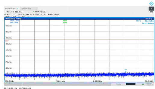
NTNV-n77(3700-3980)-PC1.5-30-25-L-DFT-BPSK-Inner_1RB_Left-0.15-5-30-PASS
