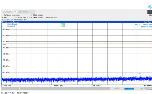
NTNV-n77(3700-3980)-PC1.5-30-20-L-DFT-QPSK-Inner_1RB_Right- 0.15-30-PASS
