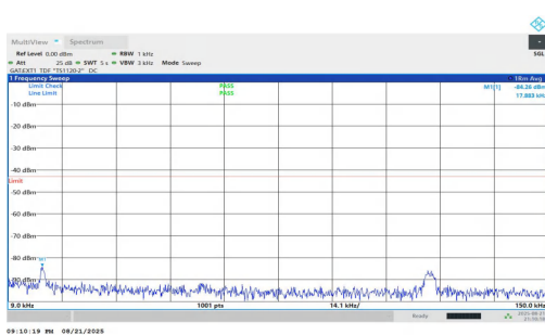
NTNV-n77(3700-3980)-PC1.5-30-20-H-DFT-QPSK-Inner_1RB_Left-0.009-0.15-PASS
