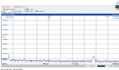
NTNV-n77(3700-3980)-PC1.5-30-25-L-DFT-BPSK-Inner_1RB_Left-0.009-0.15-PASS
