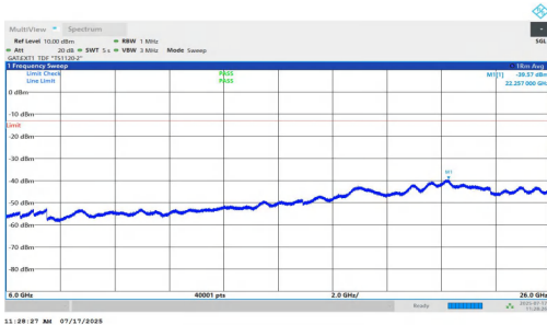
NTNV-n77(3700-3980)-PC1.5-30-20-L-DFT-QPSK-Inner_1RB_Right-6000-26000-PASS
