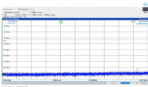
NTNV-n77(3700-3980)-PC1.5-30-20-M-DFT-QPSK-Inner_1RB_Right- 0.15-30-PASS
