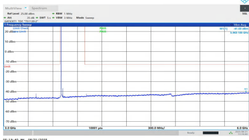
NTNV-n77(3700-3980)-PC1.5-30-25-L-DFT-BPSK-Inner_1RB_Left-30 00-6000-PASS
