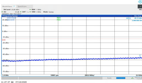
NTNV-n77(3450-3550)-PC1.5-30-80-M-DFT-BPSK-Inner_1RB_Right-1000-3000-PASS
