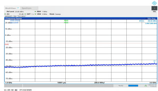
NTNV-n77(3450-3550)-PC1.5-30-80-M-DFT-BPSK-Inner_1RB_Left-1000-3000-PASS
