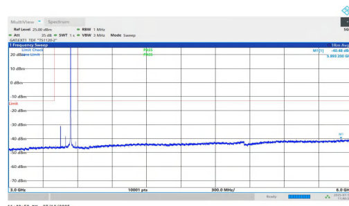
NTVN-n77(3450-3550)-PC1.5-30-90-L-DFT-BPSK-Inner_1RB_Right-3 000-6000-PASS
