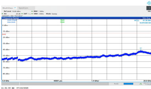
NTNV-n77(3450-3550)-PC1.5-30-80-M-DFT-QPSK-Inner_1RB_Right-6000-20000-PASS
