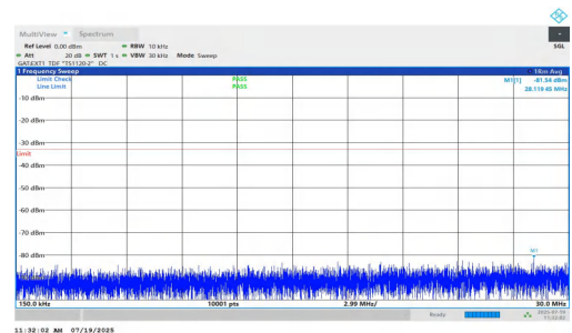
NTNV-n77(3450-3550)-PC1.5-30-80-H-DFT-BPSK-Inner_1RB_Left-0.15-5-30-PASS
