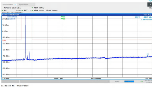
NTNV-n77(3450-3550)-PC1.5-30-80-H-DFT-BPSK-Inner_1RB_Left-3 000-6000-PASS
