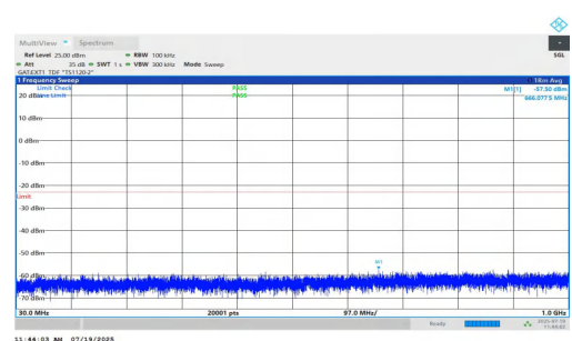
NTVN-n77(3450-3550)-PC1.5-30-90-L-DFT-QPSK-Inner_1RB_Right-3 0-1000-PASS
