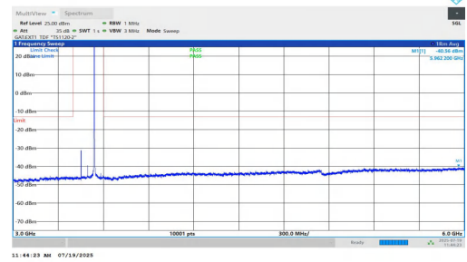
NTNV-n77(3450-3550)-PC1.5-30-90-L-DFT-QPSK-Inner_1RB_Right-3000-6000-PASS
