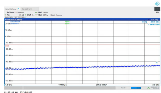
NTNV-n77(3450-3550)-PC1.5-30-80-H-DFT-QPSK-Inner_1RB_Left-1000-3000-PASS
