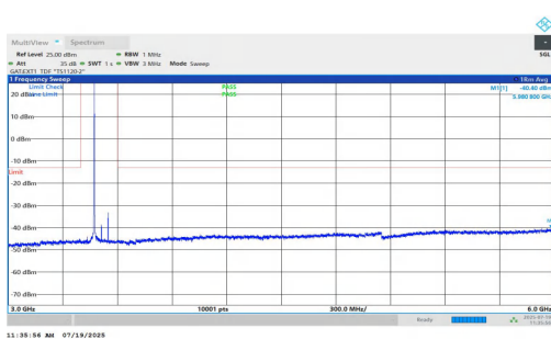
NTNV-n77(3450-3550)-PC1.5-30-80-H-DFT-QPSK-Inner_1RB_Left-3000-6000-PASS
