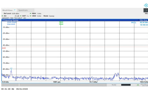
NTNV-n77(3450-3550)-PC1.5-30-80-M-DFT-QPSK-Inner_1RB_Left-0 .009-0.15-PASS
