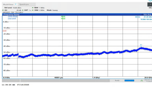
NTNV-n77(3450-3550)-PC1.5-30-80-H-DFT-BPSK-Inner_1RB_Right-6000-20000-PASS
