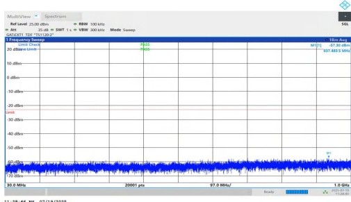
NTNV-n77(3450-3550)-PC1.5-30-80-M-DFT-QPSK-Inner_1RB_Left-3 0-1000-PASS
