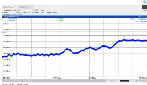
NTNV-n77(3450-3550)-PC1.5-30-90-M-DFT-QPSK-Inner_1RB_Left-2 0000-40000-PASS
