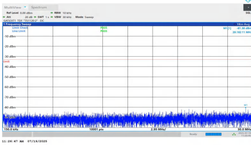
NTNV-n77(3450-3550)-PC1.5-30-80-M-DFT-BPSK-Inner_1RB_Right-0.15-30-PASS
