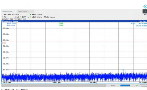
NTVN-n77(3450-3550)-PC1.5-30-90-L-DFT-QPSK-Inner_1RB_Right- 0.15-30-PASS
