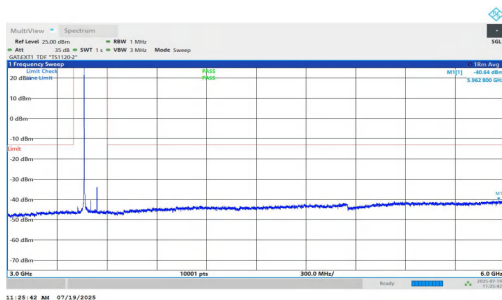
NTNV-n77(3450-3550)-PC1.5-30-80-M-DFT-BPSK-Inner_1RB_Left-3000-6000-PASS
