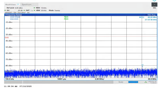
NTNV-n77(3450-3550)-PC1.5-30-90-L-DFT-BPSK-Inner_1RB_Left-0.15-30-PASS
