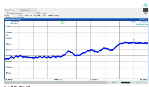
NTNV-n77(3450-3550)-PC1.5-30-80-H-DFT-QPSK-Inner_1RB_Right-2 0000-40000-PASS
