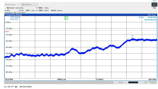
NTNV-n77(3450-3550)-PC1.5-30-90-M-DFT-BPSK-Inner_1RB_Right-20000-40000-PASS
