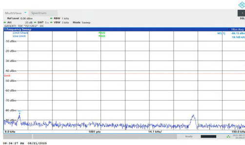
NTNV-n77(3450-3550)-PC1.5-30-80-H-DFT-QPSK-Inner_1RB_Left-0.009-0.15-PASS
