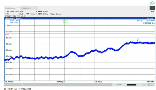
NTNV-n77(3450-3550)-PC1.5-30-90-L-DFT-QPSK-Inner_1RB_Right-20000-40000-PASS
