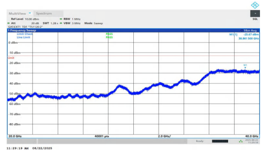
NTNV-n77(3450-3550)-PC1.5-30-80-M-DFT-QPSK-Inner_1RB_Right-20000-40000-PASS
