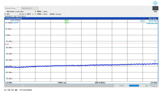
NTNV-n77(3450-3550)-PC1.5-30-90-L-DFT-BPSK-Inner_1RB_Left-1000-3000-PASS
