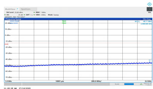
NTNV-n77(3450-3550)-PC1.5-30-90-M-DFT-QPSK-Inner_1RB_Left-1000-3000-PASS
