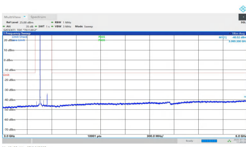
NTNV-n77(3450-3550)-PC1.5-30-90-M-DFT-QPSK-Inner_1RB_Left-3000-6000-PASS
