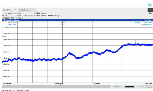
NTNV-n77(3450-3550)-PC1.5-30-80-M-DFT-QPSK-Inner_1RB_Left-2 0000-40000-PASS
