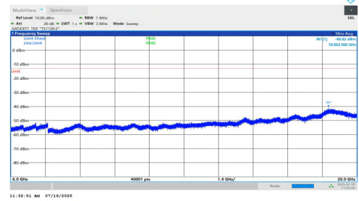
NTNV-n77(3450-3550)-PC1.5-30-80-H-DFT-BPSK-Inner_1RB_Left-60 00-20000-PASS
