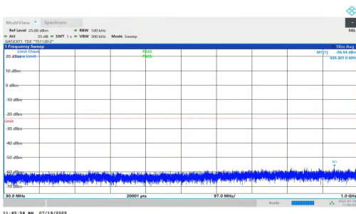
NTNV-n77(3450-3550)-PC1.5-30-90-M-DFT-BPSK-Inner_1RB_Left-30-1000-PASS
