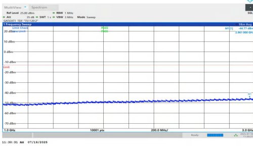
NTNV-n77(3450-3550)-PC1.5-30-80-M-DFT-QPSK-Inner_1RB_Right-1000-3000-PASS
