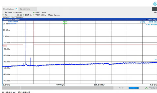
NTNV-n77(3450-3550)-PC1.5-30-90-L-DFT-BPSK-Inner_1RB_Left-3000-6000-PASS
