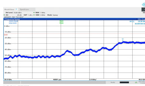
NTVN-n77(3450-3550)-PC1.5-30-90-L-DFT-BPSK-Inner_1RB_Right-2 0000-40000-PASS
