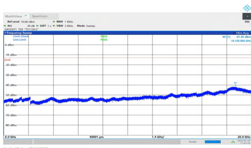
NTVN-n77(3450-3550)-PC1.5-30-90-L-DFT-BPSK-Inner_1RB_Right-6000-20000-PASS
