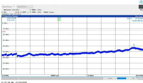
NTNV-n77(3450-3550)-PC1.5-30-80-M-DFT-BPSK-Inner_1RB_Right-6000-20000-PASS
