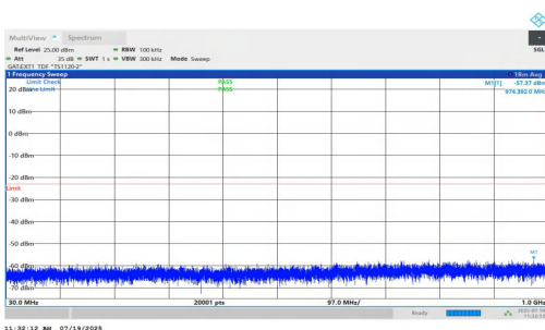
NTNV-n77(3450-3550)-PC1.5-30-80-H-DFT-BPSK-Inner_1RB_Left-30-1000-PASS
