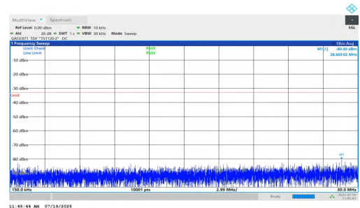
NTNV-n77(3450-3550)-PC1.5-30-90-M-DFT-BPSK-Inner_1RB_Left-0.15-30-PASS
