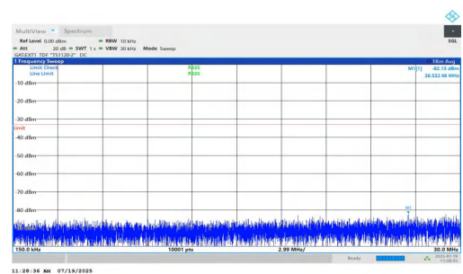
NTNV-n77(3450-3550)-PC1.5-30-80-M-DFT-QPSK-Inner_1RB_Left-0 15-30-PASS
