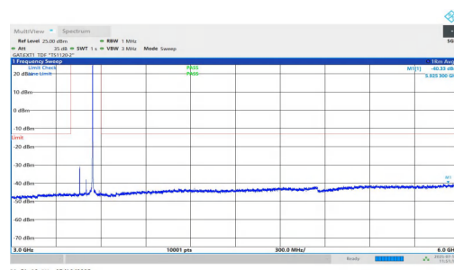
NTNV-n77(3450-3550)-PC1.5-30-90-M-DFT-QPSK-Inner_1RB_Right- 3000-6000-PASS
