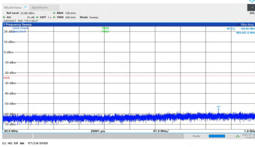
NTVN-n77(3450-3550)-PC1.5-30-90-L-DFT-QPSK-Inner_1RB_Left-3 0-1000-PASS
