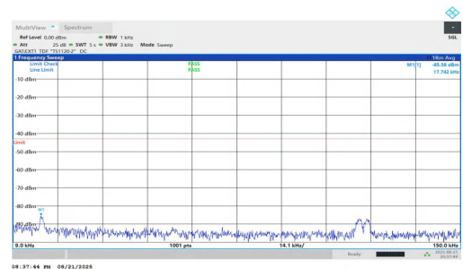
NTVN-n77(3450-3550)-PC1.5-30-90-L-DFT-QPSK-Inner_1RB_Right-0 .009-0.15-PASS
