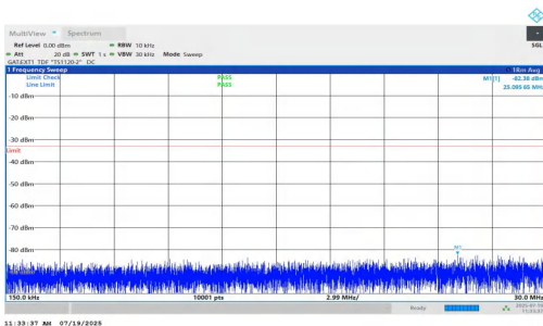
NTNV-n77(3450-3550)-PC1.5-30-80-H-DFT-BPSK-Inner_1RB_Right- 0.15-30-PASS
