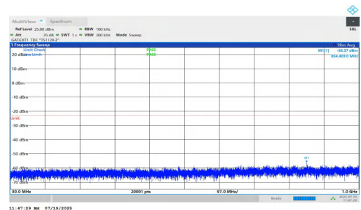
NTNV-n77(3450-3550)-PC1.5-30-90-M-DFT-BPSK-Inner_1RB_Right-3 0-1000-PASS
