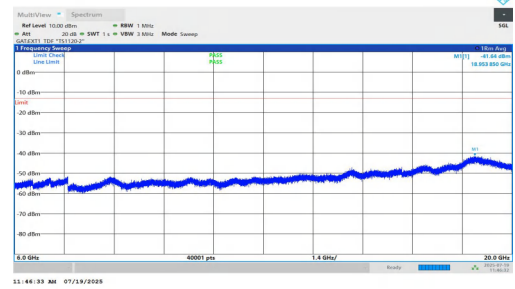
NTNV-n77(3450-3550)-PC1.5-30-90-M-DFT-BPSK-Inner_1RB_Left-60 00-20000-PASS
