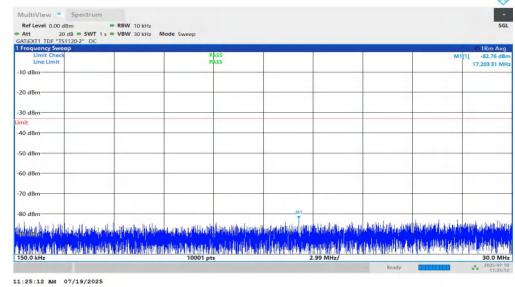
NTNV-n77(3450-3550)-PC1.5-30-80-M-DFT-BPSK-Inner_1RB_Left-0.15-30-PASS
