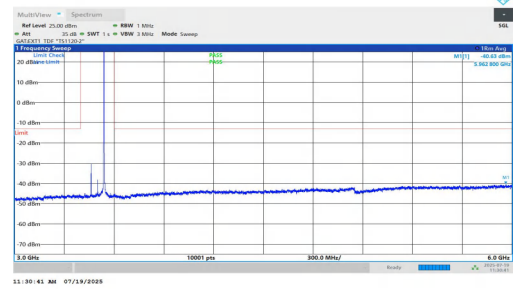
NTNV-n77(3450-3550)-PC1.5-30-80-M-DFT-QPSK-Inner_1RB_Right-3000-6000-PASS
