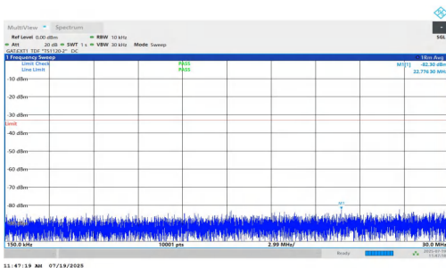
NTNV-n77(3450-3550)-PC1.5-30-90-M-DFT-BPSK-Inner_1RB_Right- 0.15-30-PASS
