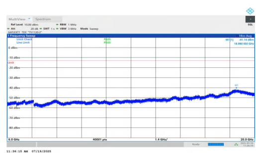
NTNV-n77(3450-3550)-PC1.5-30-80-H-DFT-QPSK-Inner_1RB_Left-6000-20000-PASS
