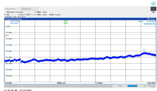
NTNV-n77(3450-3550)-PC1.5-30-90-L-DFT-BPSK-Inner_1RB_Left-6000-20000-PASS
