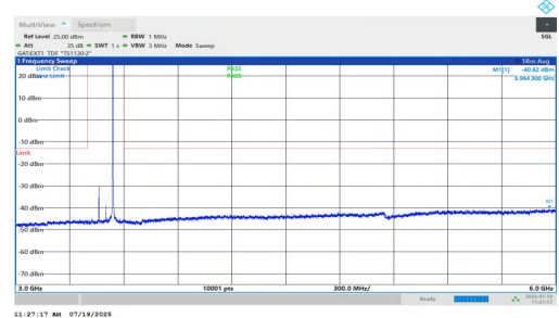
NTNV-n77(3450-3550)-PC1.5-30-80-M-DFT-BPSK-Inner_1RB_Right-3 000-6000-PASS
