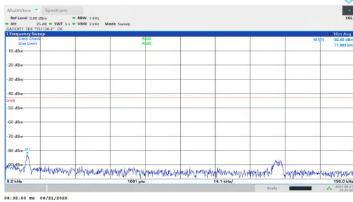
NTNV-n77(3450-3550)-PC1.5-30-90-L-DFT-BPSK-Inner_1RB_Left-0.009-0.15-PASS
