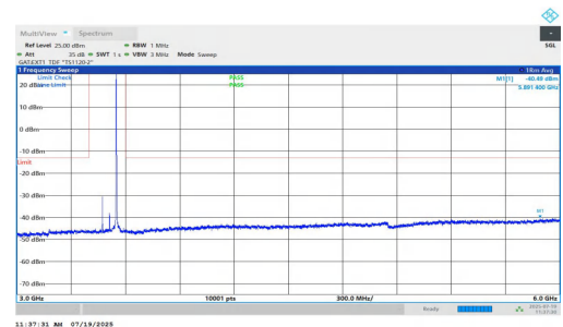
NTNV-n77(3450-3550)-PC1.5-30-80-H-DFT-QPSK-Inner_1RB_Right-3 000-6000-PASS
