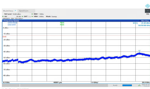
NTNV-n77(3450-3550)-PC1.5-30-90-M-DFT-QPSK-Inner_1RB_Right- 6000-20000-PASS
