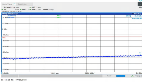
NTNV-n77(3450-3550)-PC1.5-30-90-L-DFT-QPSK-Inner_1RB_Right-1000-3000-PASS
