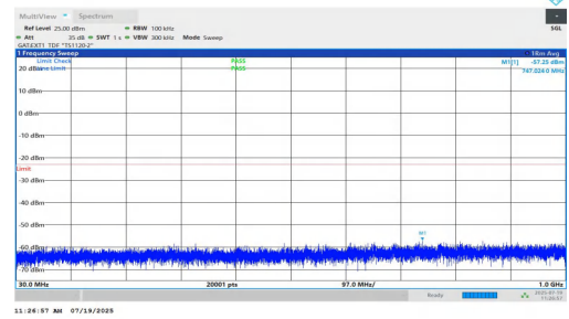
NTNV-n77(3450-3550)-PC1.5-30-80-M-DFT-BPSK-Inner_1RB_Right-3 0-1000-PASS
