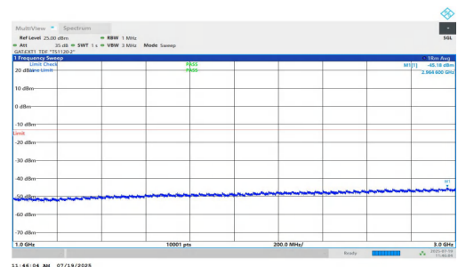
NTNV-n77(3450-3550)-PC1.5-30-90-M-DFT-BPSK-Inner_1RB_Left-1000-3000-PASS
