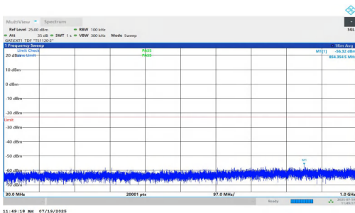
NTNV-n77(3450-3550)-PC1.5-30-90-M-DFT-QPSK-Inner_1RB_Left-30-1000-PASS
