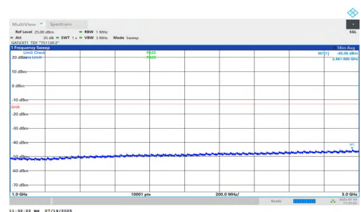
NTNV-n77(3450-3550)-PC1.5-30-80-H-DFT-BPSK-Inner_1RB_Left-1000-3000-PASS
