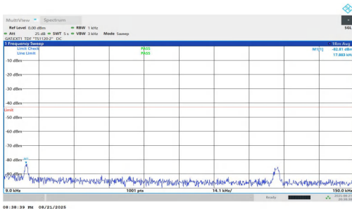
NTNV-n77(3450-3550)-PC1.5-30-90-M-DFT-BPSK-Inner_1RB_Left-0.009-0.15-PASS
