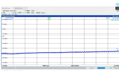
NTNV-n77(3450-3550)-PC1.5-30-90-M-DFT-BPSK-Inner_1RB_Right- 1000-3000-PASS
