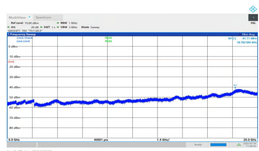
NTNV-n77(3450-3550)-PC1.5-30-90-M-DFT-QPSK-Inner_1RB_Left-6000-20000-PASS
