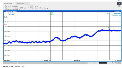
NTNV-n77(3450-3550)-PC1.5-30-80-H-DFT-BPSK-Inner_1RB_Right-20000-40000-PASS
