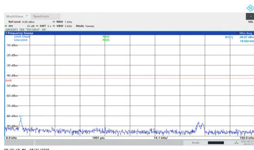
NTNV-n77(3450-3550)-PC1.5-30-80-M-DFT-QPSK-Inner_1RB_Right- 0.009-0.15-PASS
