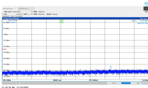
NTNV-n77(3450-3550)-PC1.5-30-80-H-DFT-QPSK-Inner_1RB_Left-30-1000-PASS
