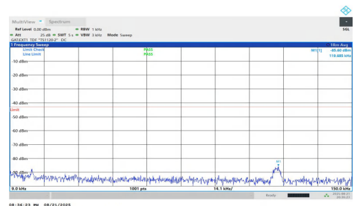
NTNV-n77(3450-3550)-PC1.5-30-90-L-DFT-BPSK-Inner_1RB_Right-0.009-0.15-PASS
