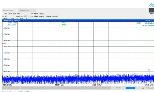
NTNV-n77(3450-3550)-PC1.5-30-90-M-DFT-QPSK-Inner_1RB_Right- 0.15-30-PASS
