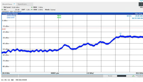
NTNV-n77(3450-3550)-PC1.5-30-80-H-DFT-QPSK-Inner_1RB_Left-2 0000-40000-PASS
