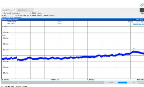
NTNV-n77(3450-3550)-PC1.5-30-80-H-DFT-QPSK-Inner_1RB_Right- 6000-20000-PASS
