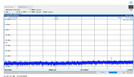
NTNV-n77(3450-3550)-PC1.5-30-80-H-DFT-QPSK-Inner_1RB_Right-3 0-1000-PASS
