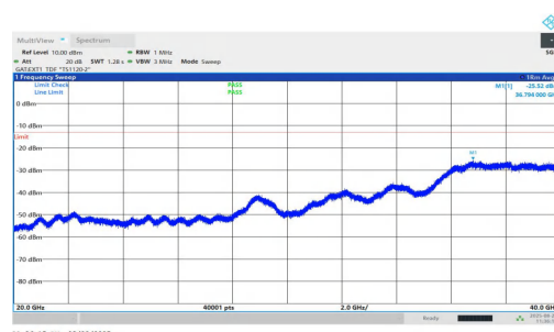
NTNV-n77(3450-3550)-PC1.5-30-90-M-DFT-QPSK-Inner_1RB_Right- 20000-40000-PASS
