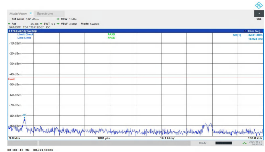
NTNV-n77(3450-3550)-PC1.5-30-80-H-DFT-BPSK-Inner_1RB_Right-0 .009-0.15-PASS
