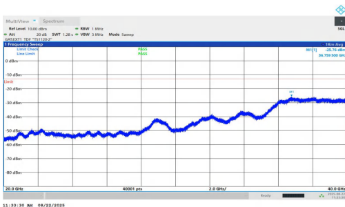
NTVN-n77(3450-3550)-PC1.5-30-90-L-DFT-QPSK-Inner_1RB_Left-2 0000-40000-PASS
