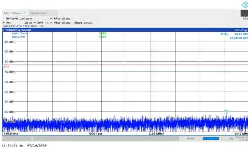
NTNV-n77(3450-3550)-PC1.5-30-80-H-DFT-QPSK-Inner_1RB_Right- 0.15-30-PASS
