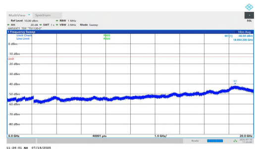
NTNV-n77(3450-3550)-PC1.5-30-80-M-DFT-BPSK-Inner_1RB_Left-6000-20000-PASS
