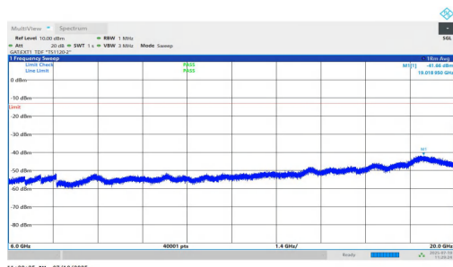
NTNV-n77(3450-3550)-PC1.5-30-80-M-DFT-QPSK-Inner_1RB_Left-60 00-20000-PASS
