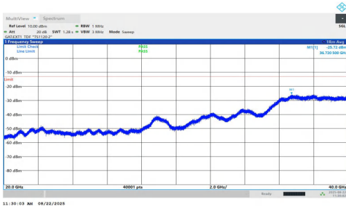
NTNV-n77(3450-3550)-PC1.5-30-80-H-DFT-BPSK-Inner_1RB_Left-2 0000-40000-PASS
