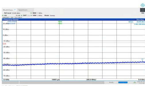
NTNV-n77(3450-3550)-PC1.5-30-90-M-DFT-QPSK-Inner_1RB_Right- 1000-3000-PASS
