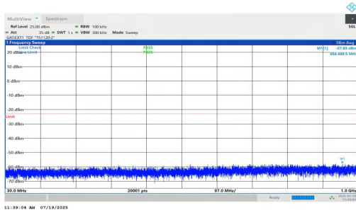
NTNV-n77(3450-3550)-PC1.5-30-90-L-DFT-BPSK-Inner_1RB_Left-30-1000-PASS
