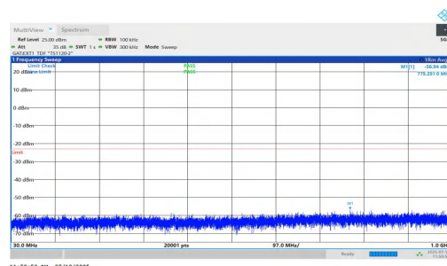
NTNV-n77(3450-3550)-PC1.5-30-90-M-DFT-QPSK-Inner_1RB_Right- 30-1000-PASS
