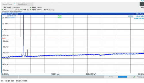
NTNV-n77(3450-3550)-PC1.5-30-90-M-DFT-BPSK-Inner_1RB_Left-3 000-6000-PASS
