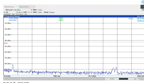
NTNV-n77(3450-3550)-PC1.5-30-90-M-DFT-QPSK-Inner_1RB_Right- 0.009-0.15-PASS
