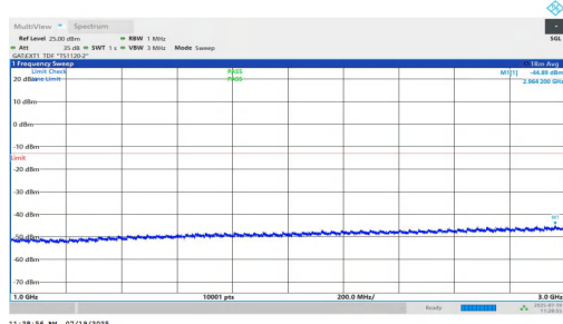
NTNV-n77(3450-3550)-PC1.5-30-80-M-DFT-QPSK-Inner_1RB_Left-10 00-3000-PASS
