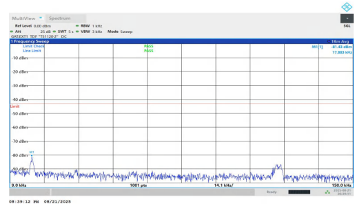
NTNV-n77(3450-3550)-PC1.5-30-90-M-DFT-BPSK-Inner_1RB_Right-0 .009-0.15-PASS
