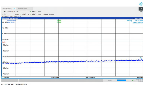
NTNV-n77(3450-3550)-PC1.5-30-80-H-DFT-QPSK-Inner_1RB_Right- 1000-3000-PASS
