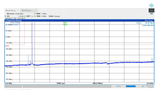
NTNV-n77(3450-3550)-PC1.5-30-80-H-DFT-BPSK-Inner_1RB_Right-3 000-6000-PASS
