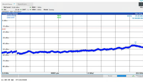
NTNV-n77(3450-3550)-PC1.5-30-90-M-DFT-BPSK-Inner_1RB_Right-6000-20000-PASS
