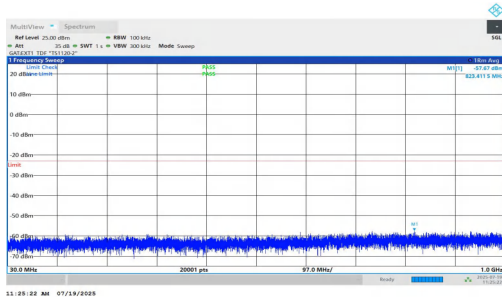
NTNV-n77(3450-3550)-PC1.5-30-80-M-DFT-BPSK-Inner_1RB_Left-30-1000-PASS
