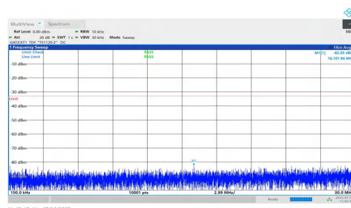
NTVN-n77(3450-3550)-PC1.5-30-90-L-DFT-QPSK-Inner_1RB_Left-0.1 5-30-PASS
