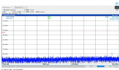
NTNV-n77(3450-3550)-PC1.5-30-80-M-DFT-QPSK-Inner_1RB_Right- 0.15-30-PASS
