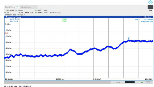
NTNV-n77(3450-3550)-PC1.5-30-80-M-DFT-BPSK-Inner_1RB_Right-2 0000-40000-PASS
