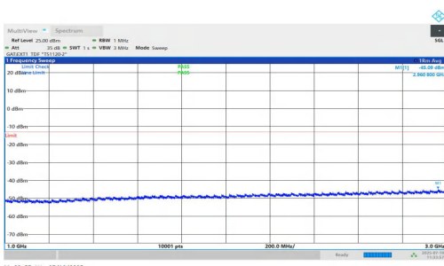
NTNV-n77(3450-3550)-PC1.5-30-80-H-DFT-BPSK-Inner_1RB_Right- 1000-3000-PASS
