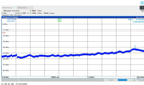
NTNV-n77(3450-3550)-PC1.5-30-90-L-DFT-QPSK-Inner_1RB_Right-6000-20000-PASS
