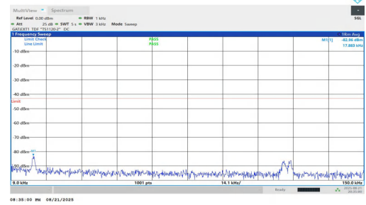
NTNV-n77(3450-3550)-PC1.5-30-80-H-DFT-QPSK-Inner_1RB_Right-0 .009-0.15-PASS
