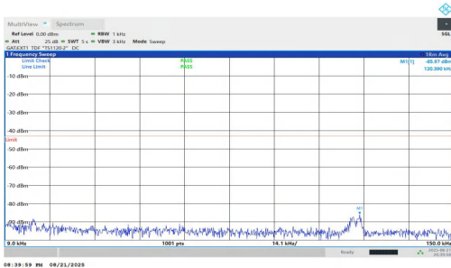
NTNV-n77(3450-3550)-PC1.5-30-90-M-DFT-QPSK-Inner_1RB_Left-0.009-0.15-PASS
