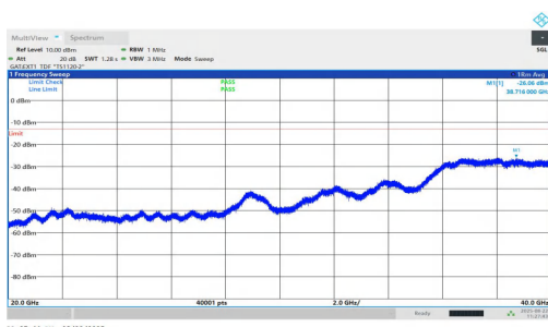
NTNV-n77(3450-3550)-PC1.5-30-80-M-DFT-BPSK-Inner_1RB_Left-20000-40000-PASS
