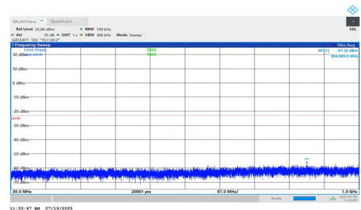
NTNV-n77(3450-3550)-PC1.5-30-80-H-DFT-BPSK-Inner_1RB_Right-3 0-1000-PASS
