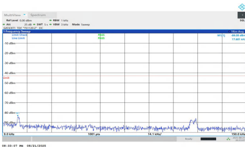
NTNV-n77(3450-3550)-PC1.5-30-80-H-DFT-BPSK-Inner_1RB_Left-0.009-0.15-PASS
