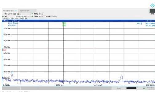
NTVN-n77(3450-3550)-PC1.5-30-90-L-DFT-QPSK-Inner_1RB_Left-0.009-0.15-PASS
