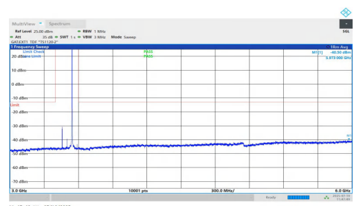
NTNV-n77(3450-3550)-PC1.5-30-90-M-DFT-BPSK-Inner_1RB_Right-3 000-6000-PASS
