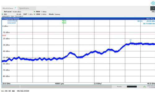
NTNV-n77(3450-3550)-PC1.5-30-90-M-DFT-BPSK-Inner_1RB_Left-2 0000-40000-PASS
