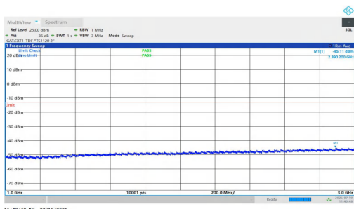
NTVN-n77(3450-3550)-PC1.5-30-90-L-DFT-BPSK-Inner_1RB_Right-1000-3000-PASS
