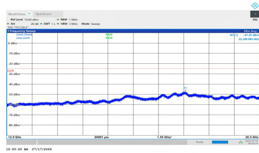
NTNV-n7-PC2-15-30-L-DFT-QPSK-Inner_1RB_Left-12000-26500-PASS
