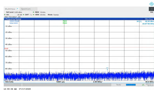
NTNV-n7-PC2-15-30-H-DFT-QPSK-Inner_1RB_Right-0.15-30-PA- SS
