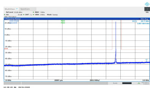
NTNV-n7-PC2-15-35-L-DFT-QPSK-Inner_1RB_Right-1000-3000-PASS
