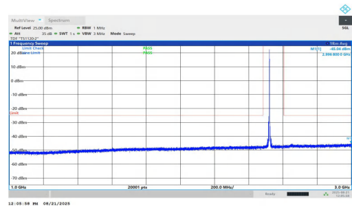
NTNV-n7-PC2-15-30-M-DFT-BPSK-Inner_1RB_Left-1000-3000-P ASS
