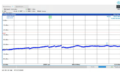
NTNV-n7-PC2-15-30-L-DFT-QPSK-Inner_1RB_Left-3000-12000-PASS
