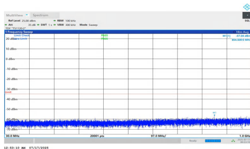
NTNV-n7-PC2-15-30-M-DFT-QPSK-Inner_1RB_Right-30-1000-P ASS
