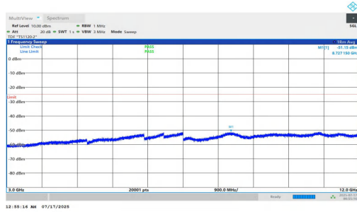
NTNV-n7-PC2-15-30-H-DFT-QPSK-Inner_1RB_Left-3000-12000- PASS
