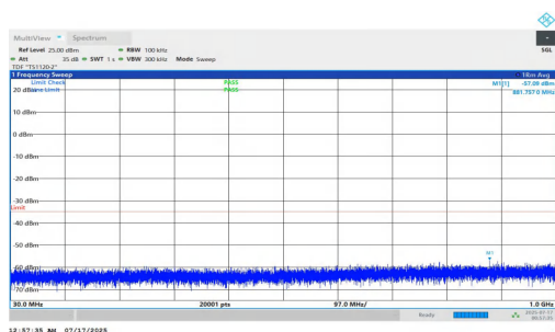
NTNV-n7-PC2-15-35-L-DFT-QPSK-Inner_1RB_Left-30-1000-PA SS
