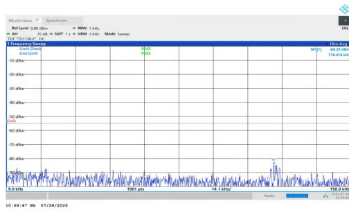
NTNV-n7-PC2-15-30-L-DFT-QPSK-Inner_1RB_Right-0.009-0.15-PASS
