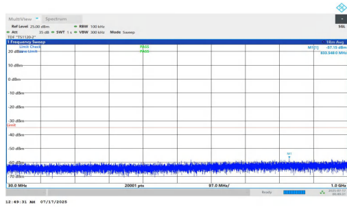
NTNV-n7-PC2-15-30-L-DFT-BPSK-Inner_1RB_Right-30-1000-PA SS
