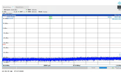
NTNV-n7-PC2-15-30-H-DFT-BPSK-Inner_1RB_Left-30-1000-PASS
