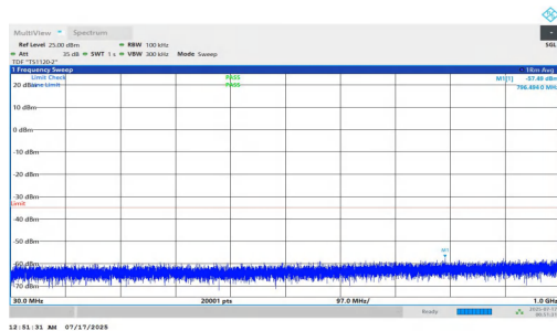
NTNV-n7-PC2-15-30-M-DFT-BPSK-Inner_1RB_Left-30-1000-PASS SS
