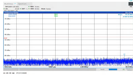
NTNV-n7-PC2-15-30-L-DFT-BPSK-Inner_1RB_Left-0.15-30-PASS
