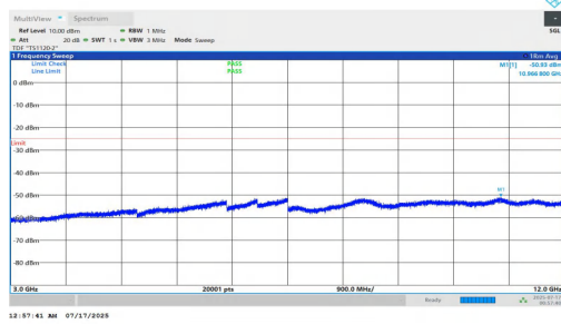
NTNV-n7-PC2-15-35-L-DFT-QPSK-Inner_1RB_Left-3000-12000-PASS
