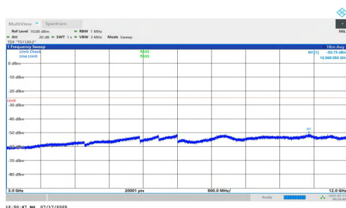
NTNV-n7-PC2-15-30-L-DFT-QPSK-Inner_1RB_Right-3000-12000-PASS
