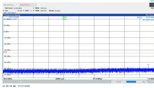
NTNV-n7-PC2-15-35-M-DFT-BPSK-Inner_1RB_Left-30-1000-PASS
