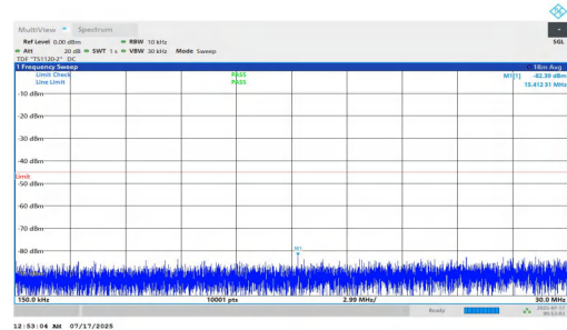
NTNV-n7-PC2-15-30-M-DFT-QPSK-Inner_1RB_Right-0.15-30-PA SS
