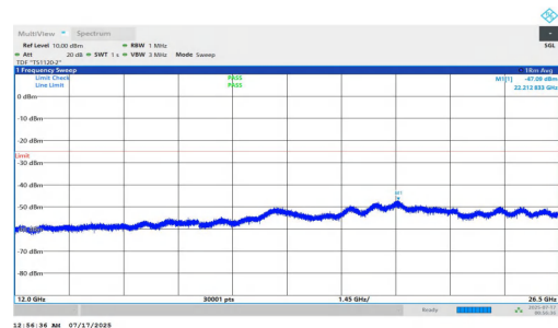
NTNV-n7-PC2-15-35-L-DFT-BPSK-Inner_1RB_Left-12000-26500- PASS
