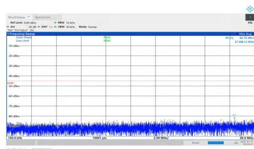
NTNV-n7-PC2-15-35-L-DFT-BPSK-Inner_1RB_Right-0.15-30-PASS S
