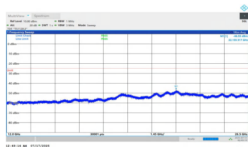
NTNV-n7-PC2-15-30-L-DFT-BPSK-Inner_1RB_Left-12000-26500- PASS
