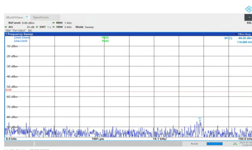
NTNV-n7-PC2-15-35-L-DFT-BPSK-Inner_1RB_Right-0.009-0.15- PASS
