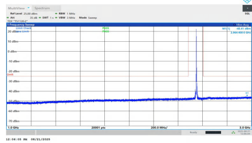
NTNV-n7-PC2-15-30-M-DFT-BPSK-Inner_1RB_Right-1000-3000-P PASS
