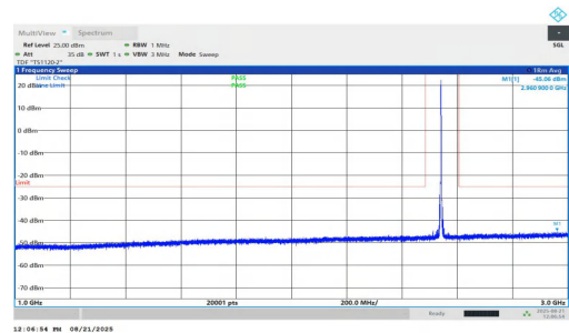
NTNV-n7-PC2-15-30-H-DFT-BPSK-Inner_1RB_Left-1000-3000-P ASS
