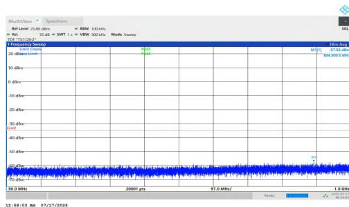
NTNV-n7-PC2-15-35-L-DFT-QPSK-Inner_1RB_Right-30-1000-PASS
