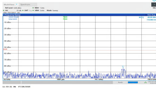
NTNV-n7-PC2-15-35-M-DFT-BPSK-Inner_1RB_Left-0.009-0.15-P ASS
