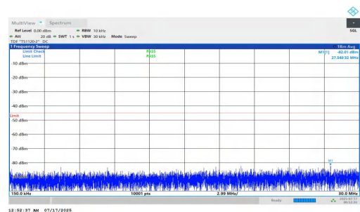
NTNV-n7-PC2-15-30-M-DFT-QPSK-Inner_1RB_Left-0.15-30-PAS S
