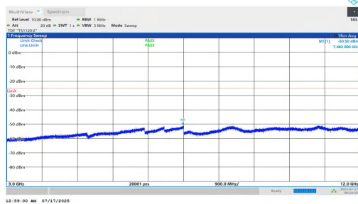
NTNV-n7-PC2-15-35-M-DFT-BPSK-Inner_1RB_Left-3000-12000-PASS
