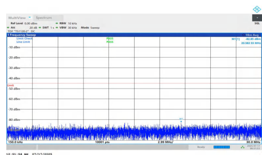
NTNV-n7-PC2-15-30-M-DFT-BPSK-Inner_1RB_Right-0.15-30-PASS SS
