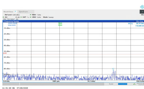
NTNV-n7-PC2-15-30-H-DFT-BPSK-Inner_1RB_Right-0.009-0.15- PASS
