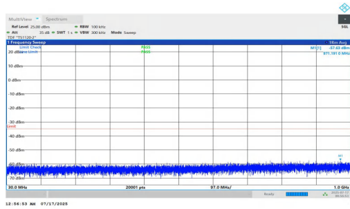
NTNV-n7-PC2-15-35-L-DFT-BPSK-Inner_1RB_Right-30-1000-PA SS
