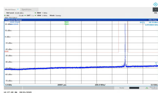
NTNV-n7-PC2-15-30-H-DFT-QPSK-Inner_1RB_Right-1000-3000- PASS
