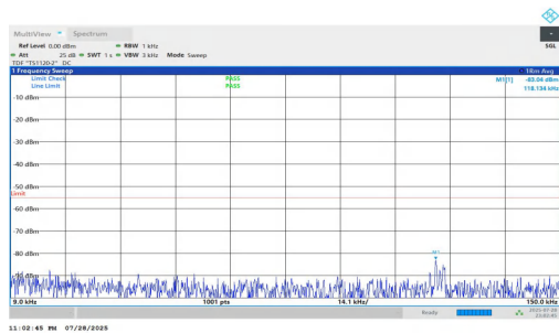
NTNV-n7-PC2-15-35-L-DFT-QPSK-Inner_1RB_Left-0.009-0.15-P ASS
