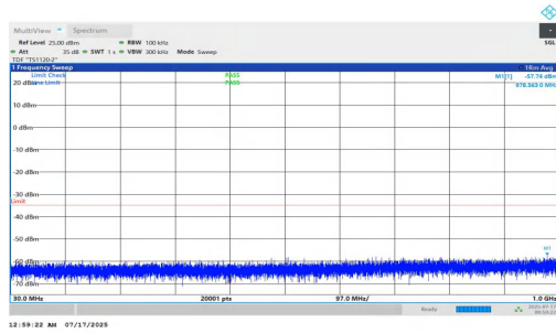
NTNV-n7-PC2-15-35-M-DFT-BPSK-Inner_1RB_Right-30-1000-P ASS
