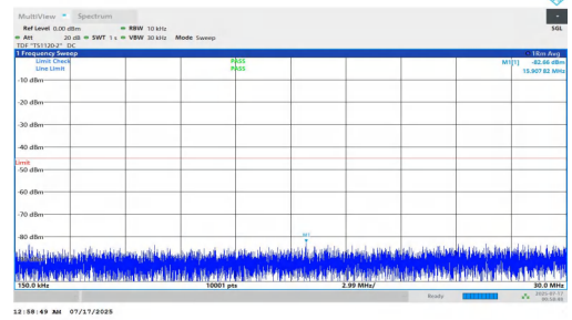
NTNV-n7-PC2-15-35-M-DFT-BPSK-Inner_1RB_Left-0.15-30-PAS S
