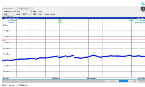
NTNV-n7-PC2-15-30-H-DFT-BPSK-Inner_1RB_Right-3000-12000-P PASS
