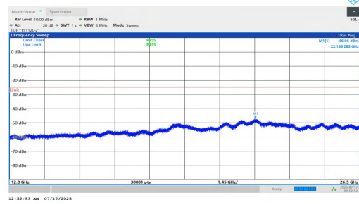
NTNV-n7-PC2-15-30-M-DFT-QPSK-Inner_1RB_Left-12000-26500 -PASS
