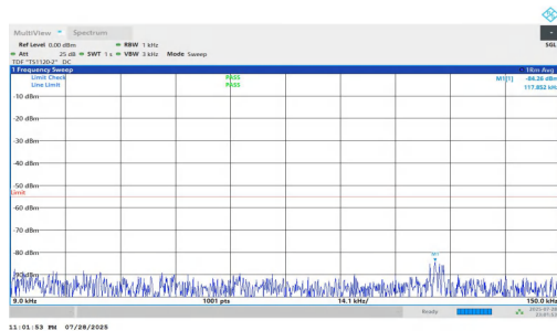
NTNV-n7-PC2-15-30-H-DFT-QPSK-Inner_1RB_Right-0.009-0.15 -PASS
