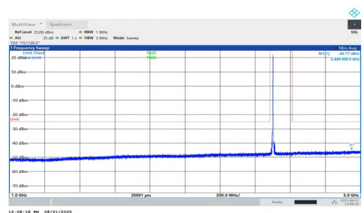
NTNV-n7-PC2-15-35-L-DFT-QPSK-Inner_1RB_Left-1000-3000-PA SS
