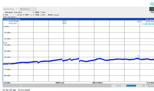
NTNV-n7-PC2-15-30-M-DFT-BPSK-Inner_1RB_Right-3000-1200 0-PASS
