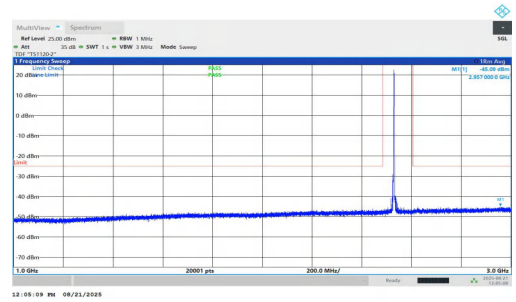
NTNV-n7-PC2-15-30-L-DFT-BPSK-Inner_1RB_Right-1000-3000-P ASS
