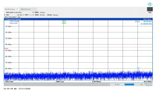
NTNV-n7-PC2-15-30-L-DFT-QPSK-Inner_1RB_Left-0.15-30-PASS
