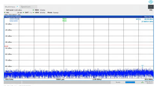
NTNV-n7-PC2-15-35-M-DFT-BPSK-Inner_1RB_Right-0.15-30-PASS
