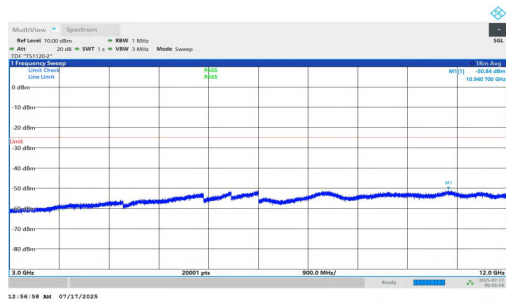
NTNV-n7-PC2-15-35-L-DFT-BPSK-Inner_1RB_Right-3000-12000 -PASS
