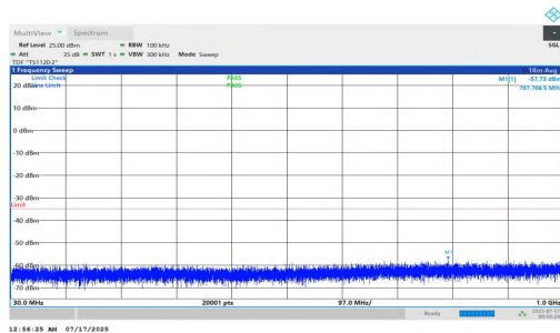
NTNV-n7-PC2-15-35-L-DFT-BPSK-Inner_1RB_Left-30-1000-PAS S
