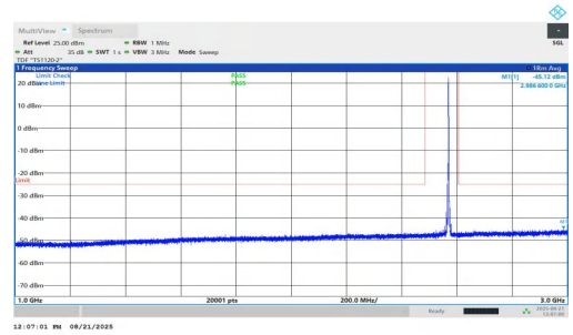
NTNV-n7-PC2-15-30-H-DFT-BPSK-Inner_1RB_Right-1000-3000-P PASS
