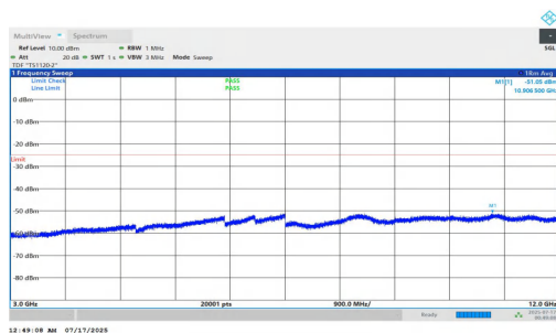
NTNV-n7-PC2-15-30-L-DFT-BPSK-Inner_1RB_Left-3000-12000- PASS
