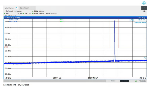
NTNV-n7-PC2-15-35-M-DFT-BPSK-Inner_1RB_Right-1000-3000-P PASS
