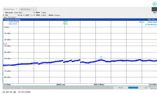
NTNV-n7-PC2-15-30-L-DFT-BPSK-Inner_1RB_Right-3000-12000 -PASS
