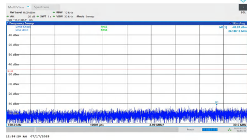
NTNV-n7-PC2-15-35-L-DFT-BPSK-Inner_1RB_Left-0.15-30-PASS
