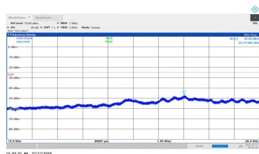
NTNV-n7-PC2-15-30-M-DFT-QPSK-Inner_1RB_Right-12000-2650 0-PASS
