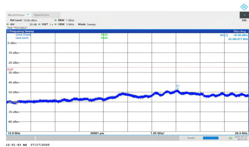
NTNV-n7-PC2-15-30-M-DFT-BPSK-Inner_1RB_Left-12000-26500- PASS
