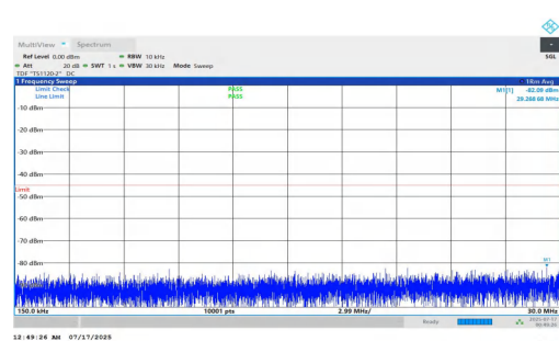
NTNV-n7-PC2-15-30-L-DFT-BPSK-Inner_1RB_Right-0.15-30-PASS S
