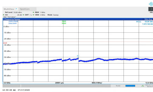
NTNV-n7-PC2-15-35-M-DFT-BPSK-Inner_1RB_Right-3000-1200 0-PASS
