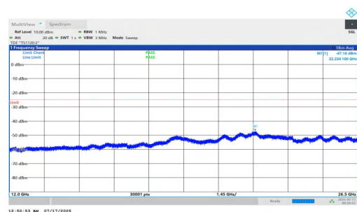
NTNV-n7-PC2-15-30-L-DFT-QPSK-Inner_1RB_Right-12000-26500-PASS
