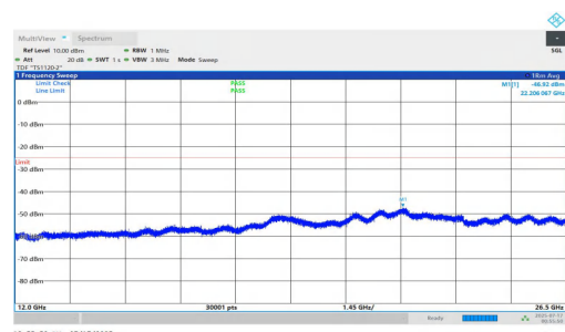
NTNV-n7-PC2-15-30-H-DFT-QPSK-Inner_1RB_Right-12000-2650 0-PASS
