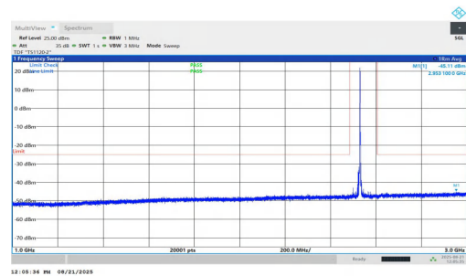
NTNV-n7-PC2-15-30-L-DFT-QPSK-Inner_1RB_Right-1000-3000-PASS
