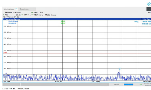
NTNV-n7-PC2-15-35-M-DFT-QPSK-Inner_1RB_Left-0.009-0.15- PASS
