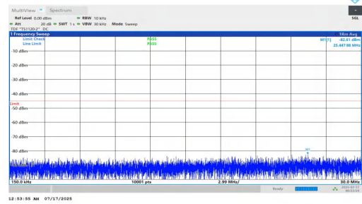
NTNV-n7-PC2-15-30-H-DFT-BPSK-Inner_1RB_Left-0.15-30-PASS
