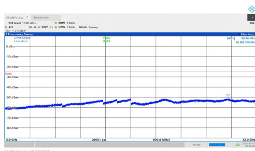
NTNV-n7-PC2-15-35-L-DFT-QPSK-Inner_1RB_Right-3000-12000-PASS
