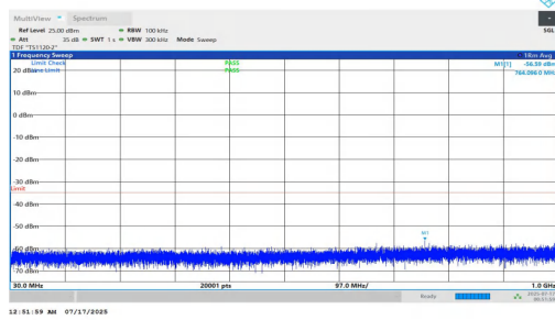
NTNV-n7-PC2-15-30-M-DFT-BPSK-Inner_1RB_Right-30-1000-P ASS
