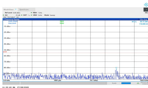
NTNV-n7-PC2-15-30-M-DFT-QPSK-Inner_1RB_Left-0.009-0.15- PASS
