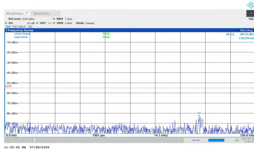
NTNV-n7-PC2-15-35-L-DFT-QPSK-Inner_1RB_Right-0.009-0.15-PASS
