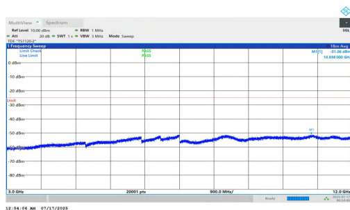
NTNV-n7-PC2-15-30-H-DFT-BPSK-Inner_1RB_Left-3000-12000- PASS
