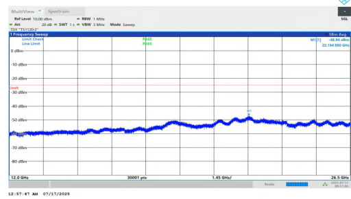
NTNV-n7-PC2-15-35-L-DFT-QPSK-Inner_1RB_Left-12000-26500-PASS
