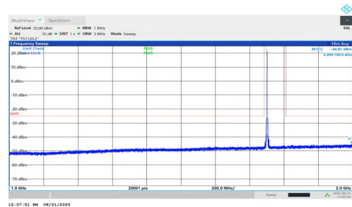
NTNV-n7-PC2-15-35-L-DFT-BPSK-Inner_1RB_Left-1000-3000-PASS S
