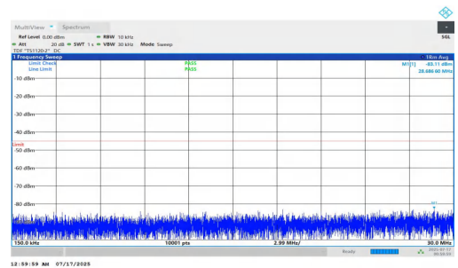
NTNV-n7-PC2-15-35-M-DFT-QPSK-Inner_1RB_Left-0.15-30-PAS S
