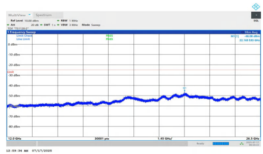
NTNV-n7-PC2-15-35-M-DFT-BPSK-Inner_1RB_Right-12000-2650 0-PASS
