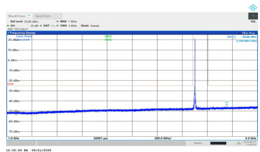
NTNV-n7-PC2-15-30-L-DFT-QPSK-Inner_1RB_Left-1000-3000-PA SS
