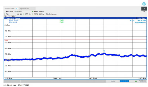
NTNV-n7-PC2-15-30-H-DFT-BPSK-Inner_1RB_Right-12000-26500-P PASS
