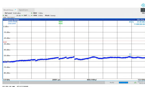
NTNV-n7-PC2-15-30-M-DFT-QPSK-Inner_1RB_Right-3000-1200 0-PASS
