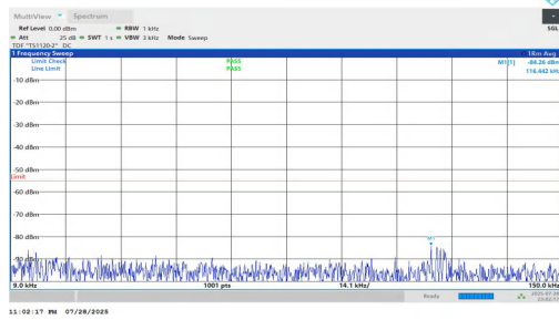
NTNV-n7-PC2-15-35-L-DFT-BPSK-Inner_1RB_Left-0.009-0.15-P ASS
