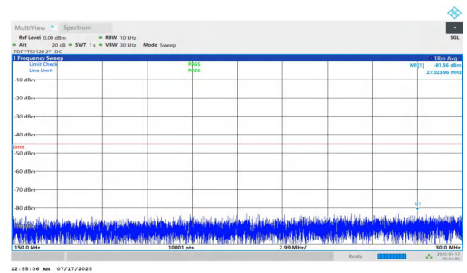
NTNV-n7-PC2-15-30-H-DFT-QPSK-Inner_1RB_Left-0.15-30-P ASS
