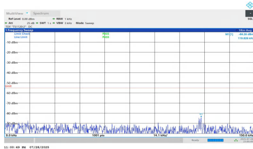
NTNV-n7-PC2-15-30-M-DFT-QPSK-Inner_1RB_Right-0.009-0.15 -PASS
