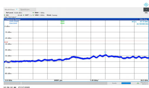
NTNV-n7-PC2-15-30-H-DFT-BPSK-Inner_1RB_Left-12000-26500- PASS
