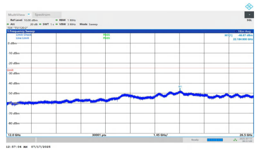
NTNV-n7-PC2-15-35-L-DFT-BPSK-Inner_1RB_Right-12000-2650 0-PASS
