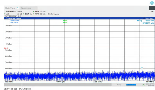
NTNV-n7-PC2-15-35-L-DFT-QPSK-Inner_1RB_Right-0.15-30-PASS
