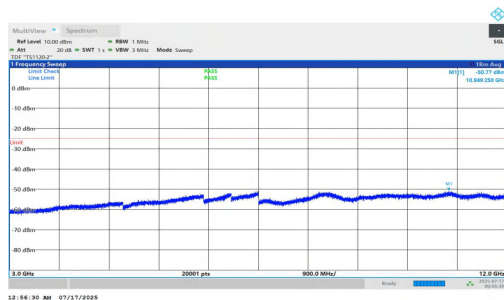
NTNV-n7-PC2-15-35-L-DFT-BPSK-Inner_1RB_Left-3000-12000- PASS
