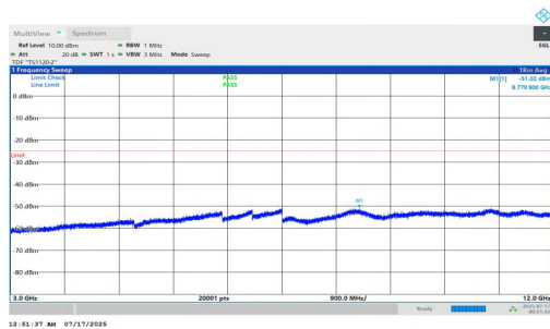
NTNV-n7-PC2-15-30-M-DFT-BPSK-Inner_1RB_Left-3000-12000- PASS
