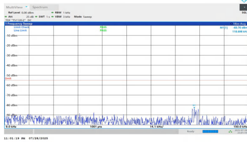
NTNV-n7-PC2-15-30-H-DFT-BPSK-Inner_1RB_Left-0.009-0.15-P ASS
