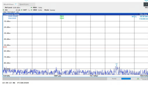
NTNV-n7-PC2-15-30-L-DFT-BPSK-Inner_1RB_Left-0.009-0.15-P ASS
