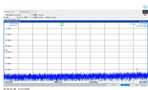
NTNV-n7-PC2-15-30-H-DFT-BPSK-Inner_1RB_Right-0.15-30-PAS S
