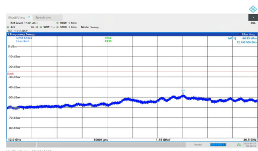
NTNV-n7-PC2-15-35-L-DFT-QPSK-Inner_1RB_Right-12000-26500-PASS
