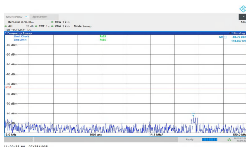
NTNV-n7-PC2-15-30-M-DFT-BPSK-Inner_1RB_Right-0.009-0.15 -PASS
