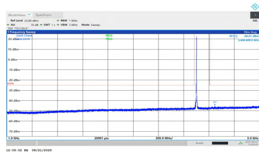
NTNV-n7-PC2-15-30-L-DFT-BPSK-Inner_1RB_Left-1000-3000-PASS S
