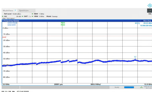
NTNV-n5-PC2-15-20-M-DFT-QPSK-Inner_1RB_Right-3000-12000-P ASS
