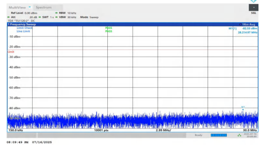
NTNV-n5-PC2-15-20-M-DFT-BPSK-Inner_1RB_Left-0.15-30-PASS
