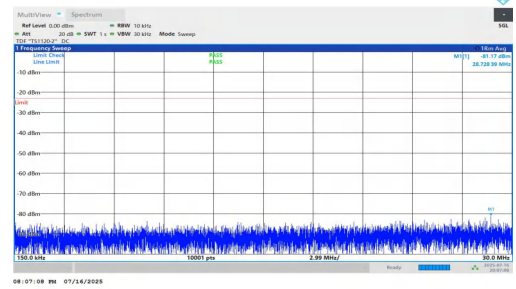
NTNV-n5-PC2-15-20-L-DFT-BPSK-Inner_1RB_Left-0.15-30-PASS
