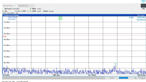
NTNV-n5-PC2-15-15-H-DFT-QPSK-Inner_1RB_Left-0.009-0.15-PASS
