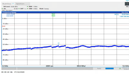
NTNV-n5-PC2-15-20-L-DFT-QPSK-Inner_1RB_Left-3000-12000-PAS
