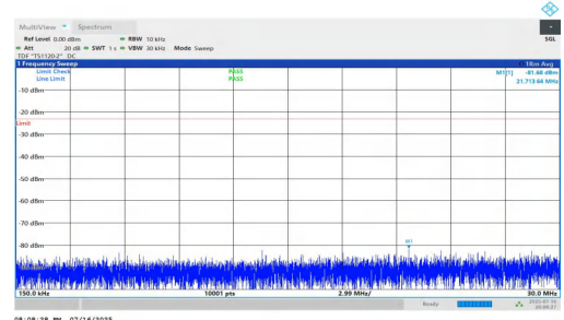
NTNV-n5-PC2-15-20-L-DFT-QPSK-Inner_1RB_Left-0.15-30-PASS
