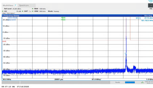
NTNV-n5-PC2-15-20-L-DFT-BPSK-Inner_1RB_Left-30-1000-PASS
