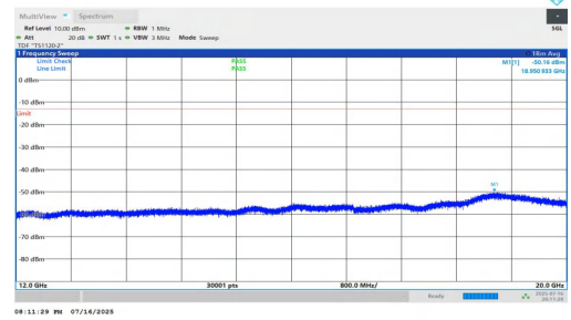
NTNV-n5-PC2-15-20-M-DFT-QPSK-Inner_1RB_Left-12000-20000-PA SS
