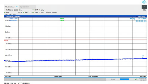
NTNV-n5-PC2-15-20-H-DFT-BPSK-Inner_1RB_Left-1000-3000-PASS
