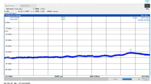
NTNV-n5-PC2-15-15-H-DFT-BPSK-Inner_1RB_Left-12000-20000-PAS
