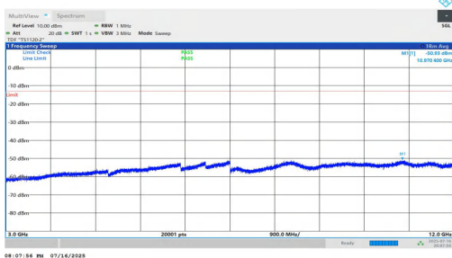
NTNV-n5-PC2-15-20-L-DFT-BPSK-Inner_1RB_Right-3000-12000-PA SS
