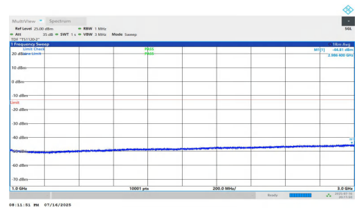
NTNV-n5-PC2-15-20-M-DFT-QPSK-Inner_1RB_Right-1000-3000-PAS S
