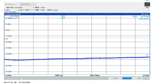
NTNV-n5-PC2-15-20-L-DFT-BPSK-Inner_1RB_Right-1000-3000-PASS
