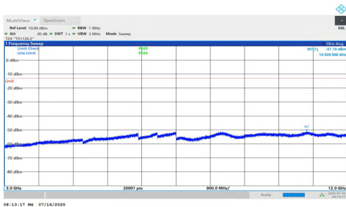
NTNV-n5-PC2-15-20-H-DFT-BPSK-Inner_1RB_Right-3000-12000-PASS SS
