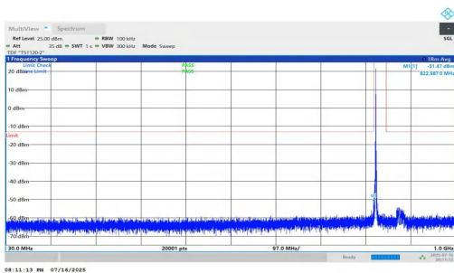
NTNV-n5-PC2-15-20-M-DFT-QPSK-Inner_1RB_Left-30-1000-PASS
