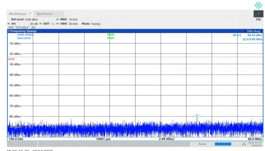
NTNV-n5-PC2-15-15-H-DFT-BPSK-Inner_1RB_Right-0.15-30-PASS
