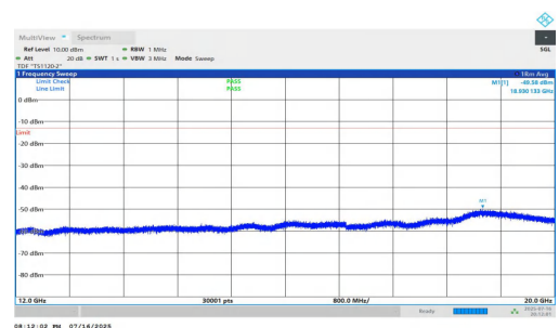
NTNV-n5-PC2-15-20-M-DFT-QPSK-Inner_1RB_Right-12000-20000-P ASS
