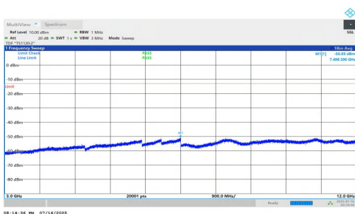
NTVN-n5-PC2-15-20-H-DFT-QPSK-Inner_1RB_Right-3000-12000-PA
