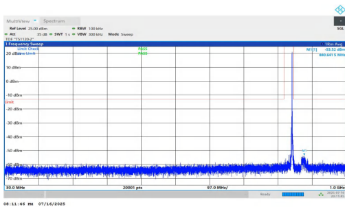
NTNV-n5-PC2-15-20-M-DFT-QPSK-Inner_1RB_Right-30-1000-PASS
