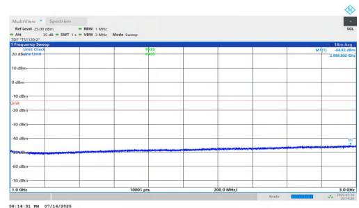
NTVN-n5-PC2-15-20-H-DFT-QPSK-Inner_1RB_Right-1000-3000-PAS
