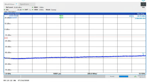
NTNV-n5-PC2-15-20-H-DFT-BPSK-Inner_1RB_Right-1000-3000-PASS S
