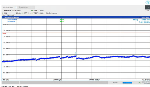
NTNV-n5-PC2-15-20-M-DFT-BPSK-Inner_1RB_Left-3000-12000-PAS S
