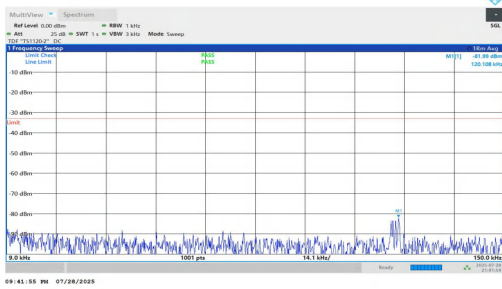
NTNV-n5-PC2-15-15-H-DFT-BPSK-Inner_1RB_Left-0.009-0.15-PASS
