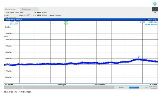
NTNV-n5-PC2-15-20-H-DFT-BPSK-Inner_1RB_Right-12000-20000-PASS SS
