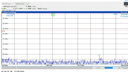
NTNV-n5-PC2-15-20-M-DFT-BPSK-Inner_1RB_Right-0.009-0.15-PA SS
