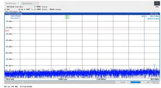
NTNV-n5-PC2-15-20-M-DFT-QPSK-Inner_1RB_Left-0.15-30-PASS
