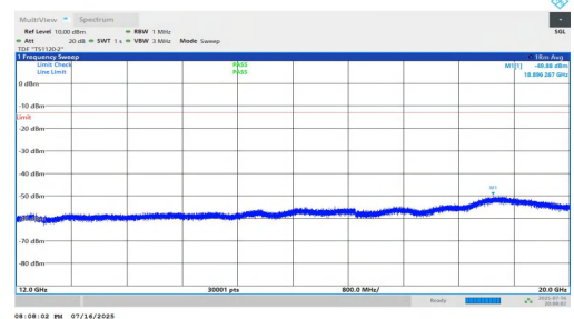
NTNV-n5-PC2-15-20-L-DFT-BPSK-Inner_1RB_Right-12000-20000-PA SS
