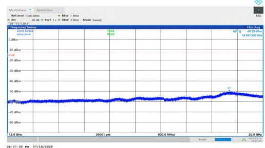
NTNV-n5-PC2-15-20-L-DFT-BPSK-Inner_1RB_Left-12000-20000-PAS
