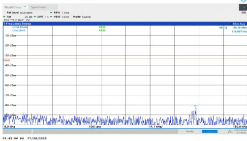
NTNV-n5-PC2-15-20-M-DFT-BPSK-Inner_1RB_Left-0.009-0.15-PAS S
