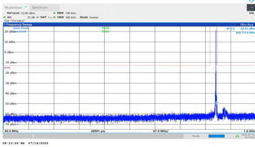
NTNV-n5-PC2-15-20-M-DFT-BPSK-Inner_1RB_Right-30-1000-PASS
