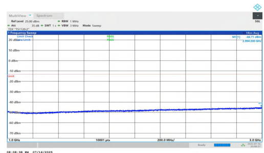
NTNV-n5-PC2-15-20-L-DFT-QPSK-Inner_1RB_Left-1000-3000-PASS
