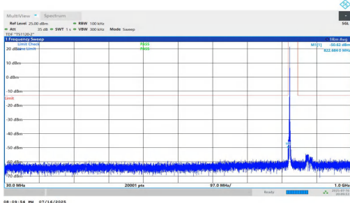
NTNV-n5-PC2-15-20-M-DFT-BPSK-Inner_1RB_Left-30-1000-PASS
