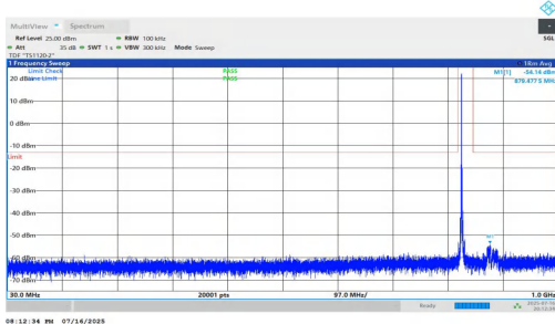
NTNV-n5-PC2-15-20-H-DFT-BPSK-Inner_1RB_Left-30-1000-PASS
