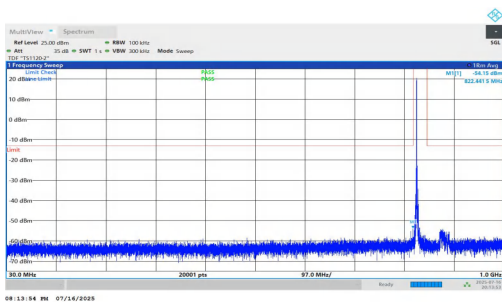
NTNV-n5-PC2-15-20-H-DFT-QPSK-Inner_1RB_Left-30-1000-PASS
