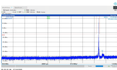
NTNV-n5-PC2-15-20-L-DFT-QPSK-Inner_1RB_Right-30-1000-PASS
