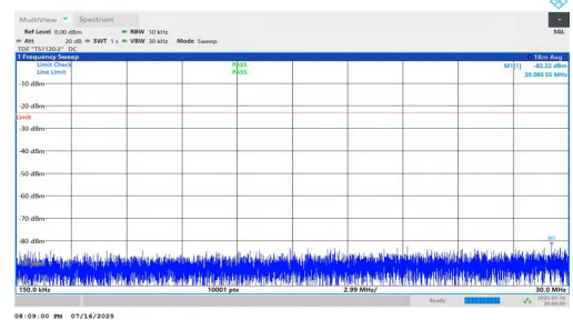
NTNV-n5-PC2-15-20-L-DFT-QPSK-Inner_1RB_Right-0.15-30-PASS
