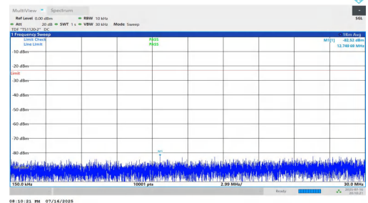
NTNV-n5-PC2-15-20-M-DFT-BPSK-Inner_1RB_Right-0.15-30-PASS
