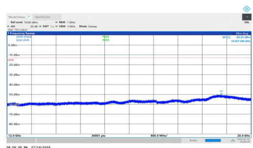
NTNV-n5-PC2-15-15-H-DFT-QPSK-Inner_1RB_Right-12000-20000-PA
