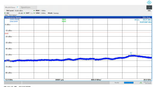
NTNV-n5-PC2-15-20-M-DFT-BPSK-Inner_1RB_Left-12000-20000-PAS S
