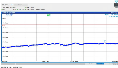
NTNV-n5-PC2-15-20-M-DFT-BPSK-Inner_1RB_Right-3000-12000-PASS SS
