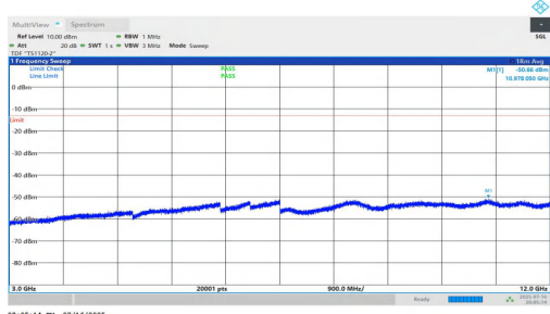
NTNV-n5-PC2-15-15-H-DFT-BPSK-Inner_1RB_Right-3000-12000-PASS
