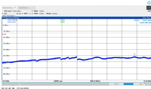
NTNV-n5-PC2-15-20-H-DFT-BPSK-Inner_1RB_Left-3000-12000-PAS
