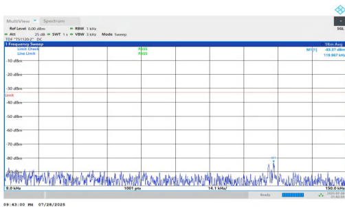
NTNV-n5-PC2-15-20-L-DFT-BPSK-Inner_1RB_Right-0.009-0.15-PAS
