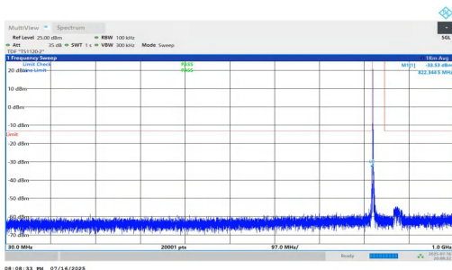
NTNV-n5-PC2-15-20-L-DFT-QPSK-Inner_1RB_Left-30-1000-PASS
