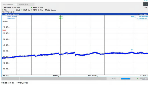
NTNV-n5-PC2-15-20-M-DFT-QPSK-Inner_1RB_Left-3000-12000-PA SS
