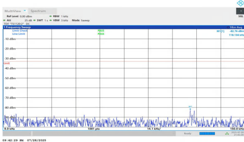
NTNV-n5-PC2-15-15-H-DFT-QPSK-Inner_1RB_Right-0.009-0.15-PA
