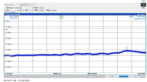
NTNV-n5-PC2-15-15-H-DFT-QPSK-Inner_1RB_Left-12000-20000-PAS
