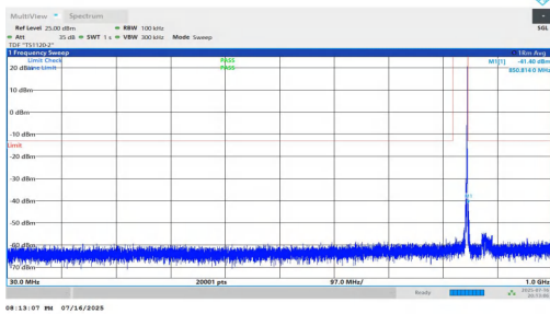
NTNV-n5-PC2-15-20-H-DFT-BPSK-Inner_1RB_Right-30-1000-PASS
