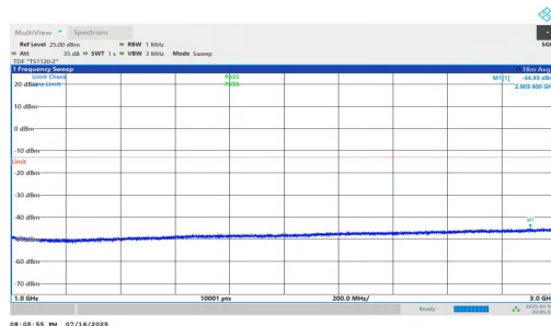
NTNV-n5-PC2-15-15-H-DFT-QPSK-Inner_1RB_Left-1000-3000-PASS
