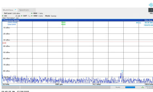
NTNV-n5-PC2-15-20-H-DFT-BPSK-Inner_1RB_Right-0.009-0.15-PAS
