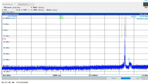
NTNV-n5-PC2-15-20-L-DFT-BPSK-Inner_1RB_Right-30-1000-PASS
