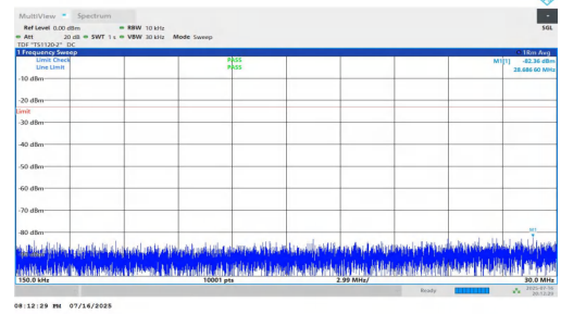
NTNV-n5-PC2-15-20-H-DFT-BPSK-Inner_1RB_Left-0.15-30-PASS
