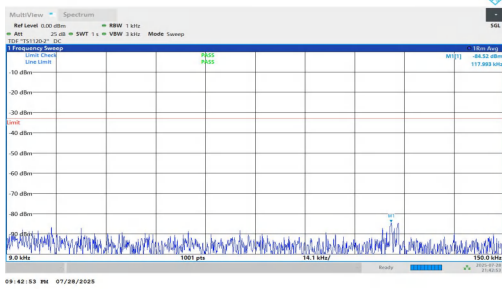
NTNV-n5-PC2-15-20-L-DFT-BPSK-Inner_1RB_Left-0.009-0.15-PASS
