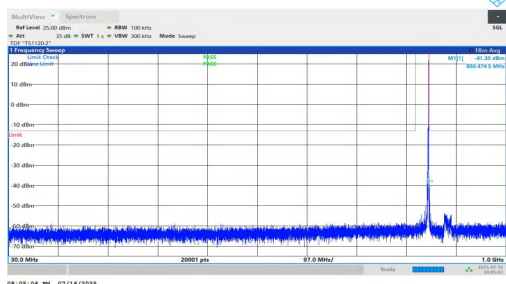
NTNV-n5-PC2-15-15-H-DFT-BPSK-Inner_1RB_Right-30-1000-PASS
