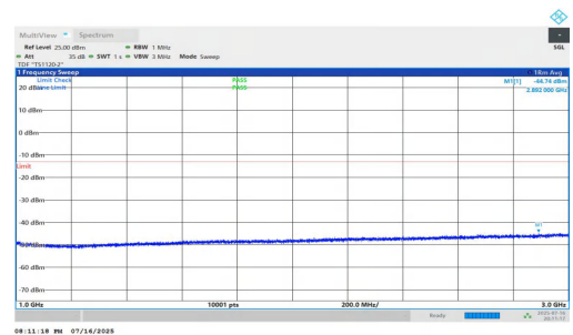
NTNV-n5-PC2-15-20-M-DFT-QPSK-Inner_1RB_Left-1000-3000-PASS
