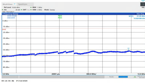
NTVN-n5-PC2-15-20-H-DFT-QPSK-Inner_1RB_Left-3000-12000-PAS
