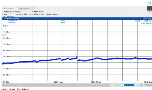
NTNV-n5-PC2-15-20-L-DFT-QPSK-Inner_1RB_Right-3000-12000-PA
