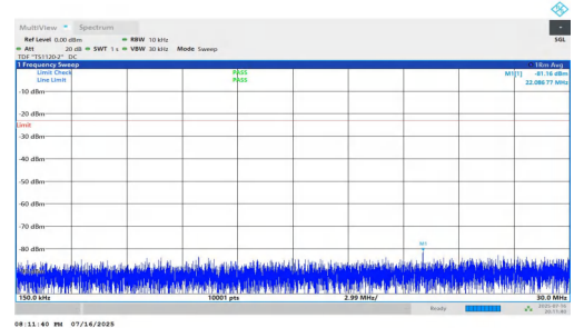
NTNV-n5-PC2-15-20-M-DFT-QPSK-Inner_1RB_Right-0.15-30-PASS
