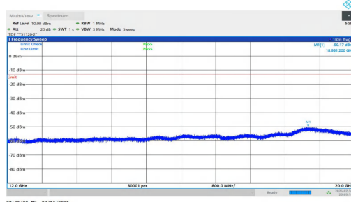
NTNV-n5-PC2-15-15-H-DFT-BPSK-Inner_1RB_Right-12000-20000-PASS
