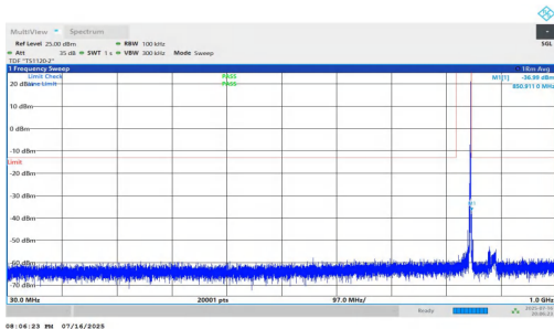
NTNV-n5-PC2-15-15-H-DFT-QPSK-Inner_1RB_Right-30-1000-PASS
