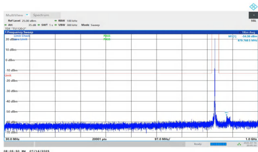
NTNV-n5-PC2-15-15-H-DFT-QPSK-Inner_1RB_Left-30-1000-PASS
