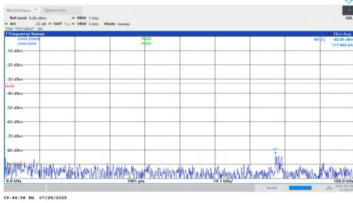
NTNV-n5-PC2-15-20-H-DFT-BPSK-Inner_1RB_Left-0.009-0.15-PASS
