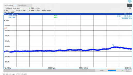
NTNV-n5-PC2-15-20-M-DFT-BPSK-Inner_1RB_Right-12000-20000-PASS SS
