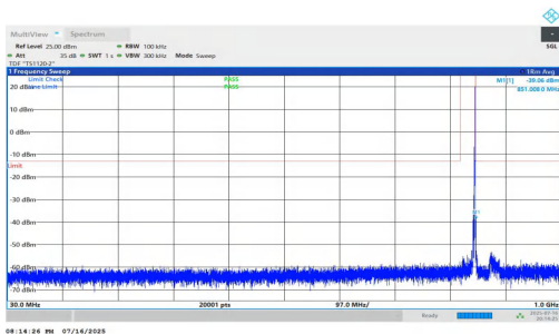
NTVN-n5-PC2-15-20-H-DFT-QPSK-Inner_1RB_Right-30-1000-PASS
