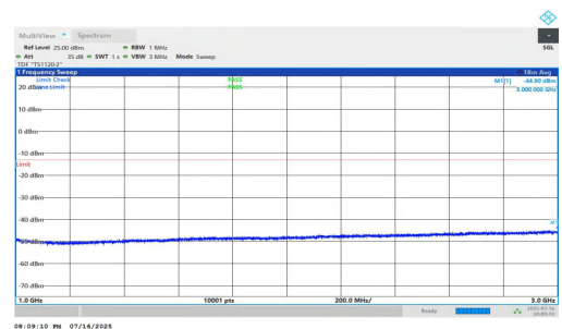
NTNV-n5-PC2-15-20-L-DFT-QPSK-Inner_1RB_Right-1000-3000-PASS
