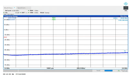
NTNV-n5-PC2-15-20-H-DFT-QPSK-Inner_1RB_Left-1000-3000-PASS
