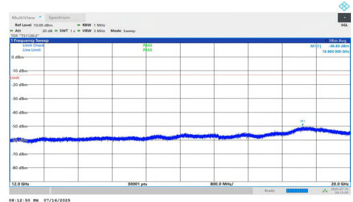
NTNV-n5-PC2-15-20-H-DFT-BPSK-Inner_1RB_Left-12000-20000-PAS
