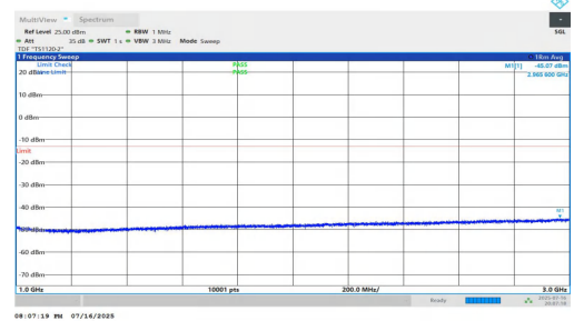
NTNV-n5-PC2-15-20-L-DFT-BPSK-Inner_1RB_Left-1000-3000-PASS
