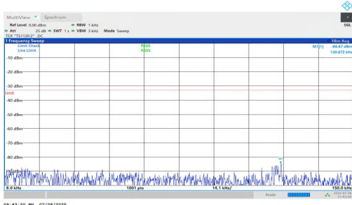
NTNV-n5-PC2-15-20-L-DFT-QPSK-Inner_1RB_Left-0.009-0.15-PASS
