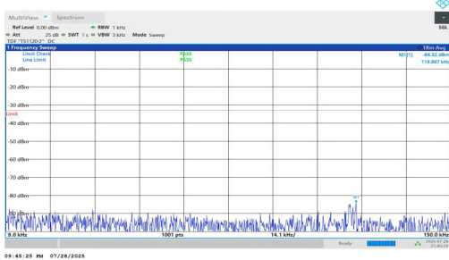
NTNV-n5-PC2-15-20-H-DFT-QPSK-Inner_1RB_Left-0.009-0.15-PASS S
