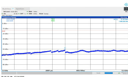
NTNV-n5-PC2-15-15-H-DFT-QPSK-Inner_1RB_Right-3000-12000-PA
