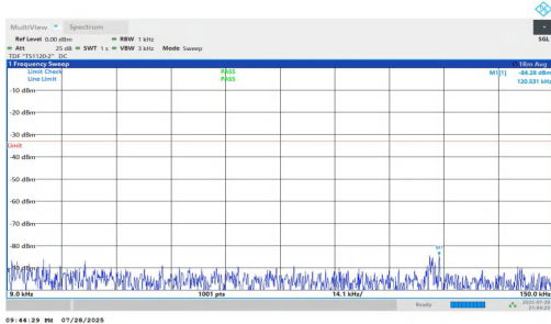
NTNV-n5-PC2-15-20-M-DFT-QPSK-Inner_1RB_Right-0.009-0.15-PA SS
