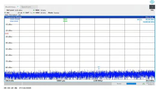
NTNV-n5-PC2-15-15-H-DFT-QPSK-Inner_1RB_Right-0.15-30-PASS
