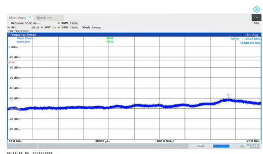
NTVN-n5-PC2-15-20-H-DFT-QPSK-Inner_1RB_Right-12000-20000-PA
