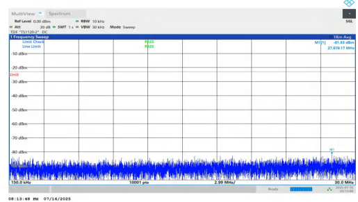
NTNV-n5-PC2-15-20-H-DFT-QPSK-Inner_1RB_Left-0.15-30-PASS
