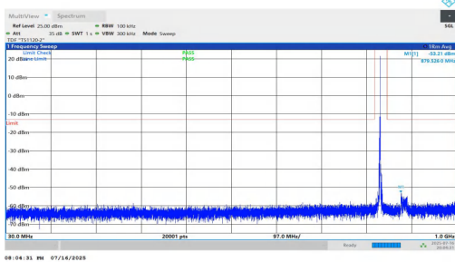
NTNV-n5-PC2-15-15-H-DFT-BPSK-Inner_1RB_Left-30-1000-PASS
