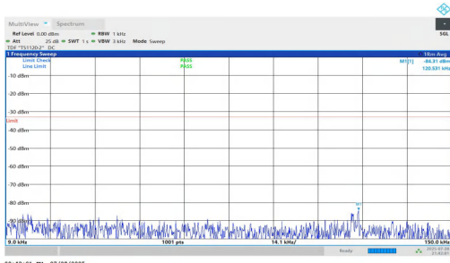
NTNV-n5-PC2-15-15-H-DFT-BPSK-Inner_1RB_Right-0.009-0.15-PAS
