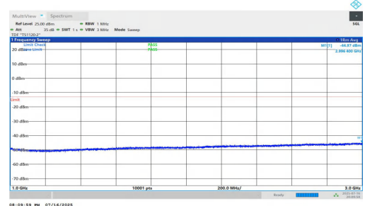
NTNV-n5-PC2-15-20-M-DFT-BPSK-Inner_1RB_Left-1000-3000-PASS
