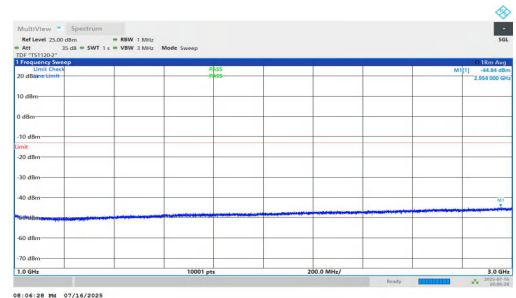
NTNV-n5-PC2-15-15-H-DFT-QPSK-Inner_1RB_Right-1000-3000-PAS
