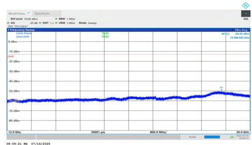
NTNV-n5-PC2-15-20-L-DFT-QPSK-Inner_1RB_Right-12000-20000-PA
