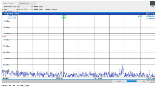
NTNV-n5-PC2-15-20-M-DFT-QPSK-Inner_1RB_Left-0.009-0.15-PASS S
