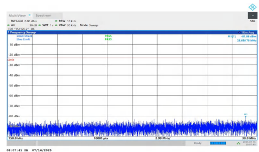
NTNV-n5-PC2-15-20-L-DFT-BPSK-Inner_1RB_Right-0.15-30-PASS
