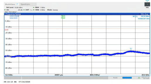
NTVN-n5-PC2-15-20-H-DFT-QPSK-Inner_1RB_Left-12000-20000-PAS
