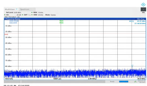
NTNV-n5-PC2-15-20-H-DFT-BPSK-Inner_1RB_Right-0.15-30-PASS
