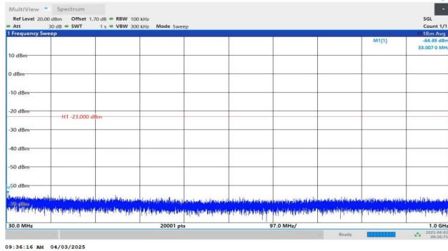
Band4-5MHz-QPSK-20175-1RB#0-30~1000-PASS
