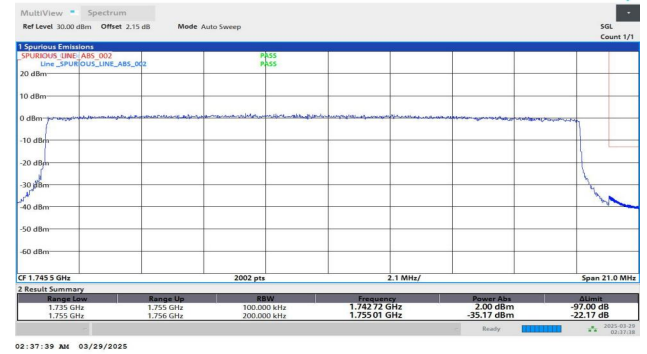
Band4-20MHz-QPSK-20300-100RB#0-PASS
