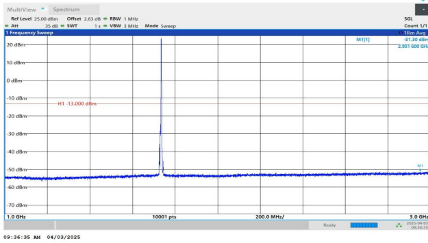
Band4-5MHz-QPSK-20175-1RB#24-1000~3000-PASS
