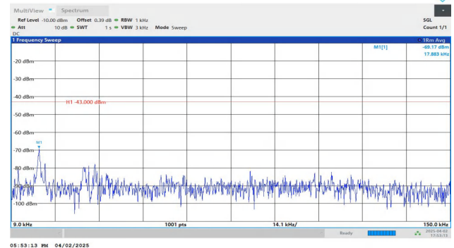
Band4-3MHz-QPSK-19965-1RB#14-0.009~0.15-PASS
