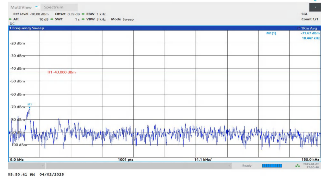
Band4-1.4MHz-QPSK-20175-1RB#5-0.009~0.15-PASS
