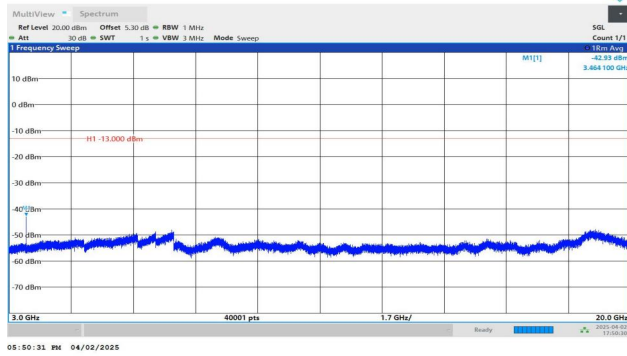
Band4-1.4MHz-QPSK-20175-1RB#0-3000~20000-PASS
