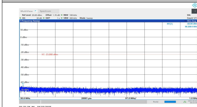
Band4-1.4MHz-QPSK-20175-1RB#0-30~1000-PASS
