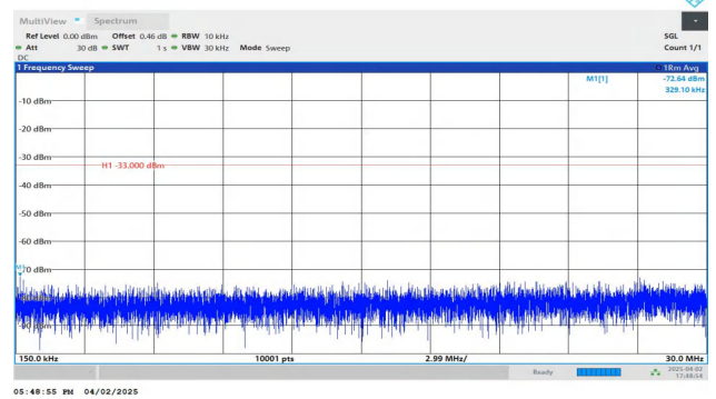
Band4-1.4MHz-QPSK-19957-1RB#0-0.15~30-PASS
