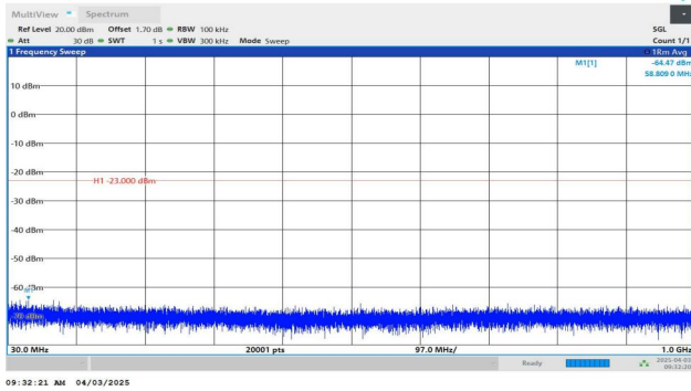
Band4-1.4MHz-QPSK-19957-1RB#0-30~1000-PASS
