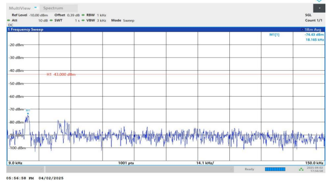
Band4-5MHz-QPSK-19975-1RB#24-0.009~0.15-PASS
