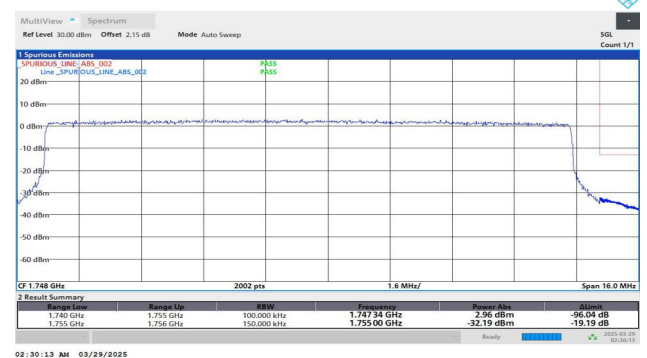
Band4-15MHz-QPSK-20325-75RB#0-PASS
