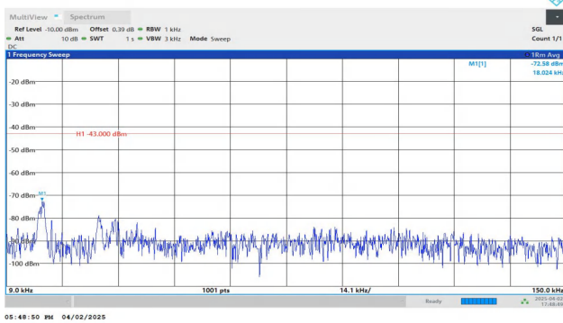
Band4-1.4MHz-QPSK-19957-1RB#0-0.009~0.15-PASS
