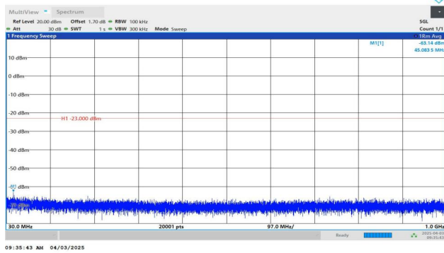
Band4-5MHz-QPSK-19975-1RB#0-30~1000-PASS
