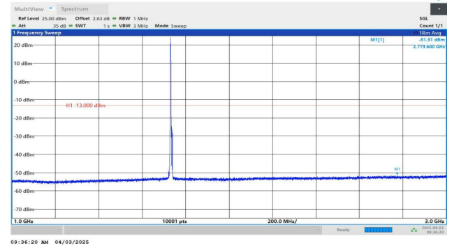
Band4-5MHz-QPSK-20175-1RB#0-1000~3000-PASS
