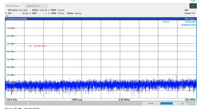
Band4-1.4MHz-QPSK-20393-1RB#0-0.15~30-PASS
