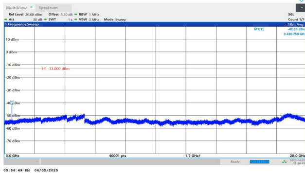
Band4-5MHz-QPSK-19975-1RB#0-3000~20000-PASS
