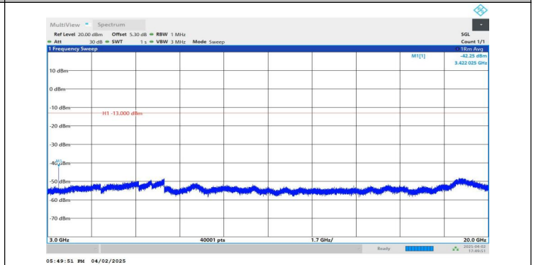
Band4-1.4MHz-QPSK-19957-1RB#5-3000~20000-PASS
