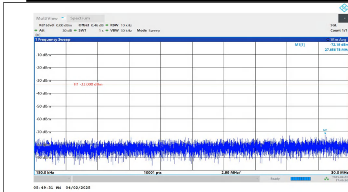
Band4-1.4MHz-QPSK-19957-1RB#5-0.15~30-PASS
