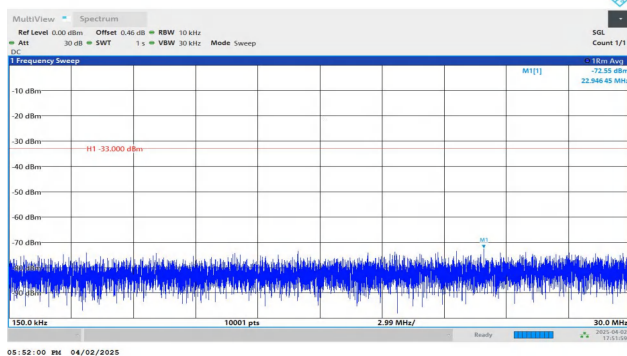
Band4-1.4MHz-QPSK-20393-1RB#5-0.15~30-PASS
