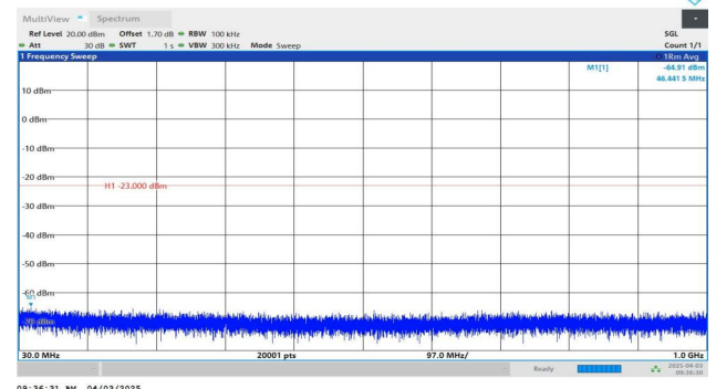
Band4-5MHz-QPSK-20175-1RB#24-30~1000-PASS
