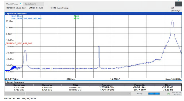
Band4-15MHz-QPSK-20025-1RB#74-PASS
