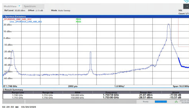
Band4-15MHz-QPSK-20325-1RB#74-PASS
