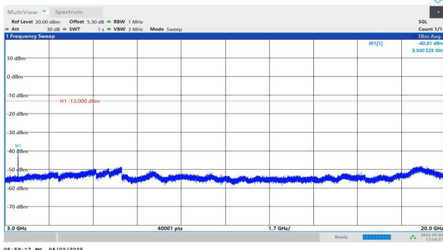
Band4-5MHz-QPSK-20375-1RB#0-3000~20000-PASS
