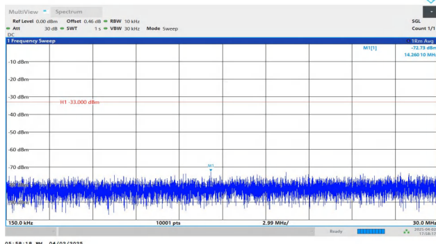
Band4-5MHz-QPSK-20175-1RB#24-0.15~30-PASS
