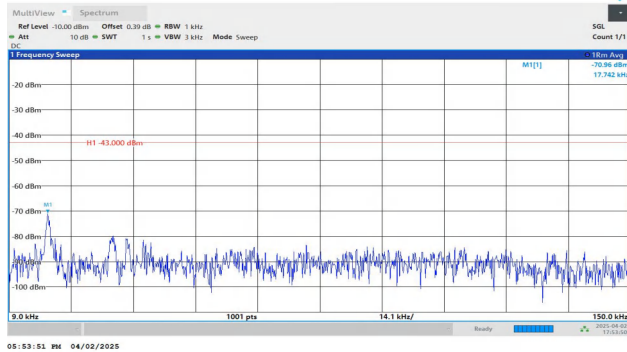
Band4-3MHz-QPSK-20175-1RB#0-0.009~0.15-PASS
