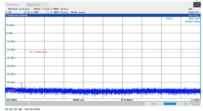
Band4-1.4MHz-QPSK-20175-1RB#5-30~1000-PASS
