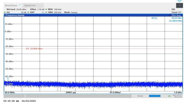
Band4-5MHz-QPSK-19975-1RB#24-30~1000-PASS
