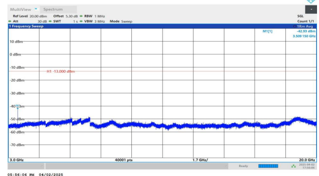
Band4-3MHz-QPSK-20385-1RB#14-3000~20000-PASS
