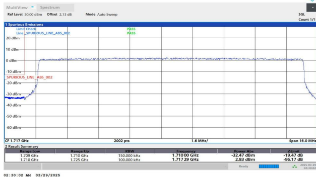
Band4-15MHz-QPSK-20025-75RB#0-PASS
