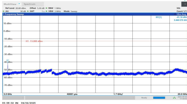
Band4-5MHz-QPSK-20175-1RB#0-3000~20000-PASS
