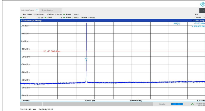
Band4-1.4MHz-QPSK-19957-1RB#5-1000~3000-PASS
