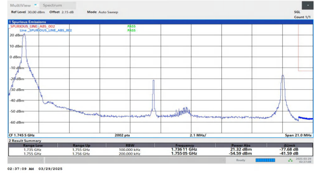
Band4-20MHz-QPSK-20300-1RB#0-PASS
