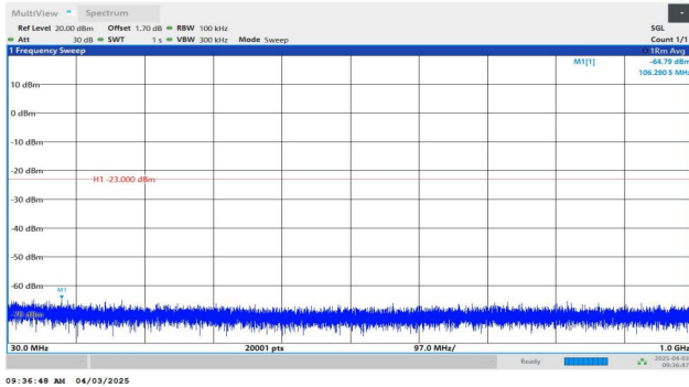
Band4-5MHz-QPSK-20375-1RB#0-30~1000-PASS
