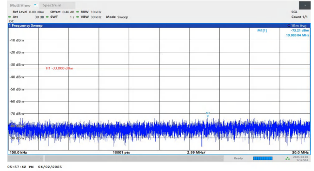
Band4-5MHz-QPSK-20175-1RB#0-0.15~30-PASS
