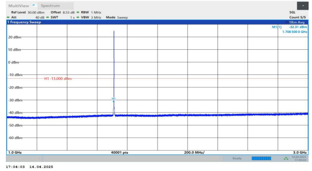
Band4-1.4MHz-QPSK-19957-1RB#0-1000~3000-PASS
