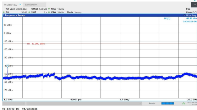
Band4-3MHz-QPSK-19965-1RB#0-3000~20000-PASS
