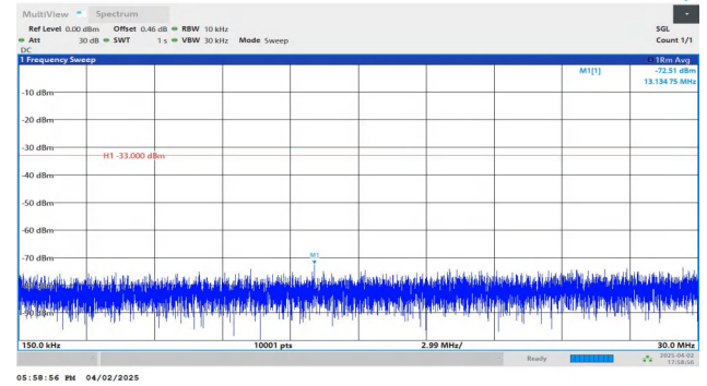
Band4-5MHz-QPSK-20375-1RB#0-0.15~30-PASS
