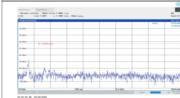
Band4-1.4MHz-QPSK-20175-1RB#0-0.009~0.15-PASS
