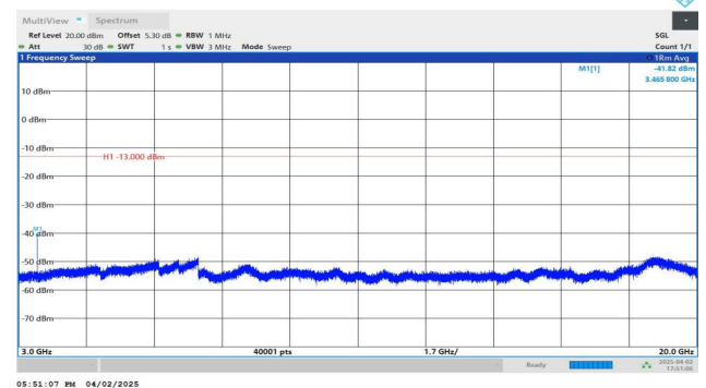
Band4-1.4MHz-QPSK-20175-1RB#5-3000~20000-PASS
