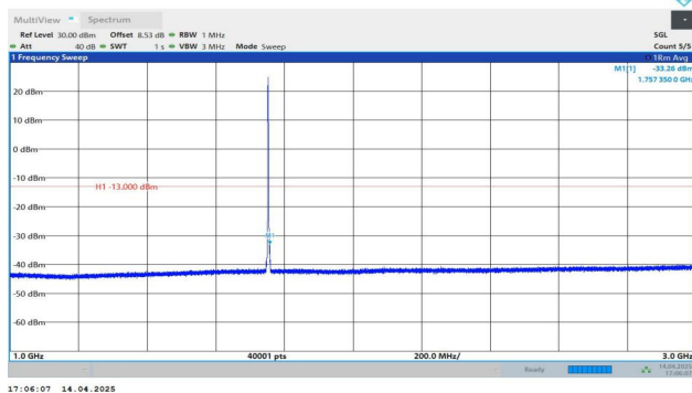
Band4-3MHz-QPSK-20385-1RB#14-1000~3000-PASS
