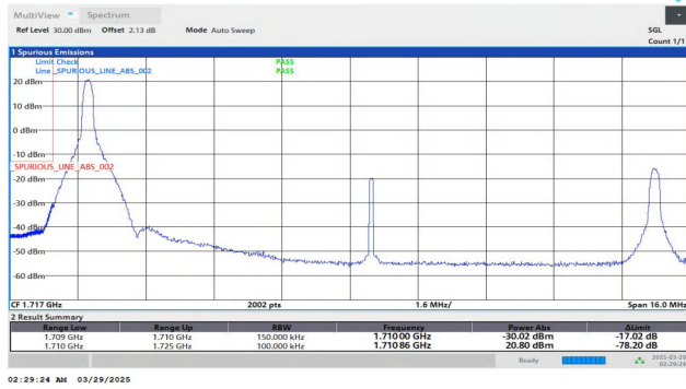
Band4-15MHz-QPSK-20025-1RB#0-PASS
