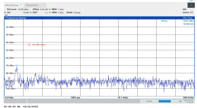
Band4-1.4MHz-QPSK-19957-1RB#5-0.009~0.15-PASS
