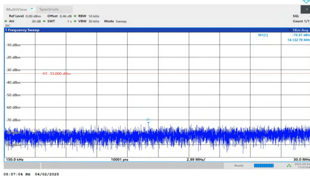
Band4-5MHz-QPSK-19975-1RB#24-0.15~30-PASS
