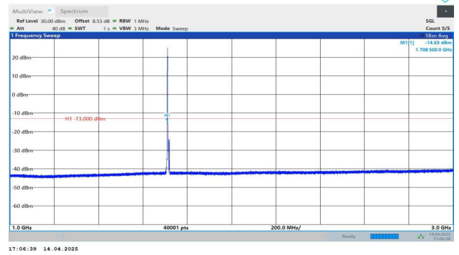
Band4-5MHz-QPSK-19975-1RB#0-1000~3000-PASS
