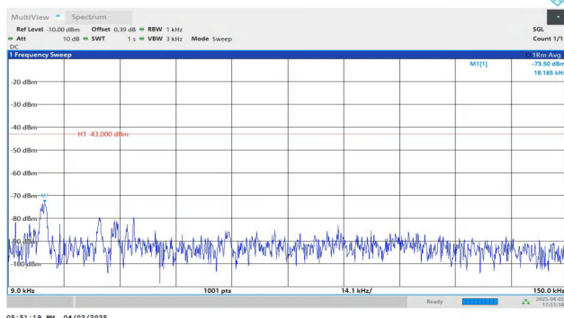
Band4-1.4MHz-QPSK-20393-1RB#0-0.009~0.15-PASS
