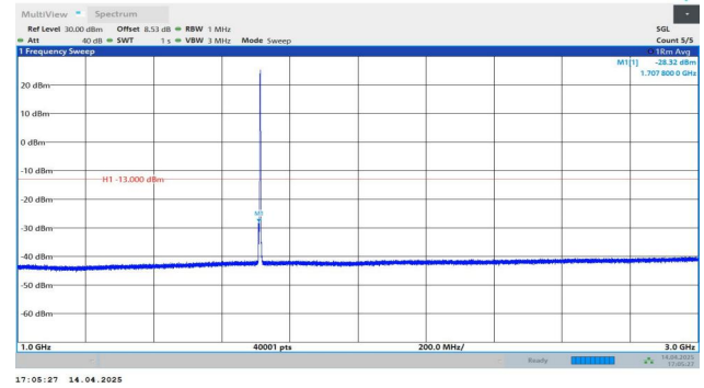
Band4-3MHz-QPSK-19965-1RB#0-1000~3000-PASS
