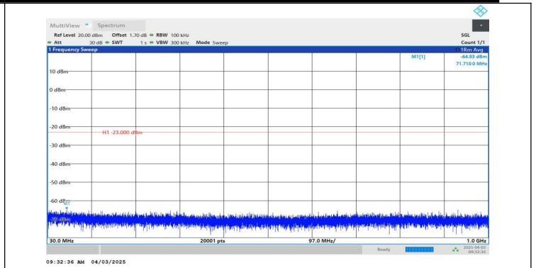
Band4-1.4MHz-QPSK-19957-1RB#5-30~1000-PASS
