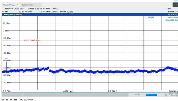
Band4-1.4MHz-QPSK-19957-1RB#0-3000~20000-PASS
