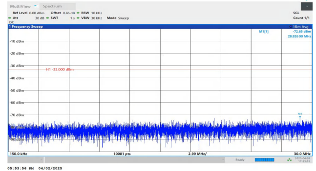
Band4-3MHz-QPSK-20175-1RB#0-0.15~30-PASS
