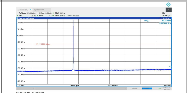
Band4-1.4MHz-QPSK-20175-1RB#0-1000~3000-PASS
