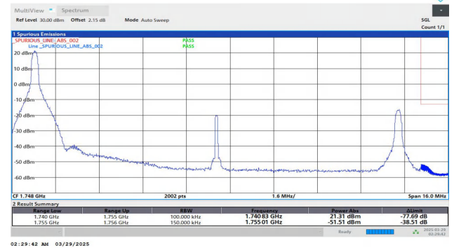
Band4-15MHz-QPSK-20325-1RB#0-PASS
