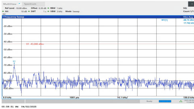
Band4-5MHz-QPSK-20375-1RB#0-0.009~0.15-PASS
