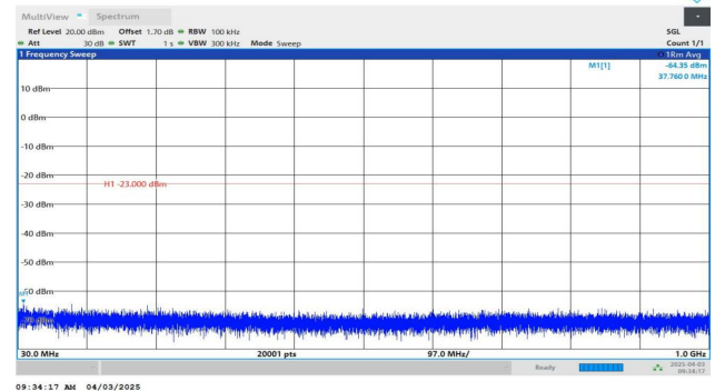
Band4-3MHz-QPSK-19965-1RB#14-30~1000-PASS
