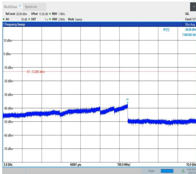
Band5-10MHz-QPSK-20450-1RB#0-3000~10000-PASS
