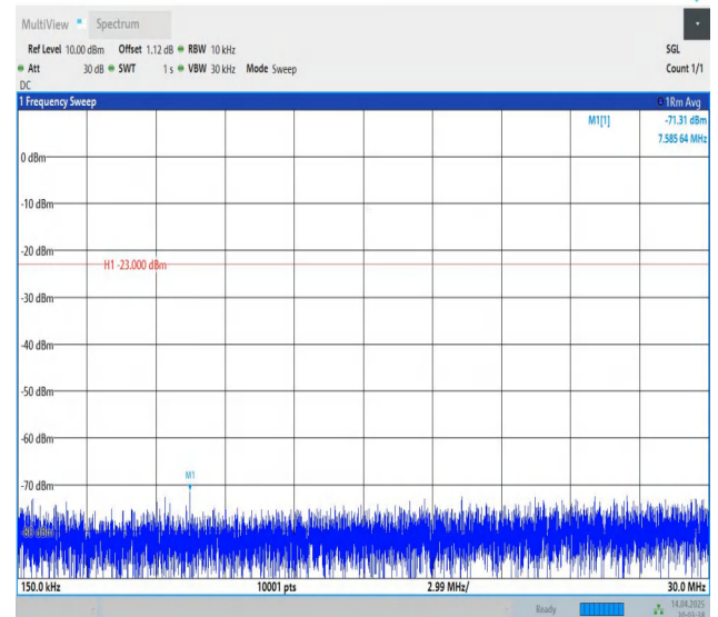
Band5-3MHz-QPSK-20635-1RB#0-0.15~30-PASS
