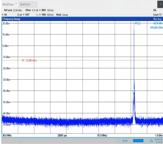
Band5-3MHz-QPSK-20415-1RB#0-30~1000-PASS
