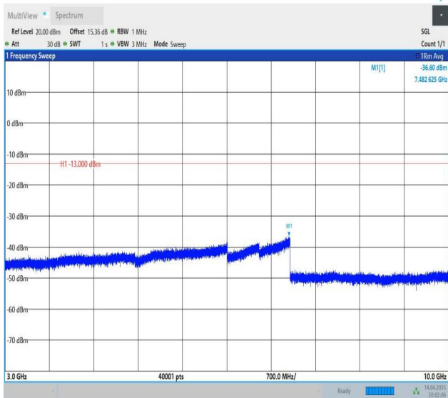
Band5-3MHz-QPSK-20415-1RB#0-3000~10000-PASS
