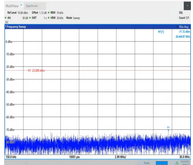
Band5-5MHz-QPSK-20525-1RB#0-0.15~30-PASS
