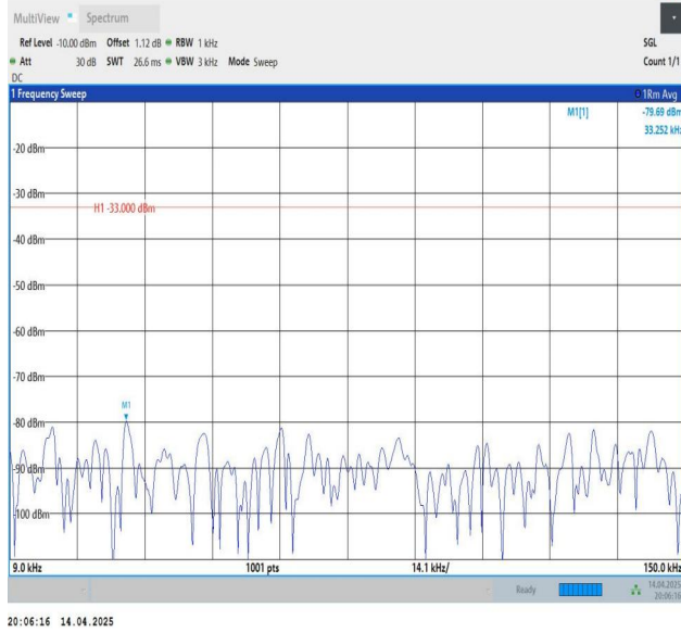
Band5-5MHz-QPSK-20625-1RB#0-0.009~0.15-PASS
