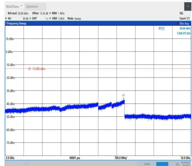
Band5-10MHz-QPSK-20600-1RB#49-3000~10000-PASS
