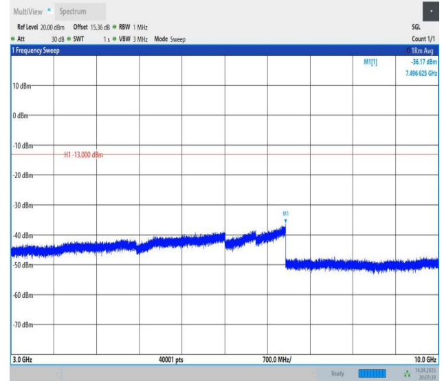
Band5-1.4MHz-QPSK-20643-1RB#5-3000~10000-PASS
