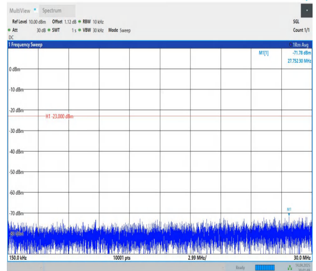
Band5-3MHz-QPSK-20415-1RB#0-0.15~30-PASS
