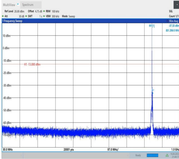
Band5-3MHz-QPSK-20635-1RB#0-30~1000-PASS
