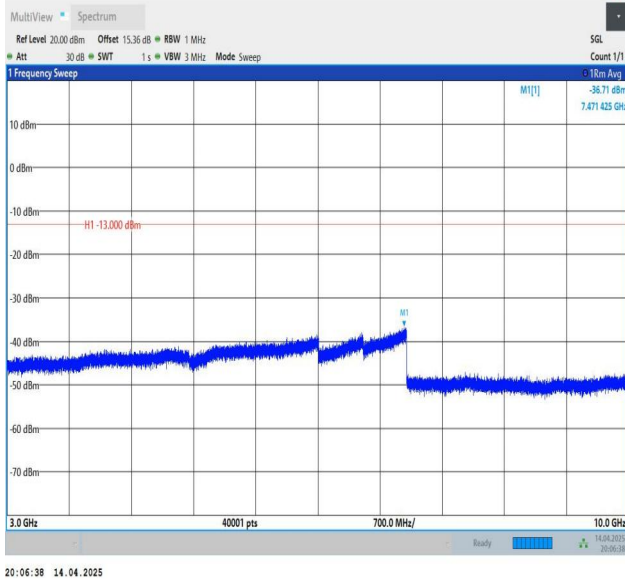
Band5-5MHz-QPSK-20625-1RB#0-3000~10000-PASS
