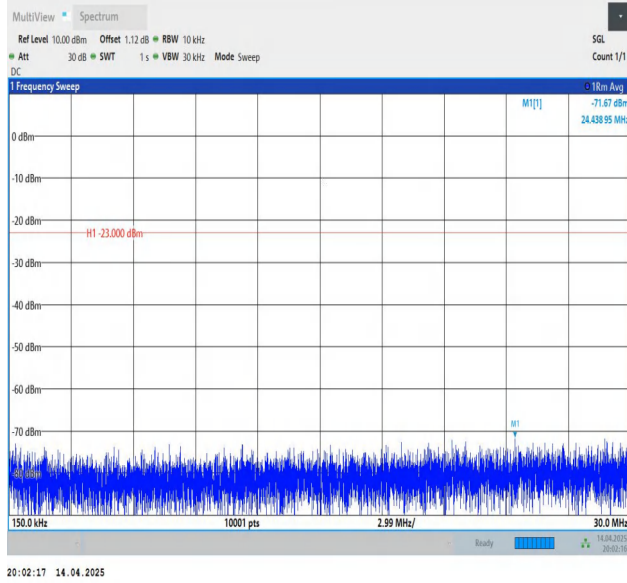
Band5-3MHz-QPSK-20415-1RB#14-0.15~30-PASS
