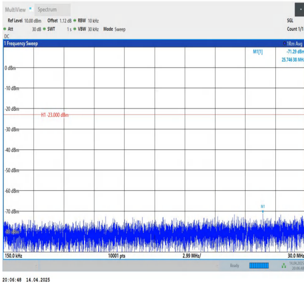
Band5-5MHz-QPSK-20625-1RB#24-0.15~30-PASS
