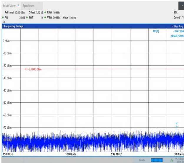
Band5-10MHz-QPSK-20525-1RB#49-0.15~30-PASS
