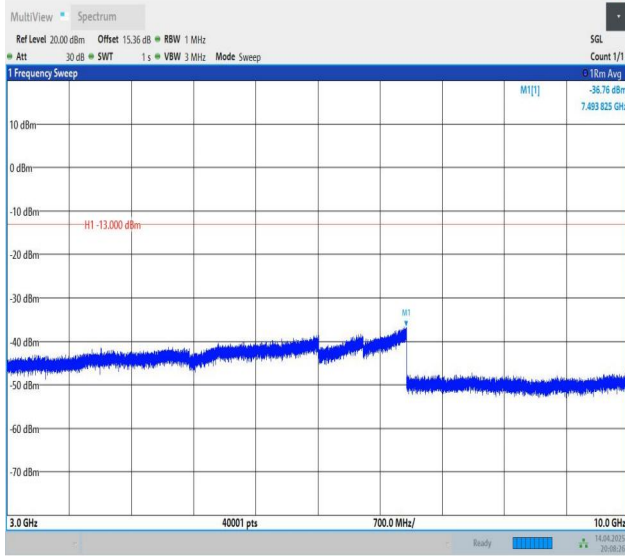
Band5-10MHz-QPSK-20525-1RB#0-3000~10000-PASS
