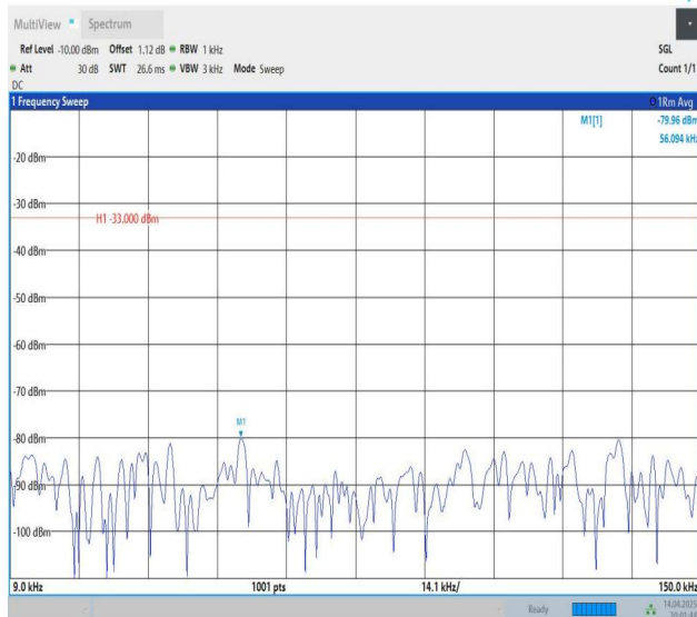
Band5-3MHz-QPSK-20415-1RB#0-0.009~0.15-PASS
