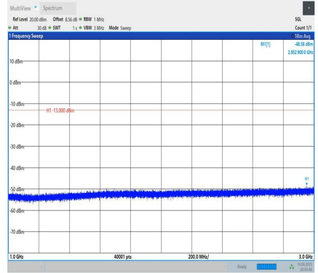
Band5-3MHz-QPSK-20635-1RB#0-1000~3000-PASS
