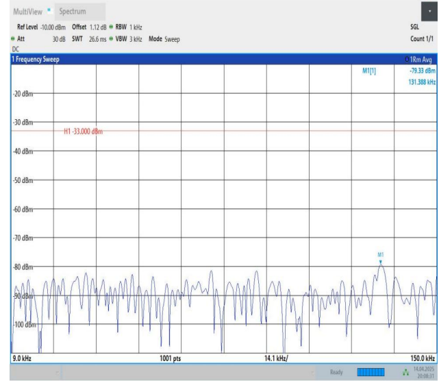
Band5-10MHz-QPSK-20525-1RB#49-0.009~0.15-PASS
