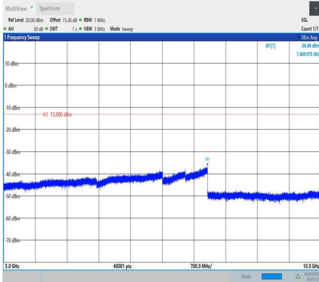
Band5-1.4MHz-QPSK-20643-1RB#0-3000~10000-PASS
