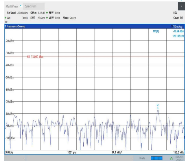
Band5-10MHz-QPSK-20450-1RB#49-0.009~0.15-PASS
