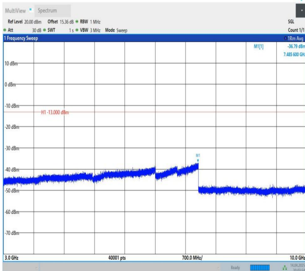
Band5-3MHz-QPSK-20635-1RB#0-3000~10000-PASS
