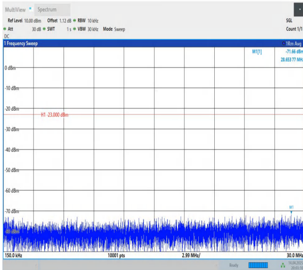
Band5-3MHz-QPSK-20525-1RB#14-0.15~30-PASS
