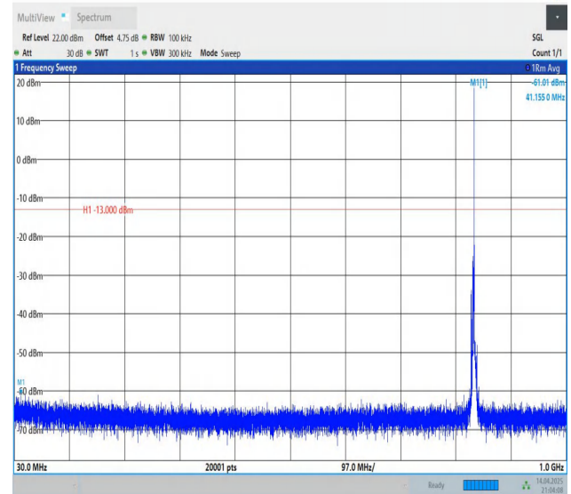
Band5-3MHz-QPSK-20525-1RB#14-30~1000-PASS
