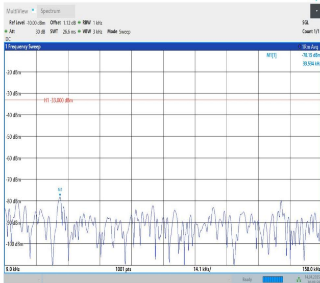
Band5-10MHz-QPSK-20600-1RB#0-0.009~0.15-PASS
