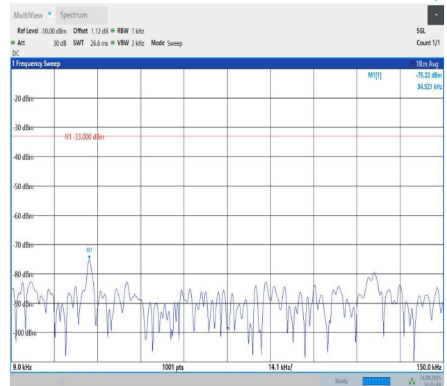
Band5-5MHz-QPSK-20525-1RB#24-0.009~0.15-PASS
