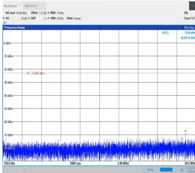
Band5-10MHz-QPSK-20600-1RB#49-0.15~30-PASS
