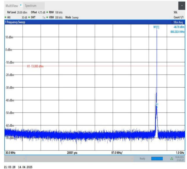
Band5-5MHz-QPSK-20625-1RB#24-30~1000-PASS
