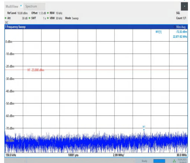
Band5-10MHz-QPSK-20600-1RB#0-0.15~30-PASS
