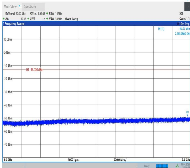
Band5-10MHz-QPSK-20600-1RB#49-1000~3000-PASS
