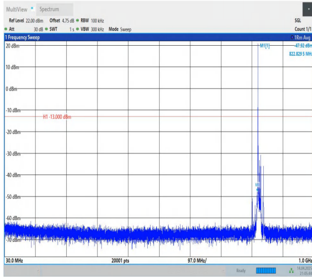
Band5-10MHz-QPSK-20450-1RB#0-30~1000-PASS
