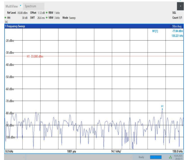
Band5-3MHz-QPSK-20415-1RB#14-0.009~0.15-PASS
