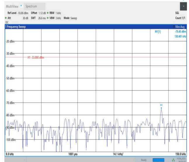
Band5-3MHz-QPSK-20635-1RB#14-0.009~0.15-PASS
