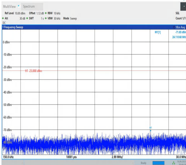
Band5-5MHz-QPSK-20425-1RB#24-0.15~30-PASS
