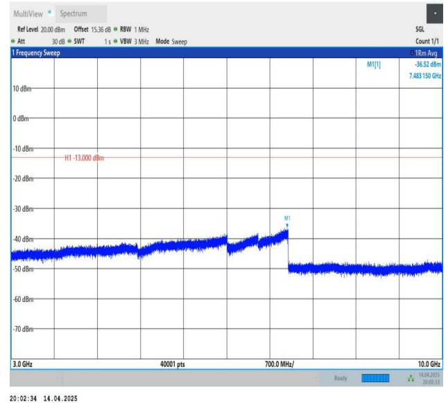
Band5-3MHz-QPSK-20415-1RB#14-3000~10000-PASS
