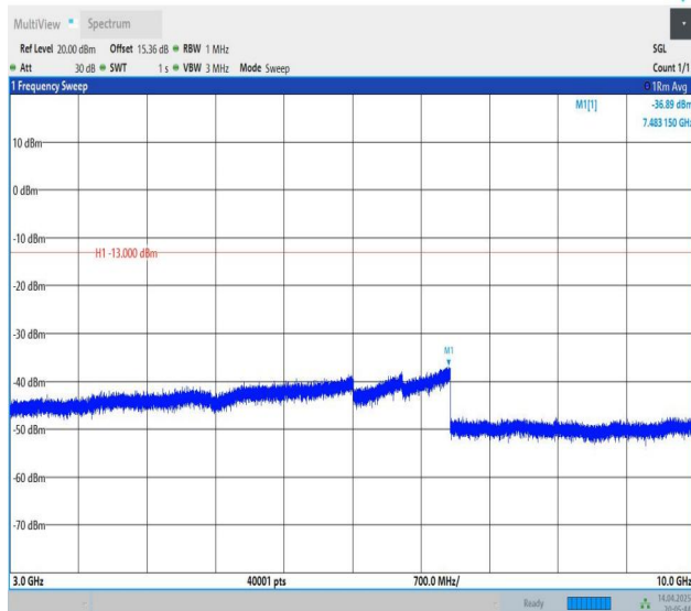
Band5-5MHz-QPSK-20525-1RB#0-3000~10000-PASS
