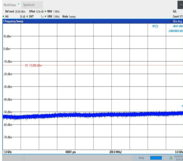
Band5-1.4MHz-QPSK-20643-1RB#5-1000~3000-PASS
