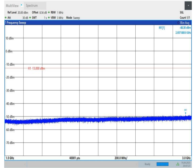
Band5-10MHz-QPSK-20450-1RB#0-1000~3000-PASS
