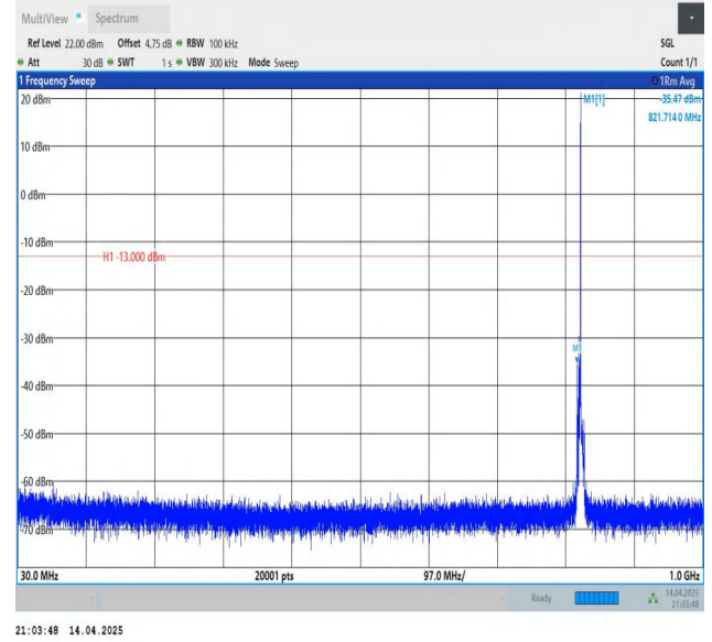
Band5-3MHz-QPSK-20415-1RB#14-30~1000-PASS
