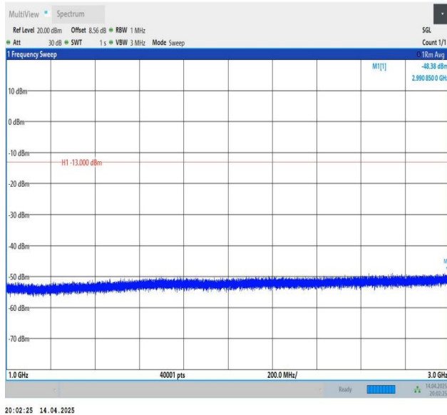
Band5-3MHz-QPSK-20415-1RB#14-1000~3000-PASS
