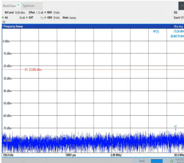
Band5-1.4MHz-QPSK-20643-1RB#5-0.15~30-PASS
