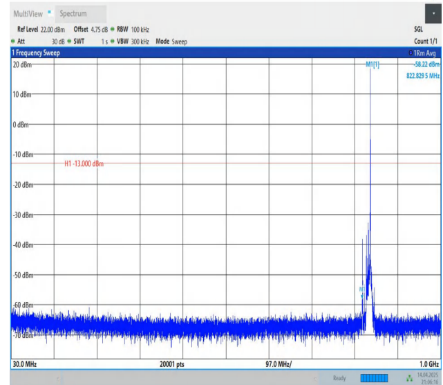
Band5-10MHz-QPSK-20525-1RB#49-30~1000-PASS
