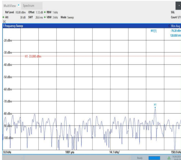
Band5-5MHz-QPSK-20525-1RB#0-0.009~0.15-PASS
