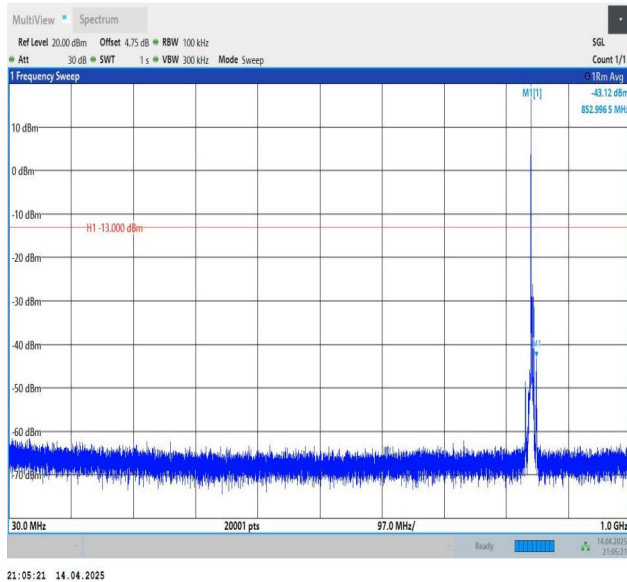
Band5-5MHz-QPSK-20625-1RB#0-30~1000-PASS
