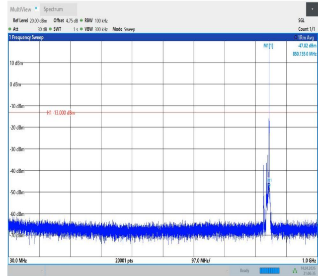
Band5-10MHz-QPSK-20600-1RB#49-30~1000-PASS
