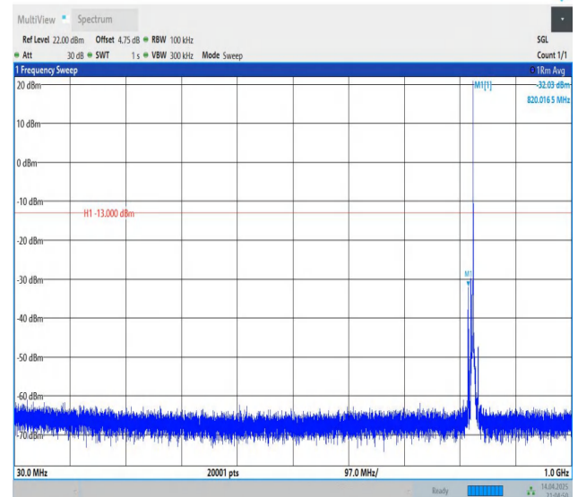
Band5-5MHz-QPSK-20425-1RB#24-30~1000-PASS
