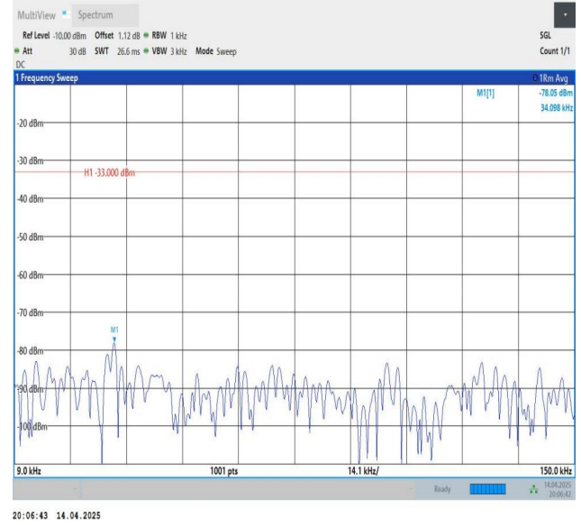
Band5-5MHz-QPSK-20625-1RB#24-0.009~0.15-PASS
