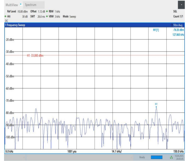
Band5-3MHz-QPSK-20525-1RB#14-0.009~0.15-PASS
