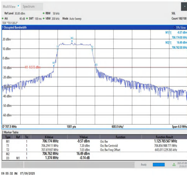
Band12-3MHz-16QAM-23095-PASS
