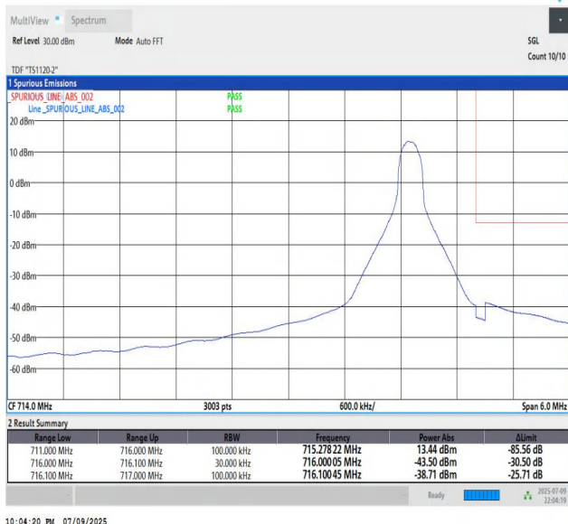
Band12_5MHz_QPSK_23155_1_High
