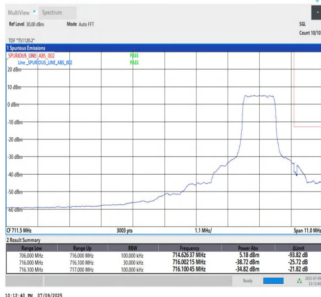
Band12_10MHz_QPSK_23130_6_High
