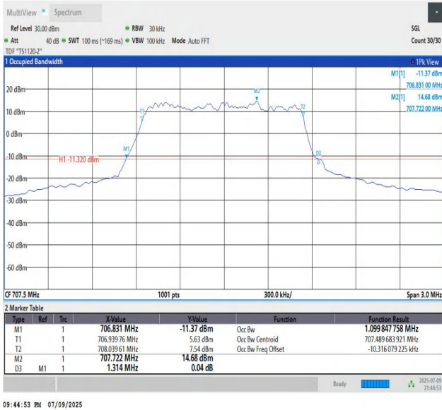
Band12-1.4MHz-16QAM-23095-PASS
