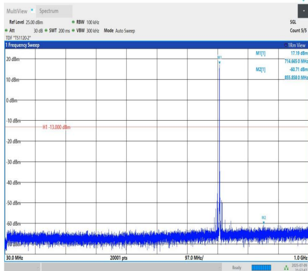
Band12-3MHz-QPSK-23165-PASS
