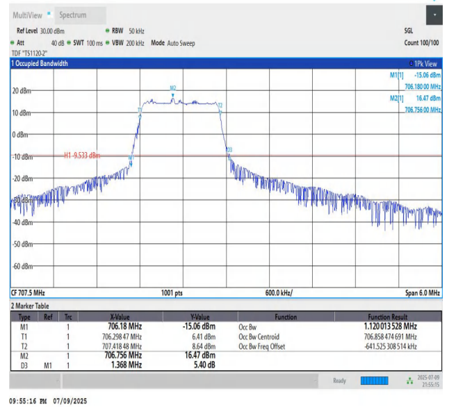
Band12-3MHz-QPSK-23095-PASS
