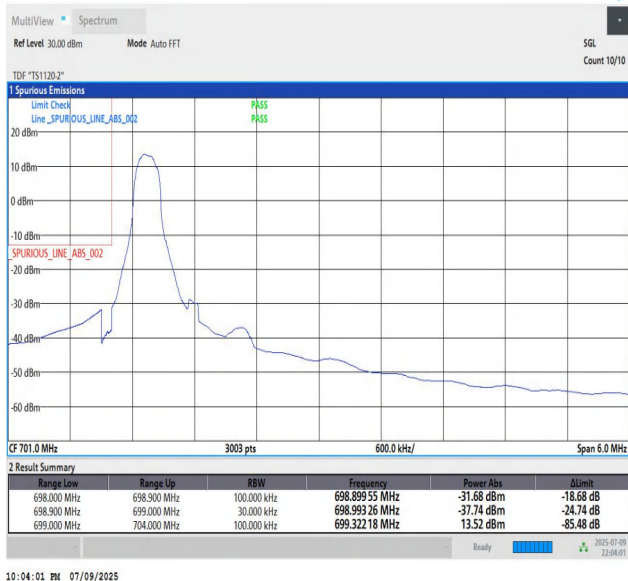
Band12_5MHz_QPSK_23035_1_Low
