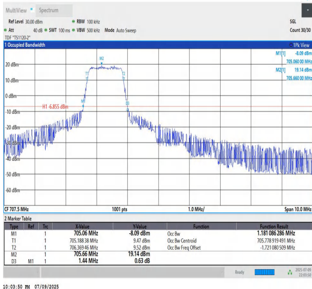
Band12-5MHz-16QAM-23095-PASS
