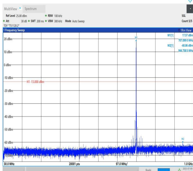
Band12-1.4MHz-QPSK-23095-PASS
