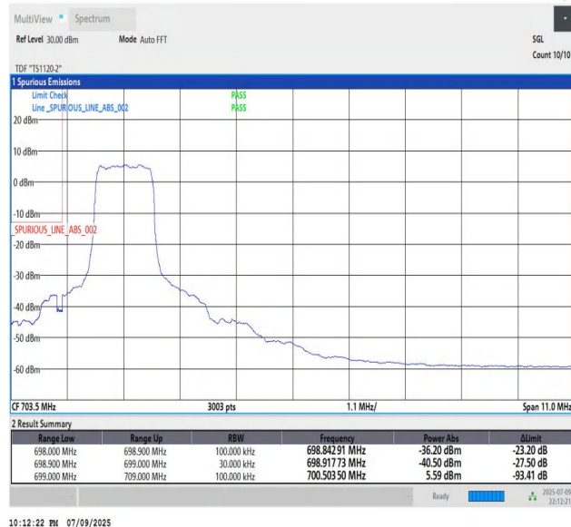
Band12_10MHz_QPSK_23060_6_Low
