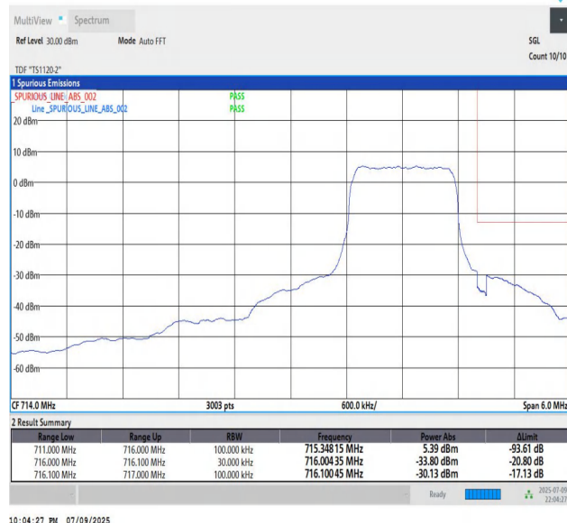
Band12_5MHz_QPSK_23155_6_High
