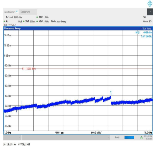
Band12-10MHz-QPSK-23060-PASS
