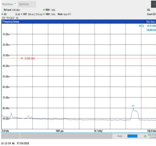
Band12-10MHz-QPSK-23130-PASS
