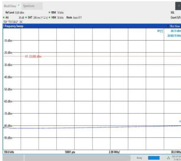
Band12-1.4MHz-QPSK-23095-PASS
