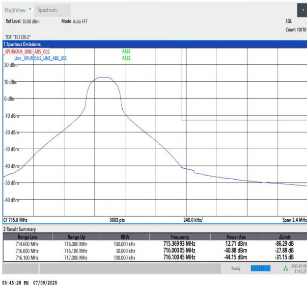
Band12_1.4MHz_QPSK_23173_1_High
