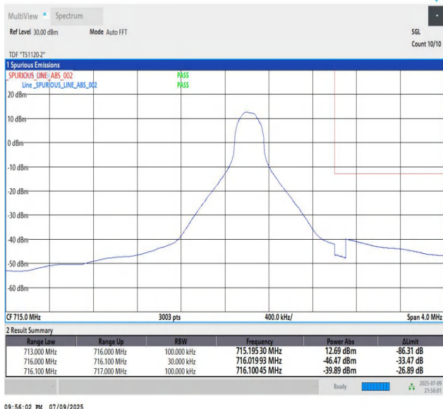
Band12_3MHz_QPSK_23165_1_High
