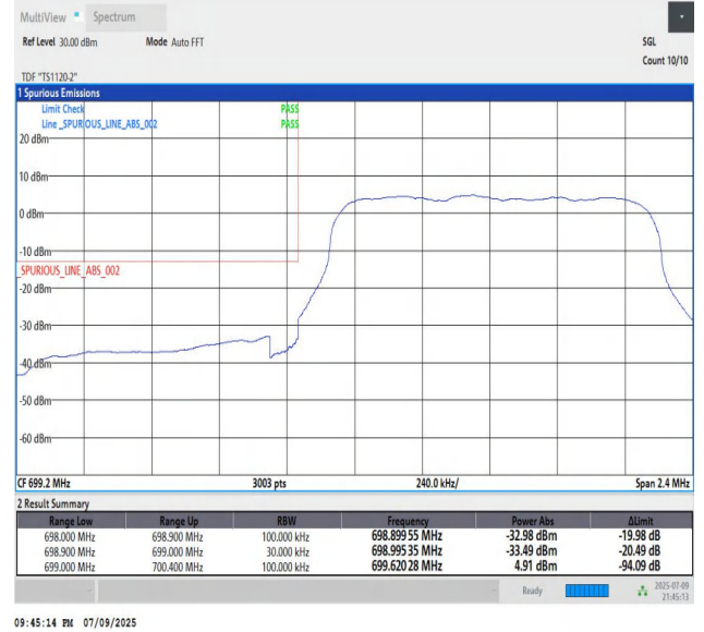
Band12_1.4MHz_QPSK_23017_6_Low
