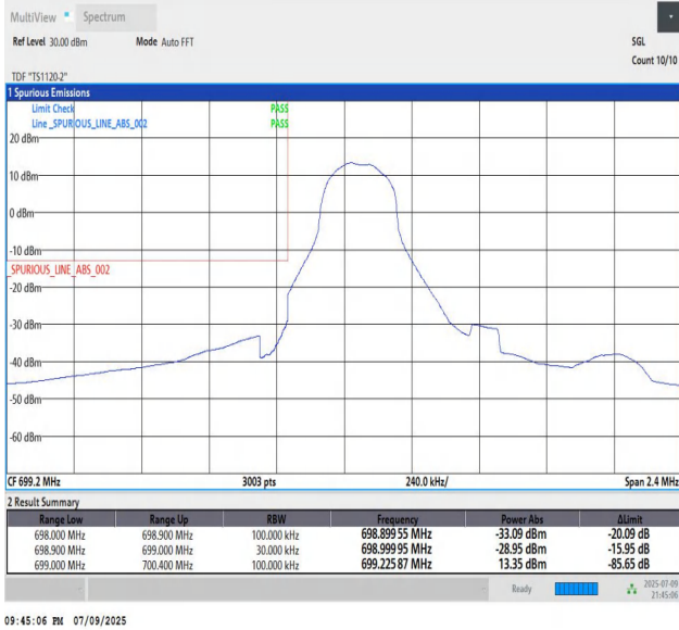
Band12_1.4MHz_QPSK_23017_1_Low
