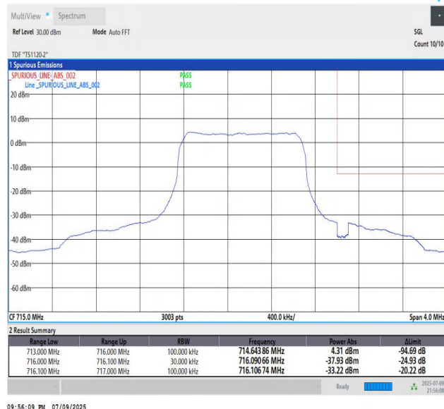
Band12_3MHz_QPSK_23165_6_High
