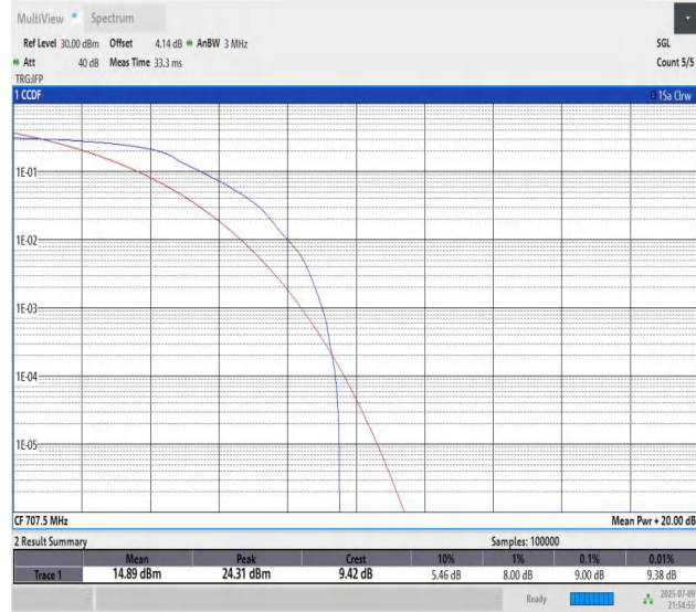
Band12-3MHz-QPSK-23095-PASS
