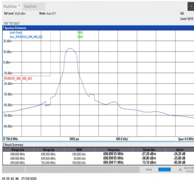
Band12_3MHz_QPSK_23025_1_Low
