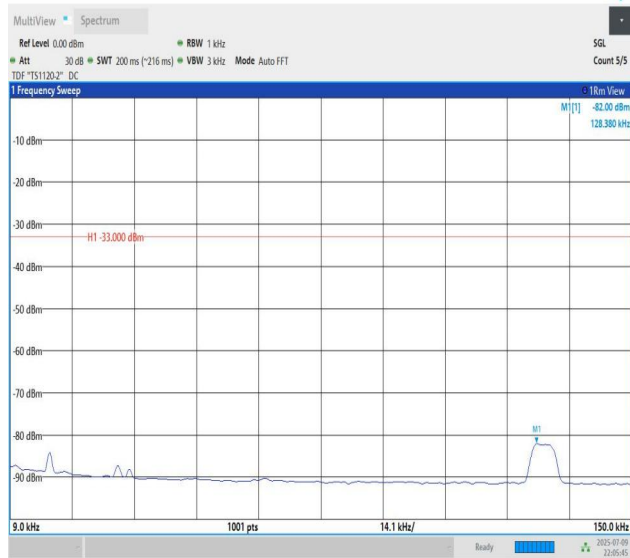
Band12-5MHz-QPSK-23155-PASS
