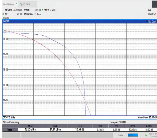
Band12-3MHz-16QAM-23095-PASS
