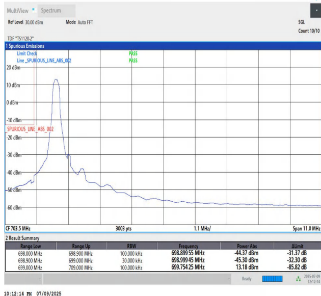
Band12_10MHz_QPSK_23060_1_Low
