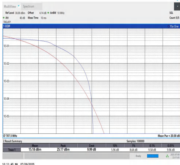
Band12-10MHz-16QAM-23095-PASS
