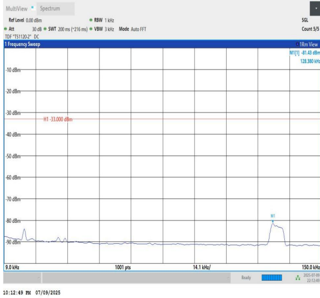
Band12-10MHz-QPSK-23060-PASS
