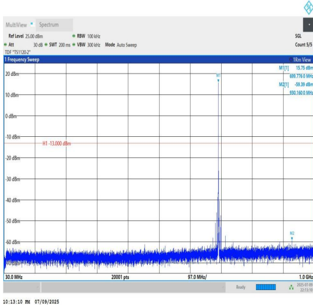
Band12-10MHz-QPSK-23060-PASS
