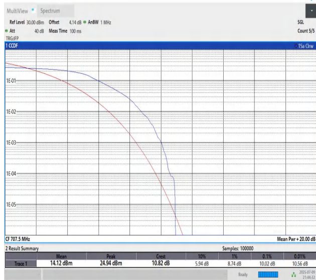
Band12-1.4MHz-16QAM-23095-PASS
