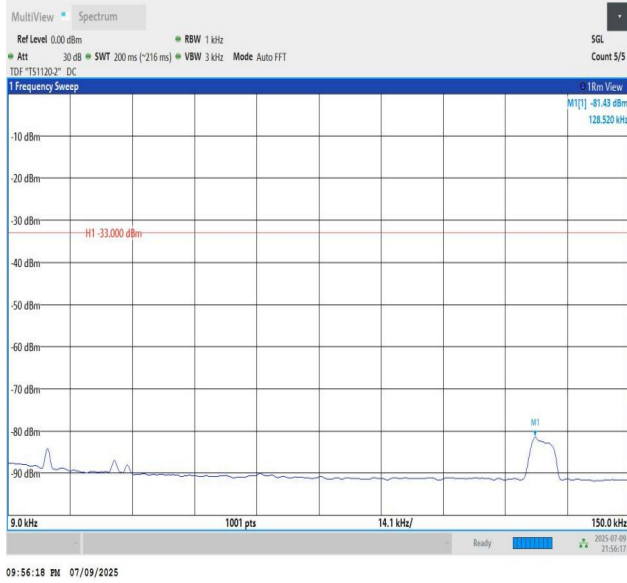
Band12-3MHz-QPSK-23025-PASS
