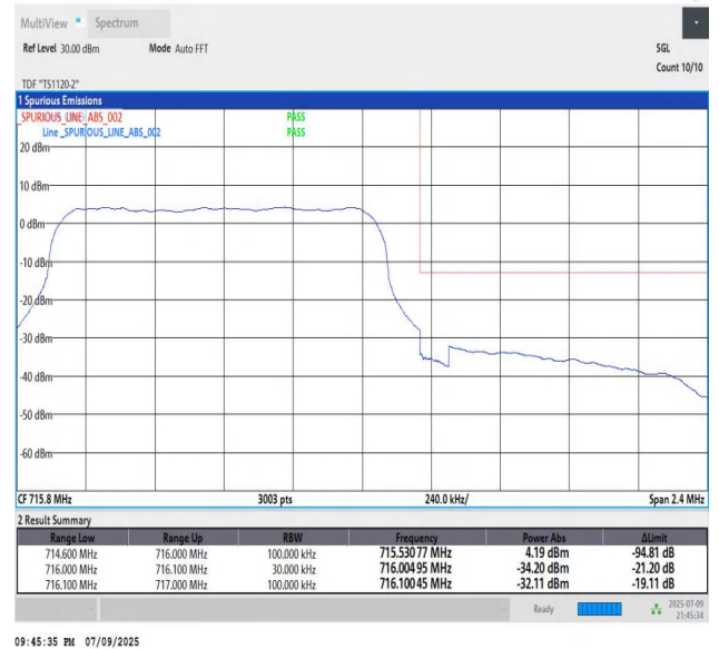
Band12_1.4MHz_QPSK_23173_6_High
