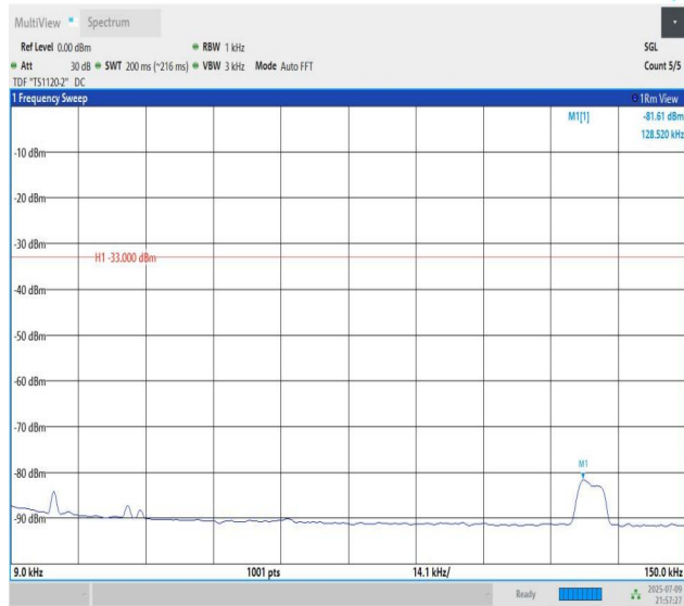
Band12-3MHz-QPSK-23165-PASS
