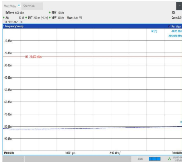
Band12-3MHz-QPSK-23165-PASS
