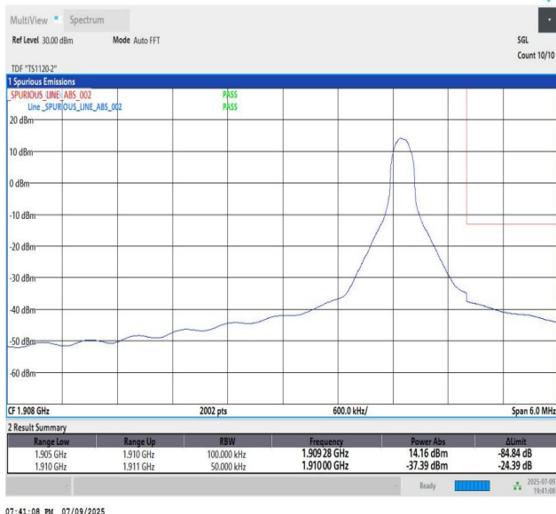
Band2_5MHz_QPSK_19175_1_High
