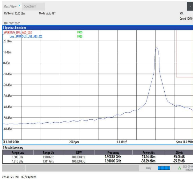
Band2_10MHz_QPSK_19150_1_High
