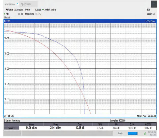
Band2-3MHz-QPSK-18900-PASS
