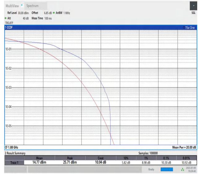
Band2-1.4MHz-QPSK-18900-PASS
