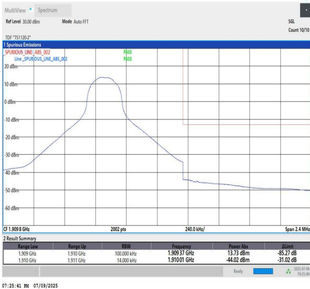
Band2_1.4MHz_QPSK_19193_1_High
