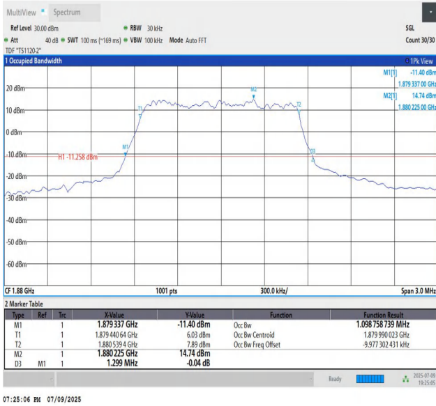
Band2-1.4MHz-16QAM-18900-PASS
