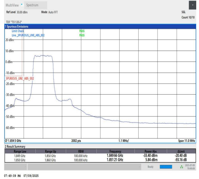
Band2_10MHz_QPSK_18650_6_Low
