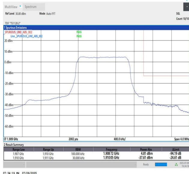
Band2_3MHz_QPSK_19185_6_High
