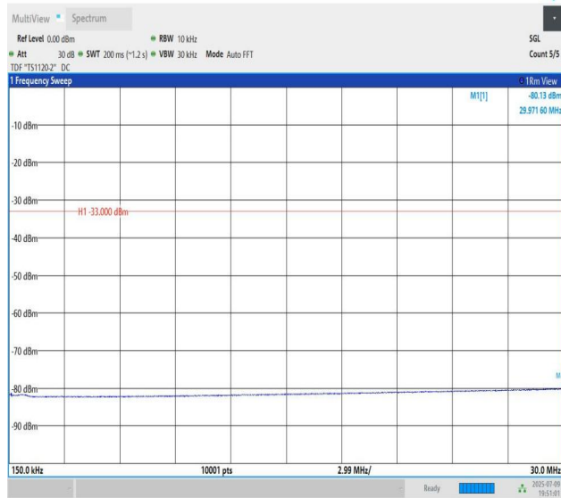
Band2-10MHz-QPSK-19150-PASS
