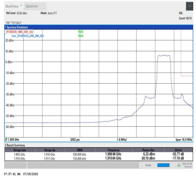
Band2_15MHz_QPSK_19125_6_High
