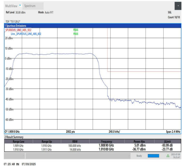
Band2_1.4MHz_QPSK_19193_6_High
