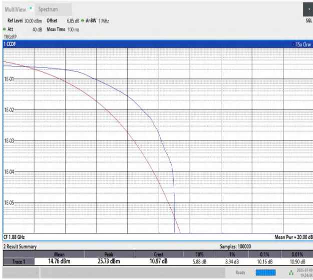
Band2-1.4MHz-16QAM-18900-PASS
