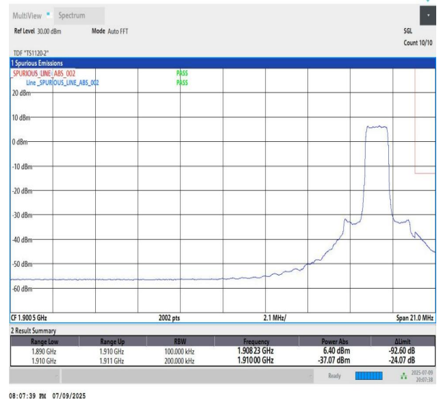
Band2_20MHz_QPSK_19100_6_High
