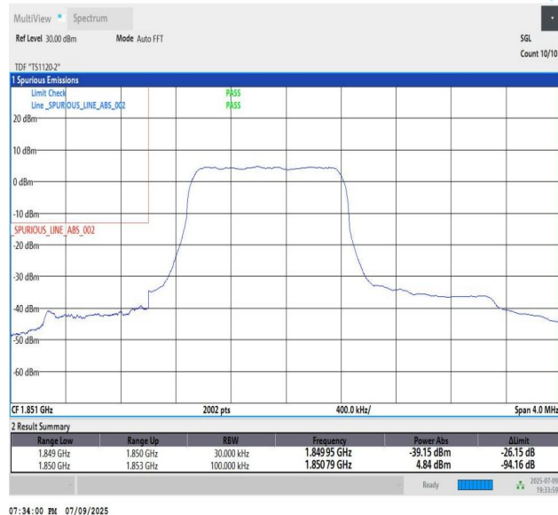
Band2_3MHz_QPSK_18615_6_Low
