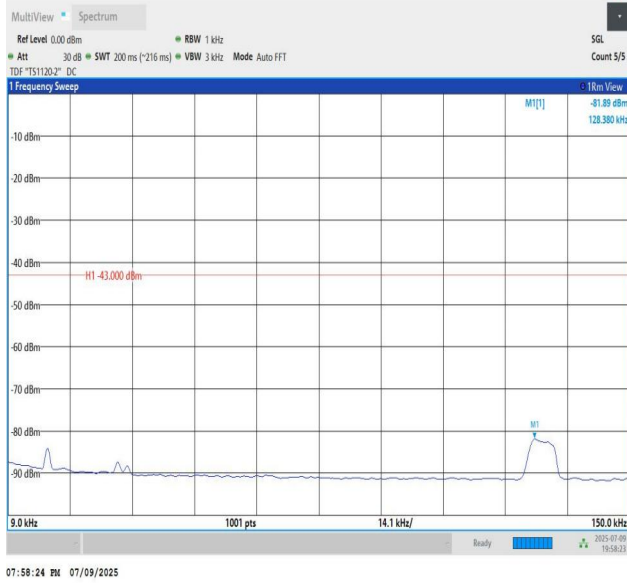
Band2-15MHz-QPSK-18900-PASS
