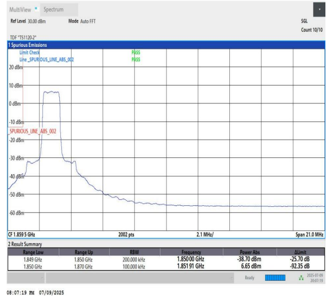
Band2_20MHz_QPSK_18700_6_Low
