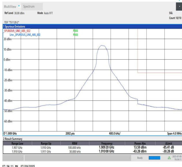
Band2_3MHz_QPSK_19185_1_High
