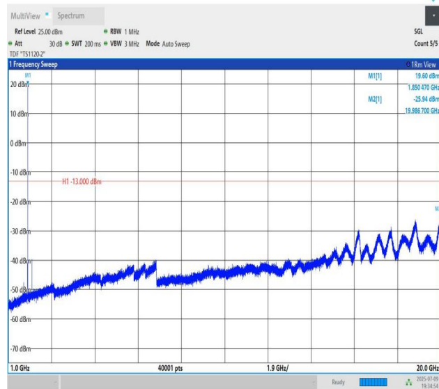
Band2-3MHz-QPSK-18615-PASS
