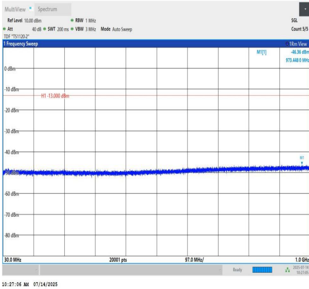
Band2-3MHz-QPSK-19185-PASS
