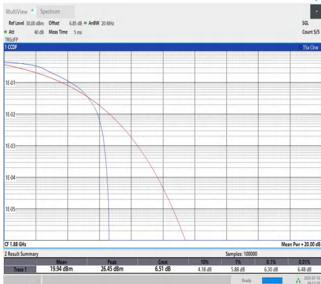
Band2-20MHz-16QAM-18900-PASS
