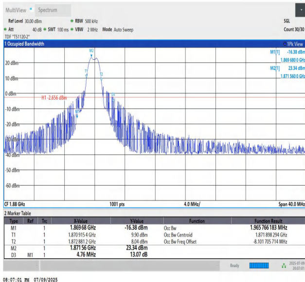
Band2-20MHz-16QAM-18900-PASS
