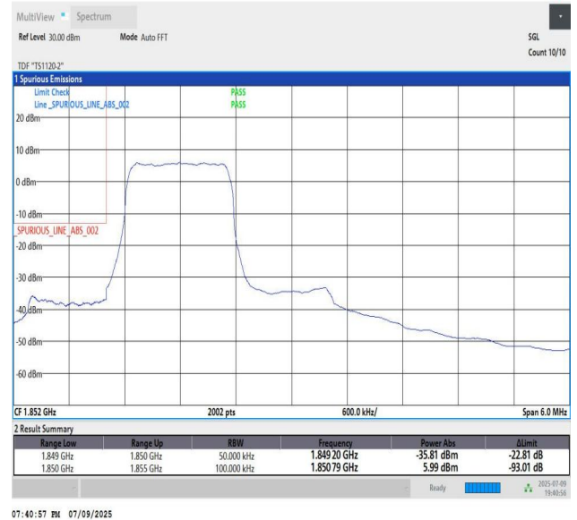
Band2_5MHz_QPSK_18625_6_Low
