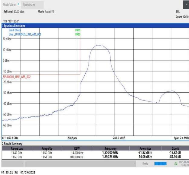
Band2_1.4MHz_QPSK_18607_1_Low
