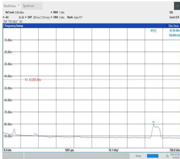
Band2-10MHz-QPSK-19150-PASS
