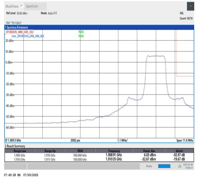
Band2_10MHz_QPSK_19150_6_High
