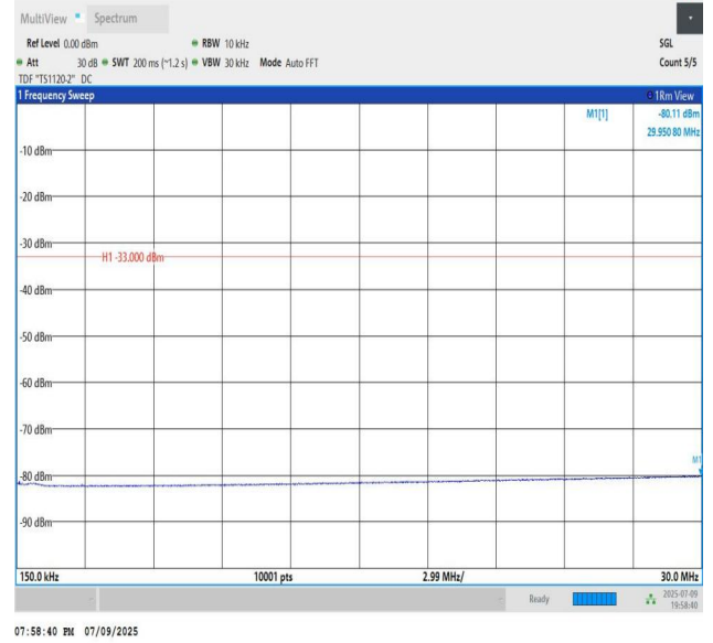
Band2-15MHz-QPSK-18900-PASS
