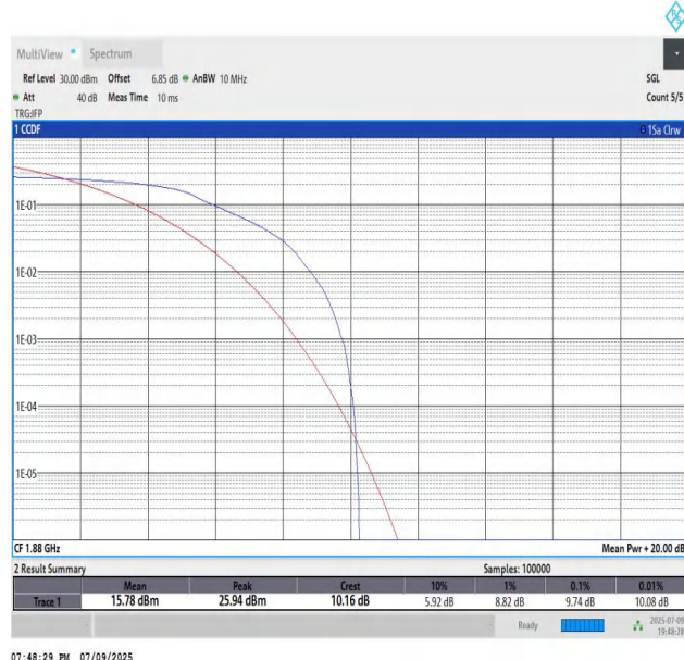
Band2-10MHz-QPSK-18900-PASS
