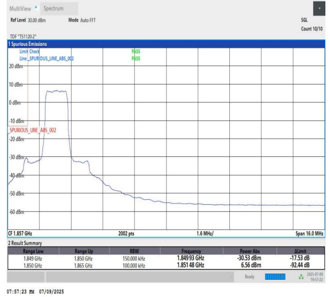
Band2_15MHz_QPSK_18675_6_Low
