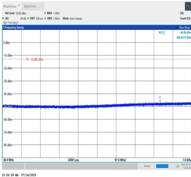
Band2-1.4MHz-QPSK-18607-PASS
