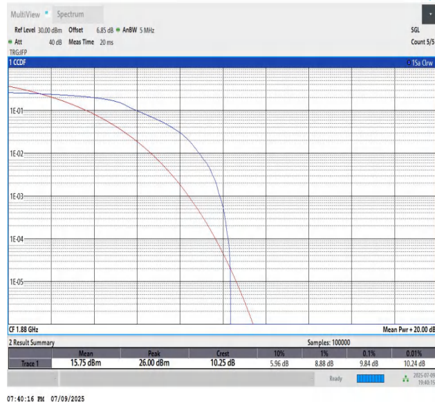
Band2-5MHz-QPSK-18900-PASS
