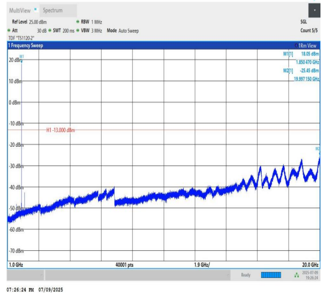
Band2-1.4MHz-QPSK-18607-PASS
