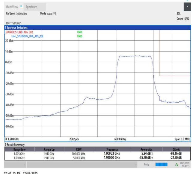
Band2_5MHz_QPSK_19175_6_High
