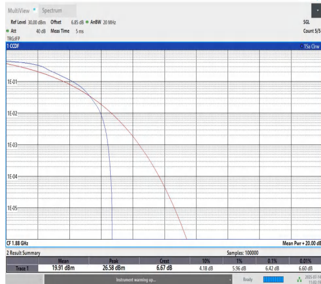
Band2-15MHz-QPSK-18900-PASS
