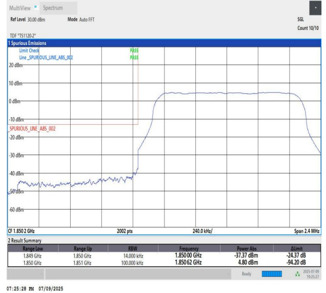
Band2_1.4MHz_QPSK_18607_6_Low
