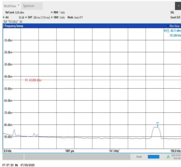
Band2-15MHz-QPSK-18675-PASS
