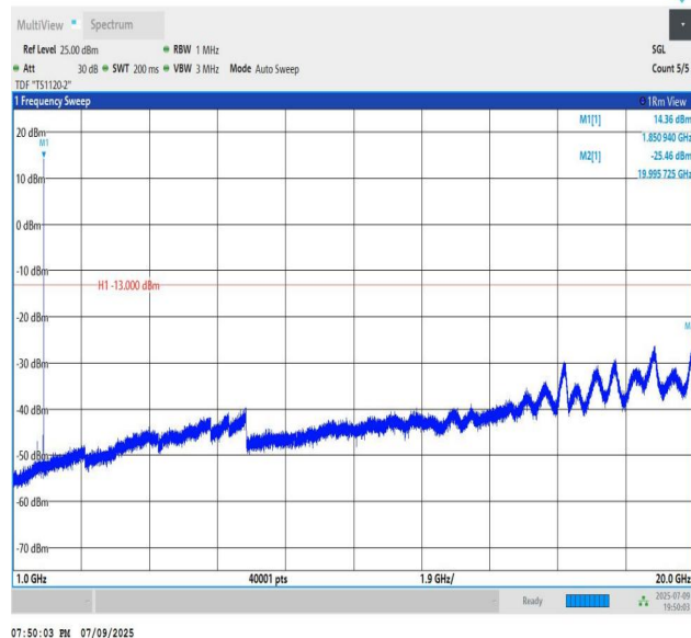
Band2-10MHz-QPSK-18650-PASS
