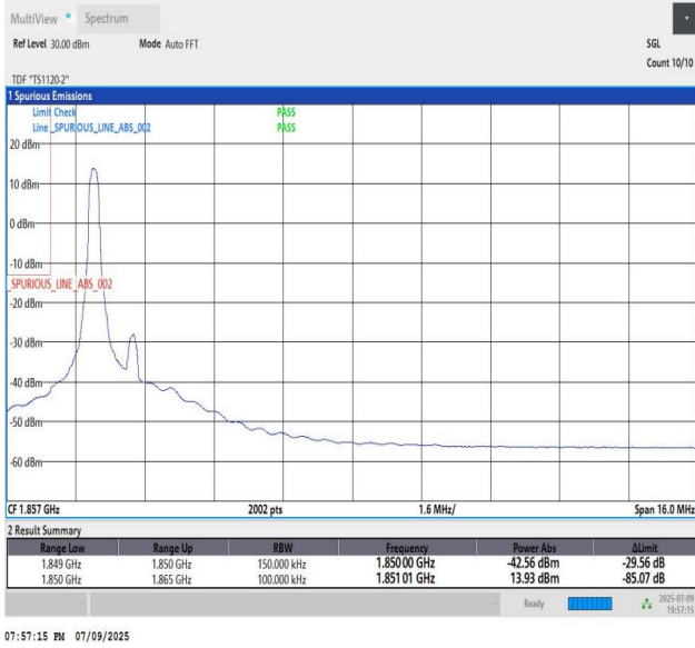
Band2_15MHz_QPSK_18675_1_Low
