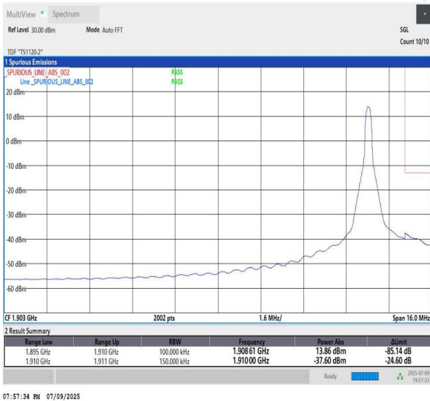
Band2_15MHz_QPSK_19125_1_High
