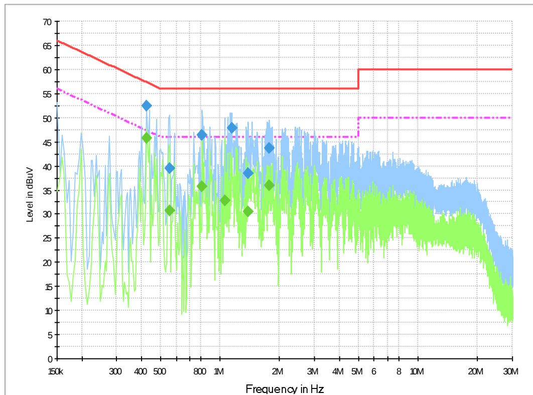
Fig.A.6.2. AC Powerline Conducted Emission-Idle
