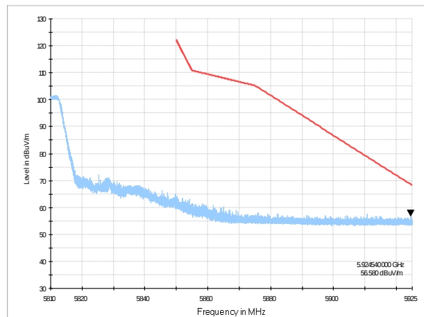
Fig. 5 Band Edges (802.11n-HT40 Ch151, 5755MHz)
