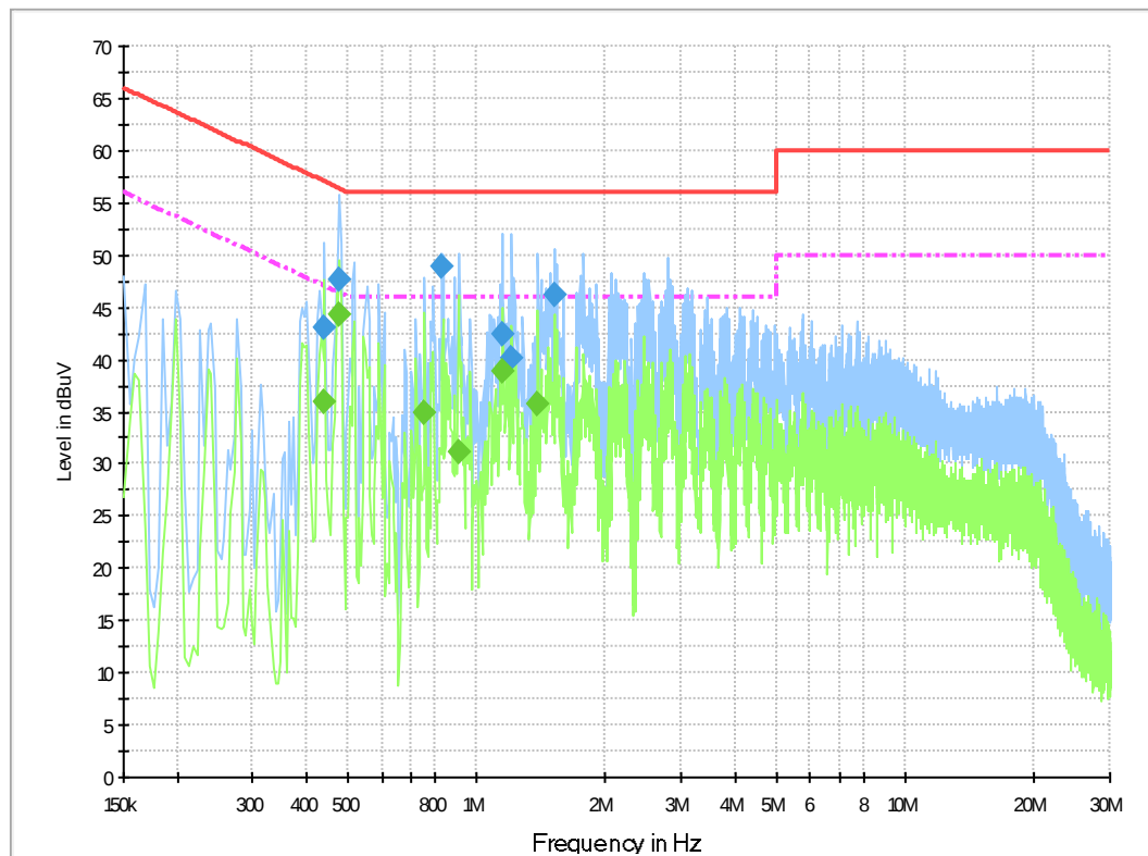
Fig.A.6.1. AC Powerline Conducted Emission-802.11a CH149
