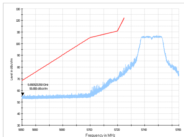
Fig. 1 Band Edges (802.11a Ch149,5745MHz)
