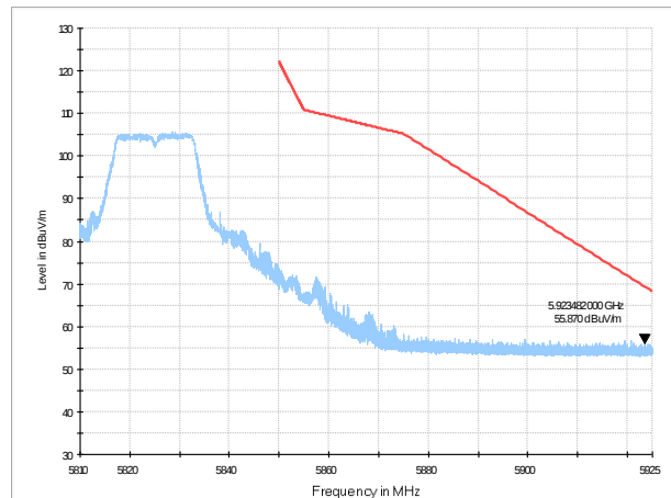
Fig. 2 Band Edges (802.11a Ch165, 5825MHz)
