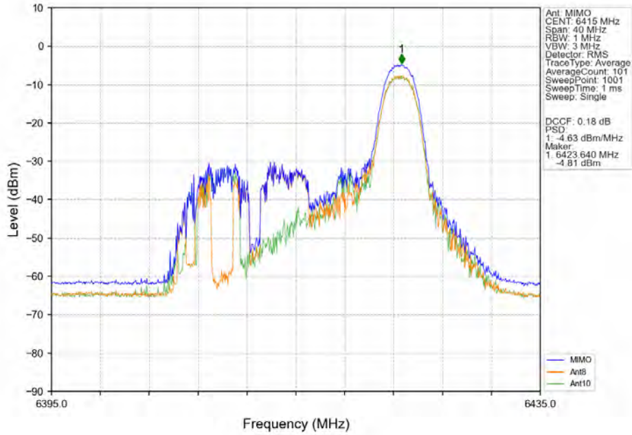
802.11ax(HEW20) HCH 6415MHz RU52 Right Ant8 NTN
