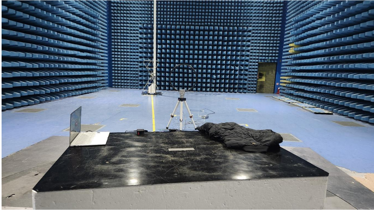
Radiated Spurious Emissions(30 MHz to 1 GHz)
