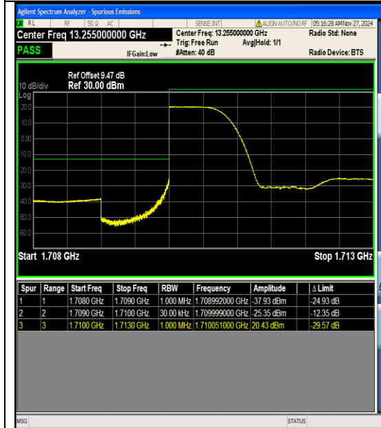
Band4_3MHz_16QAM_19965_1RB#0
