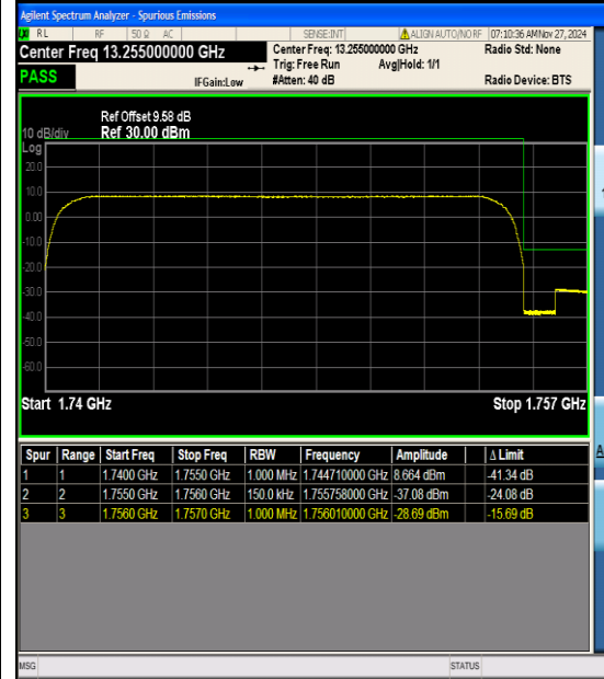
Band4_15MHz_QPSK_20325_75RB#0
