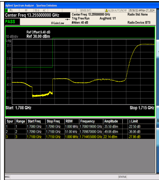
Band4_5MHz_QPSK_19975_1RB#24
