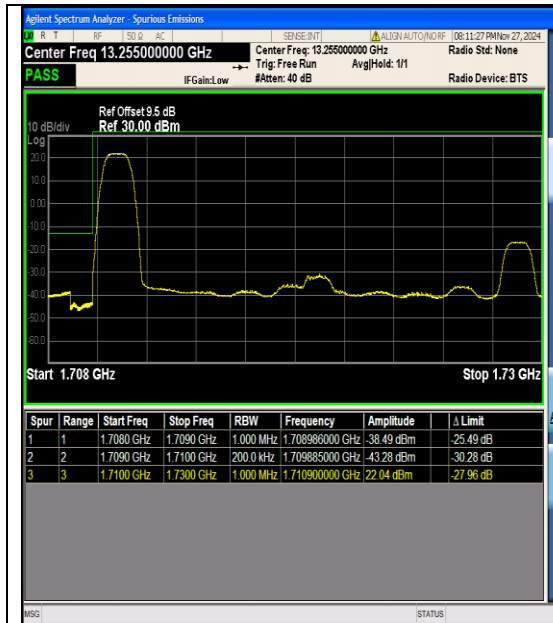
Band4_20MHz_QPSK_20050_1RB#0
