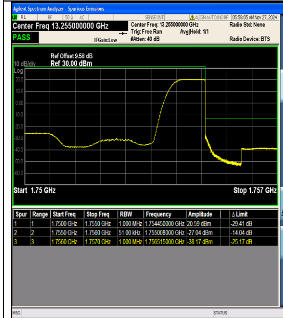
Band4_5MHz_16QAM_20375_1RB#24
