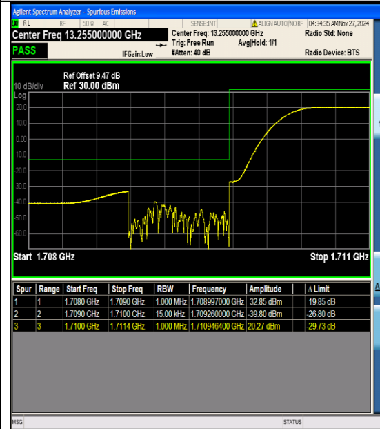
Band4_1.4MHz_16QAM_19957_1RB#5
