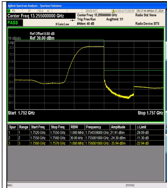
Band4_3MHz_QPSK_20385_1RB#14
