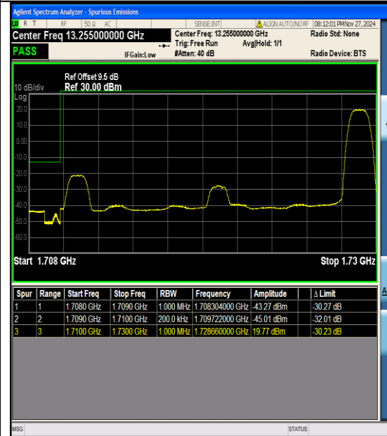
Band4_20MHz_16QAM_20050_1RB#99
