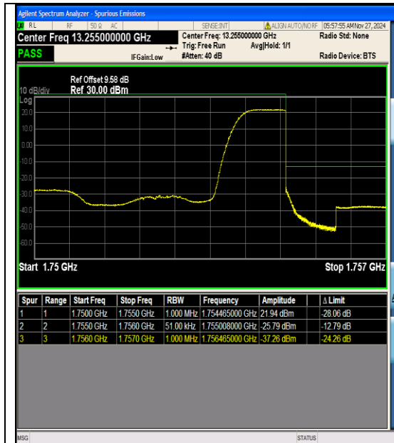
Band4_5MHz_QPSK_20375_1RB#24
