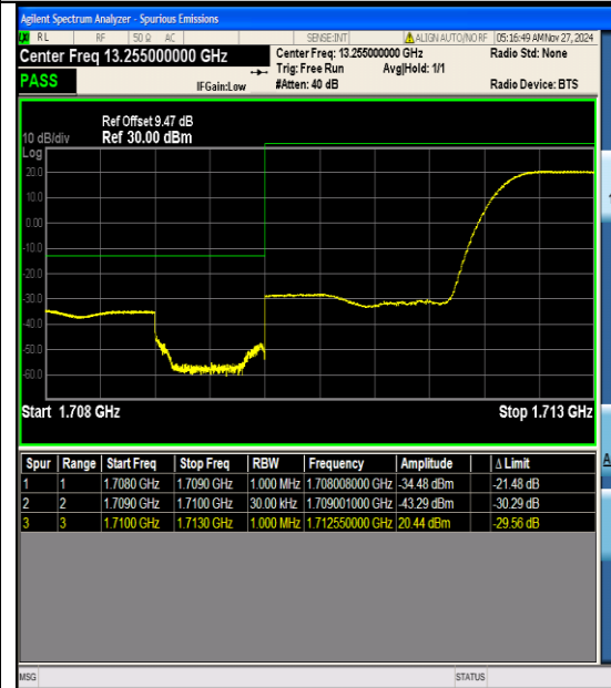
Band4_3MHz_16QAM_19965_1RB#14
