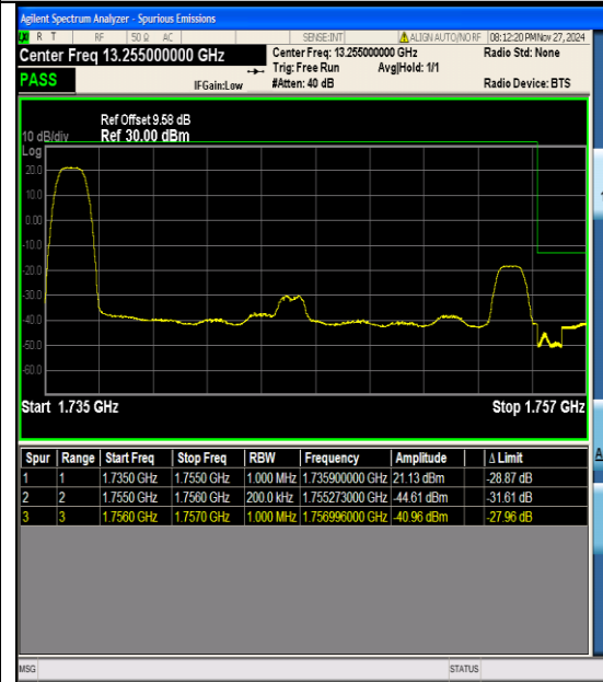
Band4_20MHz_QPSK_20300_1RB#0
