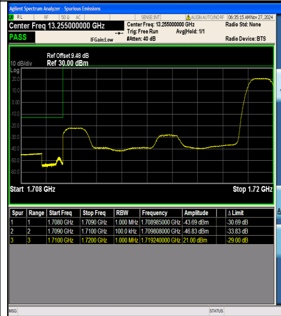
Band4_10MHz_16QAM_20000_1RB#49
