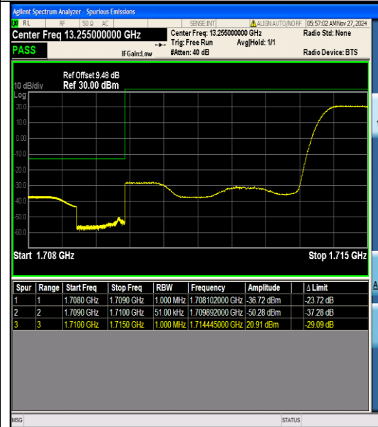
Band4_5MHz_16QAM_19975_1RB#24
