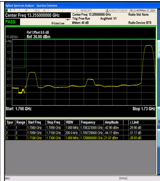
Band4_20MHz_QPSK_20050_1RB#99
