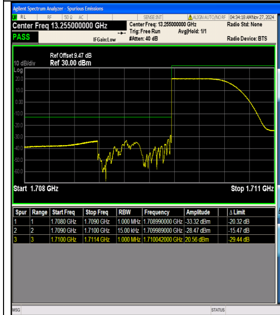
Band4_1.4MHz_16QAM_19957_1RB#0
