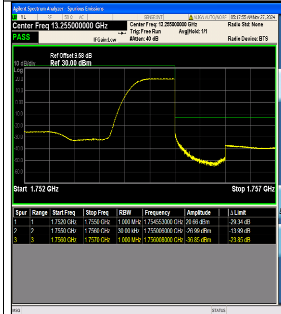
Band4_3MHz_16QAM_20385_1RB#14
