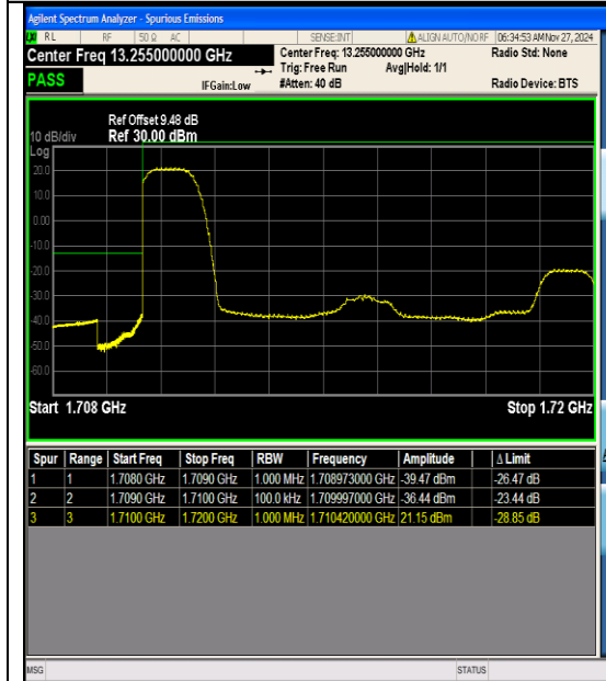
Band4_10MHz_16QAM_20000_1RB#0
