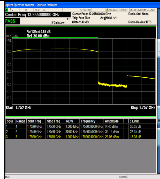
Band4_3MHz_16QAM_20385_15RB#0
