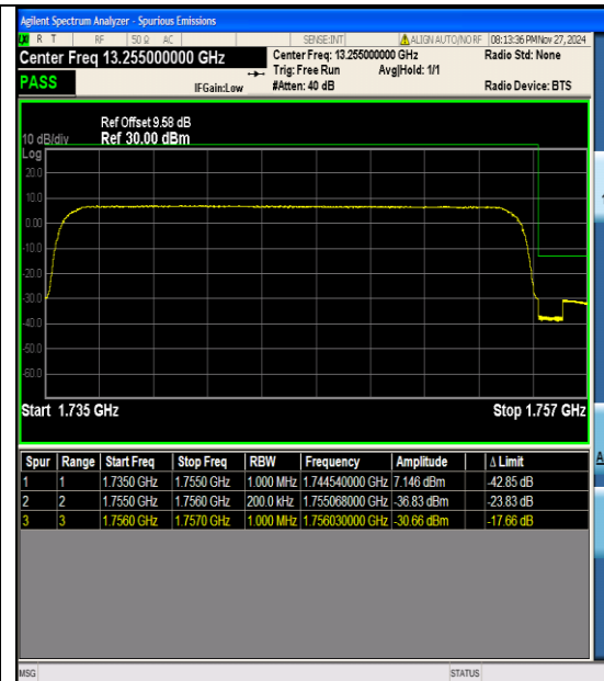
Band4_20MHz_QPSK_20300_100RB#0
