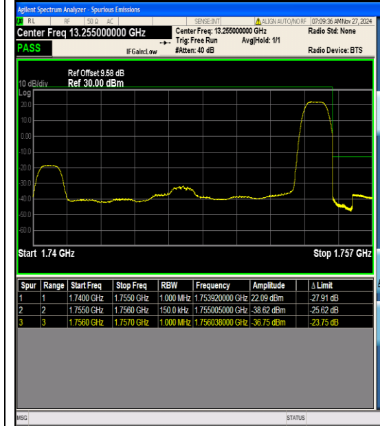
Band4_15MHz_QPSK_20325_1RB#74
