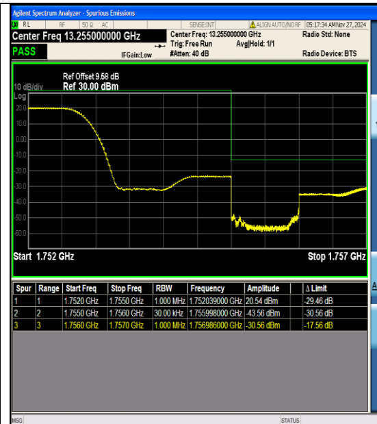
Band4_3MHz_16QAM_20385_1RB#0
