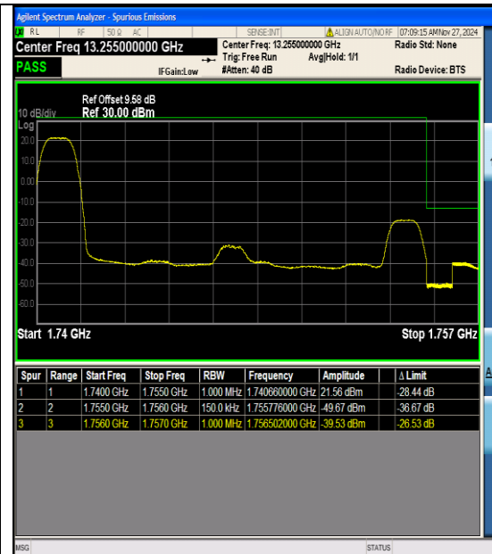
Band4_15MHz_QPSK_20325_1RB#0
