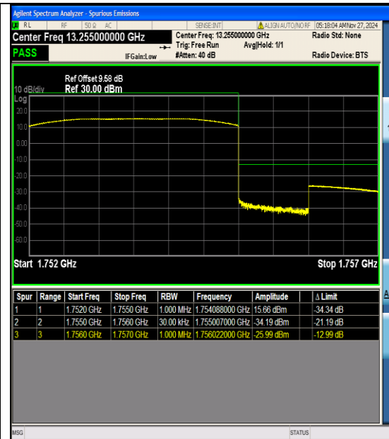
Band4_3MHz_QPSK_20385_15RB#0
