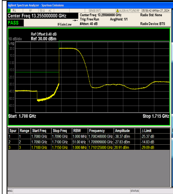
Band4_5MHz_16QAM_19975_1RB#0
