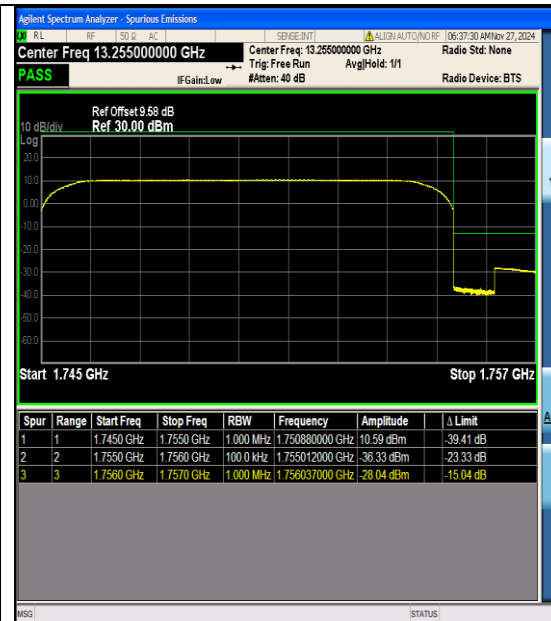
Band4_10MHz_QPSK_20350_50RB#0
