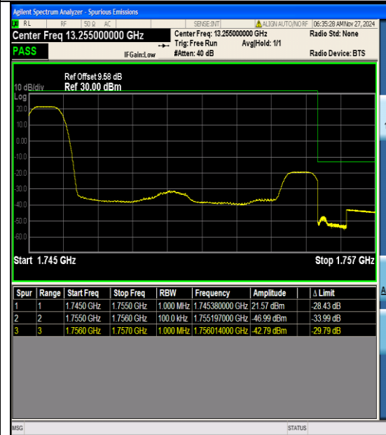
Band4_10MHz_QPSK_20350_1RB#0
