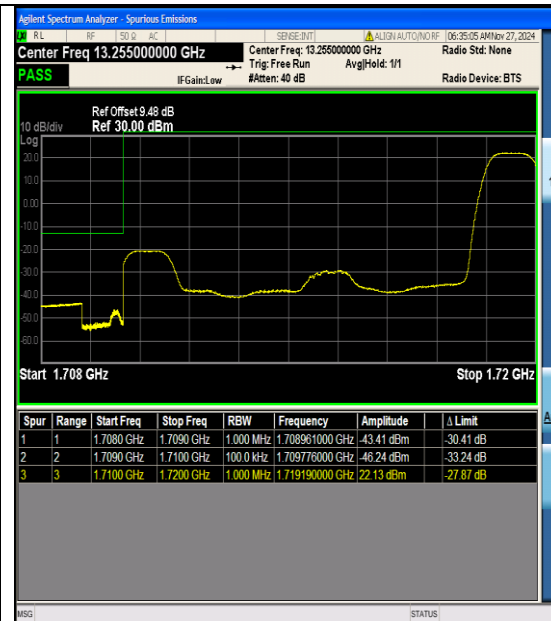
Band4_10MHz_QPSK_20000_1RB#49
