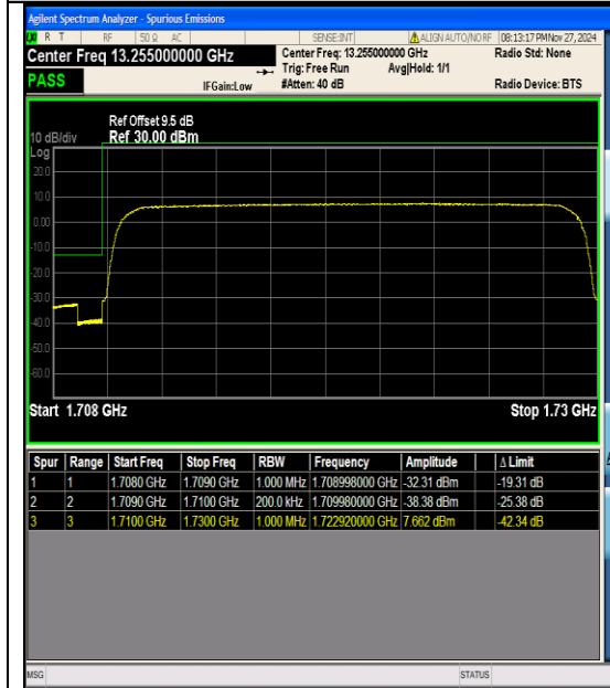
Band4_20MHz_QPSK_20050_100RB#0
