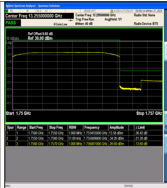
Band4_5MHz_QPSK_20375_25RB#0
