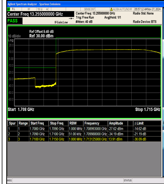
Band4_5MHz_QPSK_19975_25RB#0
