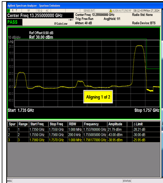
Band4_20MHz_QPSK_20300_1RB#99
