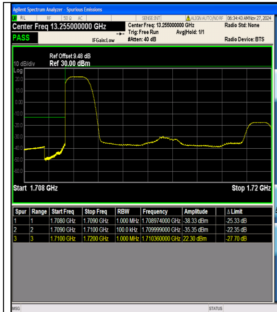
Band4_10MHz_QPSK_20000_1RB#0
