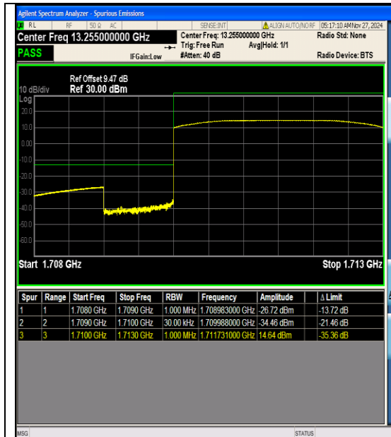
Band4_3MHz_16QAM_19965_15RB#0
