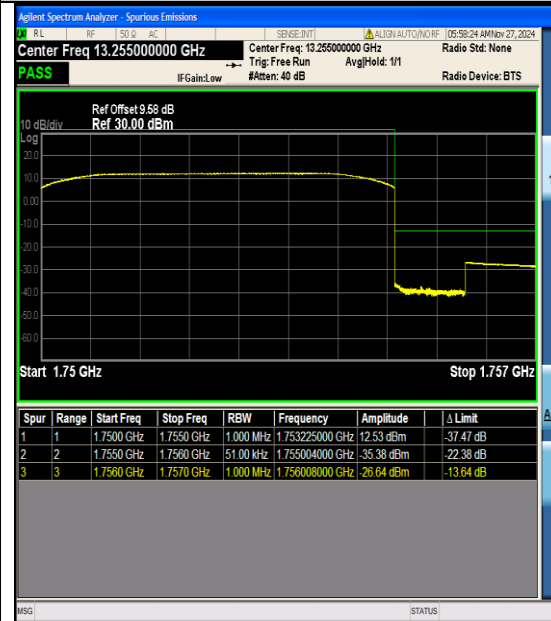
Band4_5MHz_16QAM_20375_25RB#0
