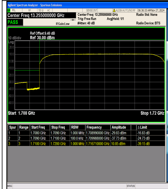
Band4_10MHz_QPSK_20000_50RB#0
