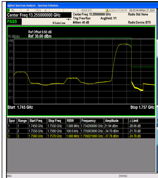
Band4_10MHz_QPSK_20350_1RB#49
