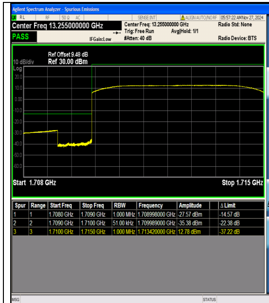
Band4_5MHz_16QAM_19975_25RB#0
