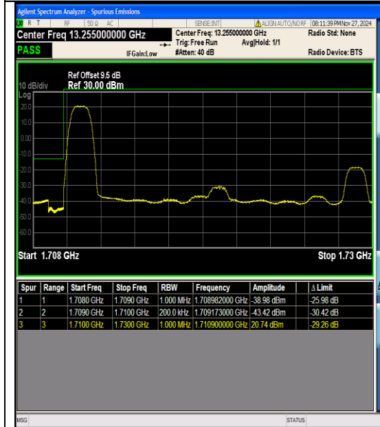
Band4_20MHz_16QAM_20050_1RB#0
