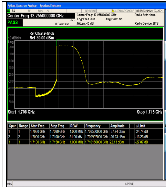
Band4_5MHz_QPSK_19975_1RB#0
