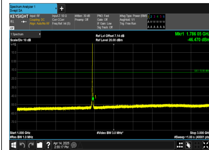
Band66-3MHz-QPSK-132657-1RB#14-1000~3000-PASS
