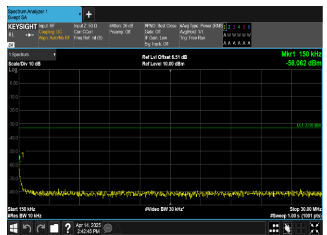
Band66-3MHz-16QAM-131987-1RB#14-0.15~30-PASS
