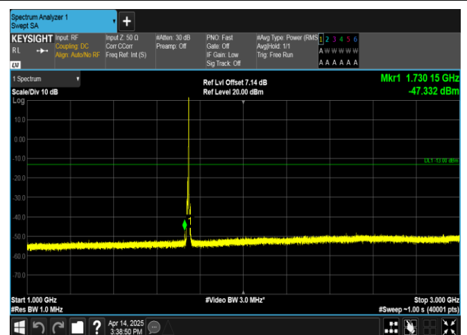
Band66-5MHz-QPSK-132322-1RB#24-1000~3000-PASS
