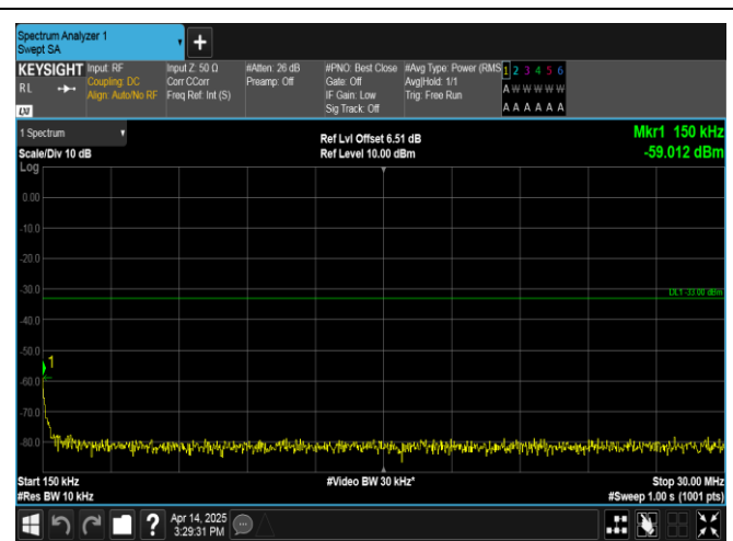
Band66-5MHz-QPSK-131997-1RB#0-0.15~30-PASS
