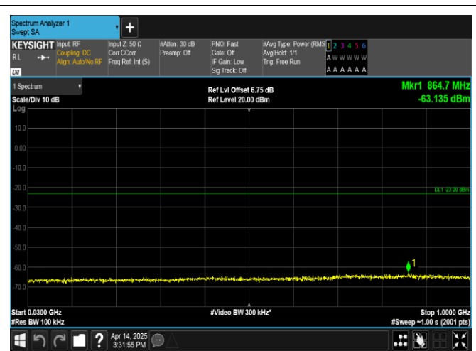
Band66-5MHz-QPSK-131997-1RB#24-30~1000-PASS
