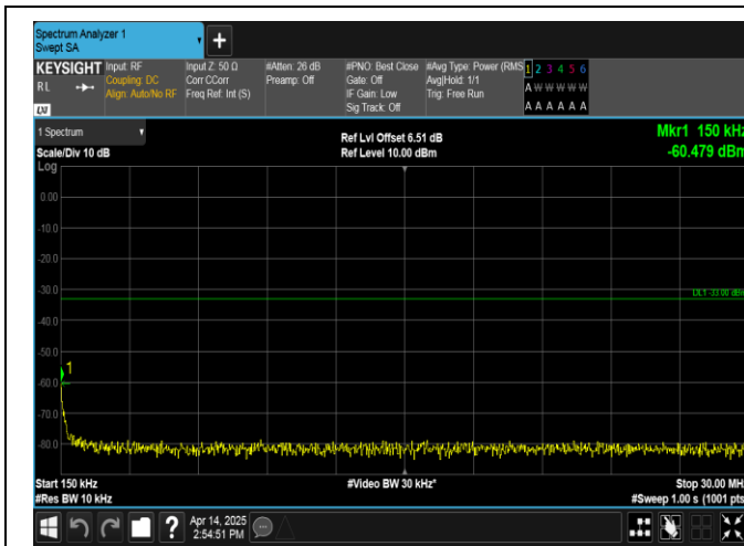
Band66-3MHz-QPSK-132657-1RB#14-0.15~30-PASS
