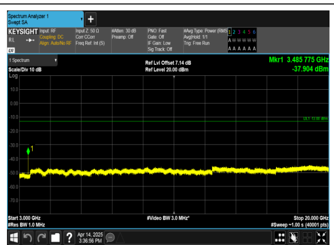
Band66-5MHz-QPSK-132322-1RB#0-3000~20000-PASS
