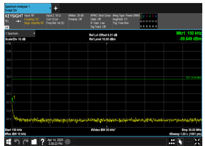
Band66-5MHz-QPSK-132322-1RB#24-0.15~30-PASS
