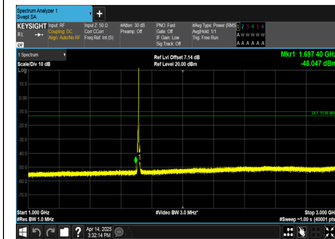
Band66-5MHz-QPSK-131997-1RB#24-1000~3000-PASS
