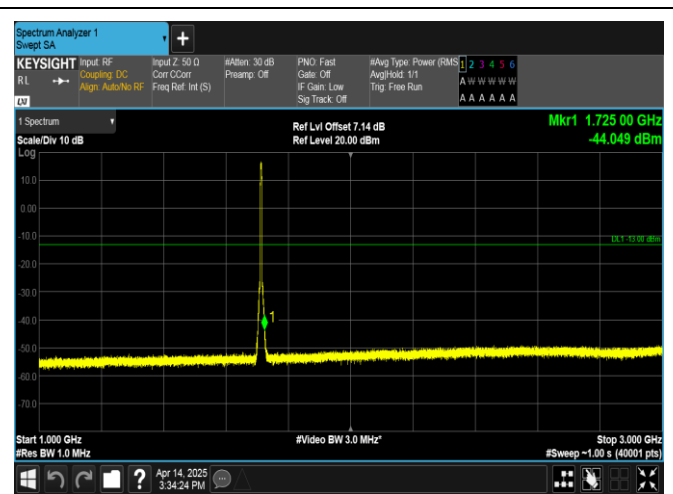
Band66-5MHz-QPSK-131997-25RB#0-1000~3000-PASS
