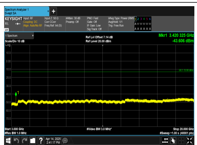
Band66-3MHz-16QAM-131987-1RB#0-3000~20000-PASS
