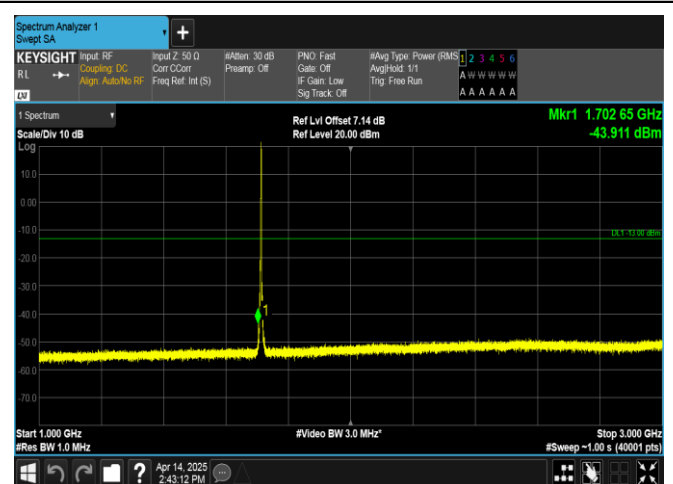
Band66-3MHz-16QAM-131987-1RB#14-1000~3000-PASS
