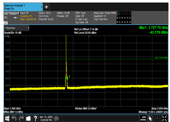
Band66-5MHz-QPSK-131997-1RB#0-1000~3000-PASS
