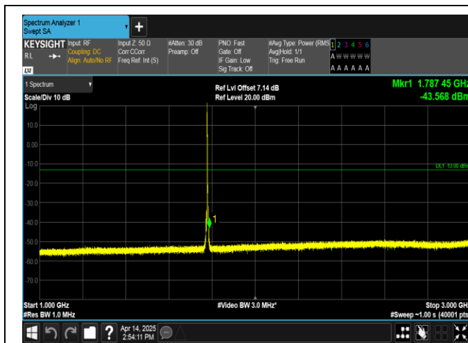
Band66-3MHz-16QAM-132657-1RB#0-1000~3000-PASS
