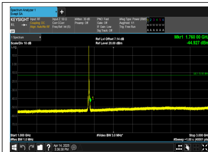
Band66-5MHz-QPSK-132322-1RB#0-1000~3000-PASS
