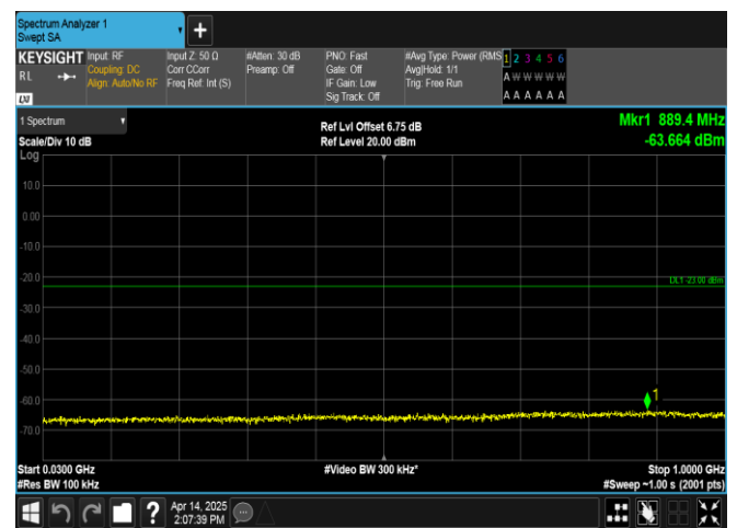
Band66-1.4MHz-16QAM-132665-6RB#0-30~1000-PASS
