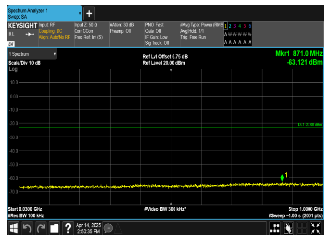
Band66-3MHz-QPSK-132322-15RB#0-30~1000-PASS
