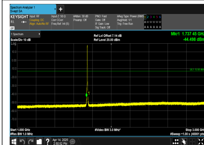
Band66-3MHz-QPSK-132322-15RB#0-1000~3000-PASS
