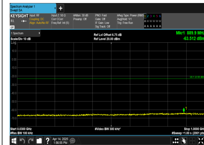
Band66-1.4MHz-16QAM-132322-1RB#0-30~1000-PASS
