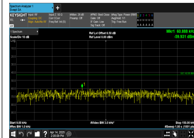
Band66-1.4MHz-16QAM-132665-1RB#5-0.009~0.15-PASS
