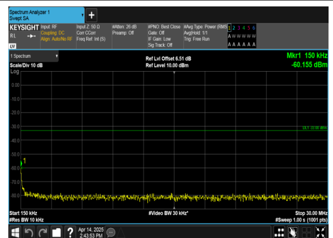
Band66-3MHz-QPSK-131987-15RB#0-0.15~30-PASS
