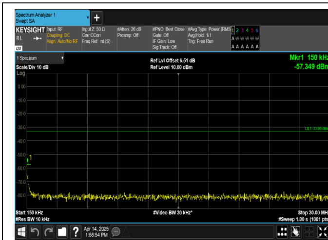
Band66-1.4MHz-16QAM-132322-1RB#5-0.15~30-PASS
