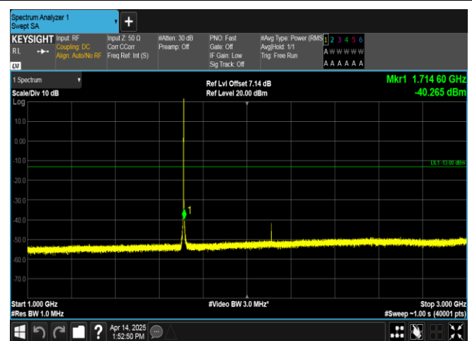
Band66-1.4MHz-16QAM-131979-1RB#5-1000~3000-PASS
