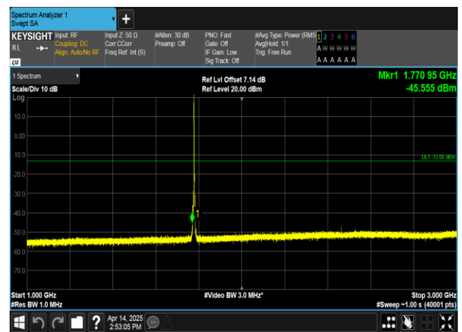
Band66-3MHz-QPSK-132657-1RB#0-1000~3000-PASS
