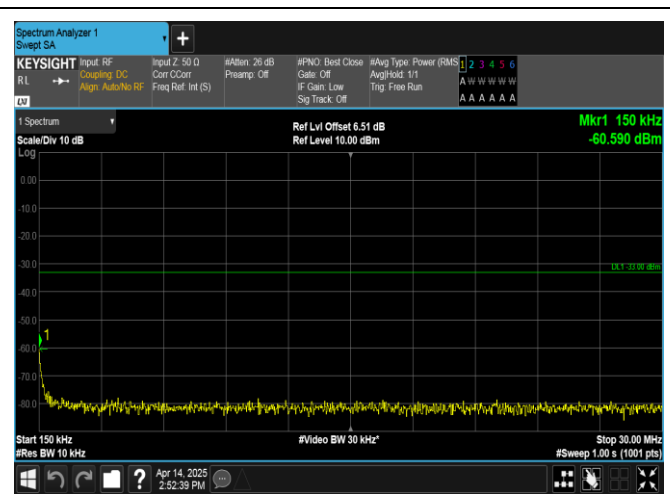
Band66-3MHz-QPSK-132657-1RB#0-0.15~30-PASS
