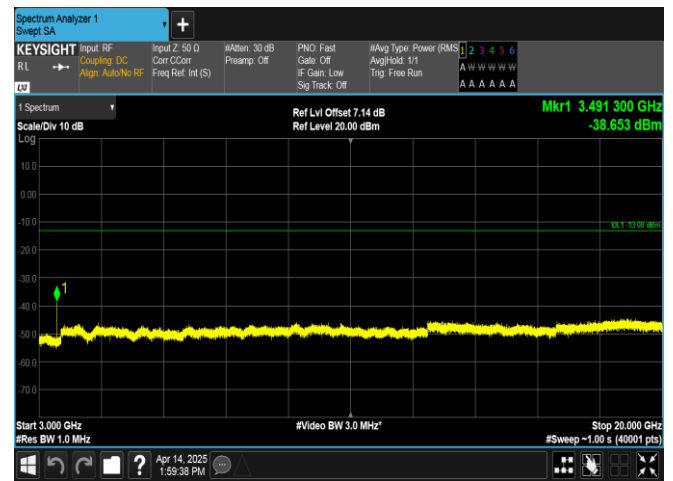
Band66-1.4MHz-16QAM-132322-1RB#5-3000~20000-PASS
