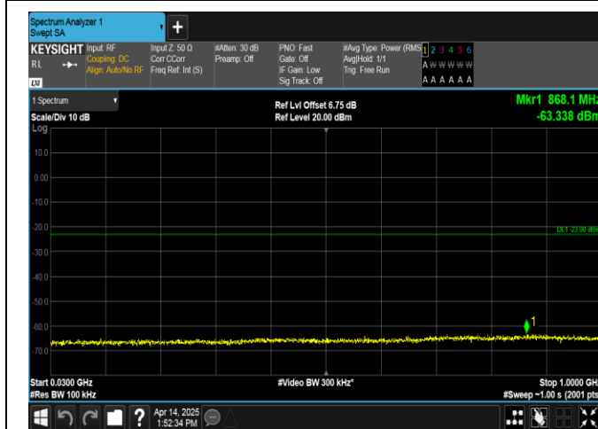
Band66-1.4MHz-16QAM-131979-1RB#5-30~1000-PASS
