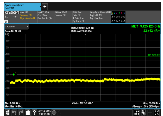
Band66-3MHz-QPSK-131987-1RB#14-3000~20000-PASS
