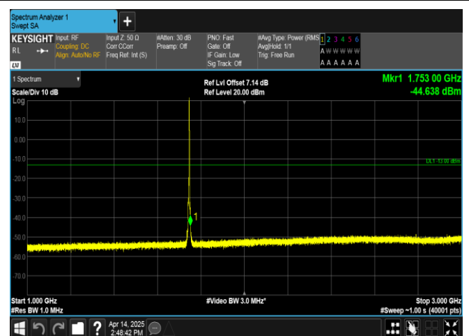
Band66-3MHz-QPSK-132322-1RB#14-1000~3000-PASS
