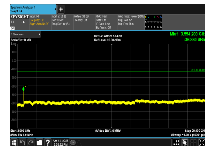
Band66-3MHz-QPSK-132657-1RB#0-3000~20000-PASS
