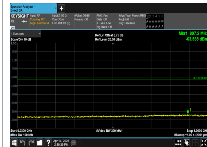
Band66-3MHz-QPSK-131987-1RB#0-30~1000-PASS
