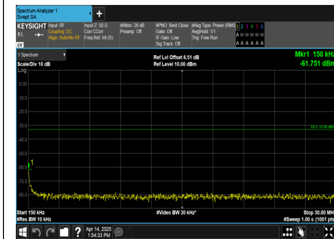
Band66-1.4MHz-16QAM-131979-6RB#0-0.15~30-PASS
