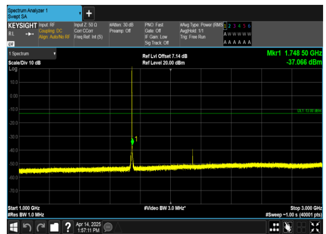
Band66-1.4MHz-16QAM-132322-1RB#0-1000~3000-PASS
