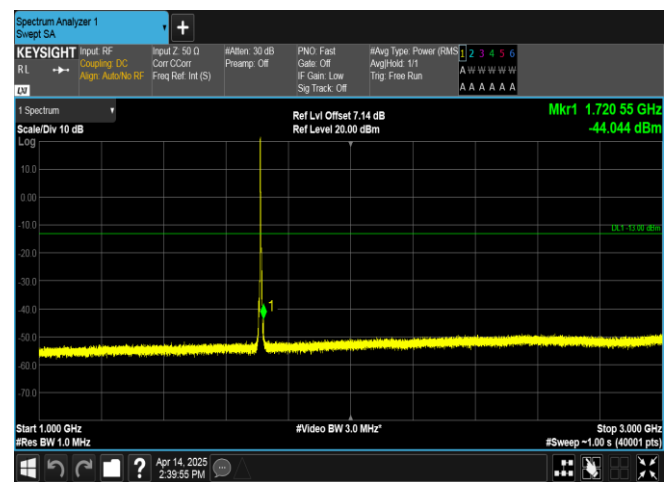
Band66-3MHz-QPSK-131987-1RB#0-1000~3000-PASS
