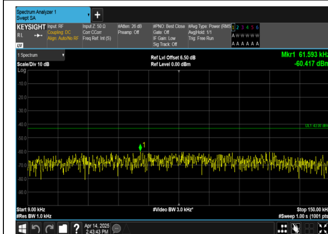
Band66-3MHz-QPSK-131987-15RB#0-0.009~0.15-PASS
