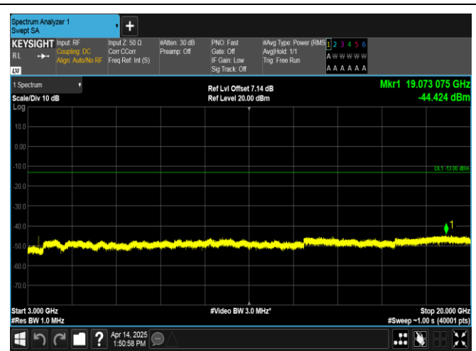
Band66-1.4MHz-16QAM-131979-1RB#0-3000~20000-PASS
