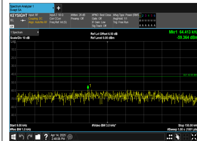
Band66-3MHz-QPSK-132322-1RB#14-0.009~0.15-PASS
