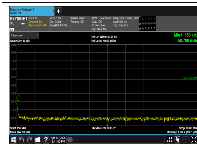
Band66-3MHz-QPSK-131987-1RB#14-0.15~30-PASS
