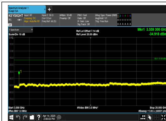
Band66-1.4MHz-16QAM-132665-1RB#5-3000~20000-PASS
