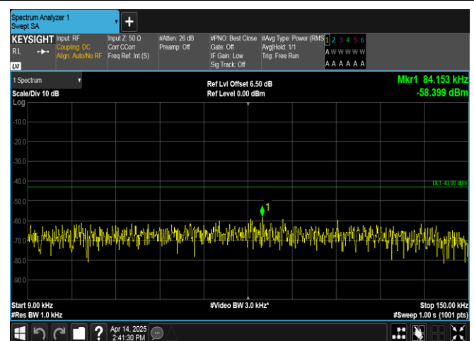
Band66-3MHz-QPSK-131987-1RB#14-0.009~0.15-PASS
