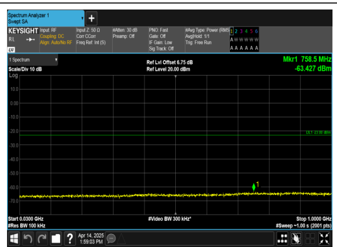
Band66-1.4MHz-16QAM-132322-1RB#5-30~1000-PASS
