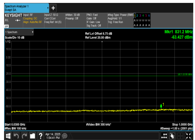
Band66-1.4MHz-16QAM-131979-6RB#0-30~1000-PASS
