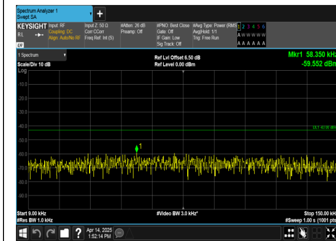
Band66-1.4MHz-16QAM-131979-1RB#5-0.009~0.15-PASS
