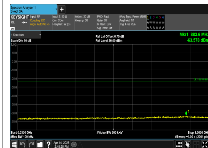
Band66-3MHz-QPSK-132322-1RB#14-30~1000-PASS
