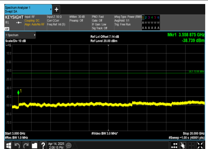
Band66-1.4MHz-16QAM-132665-6RB#0-3000~20000-PASS
