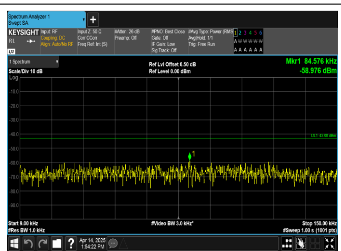
Band66-1.4MHz-16QAM-131979-6RB#0-0.009~0.15-PASS
