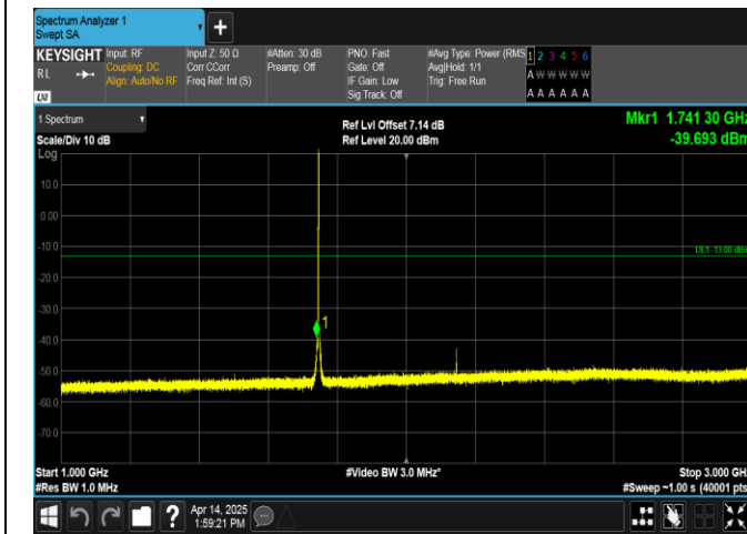
Band66-1.4MHz-16QAM-132322-1RB#5-1000~3000-PASS
