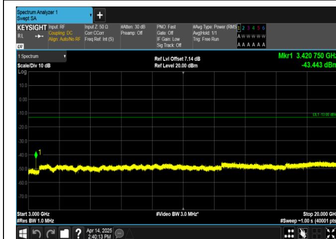
Band66-3MHz-QPSK-131987-1RB#0-3000~20000-PASS
