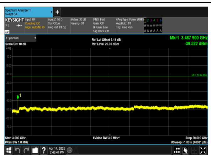
Band66-3MHz-QPSK-132322-1RB#0-3000~20000-PASS
