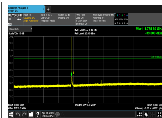
Band66-1.4MHz-16QAM-132665-1RB#0-1000~3000-PASS
