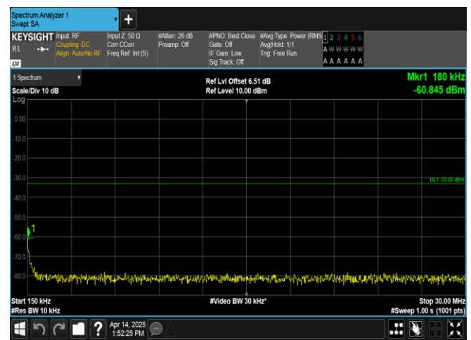
Band66-1.4MHz-16QAM-131979-1RB#5-0.15~30-PASS
