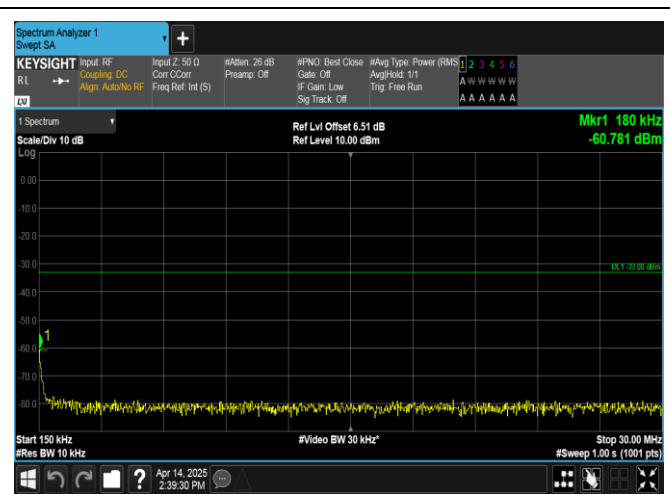
Band66-3MHz-QPSK-131987-1RB#0-0.15~30-PASS
