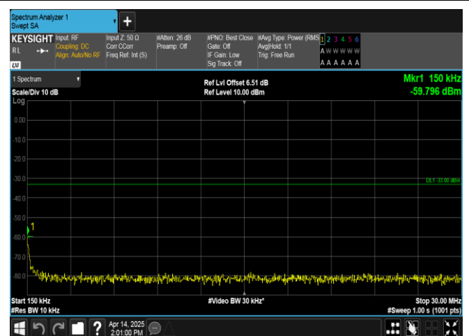
Band66-1.4MHz-16QAM-132322-6RB#0-0.15~30-PASS
