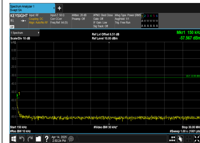
Band66-3MHz-QPSK-132322-15RB#0-0.15~30-PASS
