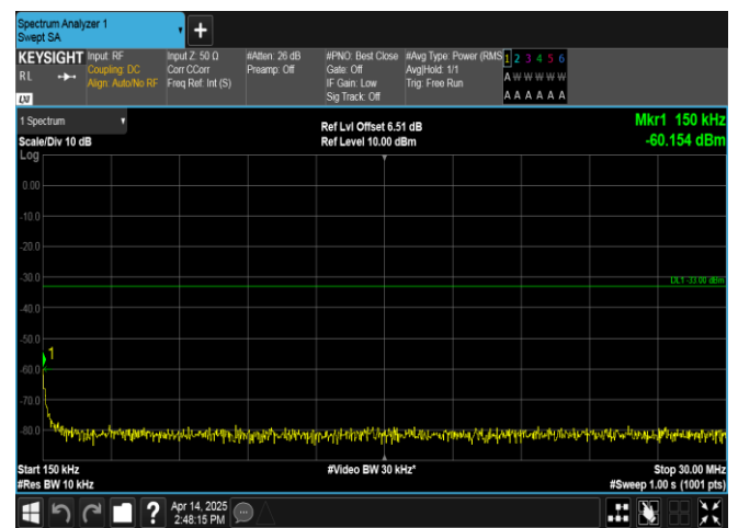
Band66-3MHz-QPSK-132322-1RB#14-0.15~30-PASS
