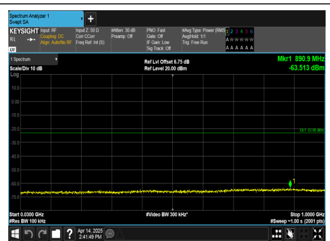
Band66-3MHz-QPSK-131987-1RB#14-30~1000-PASS
