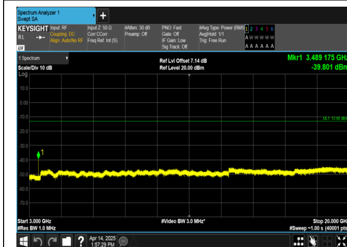
Band66-1.4MHz-16QAM-132322-1RB#0-3000~20000-PASS
