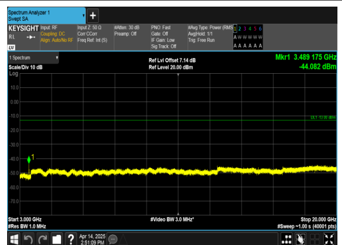
Band66-3MHz-QPSK-132322-15RB#0-3000~20000-PASS
