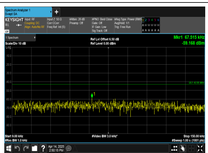
Band66-3MHz-QPSK-132322-15RB#0-0.009~0.15-PASS
