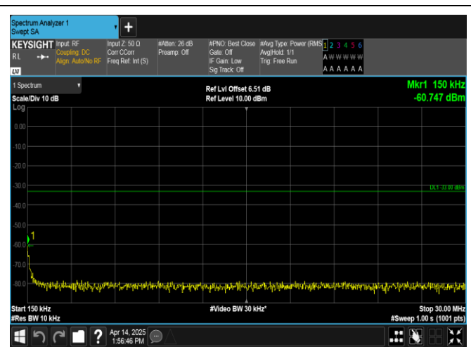
Band66-1.4MHz-16QAM-132322-1RB#0-0.15~30-PASS
