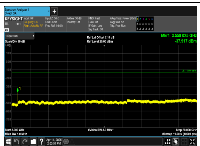
Band66-1.4MHz-16QAM-132665-1RB#0-3000~20000-PASS
