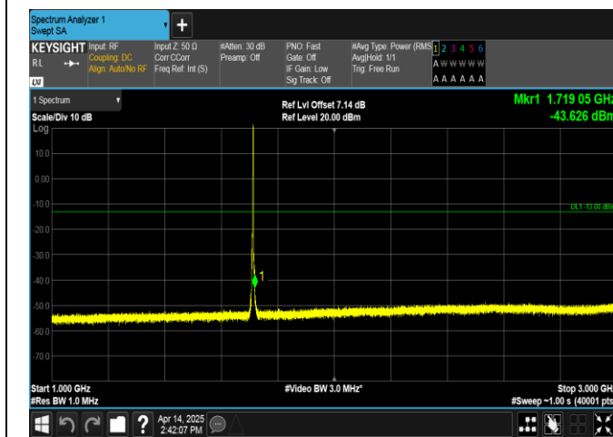
Band66-3MHz-QPSK-131987-1RB#14-1000~3000-PASS
