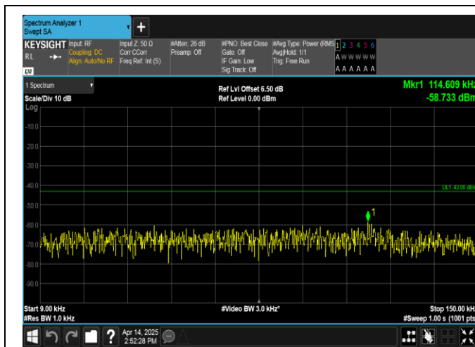
Band66-3MHz-QPSK-132657-1RB#0-0.009~0.15-PASS
