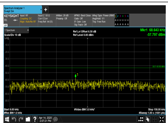
Band66-1.4MHz-16QAM-132665-6RB#0-0.009~0.15-PASS
