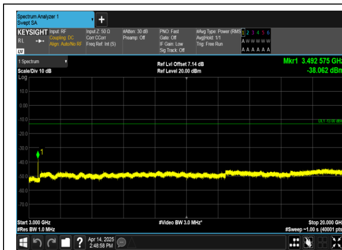
Band66-3MHz-QPSK-132322-1RB#14-3000~20000-PASS
