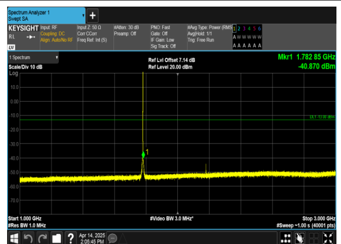
Band66-1.4MHz-16QAM-132665-1RB#5-1000~3000-PASS
