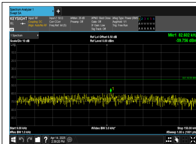
Band66-3MHz-QPSK-131987-1RB#0-0.009~0.15-PASS
