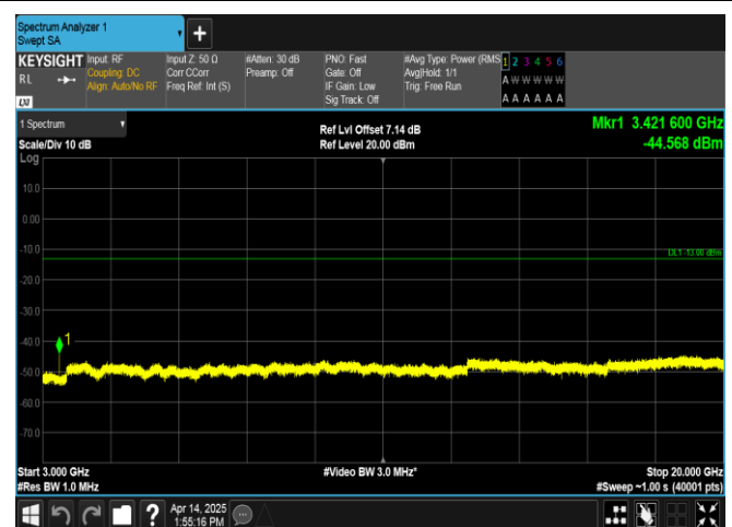
Band66-1.4MHz-16QAM-131979-6RB#0-3000~20000-PASS
