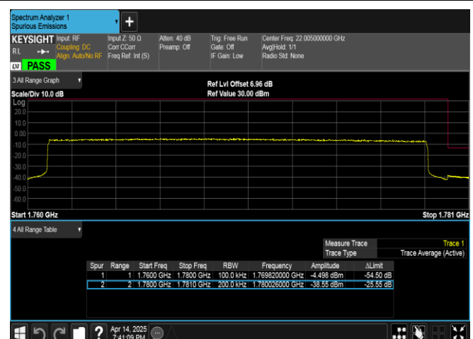
Band66-20MHz-16QAM-132572-100RB#0-PASS
