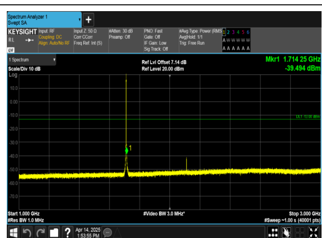
Band66-1.4MHz-QPSK-131979-6RB#0-1000~3000-PASS
