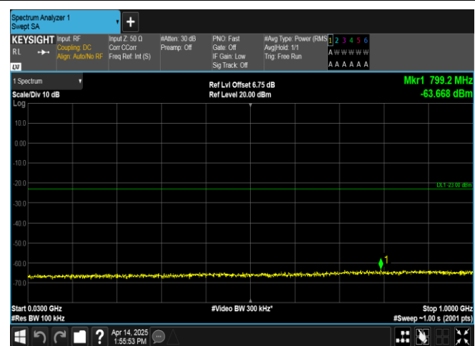
Band66-1.4MHz-QPSK-132322-1RB#0-30~1000-PASS
