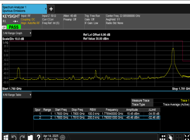
Band66-20MHz-16QAM-132572-1RB#99-PASS
