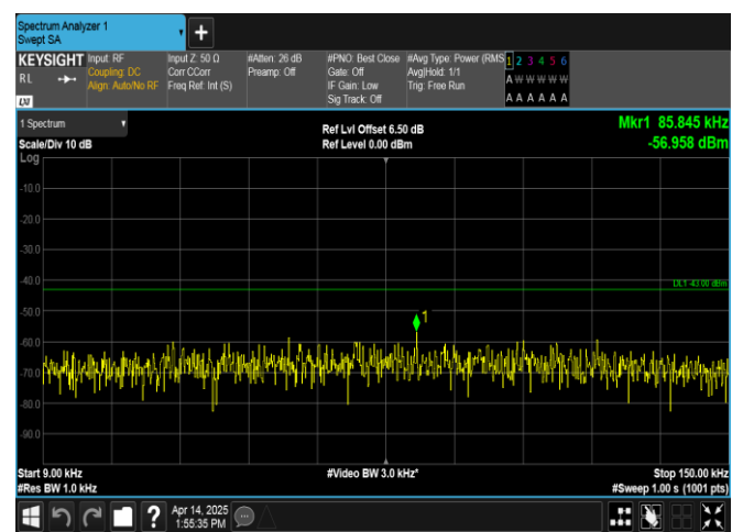
Band66-1.4MHz-QPSK-132322-1RB#0-0.009~0.15-PASS
