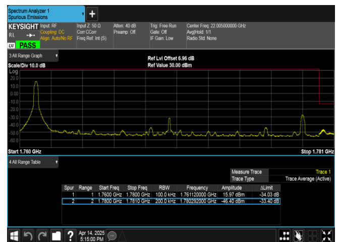
Band66-20MHz-16QAM-132572-1RB#0-PASS
