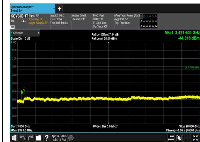
Band66-1.4MHz-QPSK-131979-6RB#0-3000~20000-PASS
