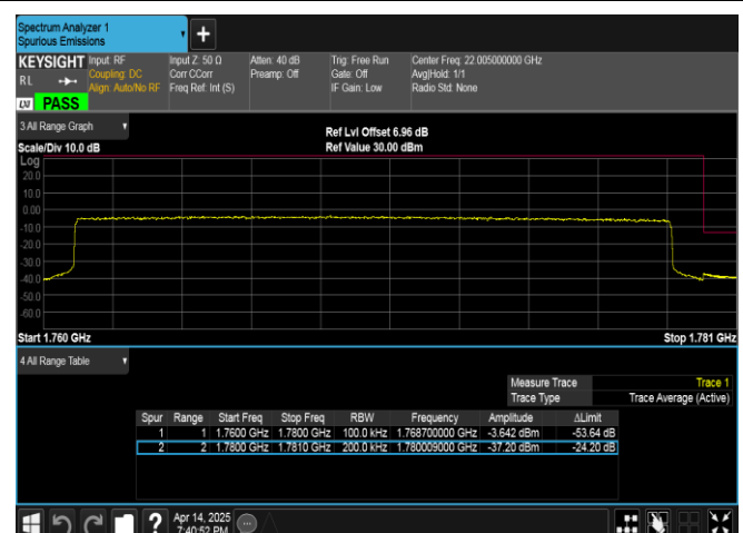
Band66-20MHz-QPSK-132572-100RB#0-PASS
