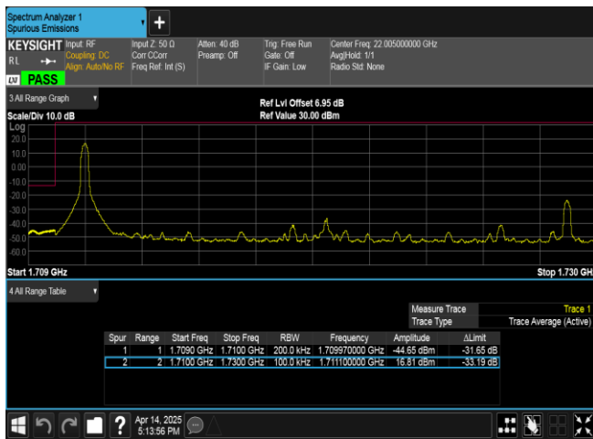
Band66-20MHz-16QAM-132072-1RB#0-PASS
