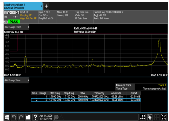
Band66-20MHz-16QAM-132072-1RB#99-PASS
