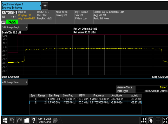
Band66-15MHz-16QAM-132047-75RB#0-PASS
