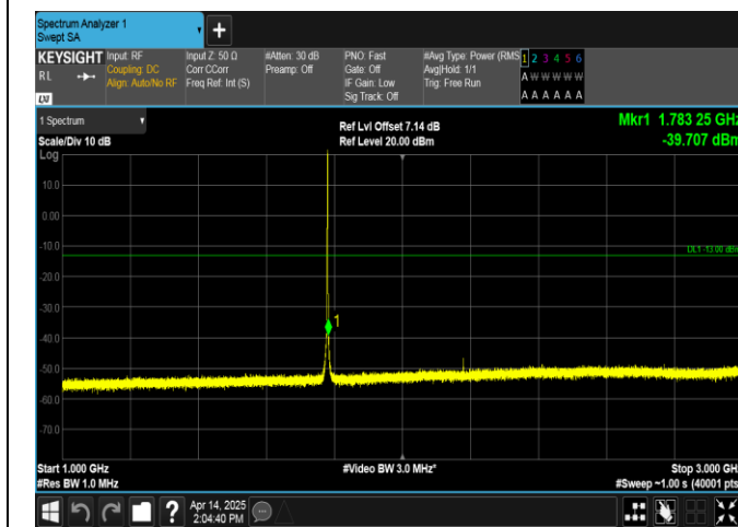
Band66-1.4MHz-QPSK-132665-1RB#5-1000~3000-PASS
