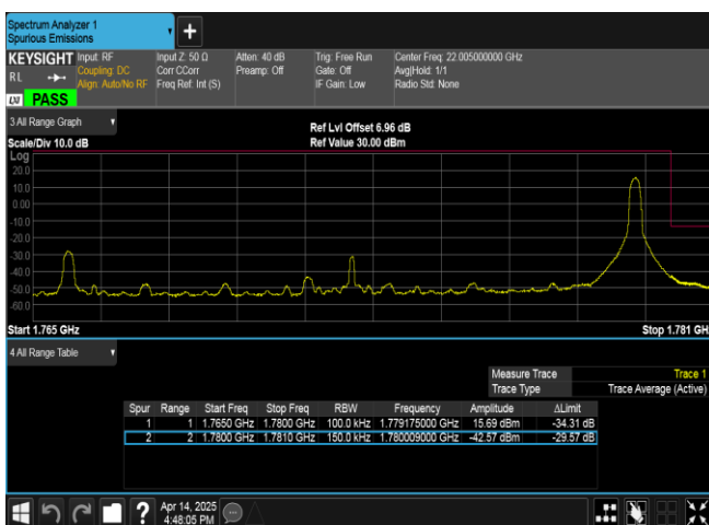
Band66-15MHz-16QAM-132597-1RB#74-PASS
