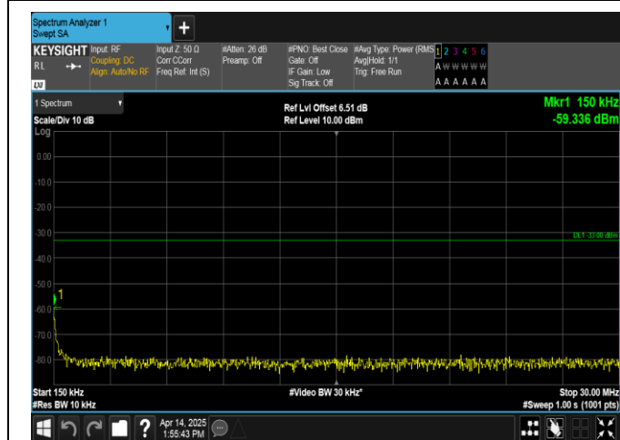
Band66-1.4MHz-QPSK-132322-1RB#0-0.15~30-PASS
