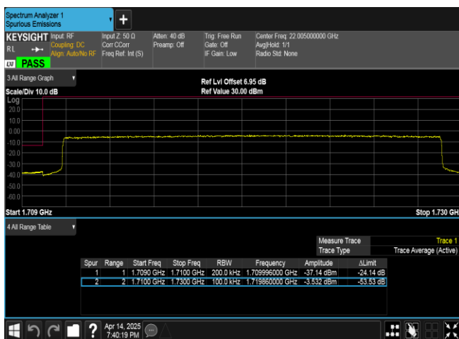
Band66-20MHz-QPSK-132072-100RB#0-PASS
