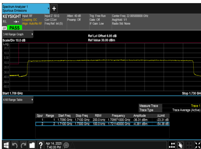
Band66-20MHz-16QAM-132072-100RB#0-PASS
