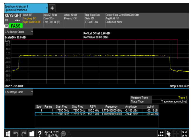
Band66-15MHz-16QAM-132597-75RB#0-PASS
