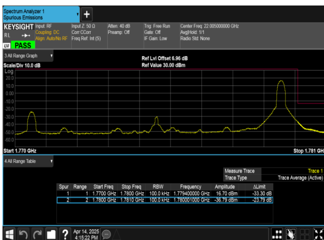
Band66-10MHz-QPSK-132622-1RB#49-PASS
