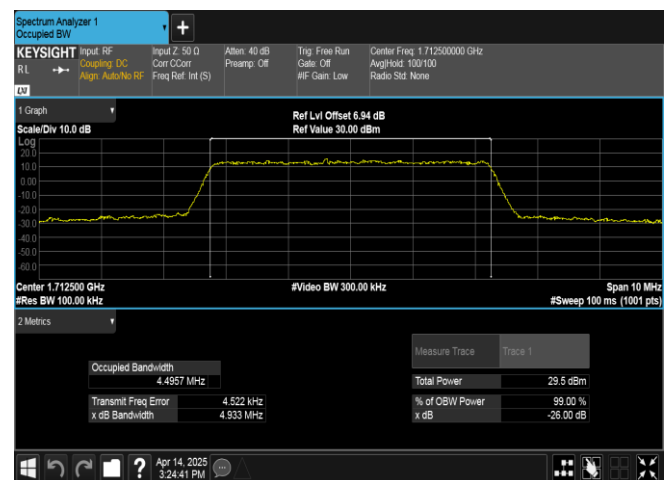
Band66-5MHz-16QAM-131997-25RB#0-PASS
