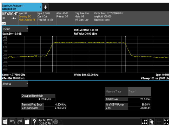
Band66-5MHz-QPSK-132647-25RB#0-PASS
