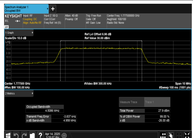
Band66-5MHz-16QAM-132647-25RB#0-PASS
