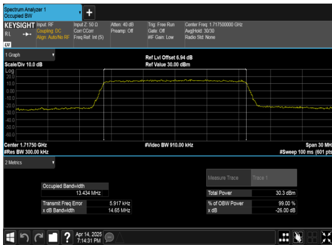
Band66-15MHz-QPSK-132047-75RB#0-PASS
