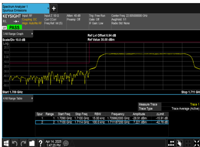
Band66-1.4MHz-16QAM-131979-6RB#0-PASS
