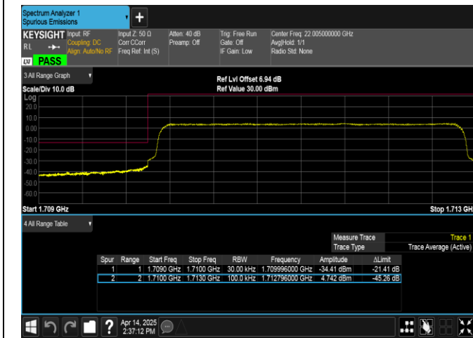
Band66-3MHz-QPSK-131987-15RB#0-PASS
