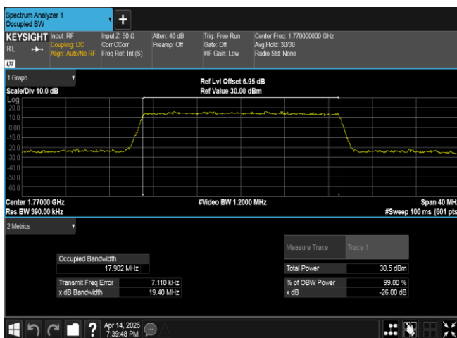
Band66-20MHz-QPSK-132572-100RB#0-PASS
