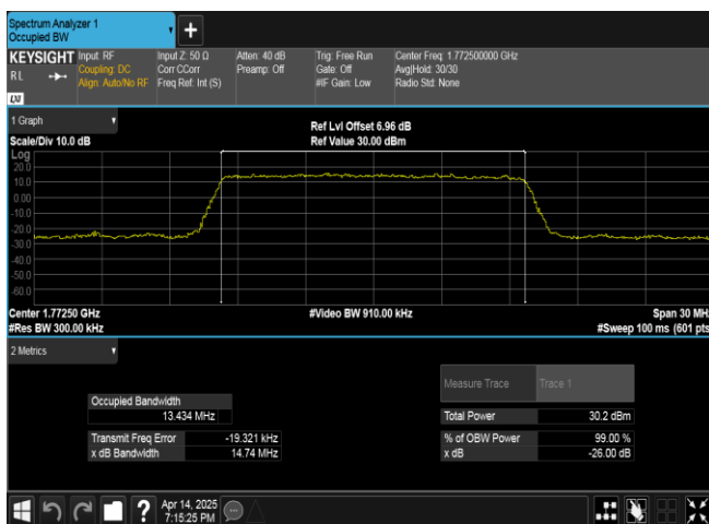
Band66-15MHz-QPSK-132597-75RB#0-PASS
