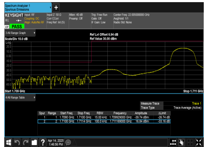
Band66-1.4MHz-16QAM-131979-1RB#5-PASS
