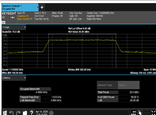
Band66-5MHz-16QAM-132322-25RB#0-PASS
