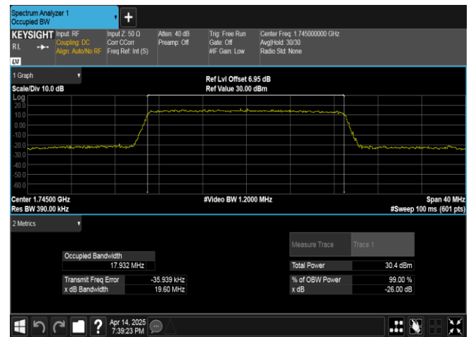
Band66-20MHz-QPSK-132322-100RB#0-PASS
