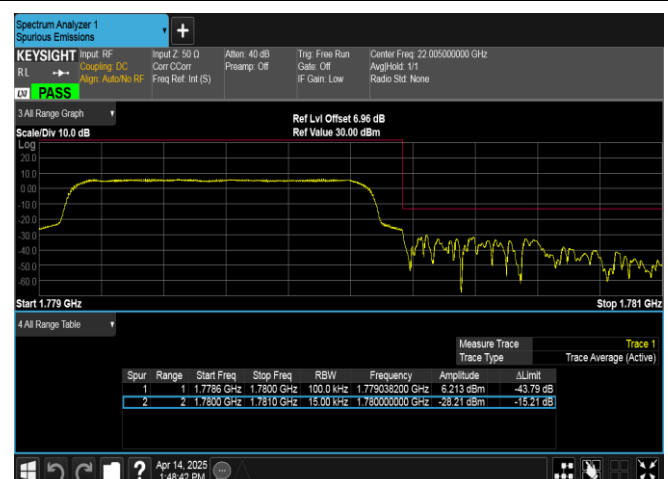
Band66-1.4MHz-16QAM-132665-6RB#0-PASS
