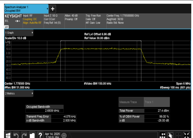
Band66-3MHz-16QAM-132657-15RB#0-PASS
