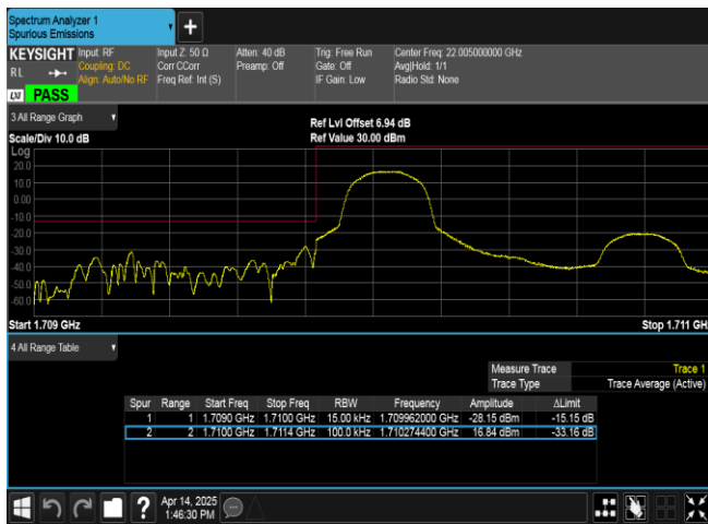
Band66-1.4MHz-16QAM-131979-1RB#0-PASS
