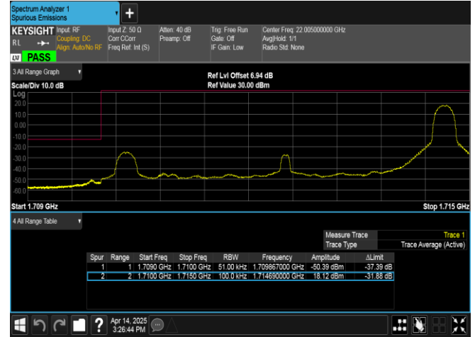
Band66-5MHz-QPSK-131997-1RB#24-PASS
