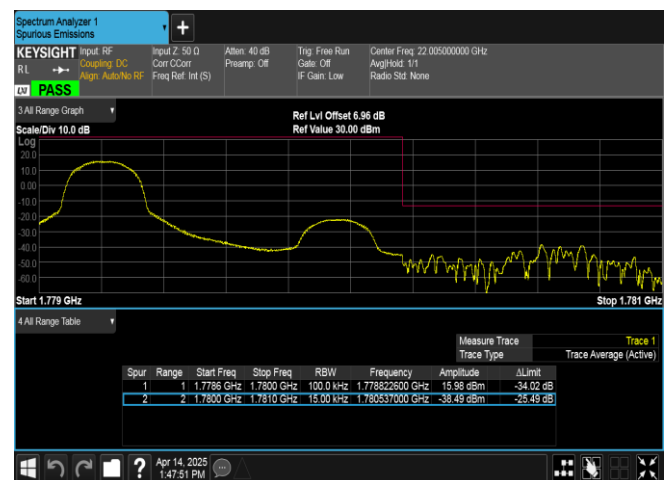
Band66-1.4MHz-16QAM-132665-1RB#0-PASS
