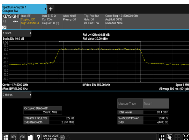
Band66-3MHz-16QAM-132322-15RB#0-PASS
