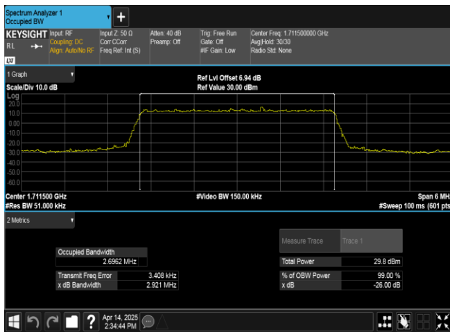
Band66-3MHz-QPSK-131987-15RB#0-PASS
