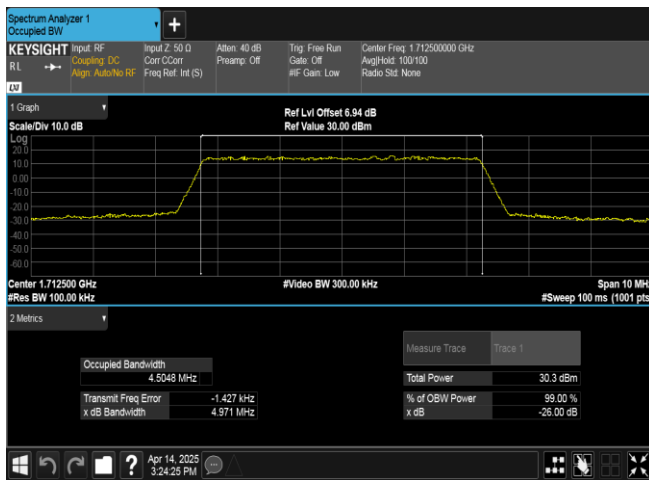
Band66-5MHz-QPSK-131997-25RB#0-PASS
