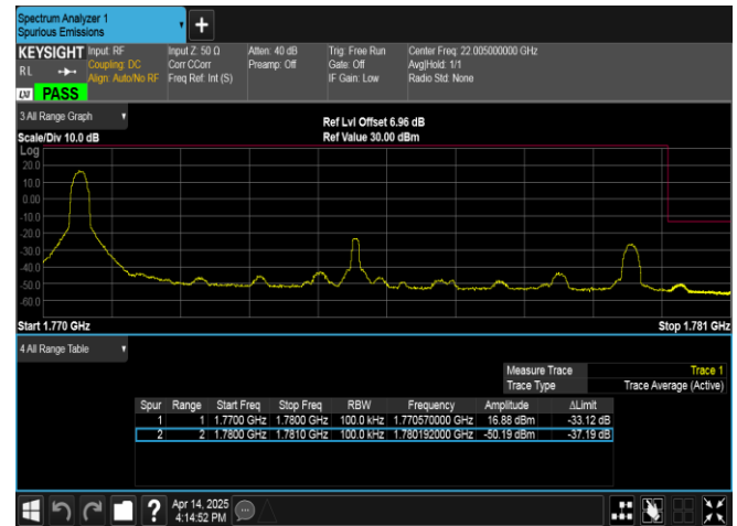
Band66-10MHz-QPSK-132622-1RB#0-PASS
