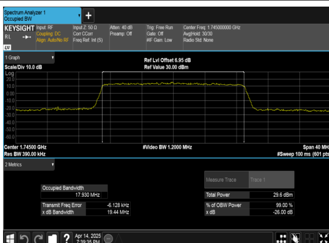
Band66-20MHz-16QAM-132322-100RB#0-PASS
