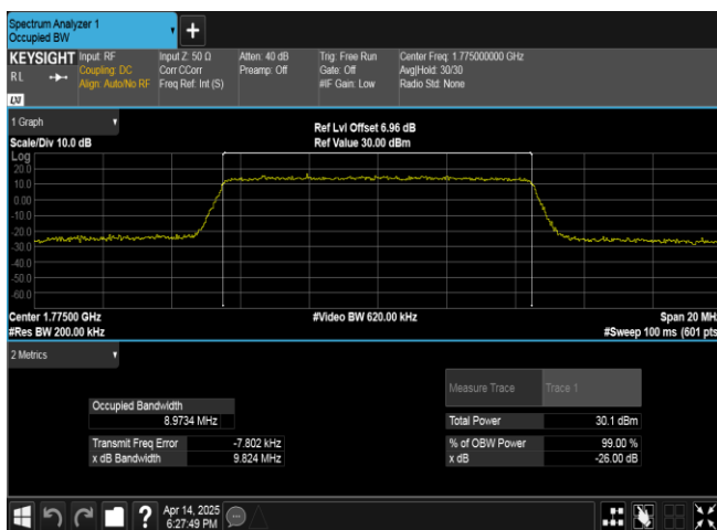
Band66-10MHz-QPSK-132622-50RB#0-PASS
