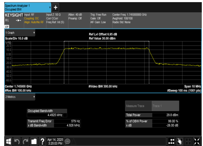
Band66-5MHz-QPSK-132322-25RB#0-PASS
