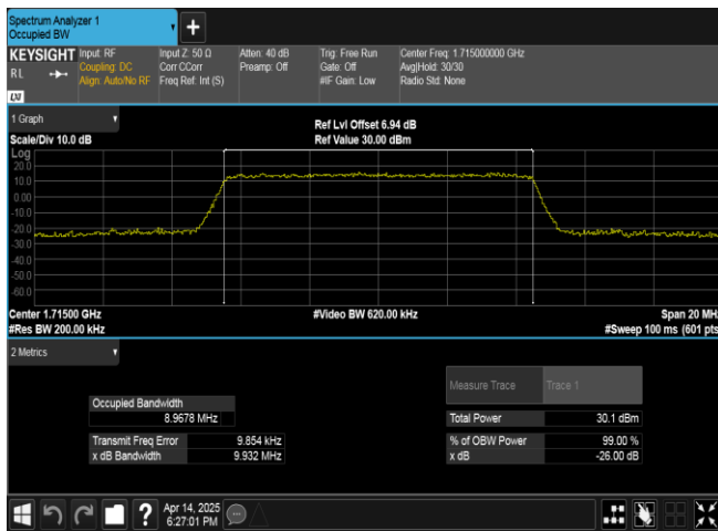
Band66-10MHz-QPSK-132022-50RB#0-PASS
