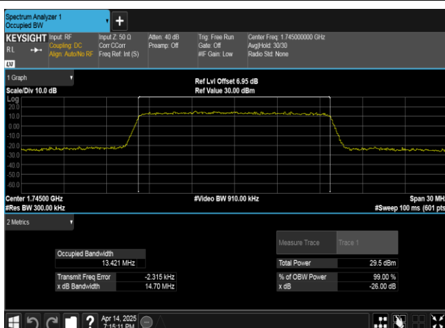
Band66-15MHz-16QAM-132322-75RB#0-PASS
