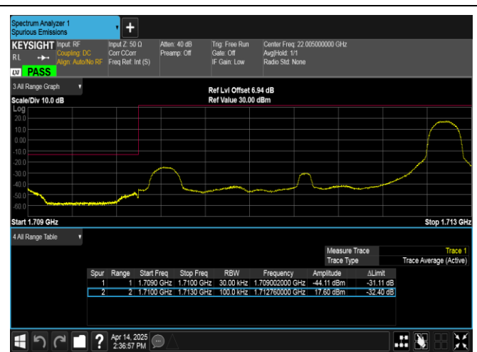
Band66-3MHz-16QAM-131987-1RB#14-PASS
