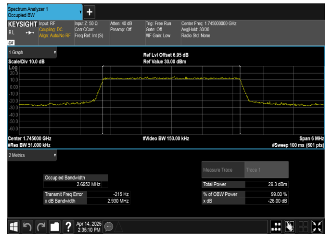
Band66-3MHz-QPSK-132322-15RB#0-PASS
