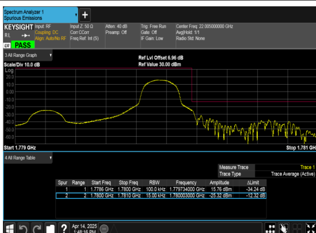
Band66-1.4MHz-16QAM-132665-1RB#5-PASS
