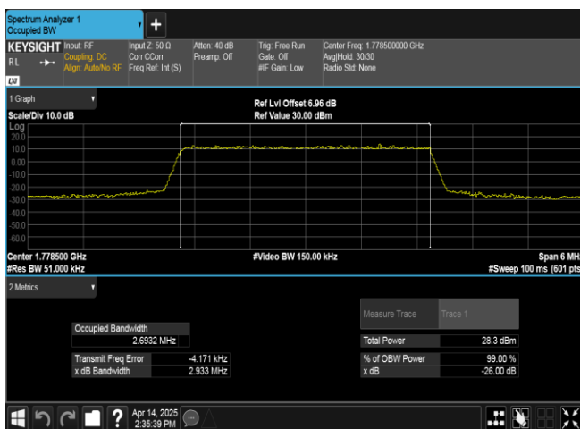
Band66-3MHz-QPSK-132657-15RB#0-PASS
