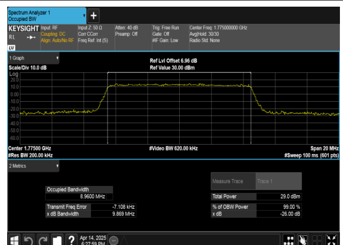
Band66-10MHz-16QAM-132622-50RB#0-PASS
