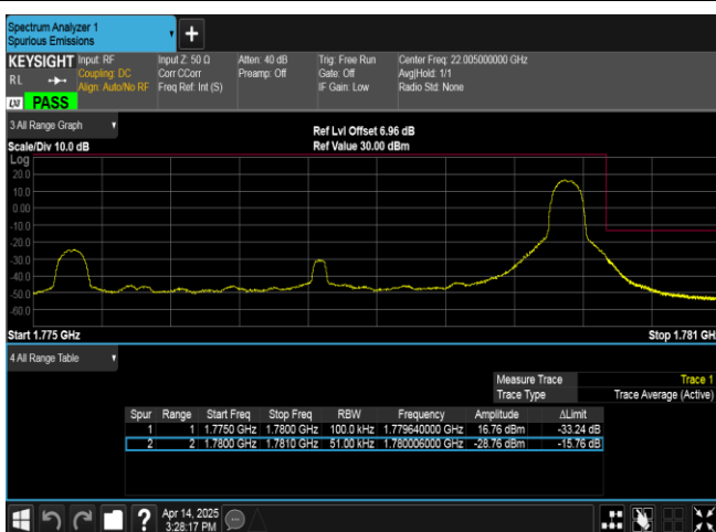
Band66-5MHz-QPSK-132647-1RB#24-PASS
