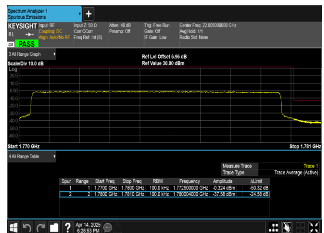
Band66-10MHz-QPSK-132622-50RB#0-PASS
