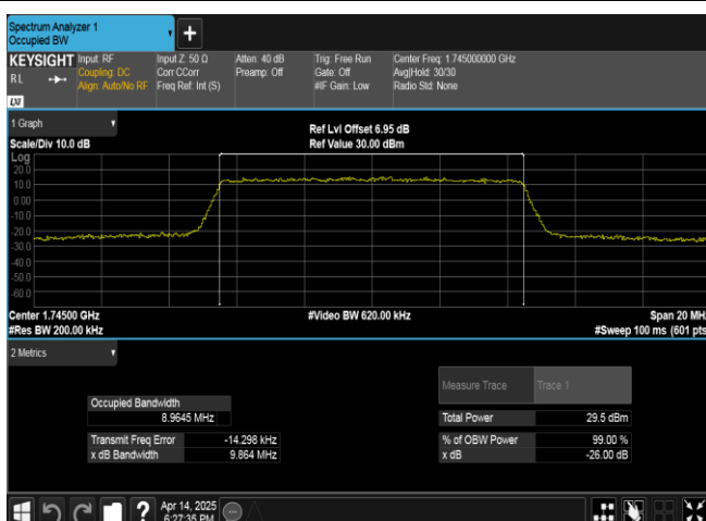
Band66-10MHz-16QAM-132322-50RB#0-PASS
