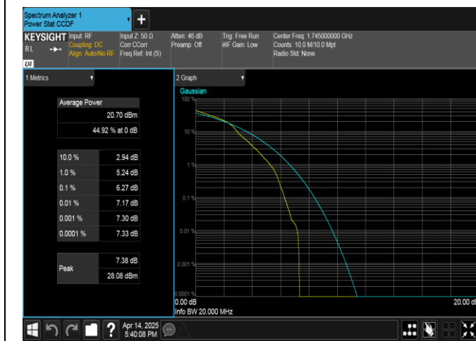
Band66-20MHz-16QAM-132322-1RB#0-PASS
