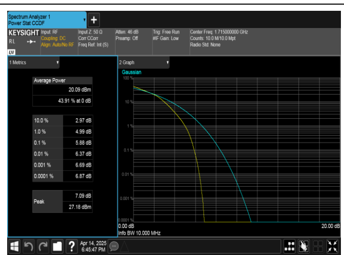
Band66-10MHz-16QAM-132022-50RB#0-PASS
