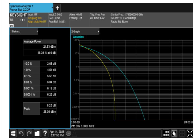
Band66-3MHz-QPSK-132322-1RB#0-PASS
