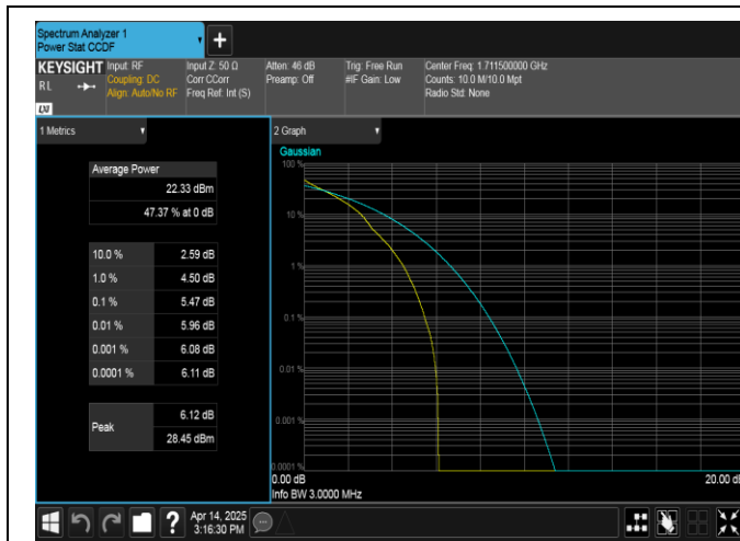
Band66-3MHz-QPSK-131987-1RB#0-PASS
