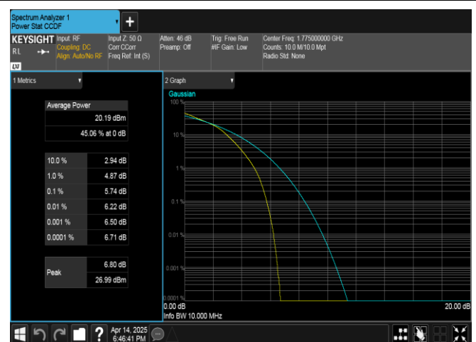
Band66-10MHz-16QAM-132622-50RB#0-PASS
