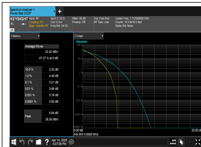
Band66-5MHz-QPSK-131997-1RB#0-PASS
