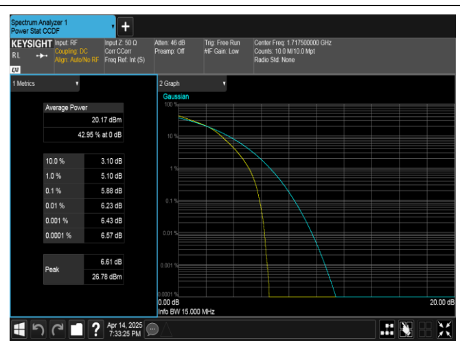
Band66-15MHz-16QAM-132047-75RB#0-PASS
