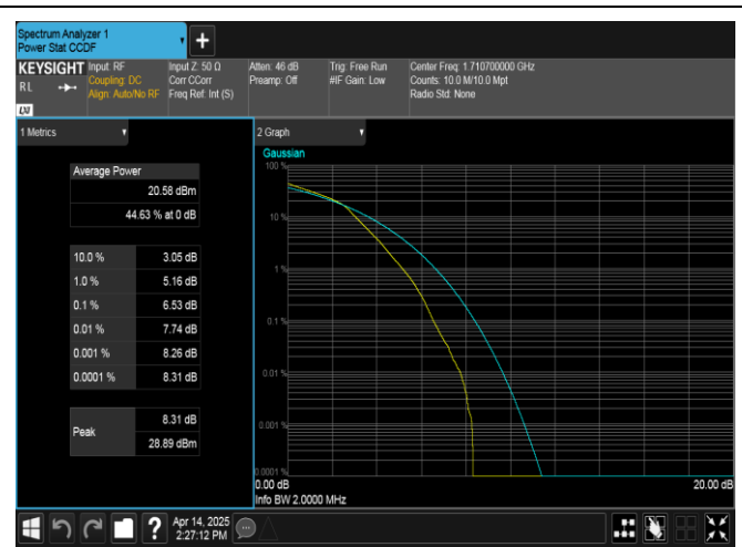
Band66-1.4MHz-16QAM-131979-6RB#0-PASS
