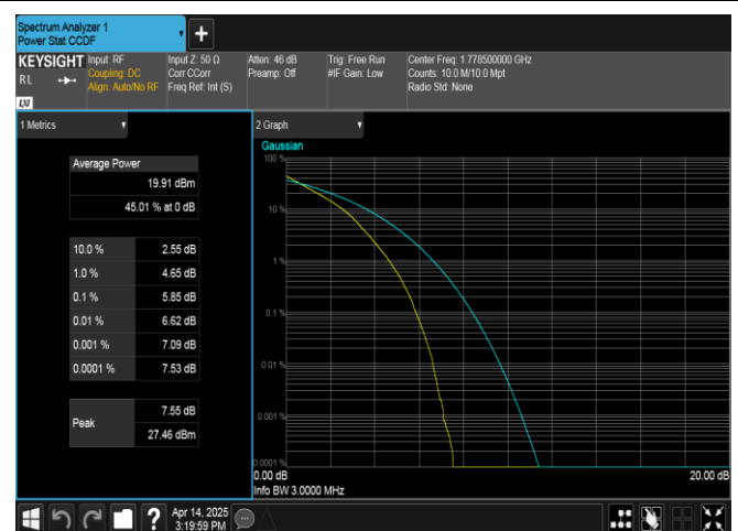
Band66-3MHz-QPSK-132657-15RB#0-PASS
