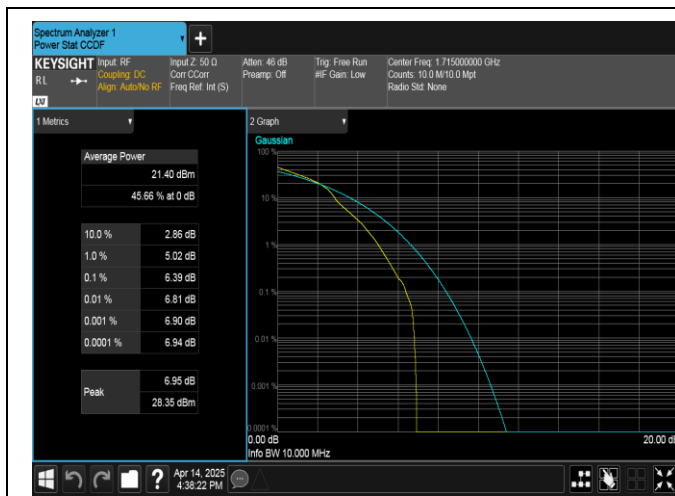
Band66-10MHz-16QAM-132022-1RB#0-PASS
