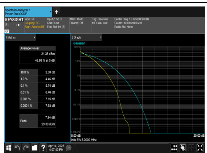
Band66-5MHz-QPSK-131997-25RB#0-PASS
