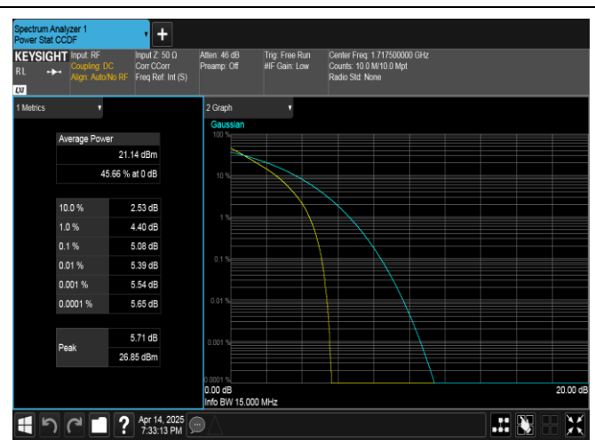
Band66-15MHz-QPSK-132047-75RB#0-PASS
