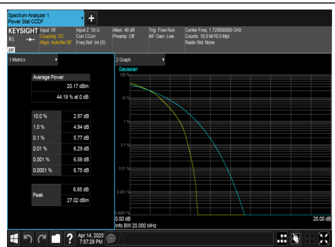
Band66-20MHz-16QAM-132072-100RB#0-PASS
