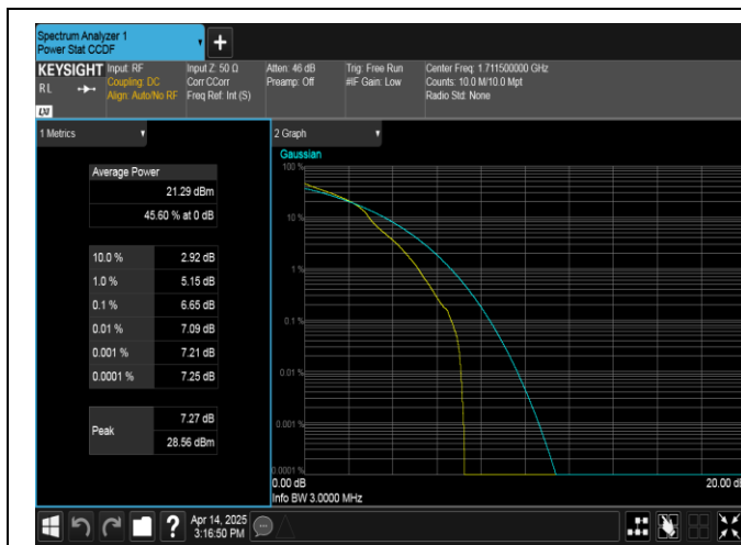
Band66-3MHz-16QAM-131987-1RB#0-PASS
