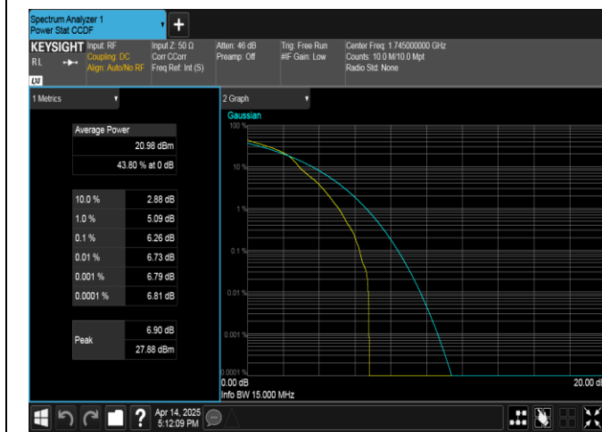
Band66-15MHz-16QAM-132322-1RB#0-PASS
