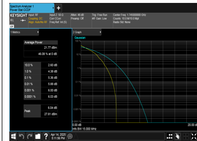
Band66-15MHz-QPSK-132322-1RB#0-PASS
