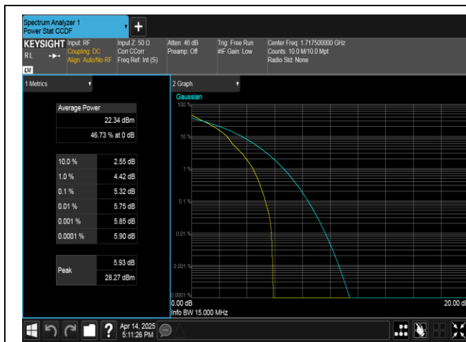
Band66-15MHz-QPSK-132047-1RB#0-PASS
