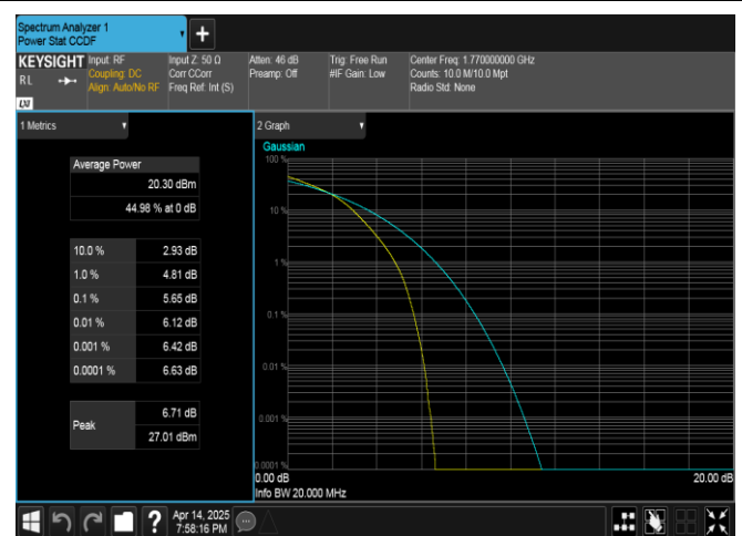
Band66-20MHz-16QAM-132572-100RB#0-PASS
