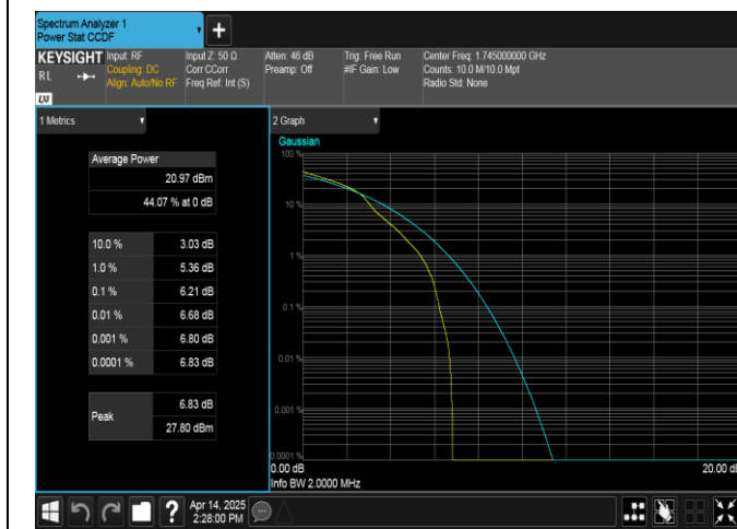
Band66-1.4MHz-16QAM-132322-1RB#0-PASS
