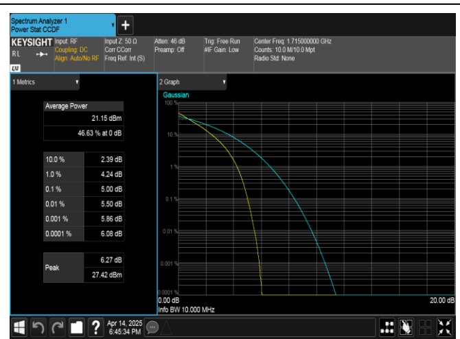
Band66-10MHz-QPSK-132022-50RB#0-PASS
