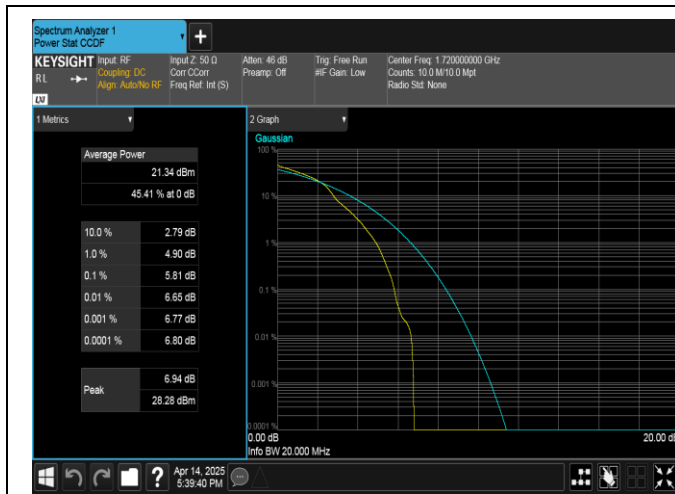
Band66-20MHz-16QAM-132072-1RB#0-PASS
