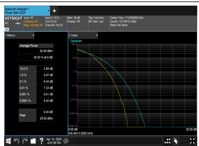
Band66-5MHz-16QAM-131997-25RB#0-PASS
