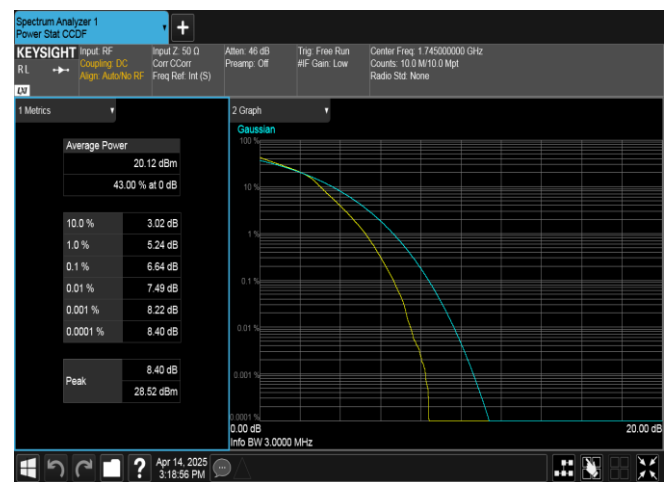
Band66-3MHz-16QAM-132322-15RB#0-PASS
