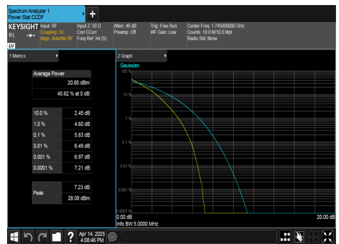
Band66-5MHz-QPSK-132322-25RB#0-PASS
