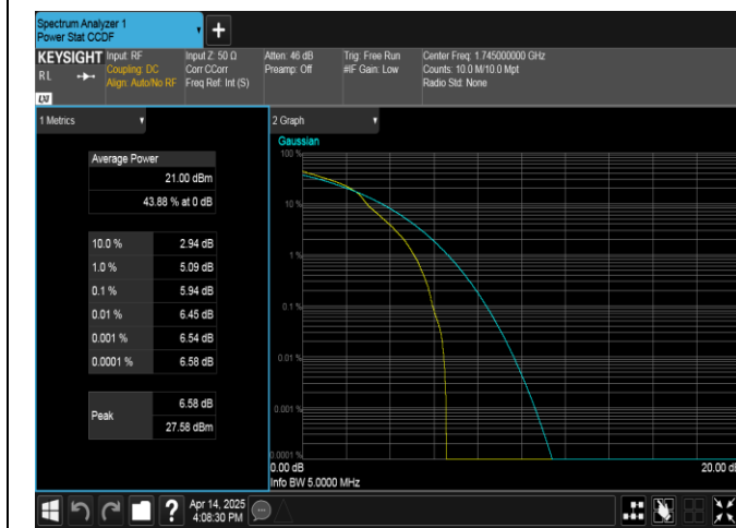
Band66-5MHz-16QAM-132322-1RB#0-PASS
