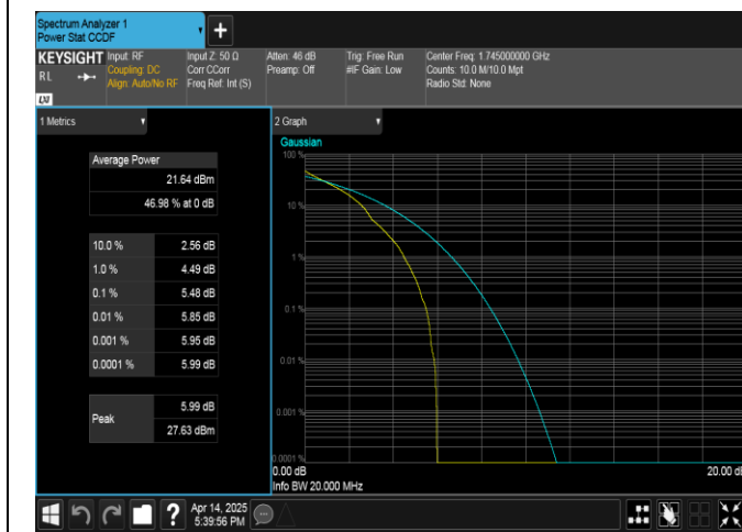
Band66-20MHz-QPSK-132322-1RB#0-PASS
