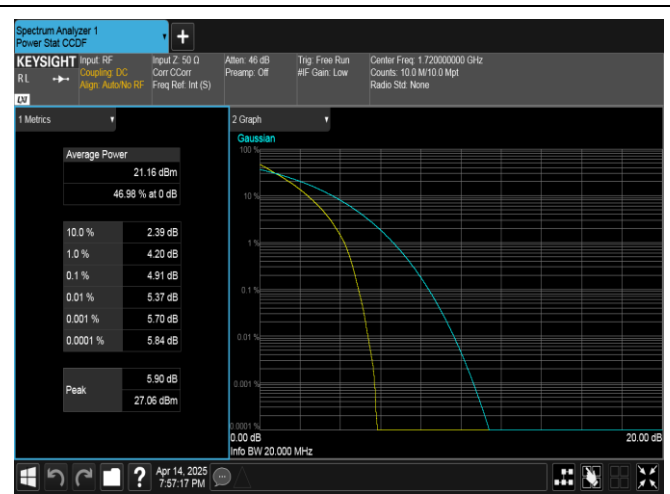
Band66-20MHz-QPSK-132072-100RB#0-PASS
