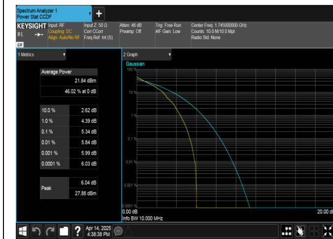
Band66-10MHz-QPSK-132322-1RB#0-PASS
