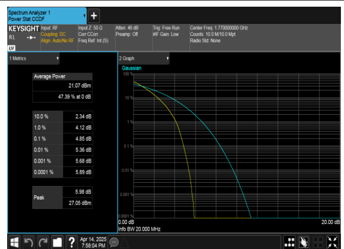
Band66-20MHz-QPSK-132572-100RB#0-PASS
