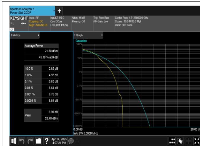
Band66-5MHz-16QAM-131997-1RB#0-PASS
