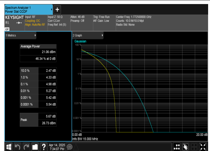
Band66-15MHz-QPSK-132597-75RB#0-PASS
