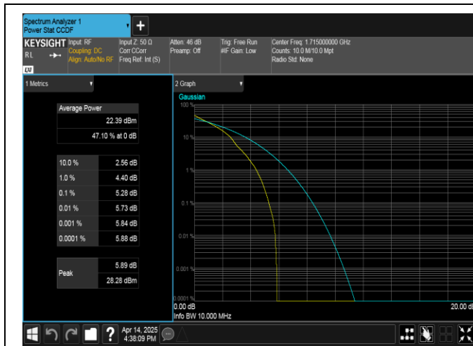
Band66-10MHz-QPSK-132022-1RB#0-PASS
