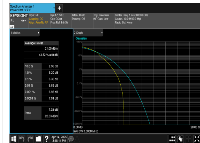
Band66-3MHz-16QAM-132322-1RB#0-PASS
