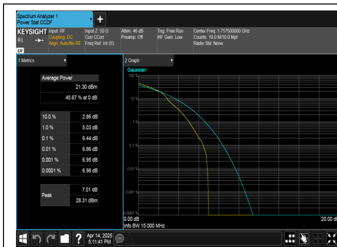
Band66-15MHz-16QAM-132047-1RB#0-PASS
