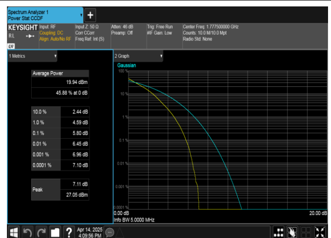
Band66-5MHz-QPSK-132647-25RB#0-PASS
