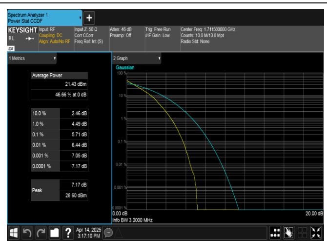
Band66-3MHz-QPSK-131987-15RB#0-PASS
