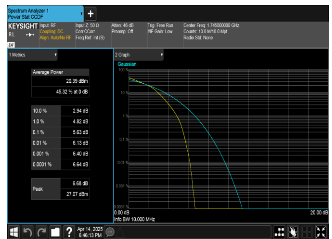
Band66-10MHz-16QAM-132322-50RB#0-PASS
