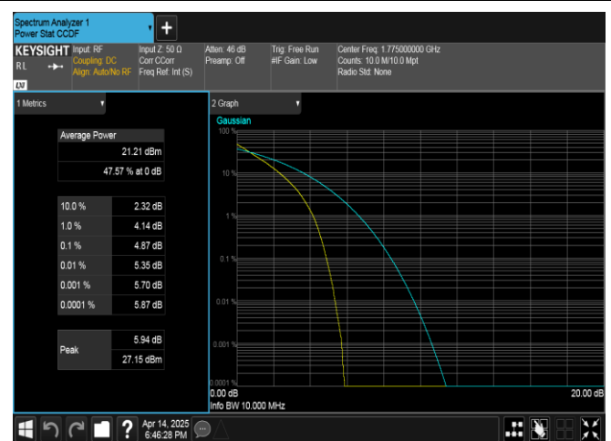
Band66-10MHz-QPSK-132622-50RB#0-PASS
