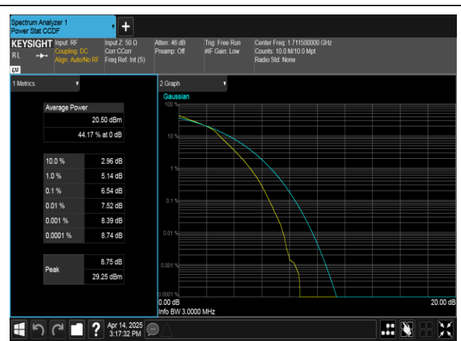
Band66-3MHz-16QAM-131987-15RB#0-PASS
