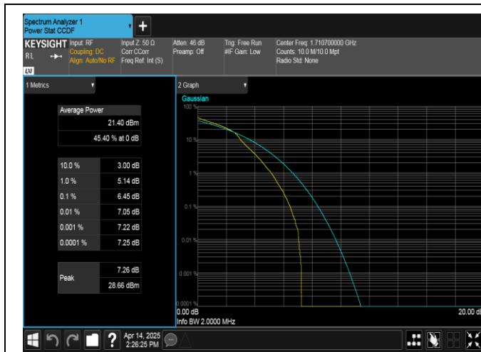
Band66-1.4MHz-16QAM-131979-1RB#0-PASS
