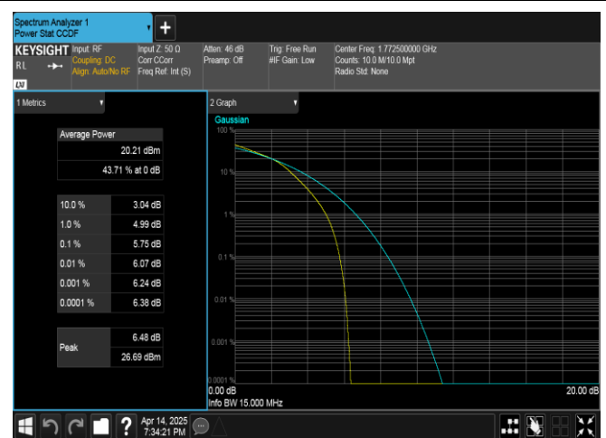
Band66-15MHz-16QAM-132597-75RB#0-PASS
