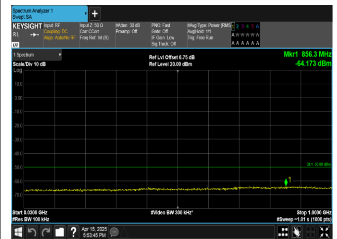
Band40(2350-2360)-5MHz-16QAM-39175-25RB#0-30-1000-PASS
