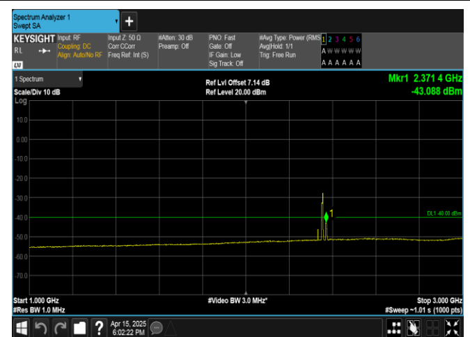
Band40(2350-2360)-5MHz-16QAM-39225-1RB#24-1000-3000-PASS
