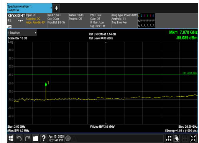
Band40(2350-2360)-5MHz-QPSK-39225-1RB#24-3000~26500-PASS
