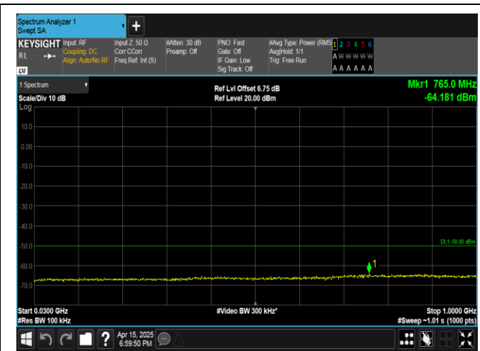
Band40(2350-2360)-10MHz-QPSK-39200-1RB#49-30~1000-PASS
