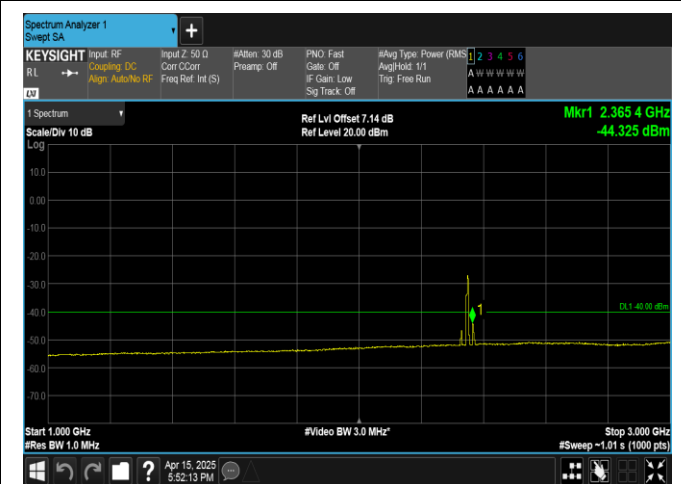
Band40(2350-2360)-5MHz-16QAM-39175-1RB#24-1000-3000-PASS
