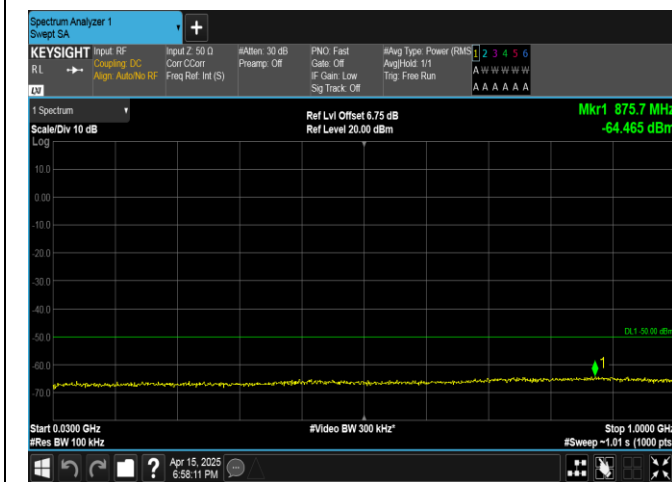
Band40(2350-2360)-10MHz-QPSK-39200-1RB#0-30-1000-PASS
