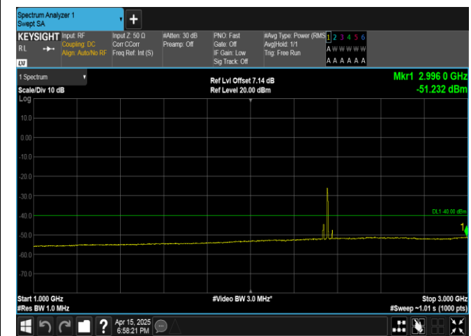
Band40(2350-2360)-10MHz-QPSK-39200-1RB#0-1000-3000-PASS
