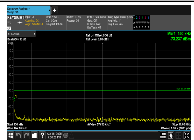
Band40(2350-2360)-10MHz-16QAM-39200-1RB#49-0.15~30-PASS
