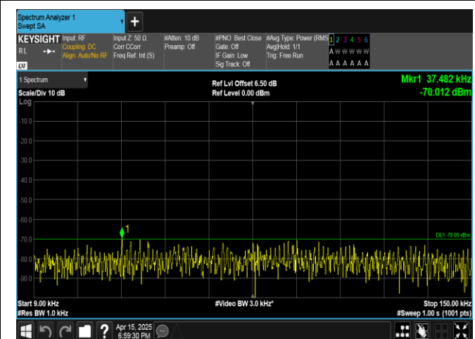
Band40(2350-2360)-10MHz-QPSK-39200-1RB#49-0.009-0.15-PASS
