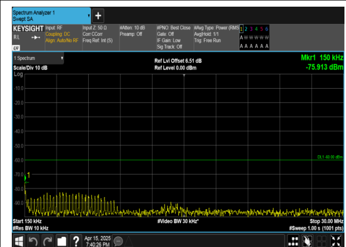
Band40(2350-2360)-10MHz-QPSK-39200-50RB#0-0.15~30-PASS
