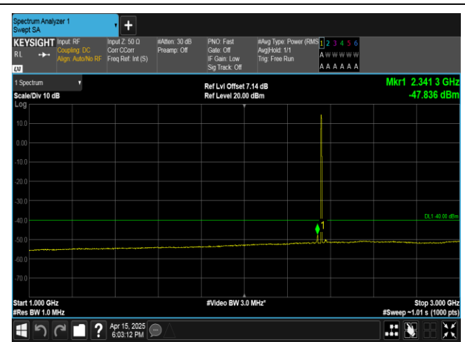
Band40(2350-2360)-5MHz-QPSK-39225-25RB#0-1000~3000-PASS
