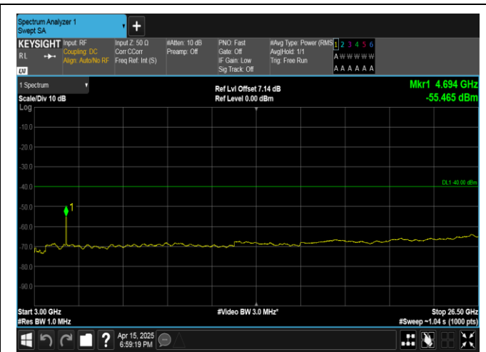
Band40(2350-2360)-10MHz-16QAM-39200-1RB#0-3000~26500-PASS
