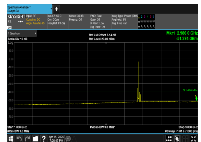
Band40(2350-2360)-10MHz-16QAM-39200-1RB#49-1000~3000-PASS
