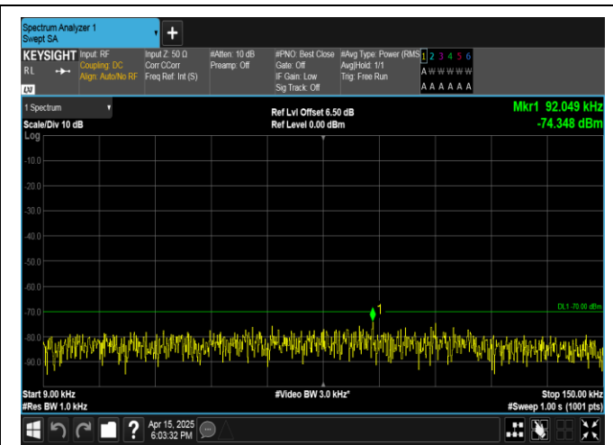
Band40(2350-2360)-5MHz-16QAM-39225-25RB#0-0.009-0.15-PASS
