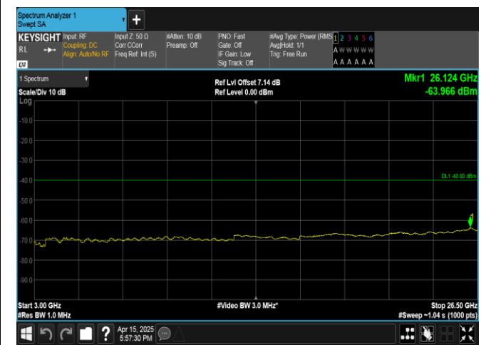
Band40(2350-2360)-5MHz-16QAM-39200-1RB#24-3000~26500-PASS
