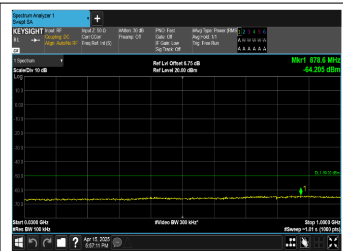
Band40(2350-2360)-5MHz-16QAM-39200-1RB#24-30~1000-PASS
