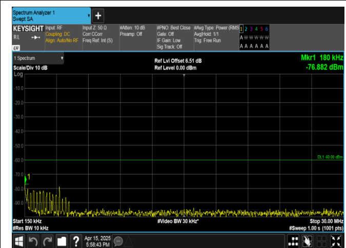
Band40(2350-2360)-5MHz-16QAM-39200-25RB#0-0.15~30-PASS
