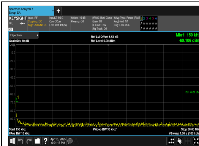
Band40(2350-2360)-5MHz-QPSK-39225-1RB#24-0.15~30-PASS
