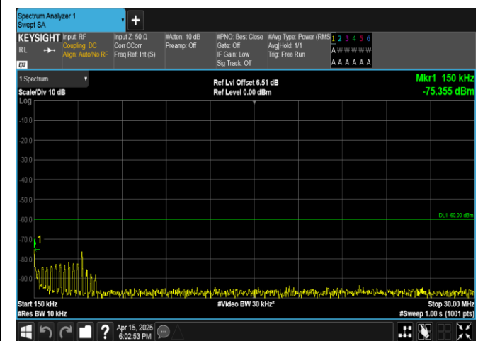
Band40(2350-2360)-5MHz-QPSK-39225-25RB#0-0.15~30-PASS
