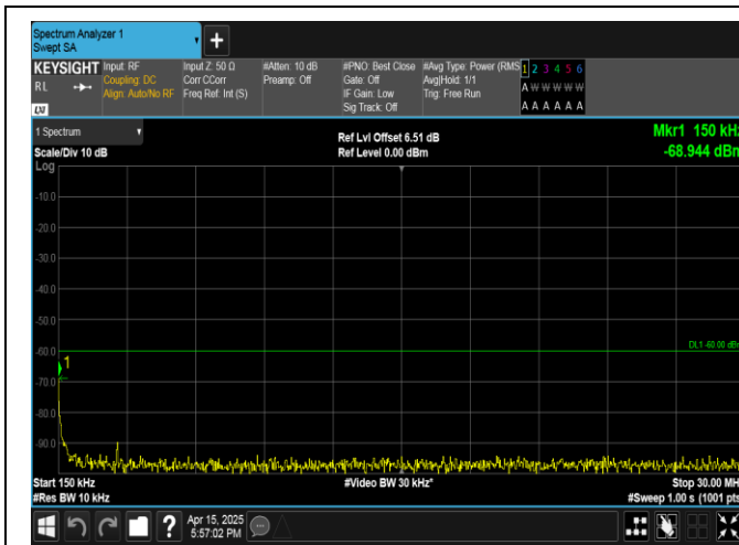
Band40(2350-2360)-5MHz-16QAM-39200-1RB#24-0.15~30-PASS
