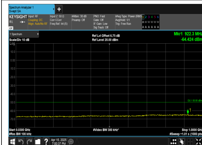
Band40(2350-2360)-10MHz-16QAM-39200-1RB#49-30~1000-PASS
