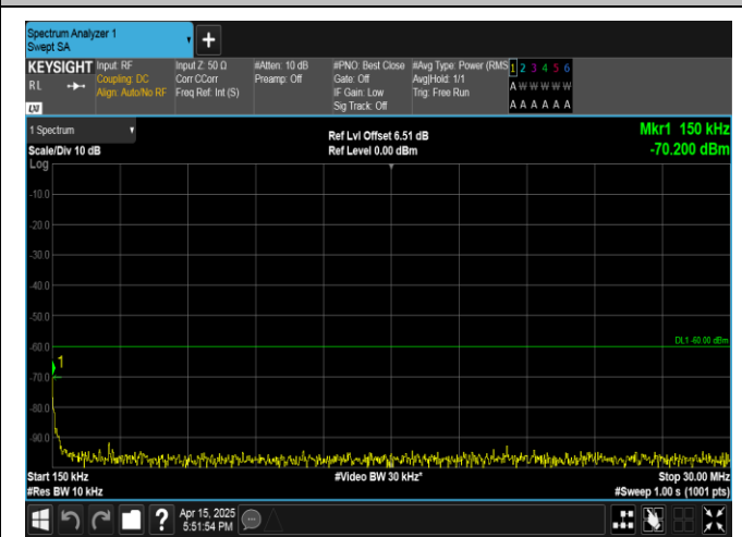
Band40(2350-2360)-5MHz-16QAM-39175-1RB#24-0.15-30-PASS
