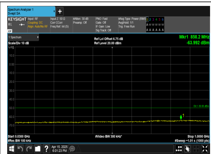
Band40(2350-2360)-5MHz-QPSK-39225-1RB#24-30~1000-PASS
