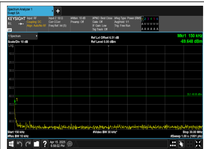
Band40(2350-2360)-10MHz-QPSK-39200-1RB#0.0.15-30-PASS
