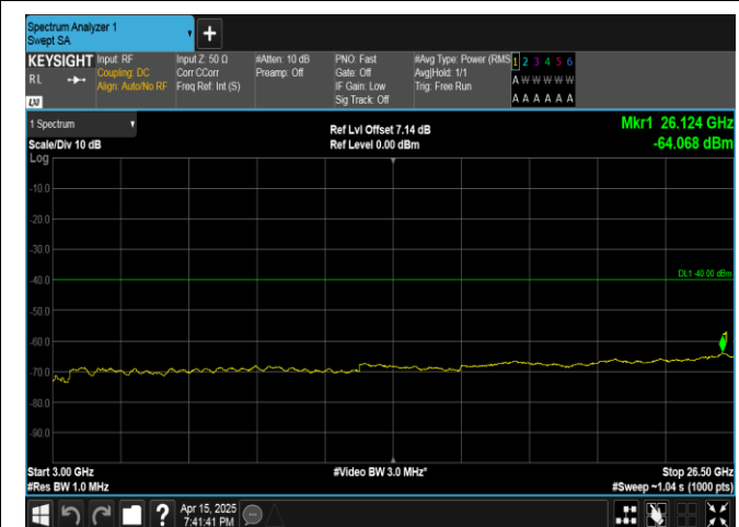
Band40(2350-2360)-10MHz-16QAM-39200-50RB#0-3000~26500-PASS
