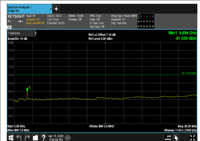
Band40(2350-2360)-5MHz-16QAM-39175-25RB#0-3000-26500-PASS
