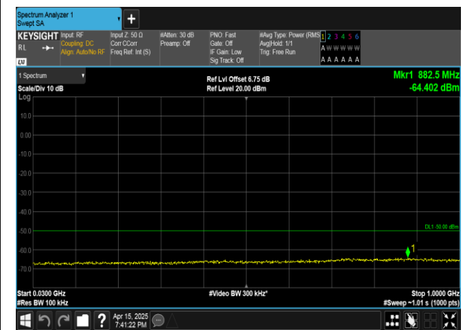
Band40(2350-2360)-10MHz-16QAM-39200-50RB#0-30~1000-PASS
