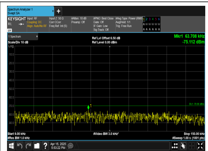
Band40(2350-2360)-5MHz-16QAM-39175-25RB#0-0.009-0.15-PASS
