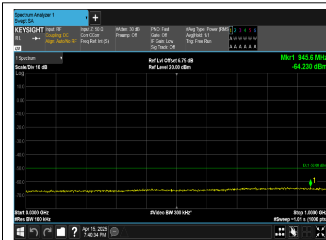
Band40(2350-2360)-10MHz-QPSK-39200-50RB#0-30~1000-PASS
