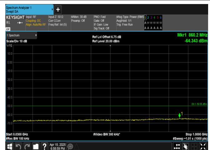
Band40(2350-2360)-10MHz-16QAM-39200-1RB#0-30~1000-PASS
