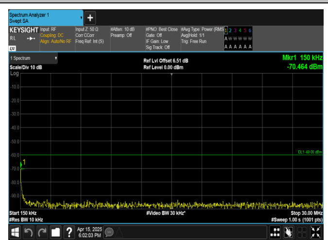
Band40(2350-2360)-5MHz-16QAM-39225-1RB#24-0.15-30-PASS
