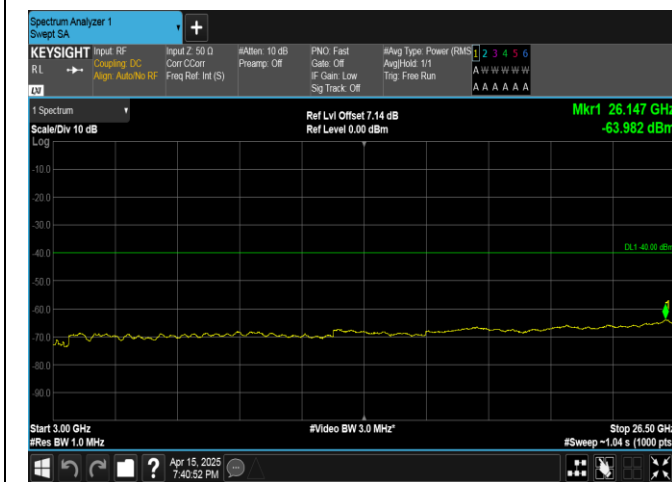
Band40(2350-2360)-10MHz-QPSK-39200-50RB#0-3000~26500-PASS
