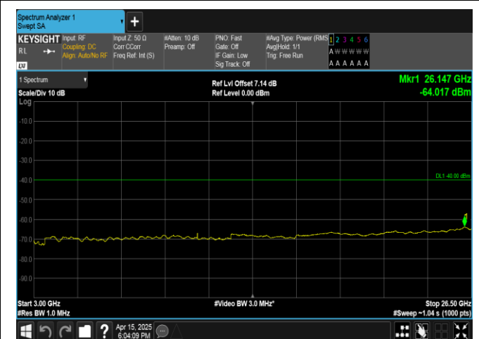
Band40(2350-2360)-5MHz-16QAM-39225-25RB#0-3000-26500-PASS
