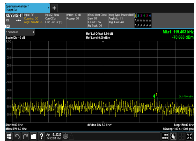
Band40(2350-2360)-5MHz-16QAM-39175-1RB#0-0.009~0.15-PASS
