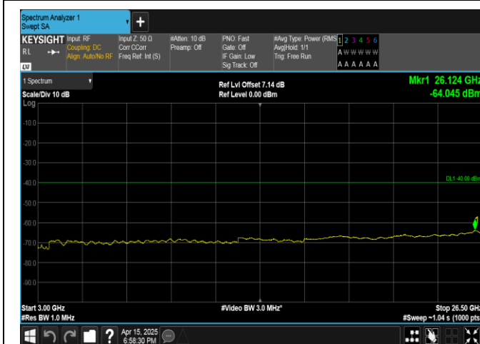
Band40(2350-2360)-10MHz-QPSK-39200-1RB#0-3000-26500-PASS
