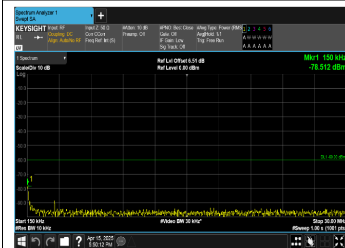
Band40(2350-2360)-5MHz-16QAM-39175-1RB#0-0.15~30-PASS
