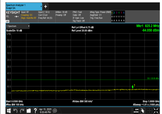
Band40(2350-2360)-5MHz-16QAM-39225-25RB#0-30-1000-PASS
