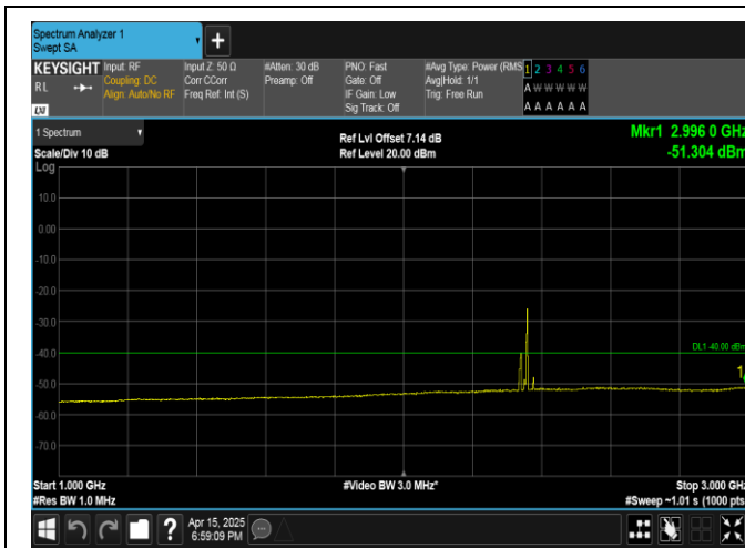
Band40(2350-2360)-10MHz-16QAM-39200-1RB#0-1000~3000-PASS
