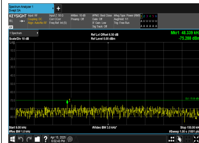
Band40(2350-2360)-5MHz-QPSK-39225-25RB#0-0.009~0.15-PASS
