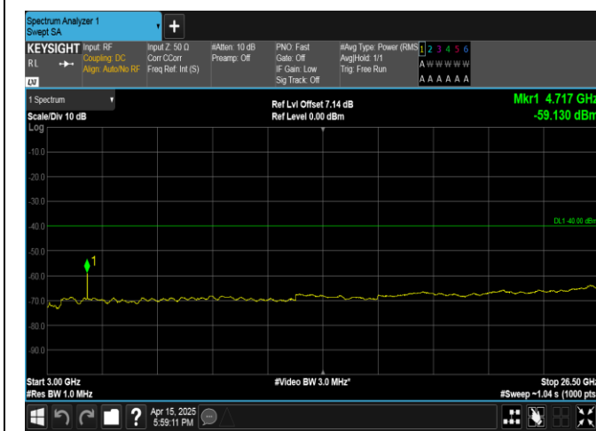
Band40(2350-2360)-5MHz-16QAM-39200-25RB#0-3000~26500-PASS
