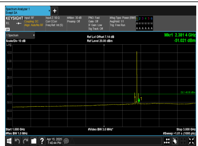
Band40(2350-2360)-10MHz-QPSK-39200-50RB#0-1000~3000-PASS
