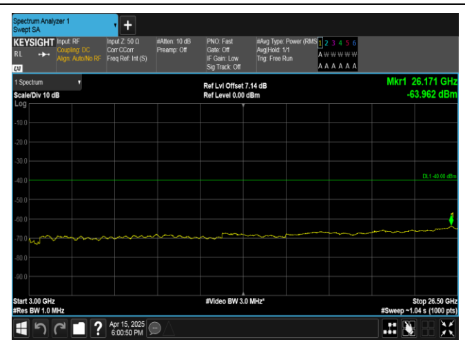
Band40(2350-2360)-5MHz-16QAM-39225-1RB#0-3000-26500-PASS
