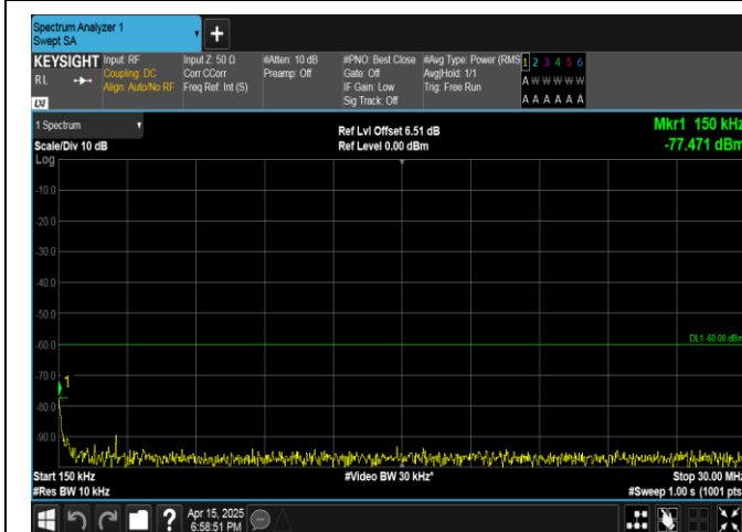
Band40(2350-2360)-10MHz-16QAM-39200-1RB#0-0.15~30-PASS
