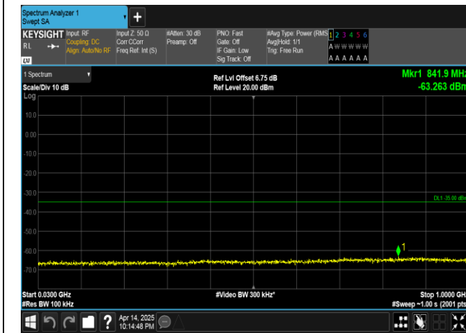
Band38-20MHz-16QAM-38150-1RB#99-30~1000-PASS
