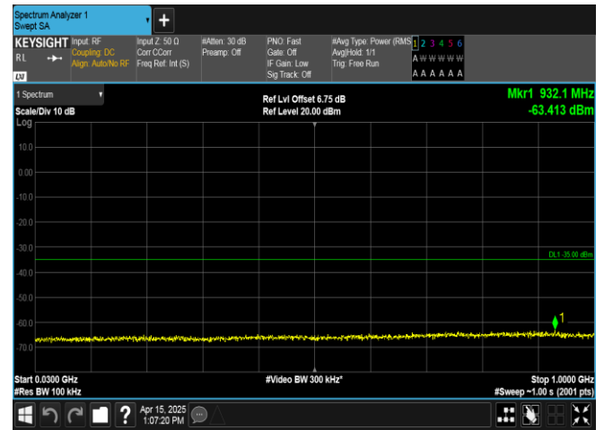
Band38-20MHz-16QAM-38150-100RB#0-30~1000-PASS
