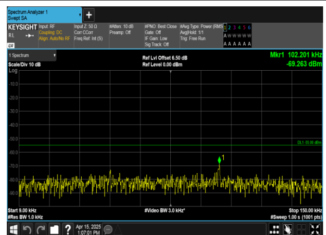
Band38-20MHz-16QAM-38150-100RB#0-0.009~0.15-PASS
