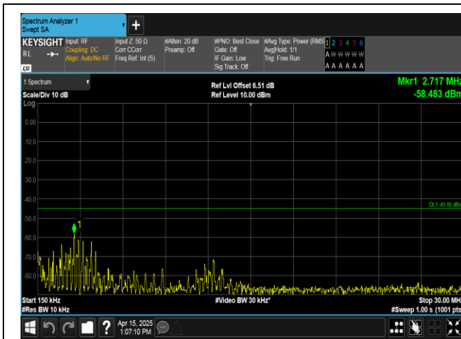
Band38-20MHz-16QAM-38150-100RB#0-0.15~30-PASS
