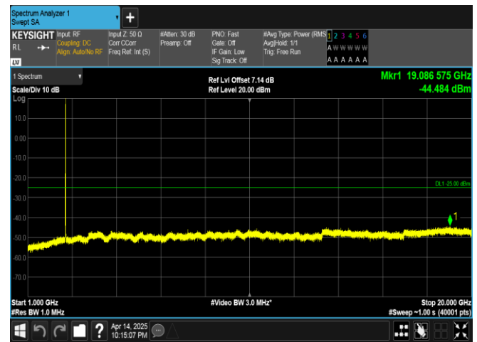
Band38-20MHz-16QAM-38150-1RB#99-1000~20000-PASS
