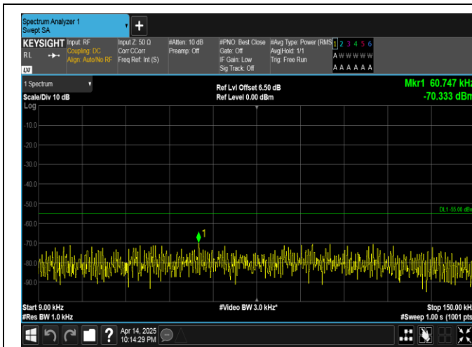
Band38-20MHz-16QAM-38150-1RB#99-0.009~0.15-PASS
