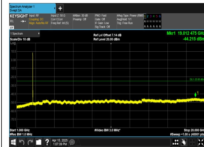
Band38-20MHz-16QAM-38150-100RB#0-1000~20000-PASS
