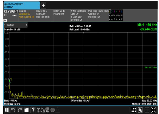
Band38-20MHz-16QAM-38150-1RB#99-0.15~30-PASS
