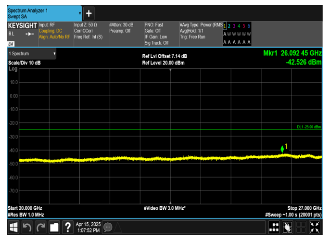
Band38-20MHz-16QAM-38150-100RB#0-20000~27000-PASS
