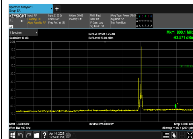
Band17-10MHz-16QAM-23800-1RB#49-30~1000-PASS
