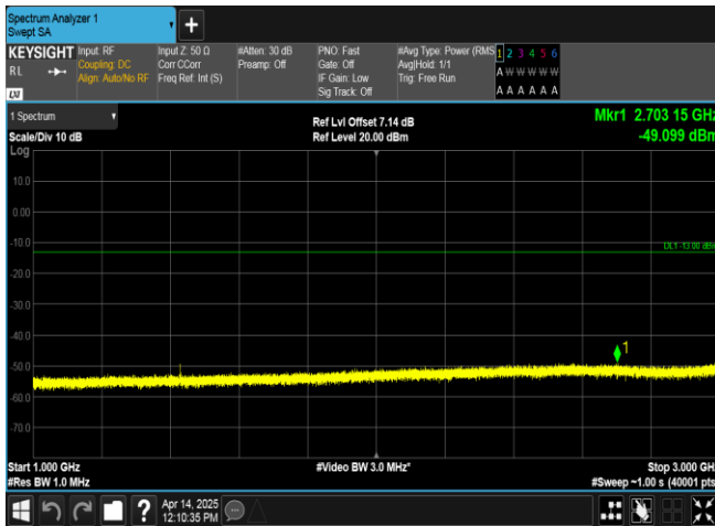
Band17-10MHz-16QAM-23790-1RB#49-1000~3000-PASS
