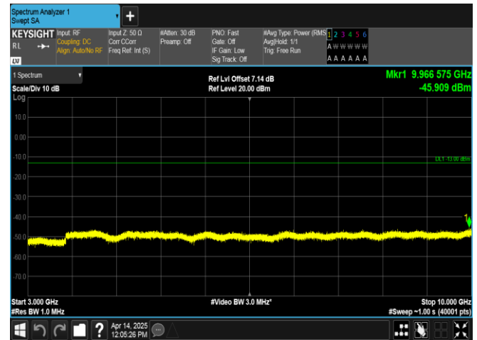
Band17-10MHz-QPSK-23780-1RB#49-3000~10000-PASS
