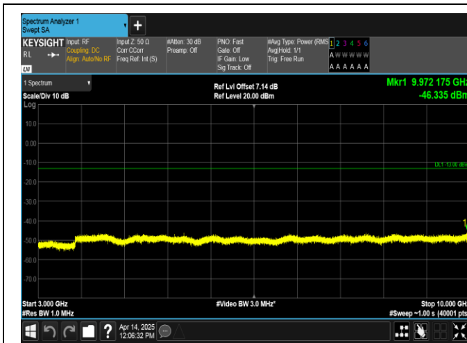
Band17-10MHz-16QAM-23780-1RB#49-3000~10000-PASS
