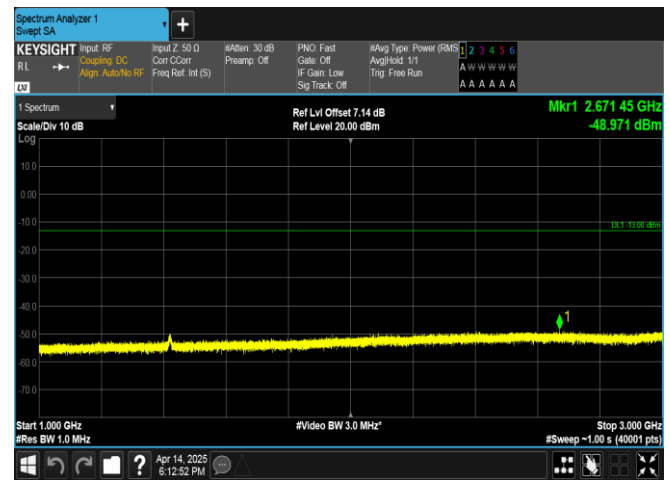
Band17-10MHz-16QAM-23790-50RB#0-1000~3000-PASS
