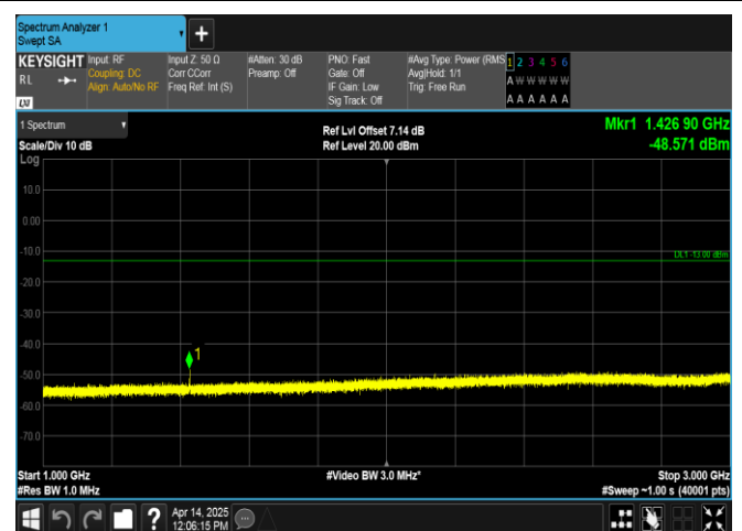
Band17-10MHz-16QAM-23780-1RB#49-1000~3000-PASS
