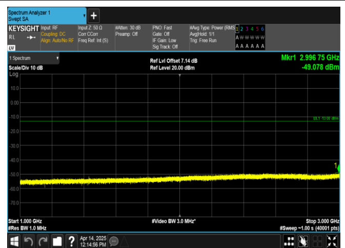
Band17-10MHz-16QAM-23800-1RB#49-1000~3000-PASS
