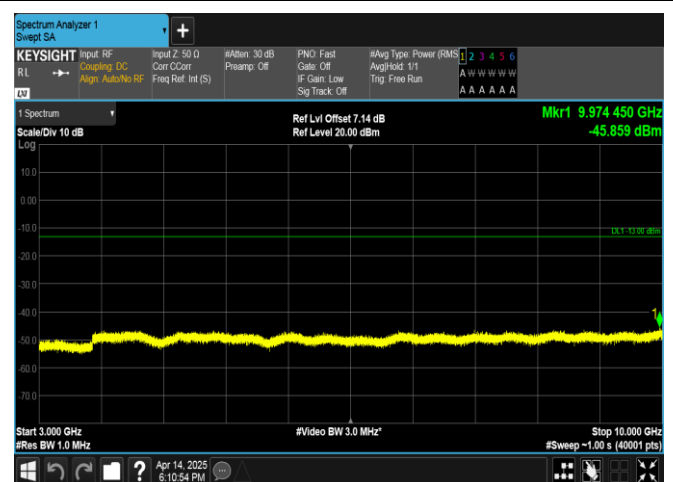
Band17-10MHz-16QAM-23780-50RB#0-3000~10000-PASS
