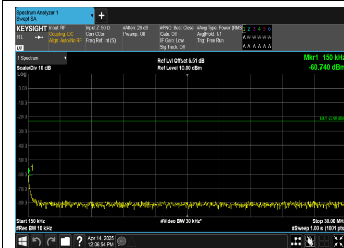
Band17-10MHz-QPSK-23790-1RB#0-0.15~30-PASS
