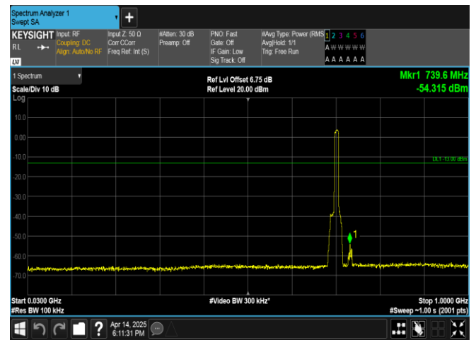
Band17-10MHz-QPSK-23790-50RB#0-30~1000-PASS
