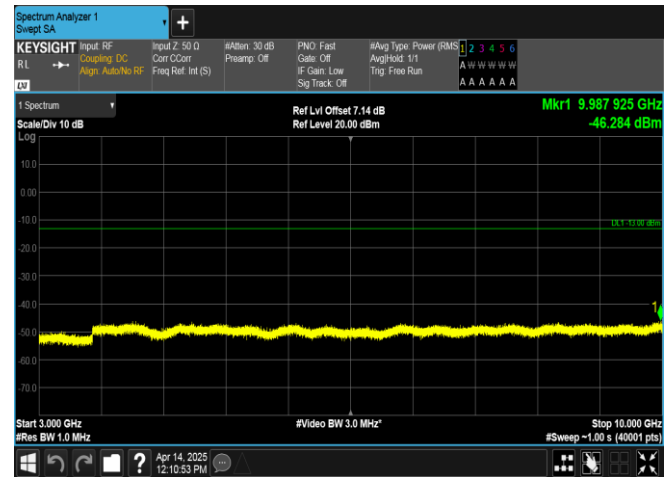
Band17-10MHz-16QAM-23790-1RB#49-3000~10000-PASS
