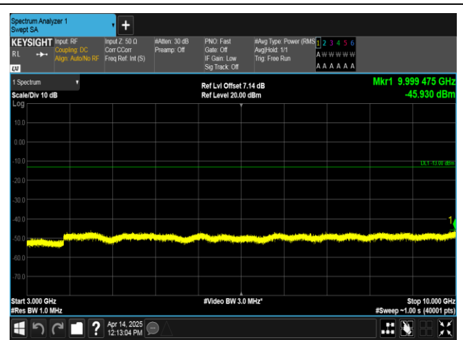
Band17-10MHz-16QAM-23800-1RB#0-3000~10000-PASS
