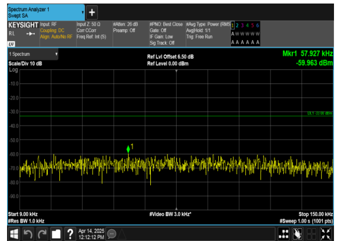
Band17-10MHz-16QAM-23800-1RB#0-0.009~0.15-PASS
