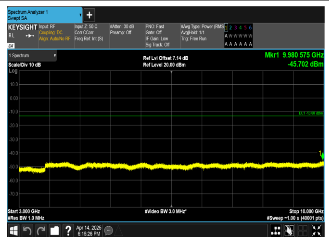
Band17-10MHz-16QAM-23800-50RB#0-3000~10000-PASS
