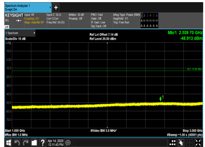
Band17-10MHz-QPSK-23800-1RB#0-1000~3000-PASS
