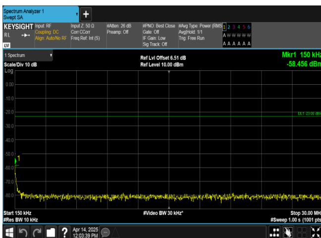
Band17-10MHz-16QAM-23780-1RB#0-0.15~30-PASS
