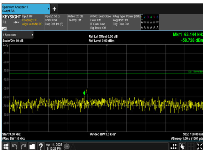
Band17-10MHz-QPSK-23800-50RB#0-0.009~0.15-PASS
