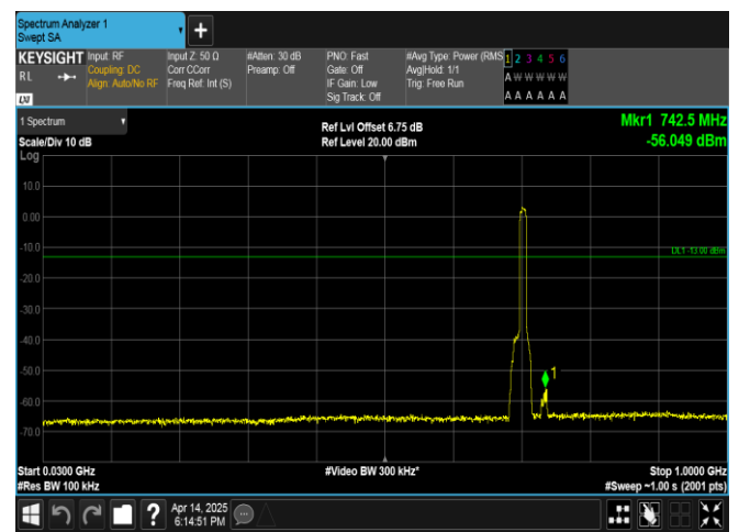
Band17-10MHz-16QAM-23800-50RB#0-30~1000-PASS
