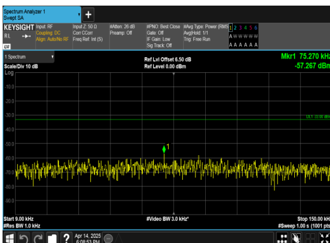
Band17-10MHz-QPSK-23780-50RB#0-0.009~0.15-PASS
