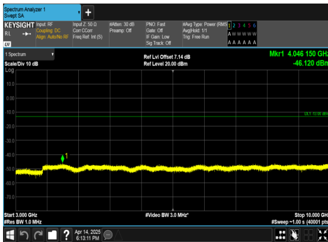
Band17-10MHz-16QAM-23790-50RB#0-3000~10000-PASS
