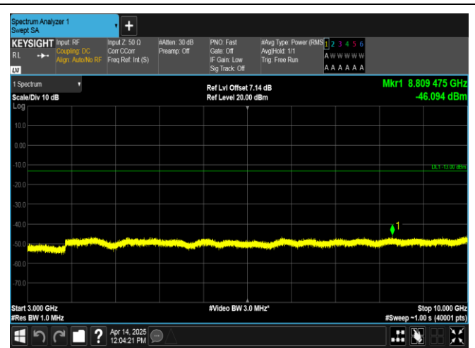
Band17-10MHz-16QAM-23780-1RB#0-3000~10000-PASS
