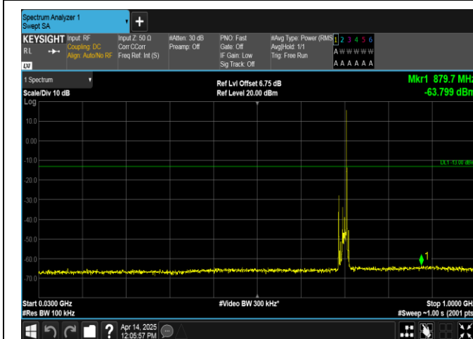
Band17-10MHz-16QAM-23780-1RB#49-30~1000-PASS
