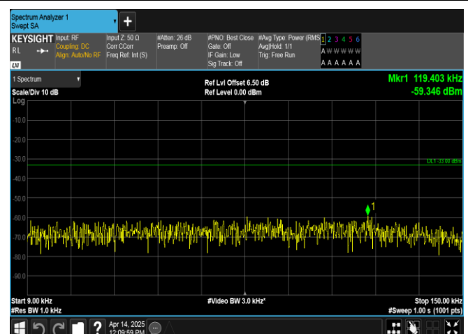
Band17-10MHz-16QAM-23790-1RB#49-0.009~0.15-PASS
