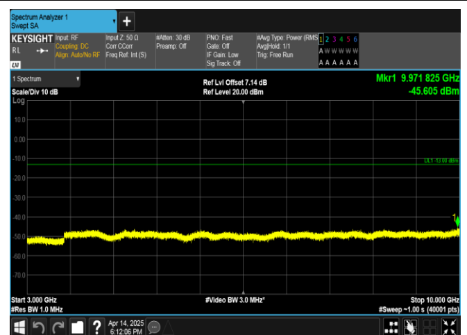
Band17-10MHz-QPSK-23790-50RB#0-3000~10000-PASS
