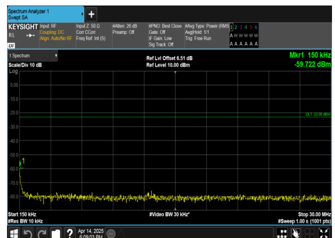
Band17-10MHz-QPSK-23780-50RB#0-0.15~30-PASS
