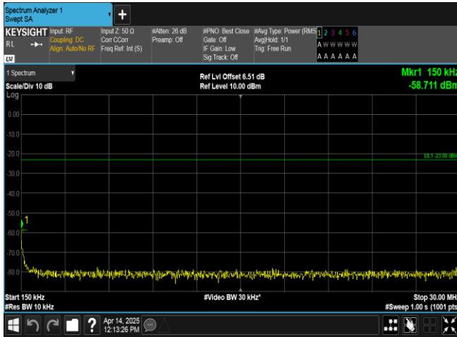
Band17-10MHz-QPSK-23800-1RB#49-0.15~30-PASS
