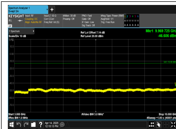
Band17-10MHz-16QAM-23800-1RB#49-3000~10000-PASS
