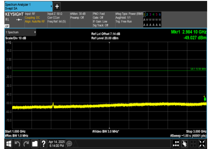
Band17-10MHz-QPSK-23800-50RB#0-1000~3000-PASS
