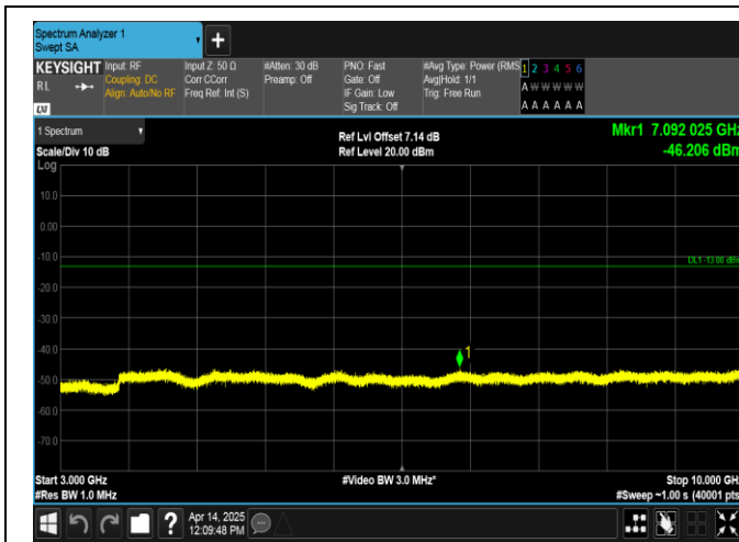
Band17-10MHz-QPSK-23790-1RB#49-3000~10000-PASS
