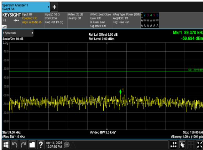
Band17-10MHz-16QAM-23790-1RB#0-0.009~0.15-PASS
