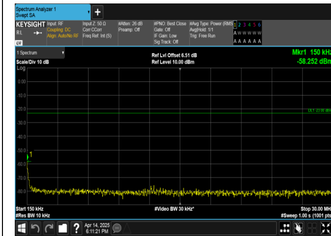
Band17-10MHz-QPSK-23790-50RB#0-0.15~30-PASS
