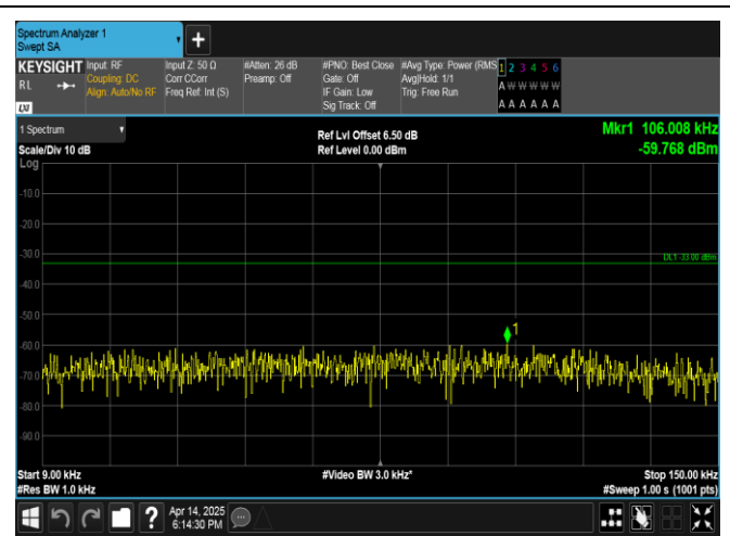
Band17-10MHz-16QAM-23800-50RB#0-0.009~0.15-PASS
