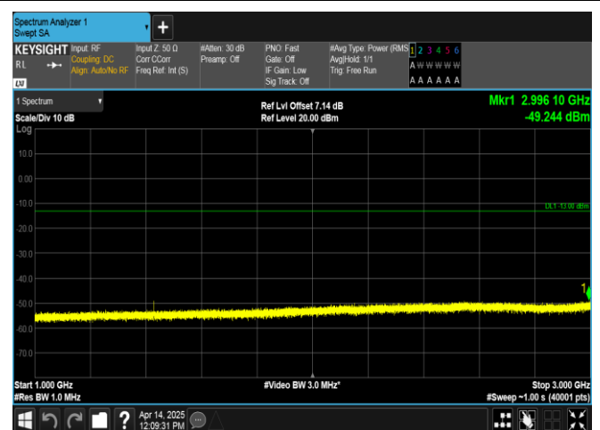
Band17-10MHz-QPSK-23790-1RB#49-1000~3000-PASS
