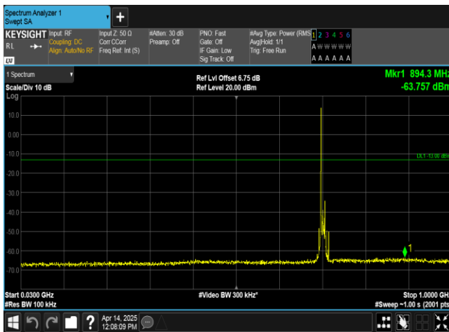
Band17-10MHz-16QAM-23790-1RB#0-30~1000-PASS
