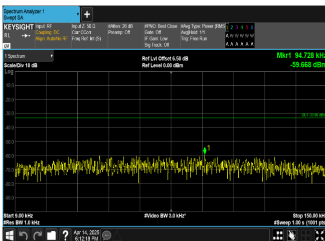
Band17-10MHz-16QAM-23790-50RB#0-0.009~0.15-PASS
