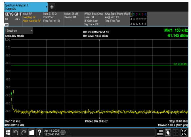
Band17-10MHz-16QAM-23780-1RB#49-0.15~30-PASS
