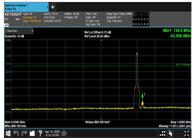
Band17-10MHz-16QAM-23780-50RB#0-30~1000-PASS
