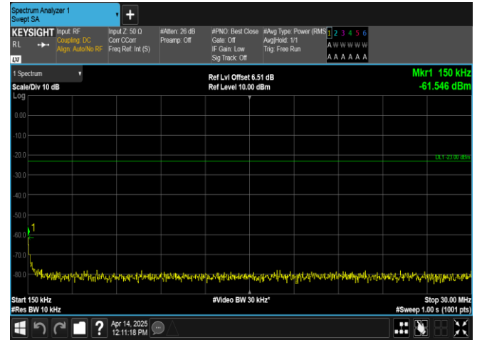
Band17-10MHz-QPSK-23800-1RB#0-0.15~30-PASS
