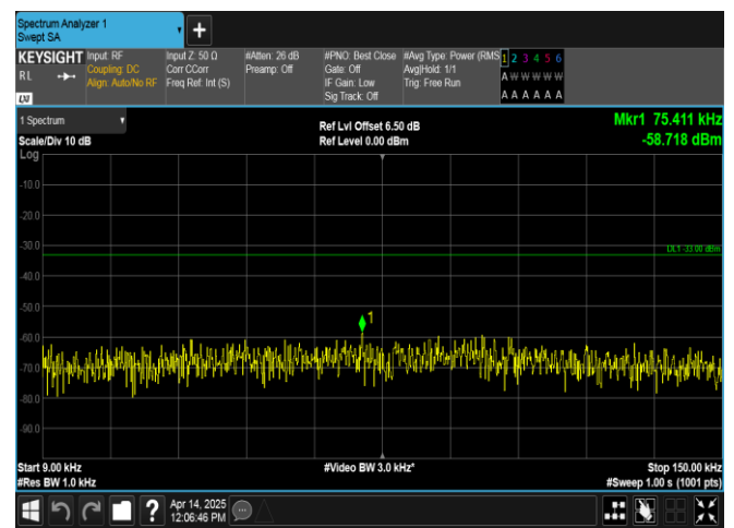
Band17-10MHz-QPSK-23790-1RB#0-0.009~0.15-PASS
