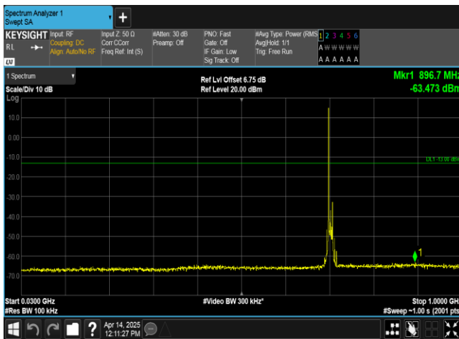
Band17-10MHz-QPSK-23800-1RB#0-30~1000-PASS
