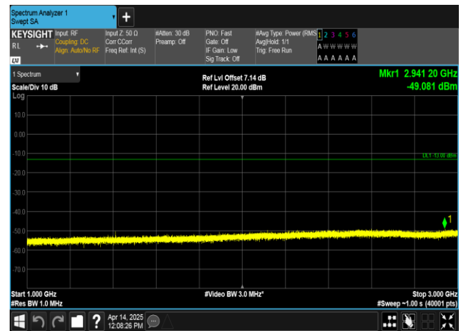
Band17-10MHz-16QAM-23790-1RB#0-1000~3000-PASS
