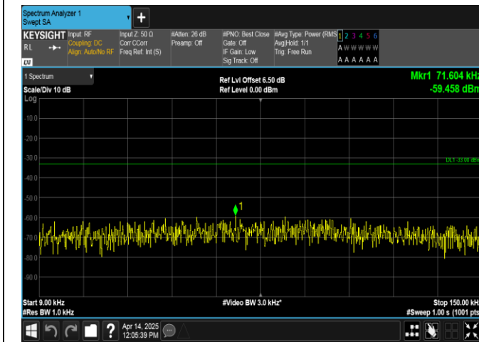
Band17-10MHz-16QAM-23780-1RB#49-0.009~0.15-PASS
