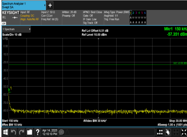
Band17-10MHz-16QAM-23790-1RB#49-0.15~30-PASS
