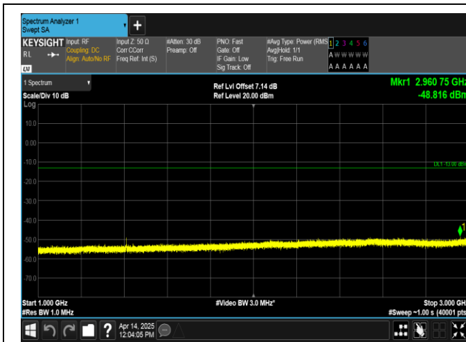
Band17-10MHz-16QAM-23780-1RB#0-1000~3000-PASS
