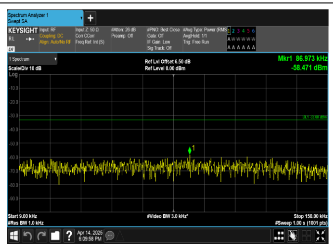
Band17-10MHz-16QAM-23780-50RB#0-0.009~0.15-PASS
