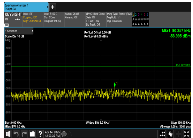
Band17-10MHz-16QAM-23780-1RB#0-0.009~0.15-PASS
