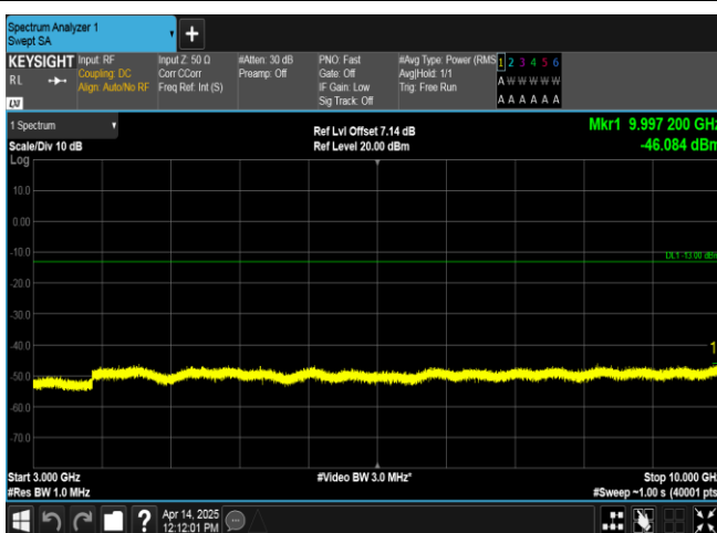
Band17-10MHz-QPSK-23800-1RB#0-3000~10000-PASS
