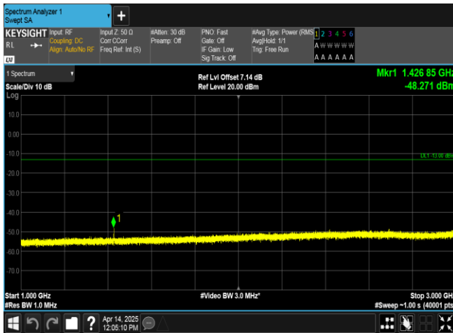
Band17-10MHz-QPSK-23780-1RB#49-1000~3000-PASS
