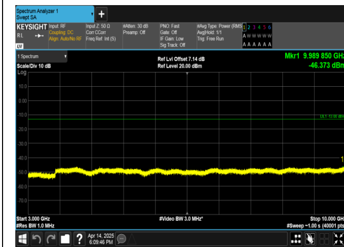
Band17-10MHz-QPSK-23780-50RB#0-3000~10000-PASS
