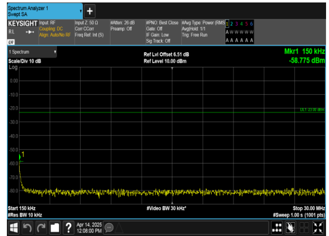
Band17-10MHz-16QAM-23790-1RB#0-0.15~30-PASS
