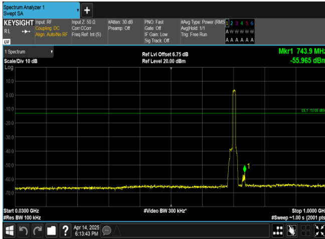
Band17-10MHz-QPSK-23800-50RB#0-30~1000-PASS
