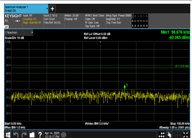
Band17-10MHz-QPSK-23800-1RB#49-0.009~0.15-PASS
