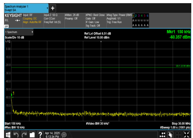
Band17-10MHz-QPSK-23800-50RB#0-0.15~30-PASS
