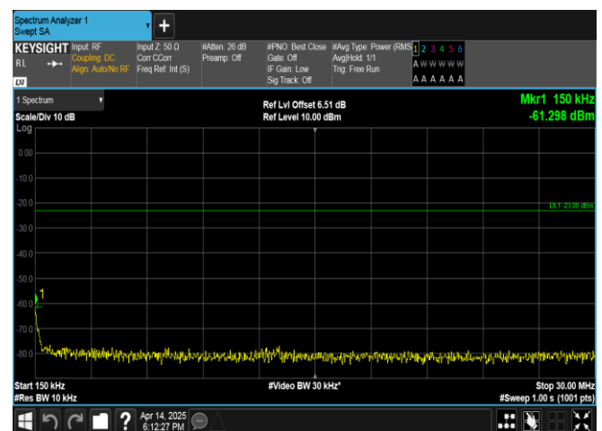
Band17-10MHz-16QAM-23790-50RB#0-0.15~30-PASS
