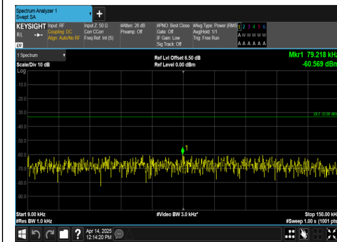
Band17-10MHz-16QAM-23800-1RB#49-0.009~0.15-PASS
