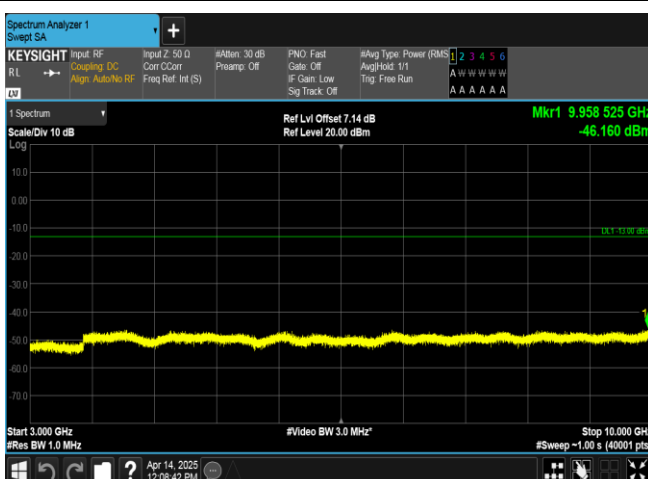
Band17-10MHz-16QAM-23790-1RB#0-3000~10000-PASS
