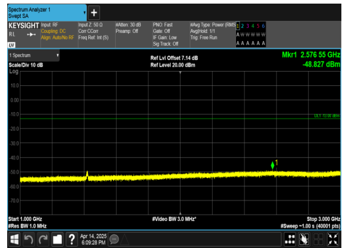
Band17-10MHz-QPSK-23780-50RB#0-1000~3000-PASS
