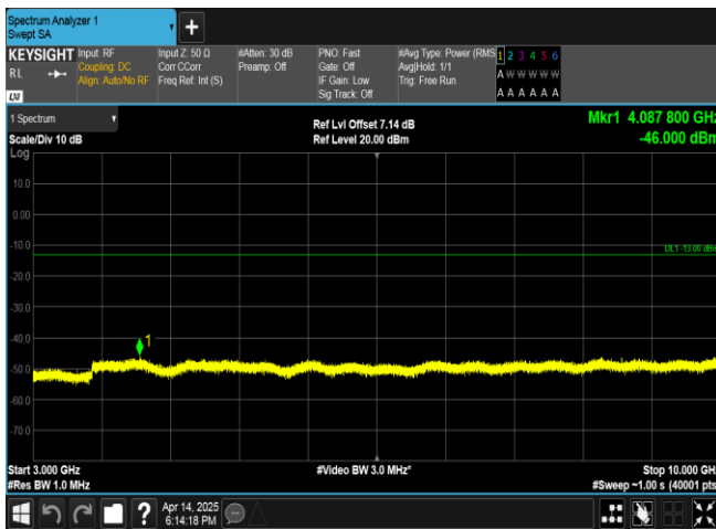
Band17-10MHz-QPSK-23800-50RB#0-3000~10000-PASS
