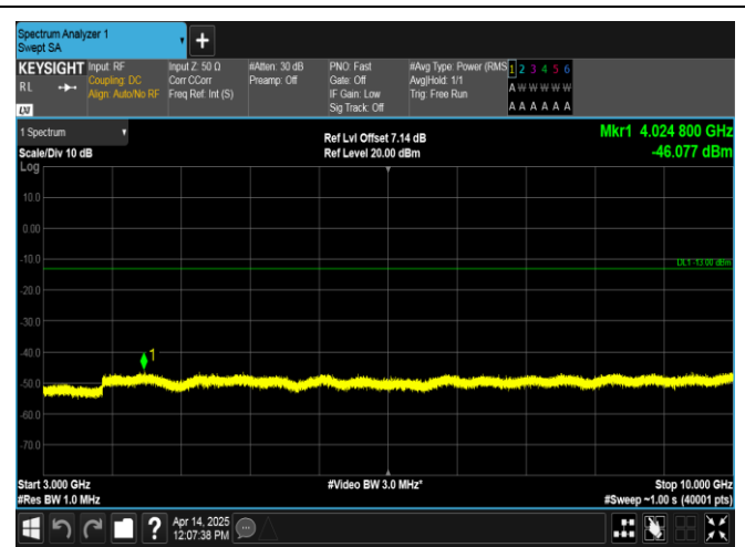
Band17-10MHz-QPSK-23790-1RB#0-3000~10000-PASS
