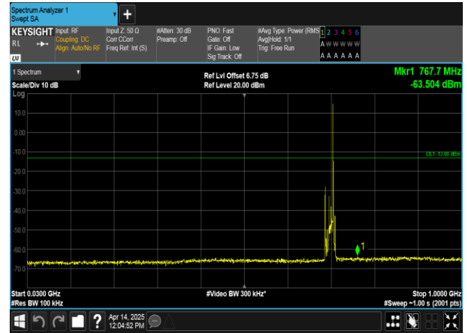
Band17-10MHz-QPSK-23780-1RB#49-30~1000-PASS
