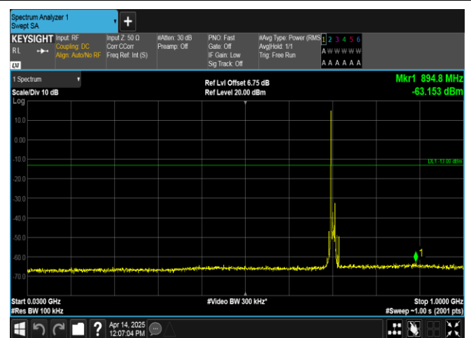
Band17-10MHz-QPSK-23790-1RB#0-30~1000-PASS
