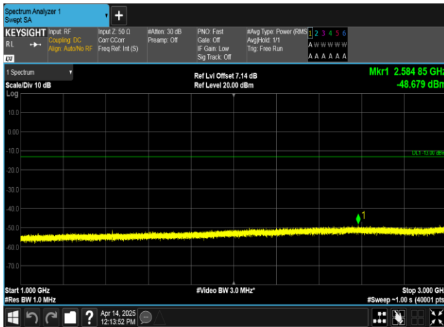
Band17-10MHz-QPSK-23800-1RB#49-1000~3000-PASS
