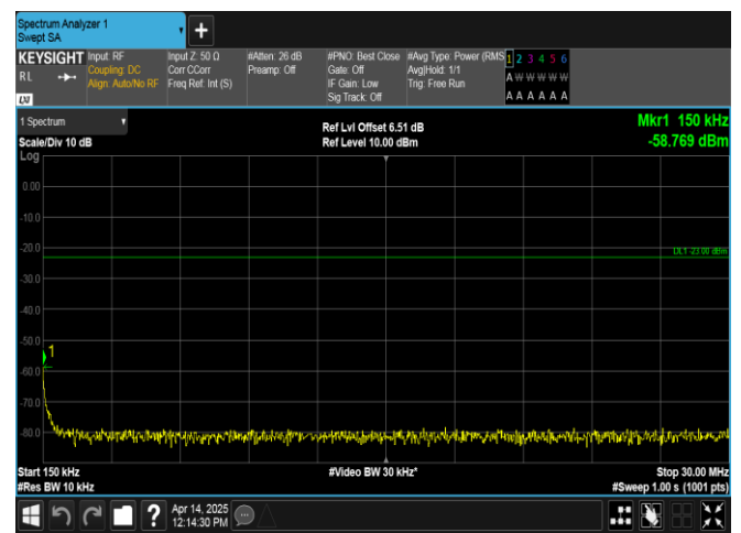
Band17-10MHz-16QAM-23800-1RB#49-0.15~30-PASS
