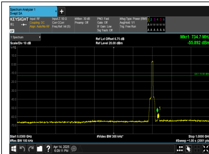
Band17-10MHz-QPSK-23780-50RB#0-30~1000-PASS
