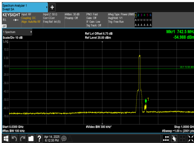
Band17-10MHz-16QAM-23790-50RB#0-30~1000-PASS
