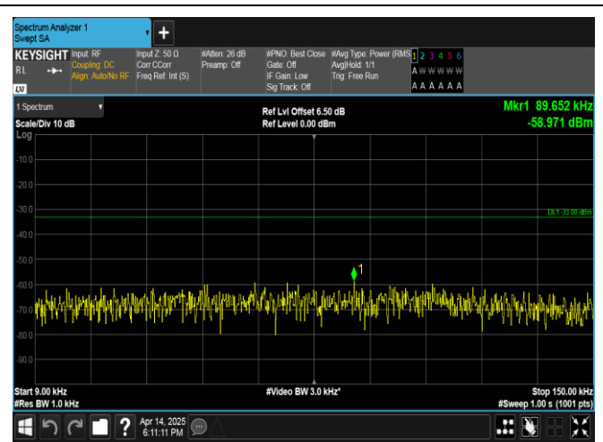
Band17-10MHz-QPSK-23790-50RB#0-0.009~0.15-PASS
