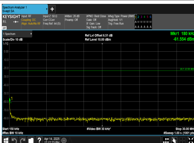
Band17-10MHz-16QAM-23800-1RB#0-0.15~30-PASS
