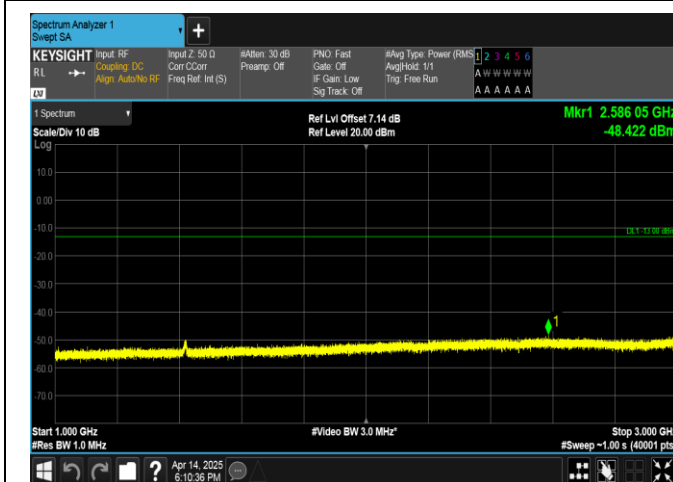
Band17-10MHz-16QAM-23780-50RB#0-1000~3000-PASS
