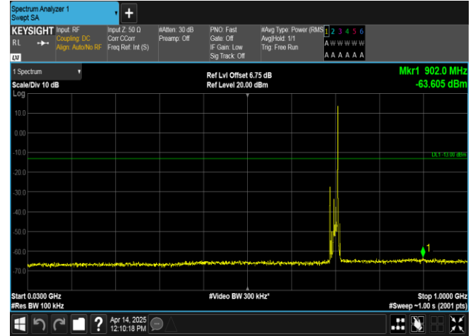
Band17-10MHz-16QAM-23790-1RB#49-30~1000-PASS
