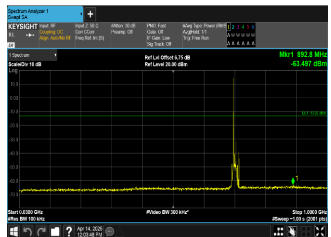
Band17-10MHz-16QAM-23780-1RB#0-30~1000-PASS
