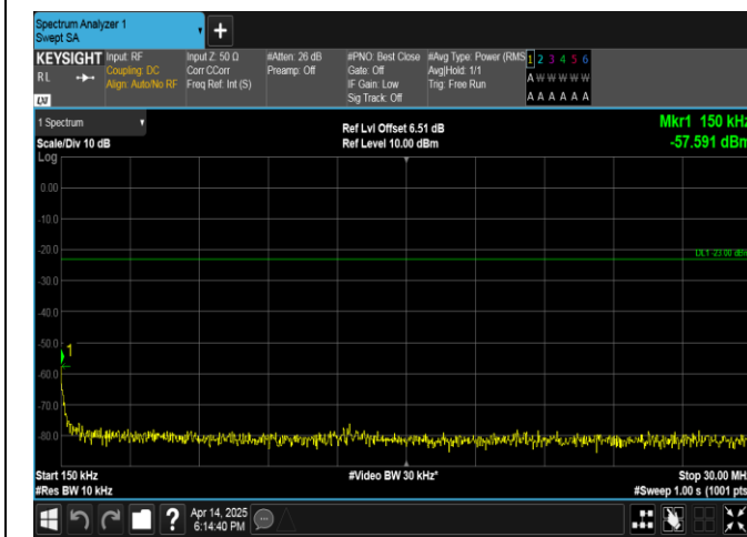
Band17-10MHz-16QAM-23800-50RB#0-0.15~30-PASS
