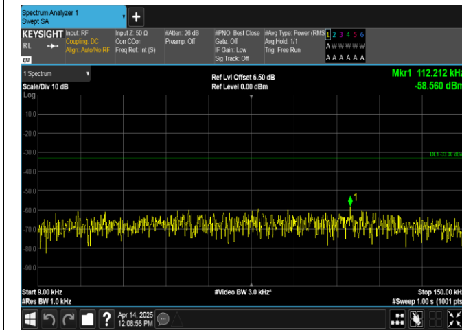
Band17-10MHz-QPSK-23790-1RB#49-0.009~0.15-PASS
