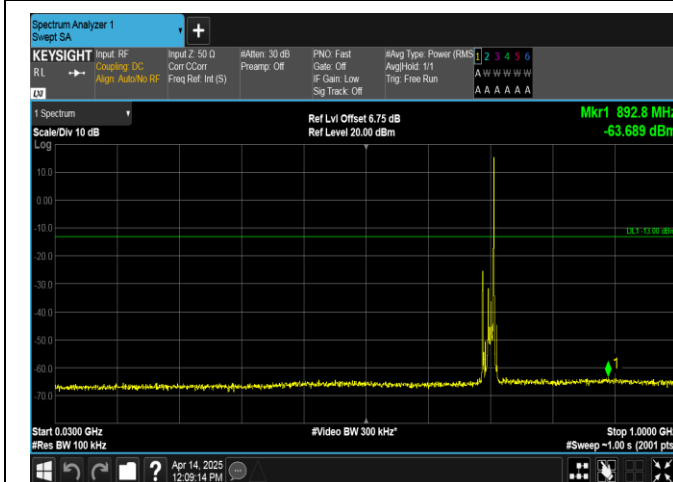
Band17-10MHz-QPSK-23790-1RB#49-30~1000-PASS
