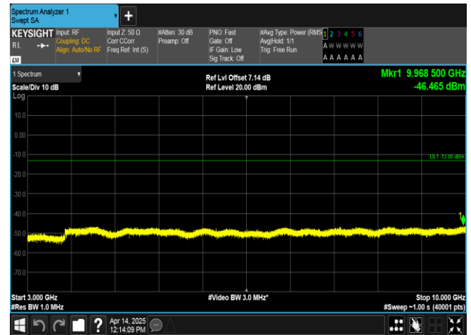
Band17-10MHz-QPSK-23800-1RB#49-3000~10000-PASS
