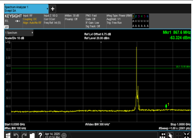
Band17-10MHz-16QAM-23800-1RB#0-30~1000-PASS
