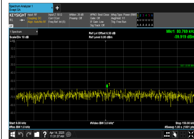
Band17-5MHz-16QAM-23825-1RB#24-0.009~0.15-PASS
