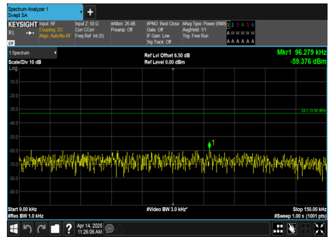
Band17-5MHz-QPSK-23790-25RB#0-0.009~0.15-PASS
