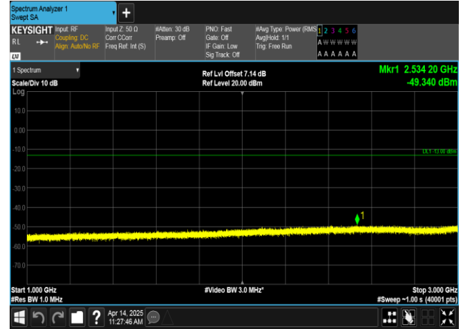
Band17-5MHz-16QAM-23790-25RB#0-1000~3000-PASS
