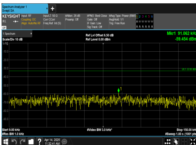
Band17-5MHz-QPSK-23825-25RB#0-0.009~0.15-PASS
