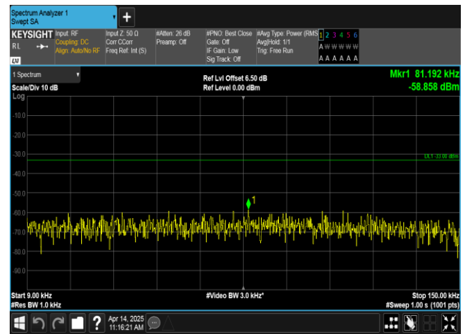
Band17-5MHz-16QAM-23755-1RB#0-0.009~0.15-PASS
