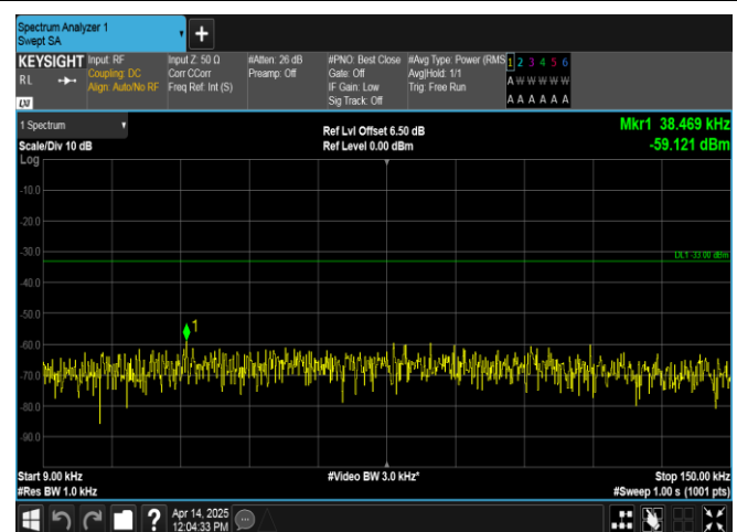
Band17-10MHz-QPSK-23780-1RB#49-0.009~0.15-PASS
