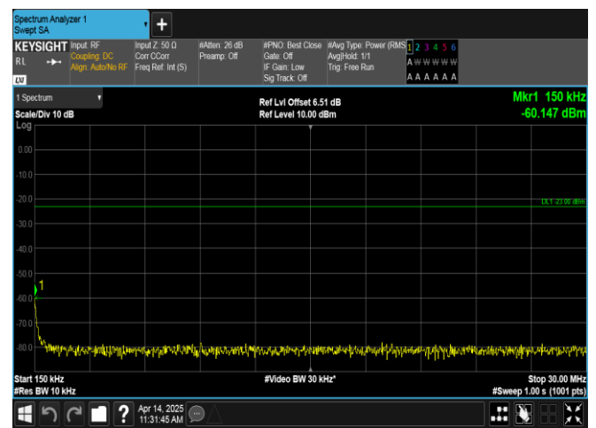
Band17-5MHz-16QAM-23825-1RB#24-0.15~30-PASS
