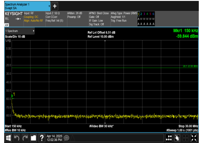
Band17-10MHz-QPSK-23780-1RB#0-0.15~30-PASS
