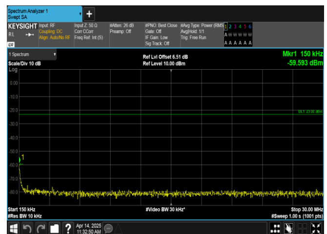
Band17-5MHz-QPSK-23825-25RB#0-0.15~30-PASS
