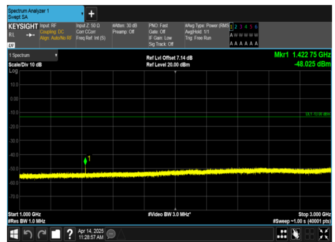
Band17-5MHz-QPSK-23825-1RB#0-1000~3000-PASS
