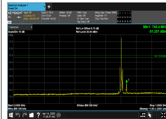
Band17-5MHz-QPSK-23825-1RB#0-30~1000-PASS
