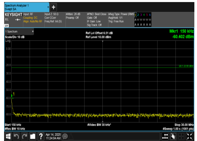
Band17-5MHz-QPSK-23790-1RB#24-0.15~30-PASS
