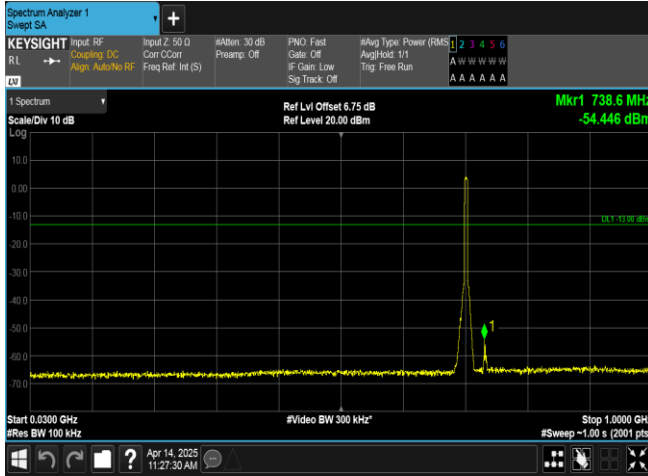
Band17-5MHz-16QAM-23790-25RB#0-30~1000-PASS
