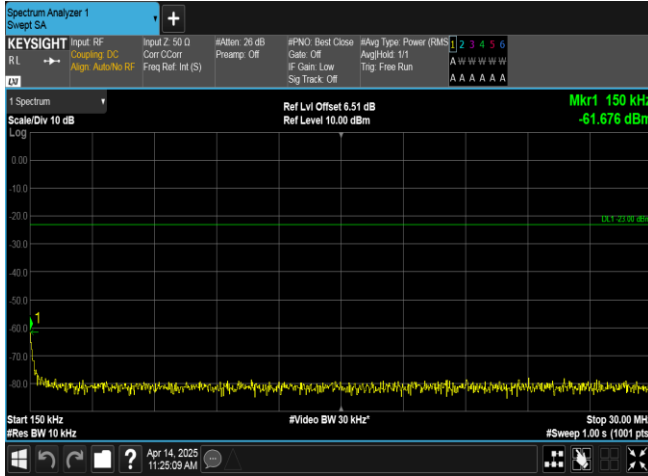
Band17-5MHz-16QAM-23790-1RB#24-0.15~30-PASS
