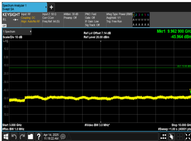
Band17-5MHz-16QAM-23755-1RB#24-3000~10000-PASS
