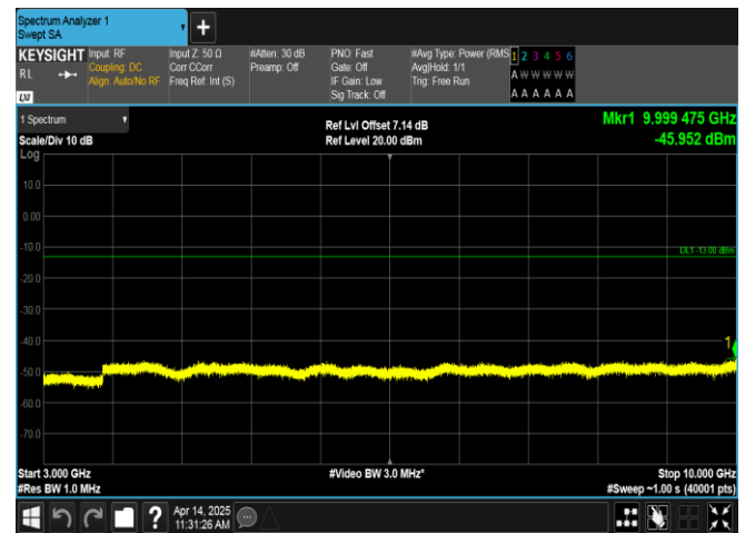
Band17-5MHz-QPSK-23825-1RB#24-3000~10000-PASS
