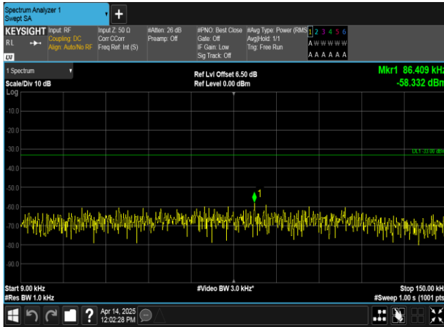
Band17-10MHz-QPSK-23780-1RB#0-0.009~0.15-PASS
