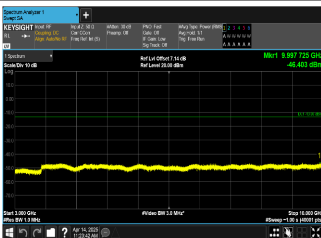
Band17-5MHz-16QAM-23790-1RB#0-3000~10000-PASS
