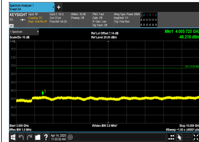
Band17-5MHz-QPSK-23825-25RB#0-3000~10000-PASS
