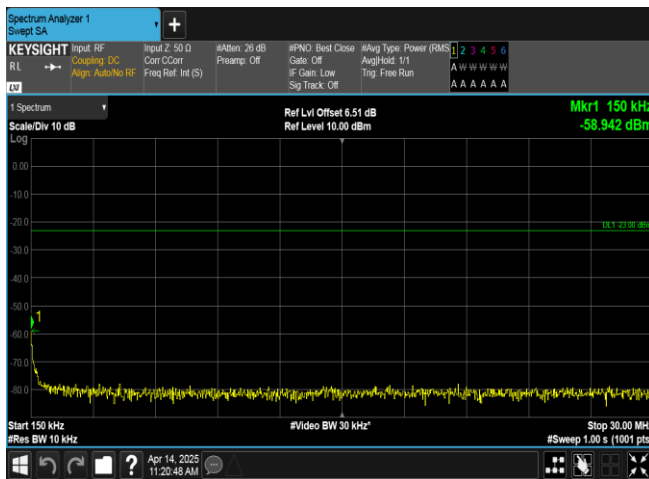
Band17-5MHz-16QAM-23755-25RB#0-0.15~30-PASS
