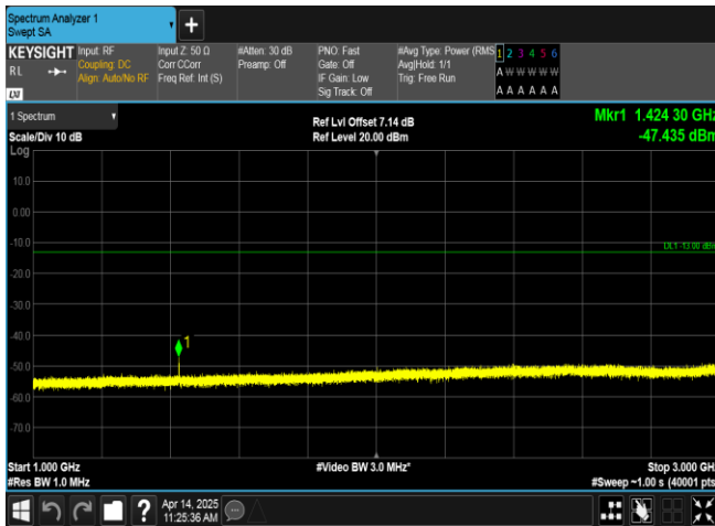
Band17-5MHz-16QAM-23790-1RB#24-1000~3000-PASS
