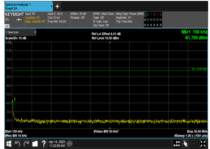
Band17-5MHz-16QAM-23790-1RB#0-0.15~30-PASS
