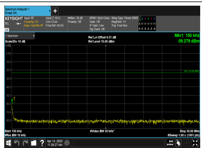
Band17-5MHz-QPSK-23825-1RB#0-0.15~30-PASS
