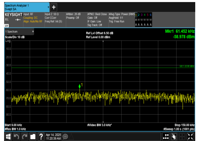
Band17-5MHz-16QAM-23755-25RB#0-0.009~0.15-PASS
