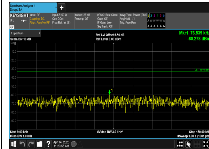
Band17-5MHz-QPSK-23790-1RB#24-0.009~0.15-PASS
