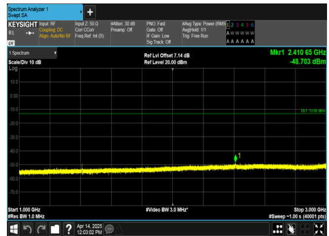
Band17-10MHz-QPSK-23780-1RB#0-1000~3000-PASS
