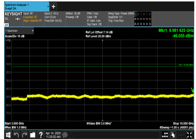
Band17-5MHz-16QAM-23790-1RB#24-3000~10000-PASS
