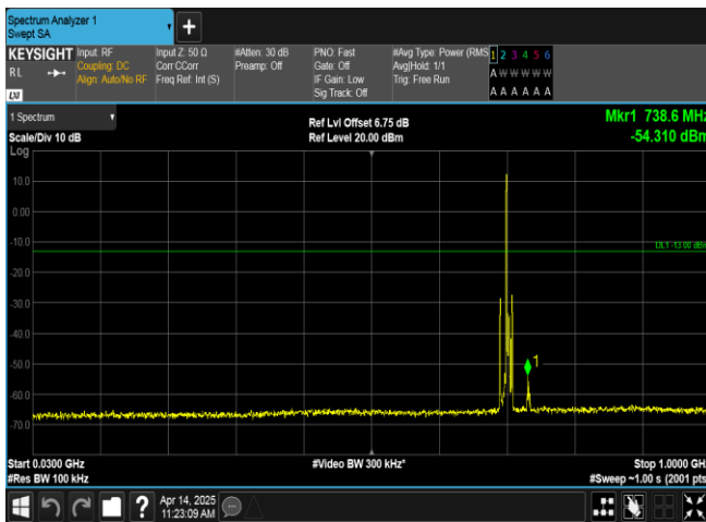
Band17-5MHz-16QAM-23790-1RB#0-30~1000-PASS
