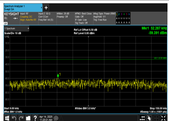
Band17-5MHz-16QAM-23790-1RB#24-0.009~0.15-PASS
