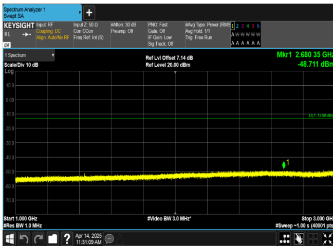
Band17-5MHz-QPSK-23825-1RB#24-1000~3000-PASS
