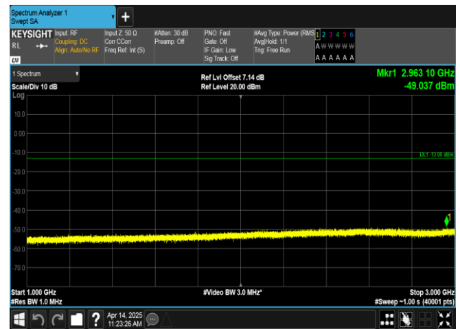
Band17-5MHz-16QAM-23790-1RB#0-1000~3000-PASS
