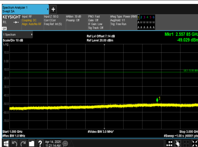
Band17-5MHz-16QAM-23755-25RB#0-1000~3000-PASS
