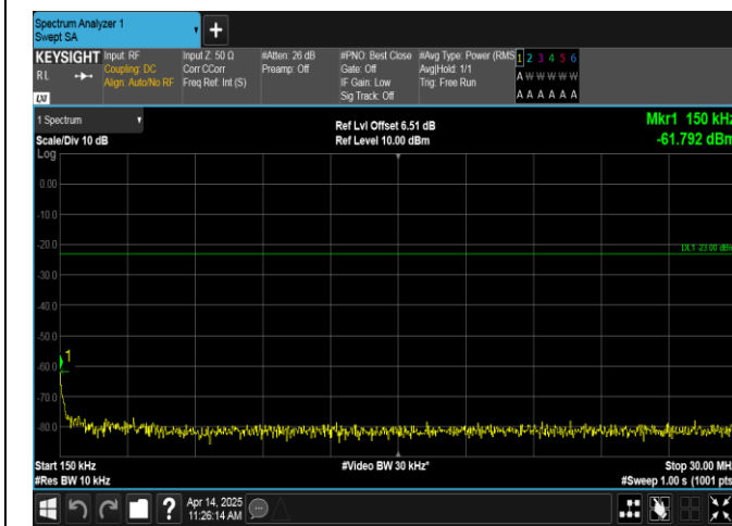
Band17-5MHz-QPSK-23790-25RB#0-0.15~30-PASS
