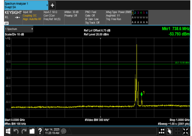
Band17-5MHz-16QAM-23790-1RB#24-30~1000-PASS
