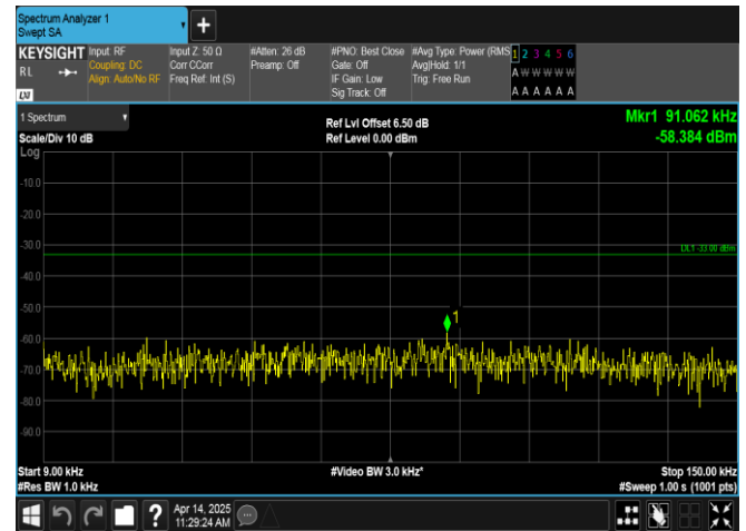
Band17-5MHz-16QAM-23825-1RB#0-0.009~0.15-PASS
