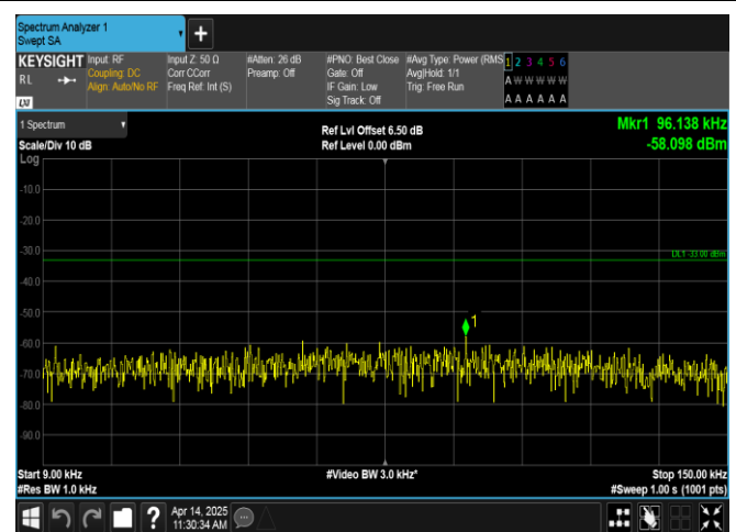
Band17-5MHz-QPSK-23825-1RB#24-0.009~0.15-PASS
