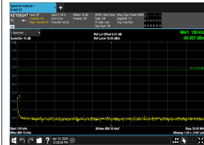
Band12-10MHz-16QAM-23095-1RB#49-0.15~30-PASS
