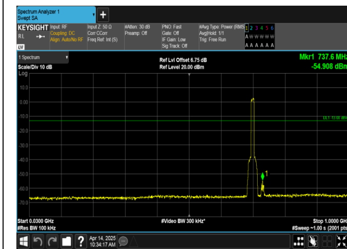
Band12-10MHz-16QAM-23095-50RB#0-30~1000-PASS
