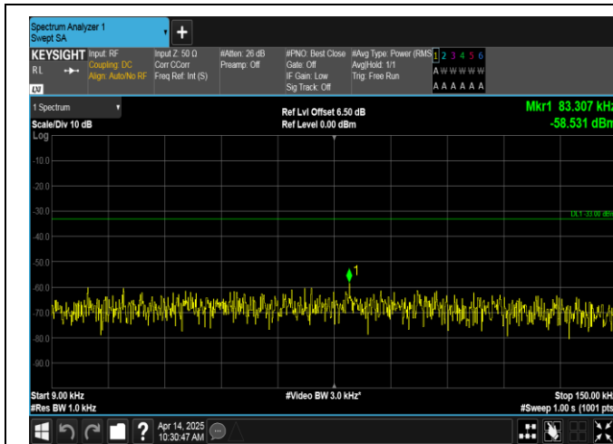
Band12-10MHz-QPSK-23060-50RB#0-0.009~0.15-PASS
