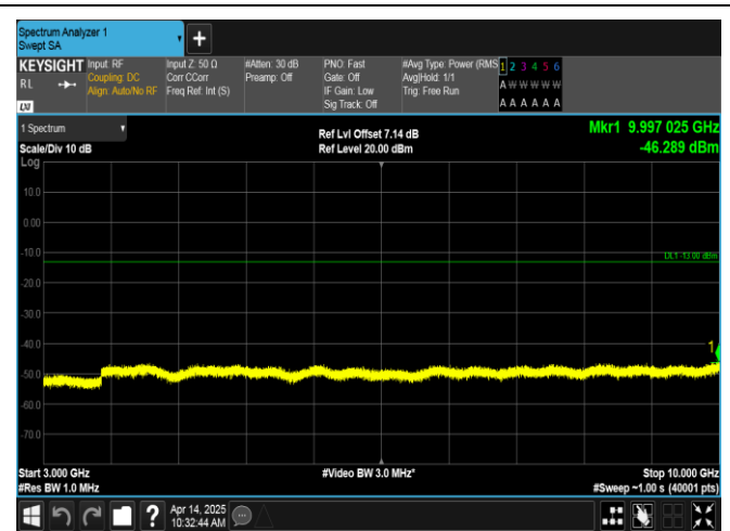
Band12-10MHz-16QAM-23060-50RB#0-3000~10000-PASS
