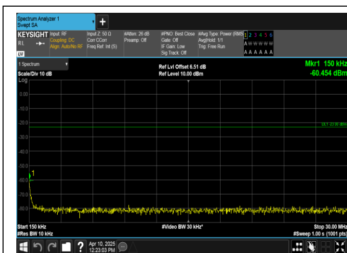
Band12-10MHz-16QAM-23060-1RB#0-0.15~30-PASS
