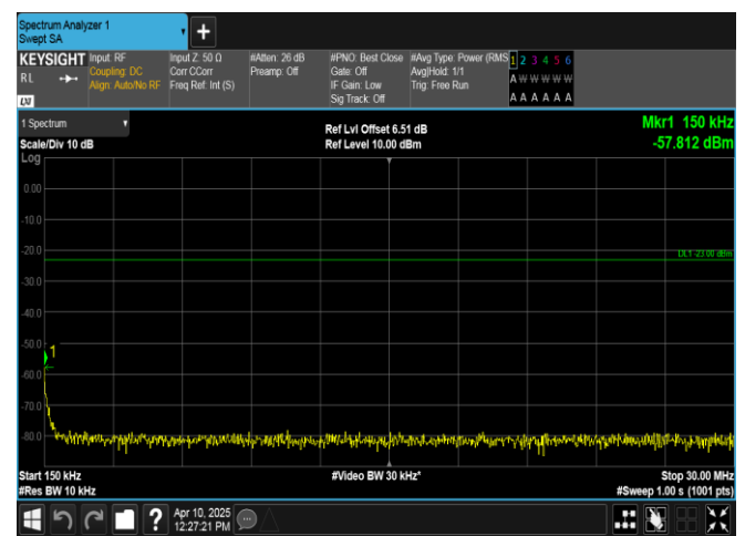
Band12-10MHz-16QAM-23095-1RB#0-0.15~30-PASS
