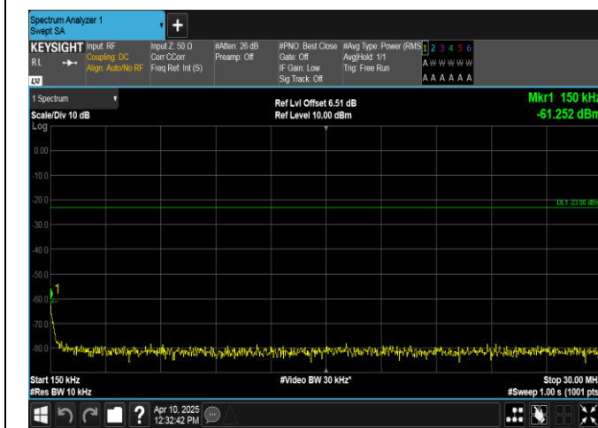
Band12-10MHz-QPSK-23130-1RB#49-0.15~30-PASS
