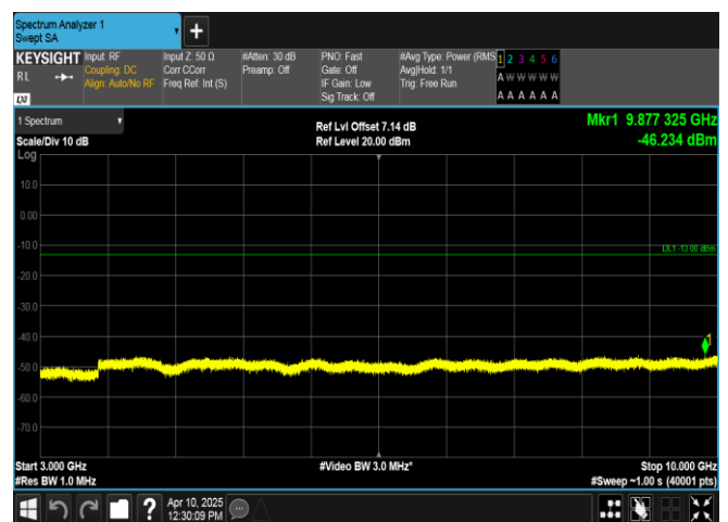
Band12-10MHz-16QAM-23095-1RB#49-3000~10000-PASS
