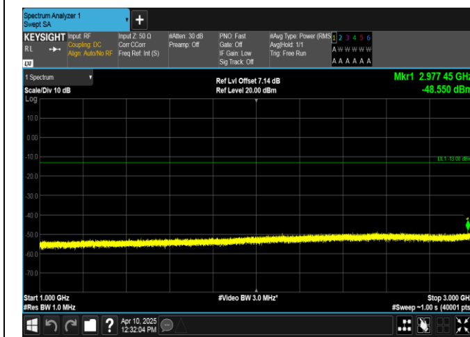
Band12-10MHz-16QAM-23130-1RB#0-1000~3000-PASS
