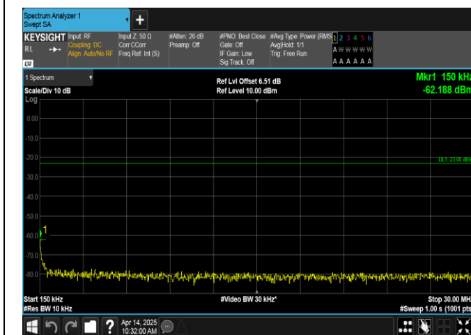
Band12-10MHz-16QAM-23060-50RB#0-0.15~30-PASS
