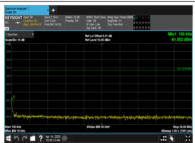
Band12-10MHz-QPSK-23130-50RB#0-0.15~30-PASS
