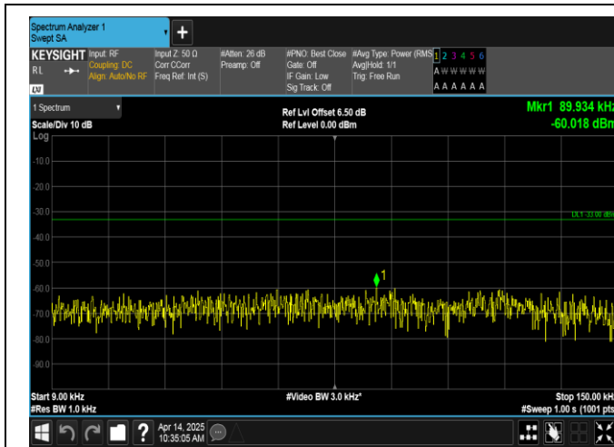
Band12-10MHz-QPSK-23130-50RB#0-0.009~0.15-PASS
