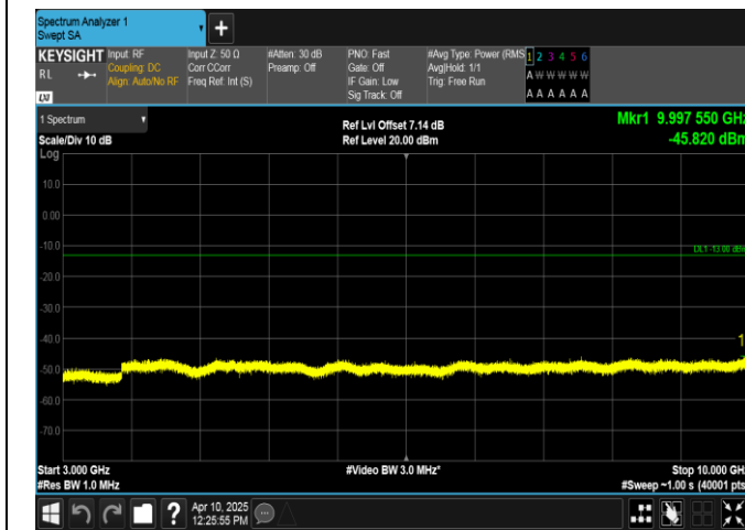
Band12-10MHz-16QAM-23060-1RB#49-3000~10000-PASS
