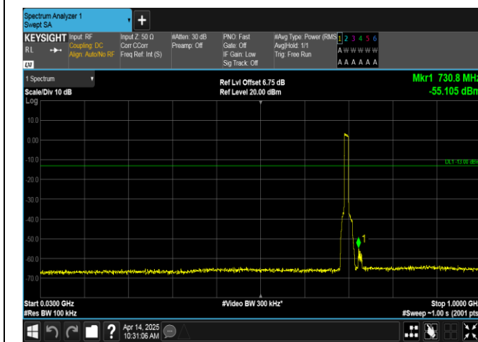
Band12-10MHz-QPSK-23060-50RB#0-30~1000-PASS
