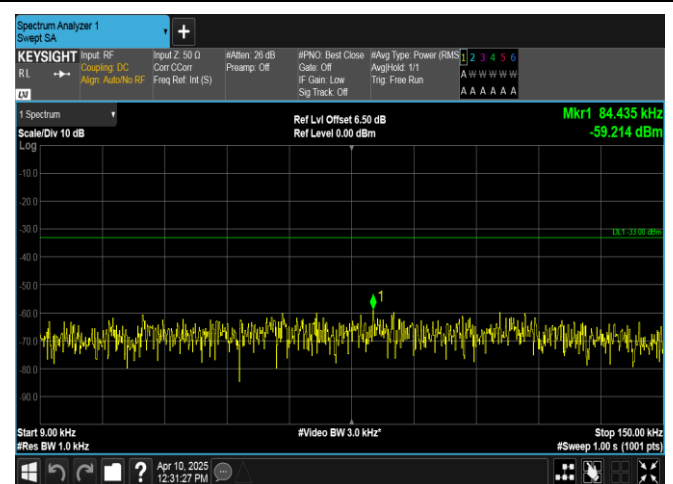
Band12-10MHz-16QAM-23130-1RB#0-0.009~0.15-PASS
