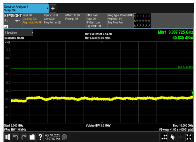
Band12-10MHz-QPSK-23095-1RB#0-3000~10000-PASS
