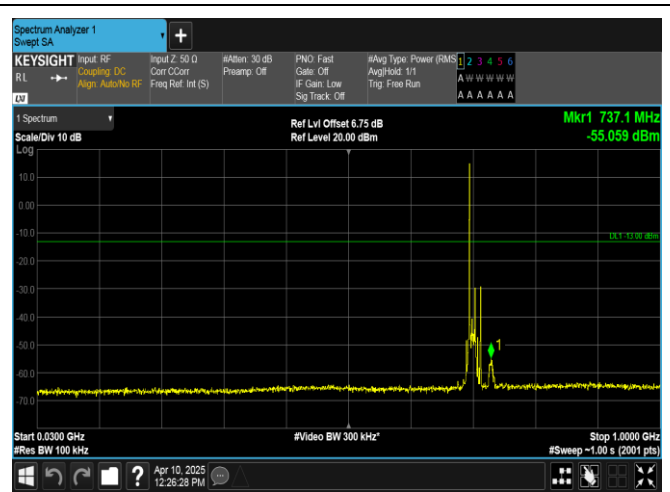
Band12-10MHz-QPSK-23095-1RB#0-30~1000-PASS
