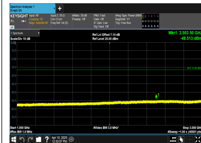
Band12-10MHz-QPSK-23130-1RB#49-1000~3000-PASS
