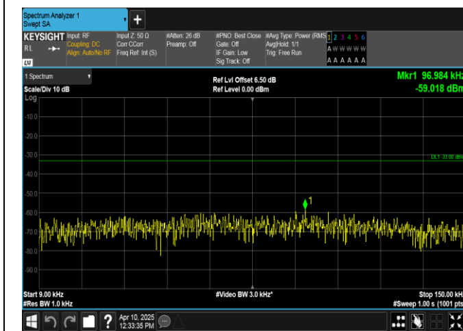
Band12-10MHz-16QAM-23130-1RB#49-0.009~0.15-PASS
