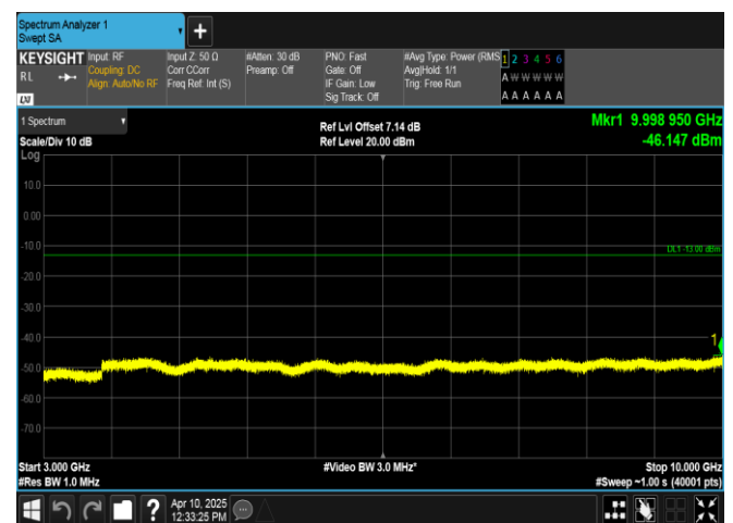
Band12-10MHz-QPSK-23130-1RB#49-3000~10000-PASS
