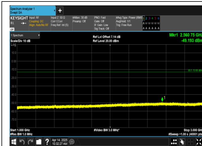
Band12-10MHz-16QAM-23060-50RB#0-1000~3000-PASS
