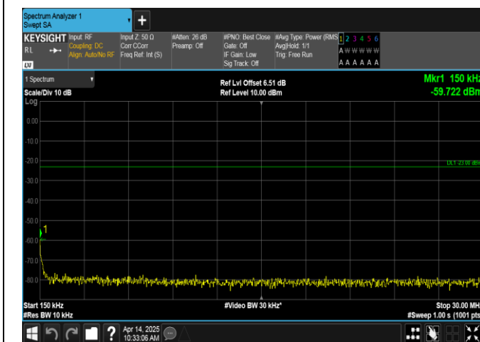
Band12-10MHz-QPSK-23095-50RB#0-0.15~30-PASS
