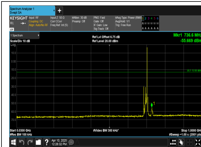
Band12-10MHz-QPSK-23095-1RB#49-30~1000-PASS
