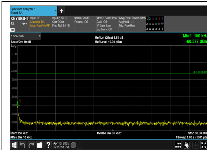
Band12-10MHz-QPSK-23095-1RB#0-0.15~30-PASS
