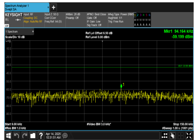
Band12-10MHz-16QAM-23060-50RB#0-0.009~0.15-PASS
