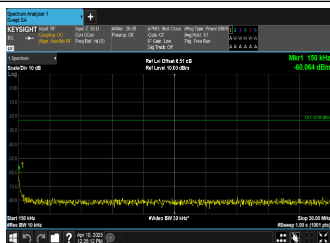
Band12-10MHz-16QAM-23060-1RB#49-0.15~30-PASS
