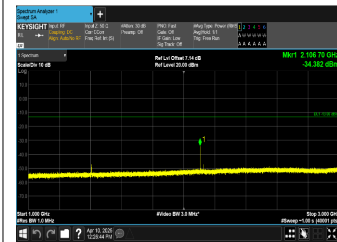
Band12-10MHz-QPSK-23095-1RB#0-1000~3000-PASS
