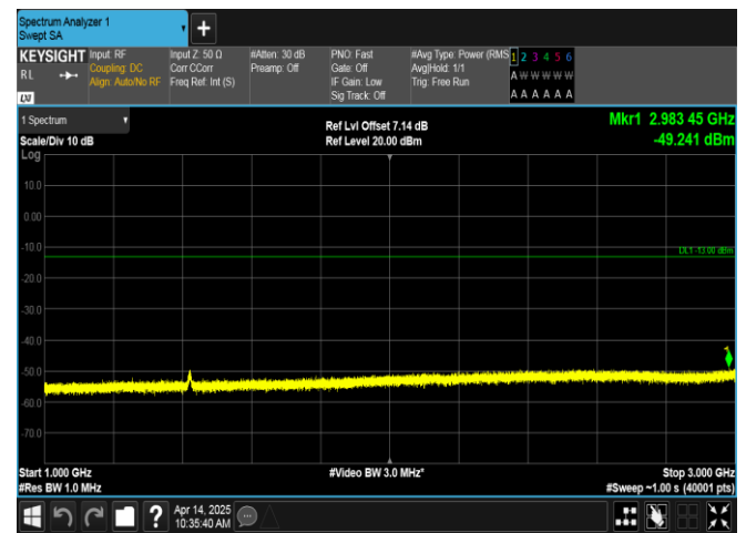
Band12-10MHz-QPSK-23130-50RB#0-1000~3000-PASS
