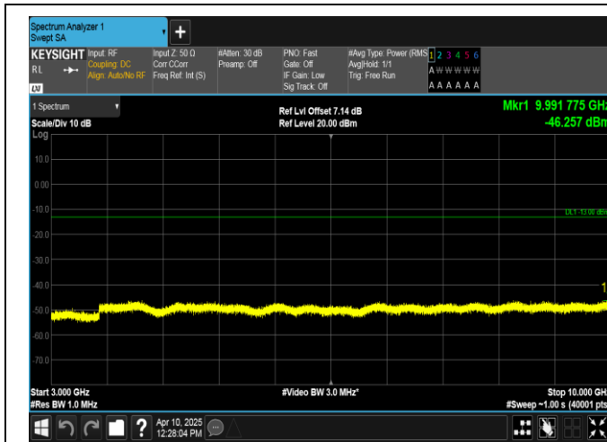
Band12-10MHz-16QAM-23095-1RB#0-3000~10000-PASS
