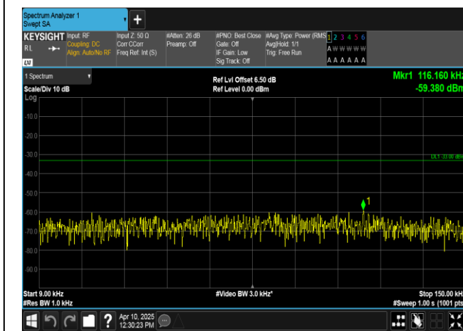
Band12-10MHz-QPSK-23130-1RB#0-0.009~0.15-PASS
