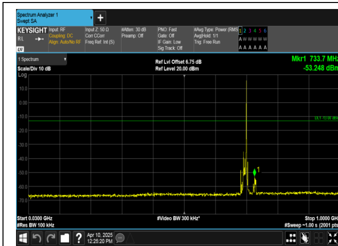
Band12-10MHz-16QAM-23060-1RB#49-30~1000-PASS
