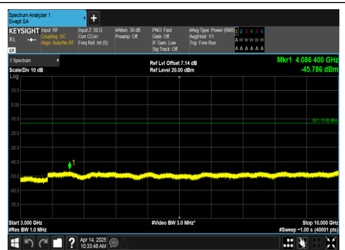
Band12-10MHz-QPSK-23095-50RB#0-3000~10000-PASS
