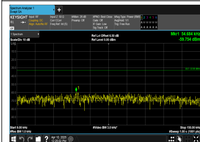
Band12-10MHz-16QAM-23060-1RB#49-0.009~0.15-PASS
