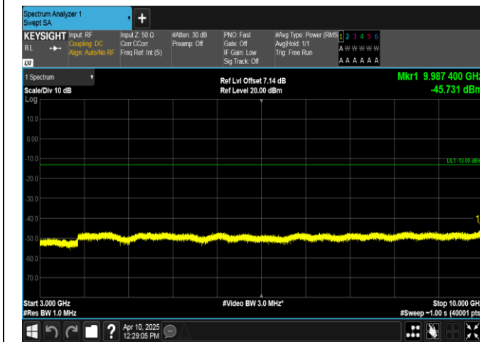
Band12-10MHz-QPSK-23095-1RB#49-3000~10000-PASS
