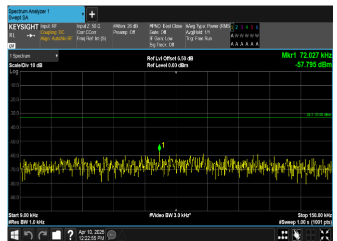
Band12-10MHz-16QAM-23060-1RB#0-0.009~0.15-PASS
