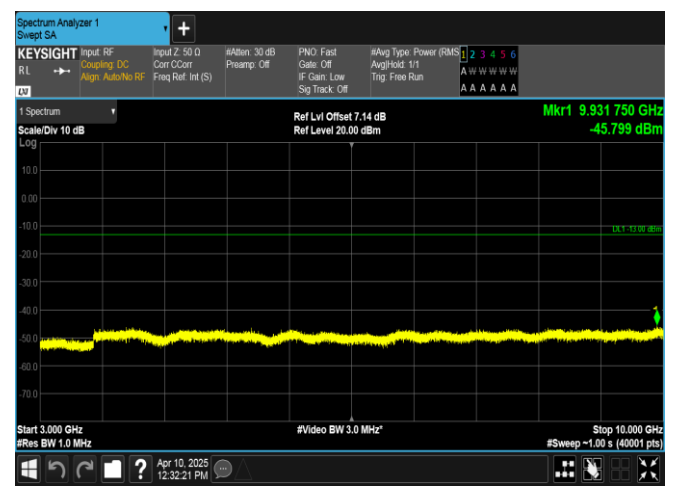
Band12-10MHz-16QAM-23130-1RB#0-3000~10000-PASS
