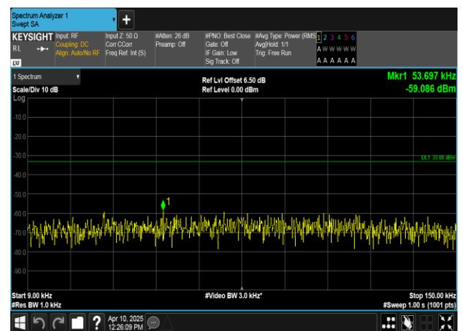
Band12-10MHz-QPSK-23095-1RB#0-0.009~0.15-PASS
