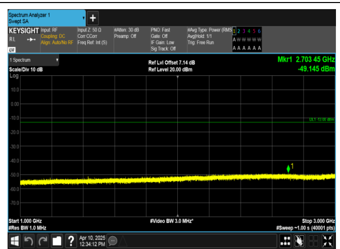
Band12-10MHz-16QAM-23130-1RB#49-1000~3000-PASS
