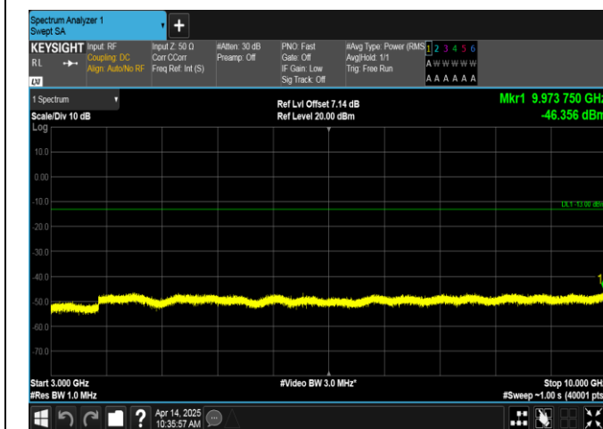
Band12-10MHz-QPSK-23130-50RB#0-3000~10000-PASS
