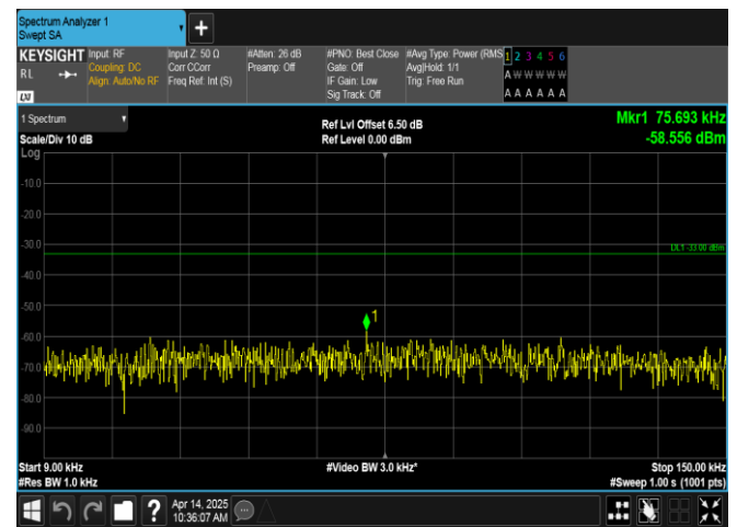
Band12-10MHz-16QAM-23130-50RB#0-0.009~0.15-PASS
