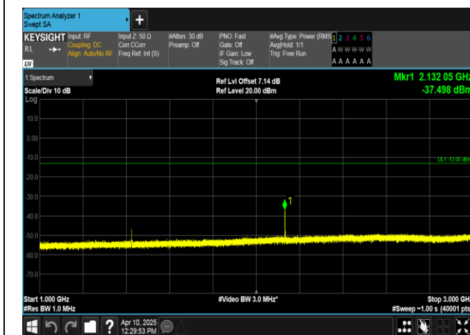
Band12-10MHz-16QAM-23095-1RB#49-1000~3000-PASS
