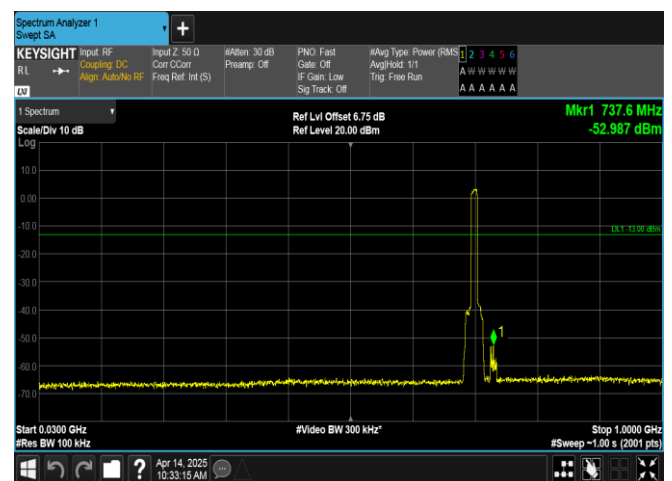
Band12-10MHz-QPSK-23095-50RB#0-30~1000-PASS
