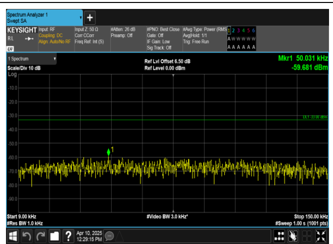
Band12-10MHz-16QAM-23095-1RB#49-0.009~0.15-PASS
