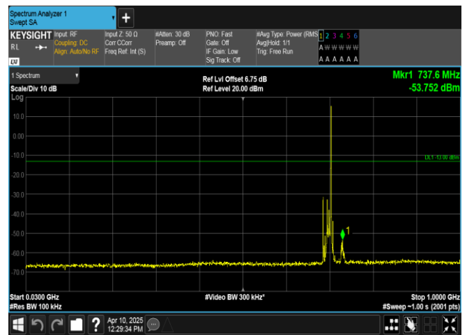
Band12-10MHz-16QAM-23095-1RB#49-30~1000-PASS
