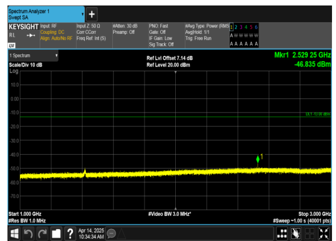
Band12-10MHz-16QAM-23095-50RB#0-1000~3000-PASS
