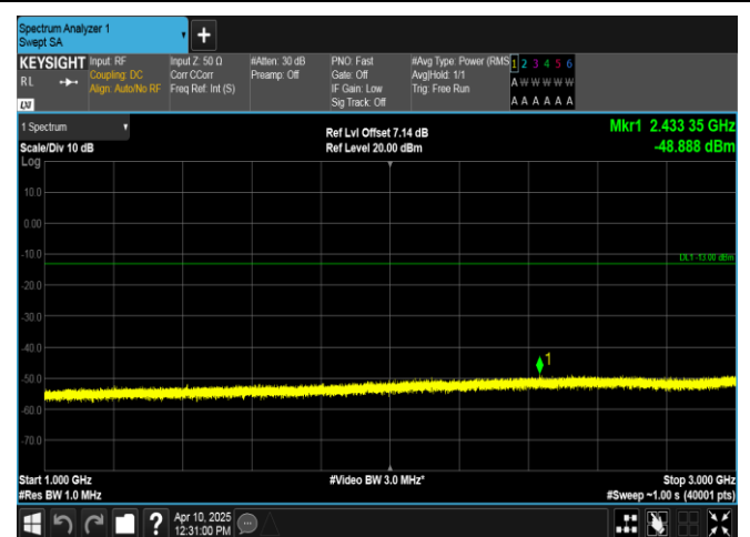
Band12-10MHz-QPSK-23130-1RB#0-1000~3000-PASS
