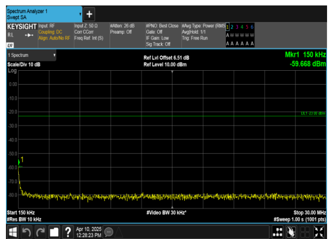
Band12-10MHz-QPSK-23095-1RB#49-0.15~30-PASS
