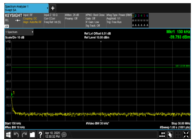
Band12-10MHz-QPSK-23130-1RB#0-0.15~30-PASS
