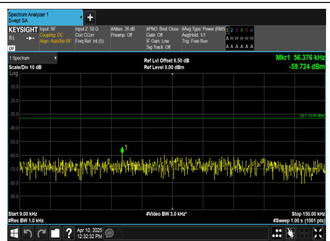
Band12-10MHz-QPSK-23130-1RB#49-0.009~0.15-PASS
