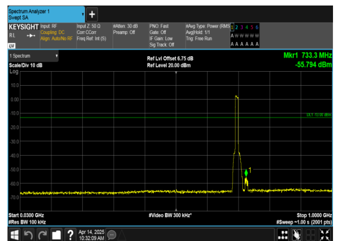
Band12-10MHz-16QAM-23060-50RB#0-30~1000-PASS
