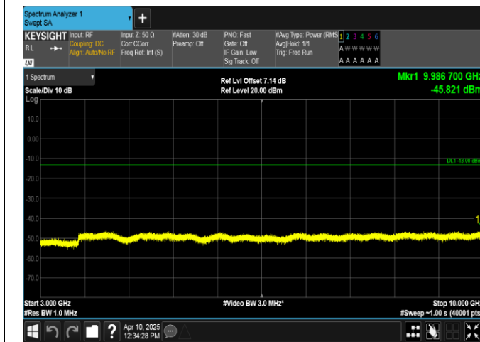
Band12-10MHz-16QAM-23130-1RB#49-3000~10000-PASS
