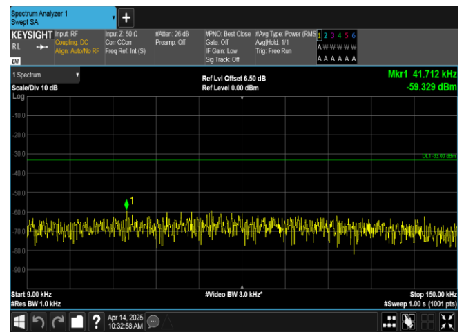
Band12-10MHz-QPSK-23095-50RB#0-0.009~0.15-PASS
