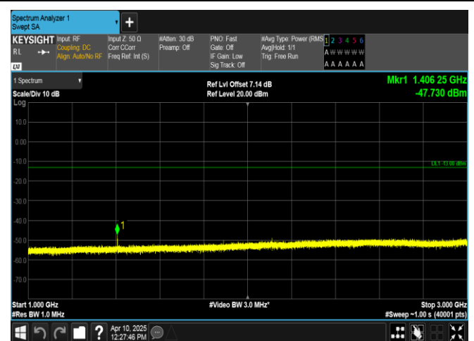
Band12-10MHz-16QAM-23095-1RB#0-1000~3000-PASS
