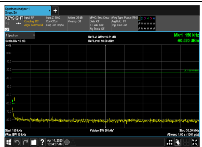
Band12-10MHz-16QAM-23095-50RB#0-0.15~30-PASS
