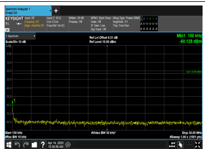
Band12-10MHz-QPSK-23060-50RB#0-0.15~30-PASS
