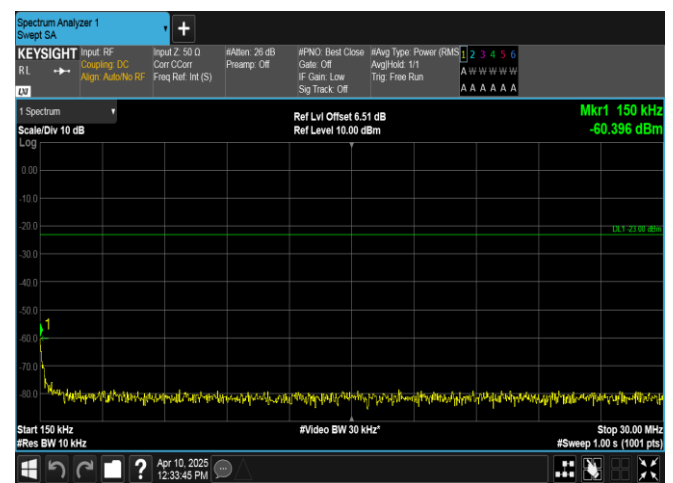
Band12-10MHz-16QAM-23130-1RB#49-0.15~30-PASS
