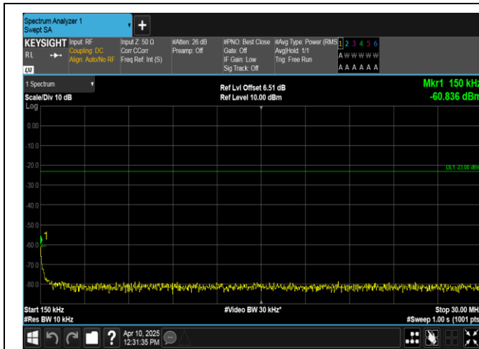
Band12-10MHz-16QAM-23130-1RB#0-0.15~30-PASS
