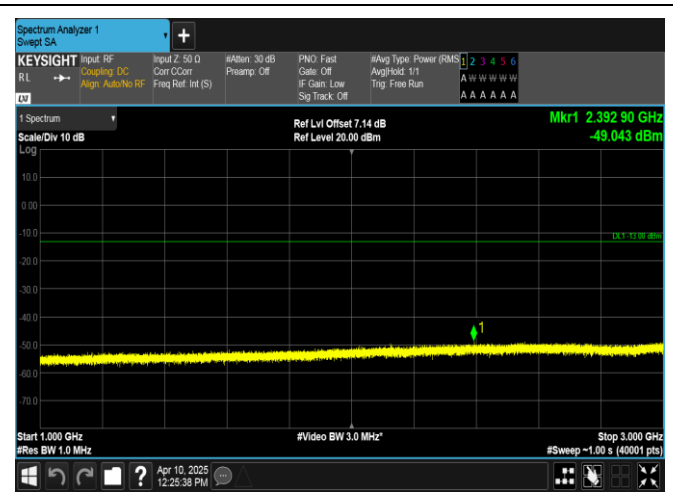
Band12-10MHz-16QAM-23060-1RB#49-1000~3000-PASS
