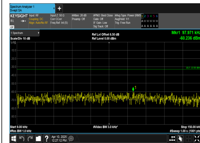
Band12-10MHz-16QAM-23095-1RB#0-0.009~0.15-PASS
