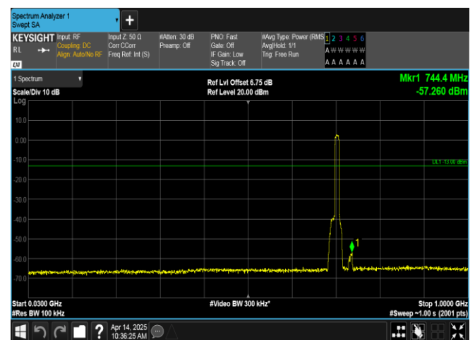
Band12-10MHz-16QAM-23130-50RB#0-30~1000-PASS
