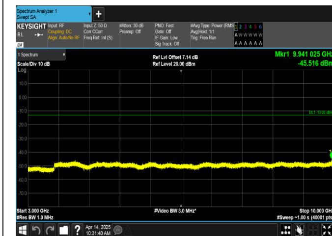
Band12-10MHz-QPSK-23060-50RB#0-3000~10000-PASS
