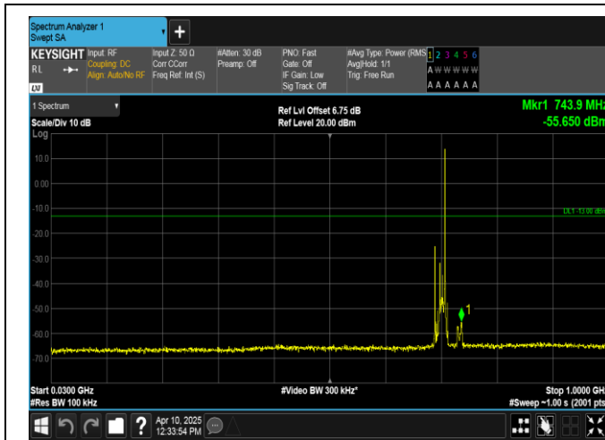
Band12-10MHz-16QAM-23130-1RB#49-30~1000-PASS
