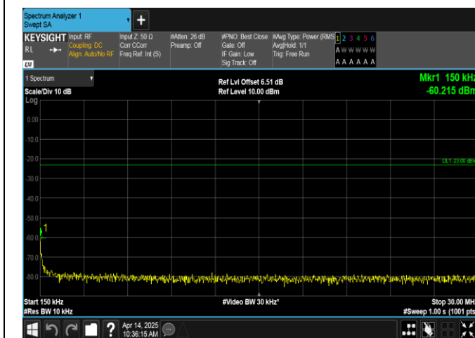
Band12-10MHz-16QAM-23130-50RB#0-0.15~30-PASS
