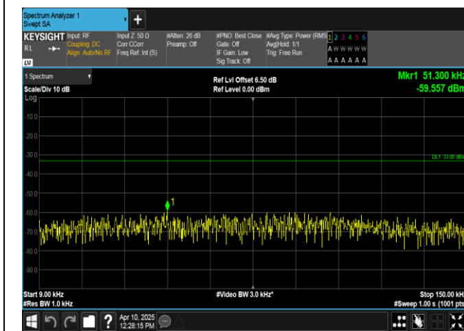
Band12-10MHz-QPSK-23095-1RB#49-0.009~0.15-PASS
