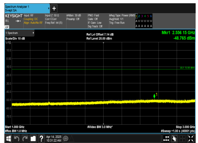
Band12-10MHz-QPSK-23060-50RB#0-1000~3000-PASS
