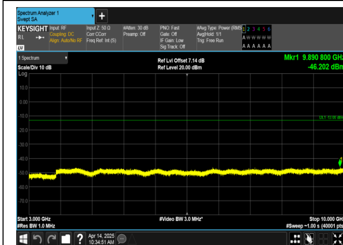
Band12-10MHz-16QAM-23095-50RB#0-3000~10000-PASS
