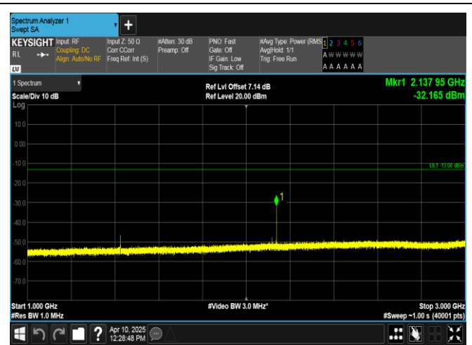
Band12-10MHz-QPSK-23095-1RB#49-1000~3000-PASS
