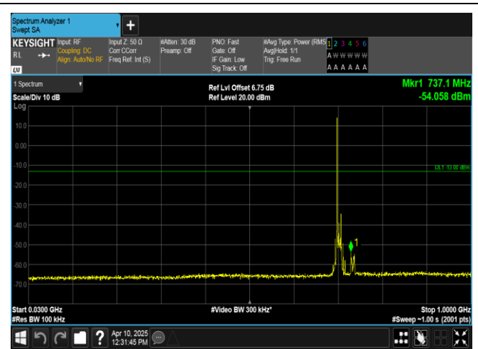
Band12-10MHz-16QAM-23130-1RB#0-30~1000-PASS
