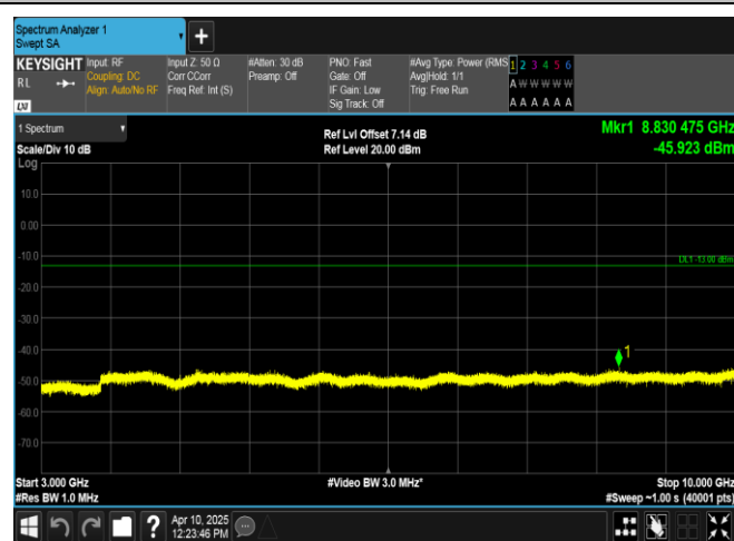
Band12-10MHz-16QAM-23060-1RB#0-3000~10000-PASS
