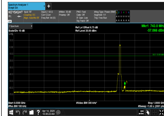
Band12-10MHz-QPSK-23130-50RB#0-30~1000-PASS
