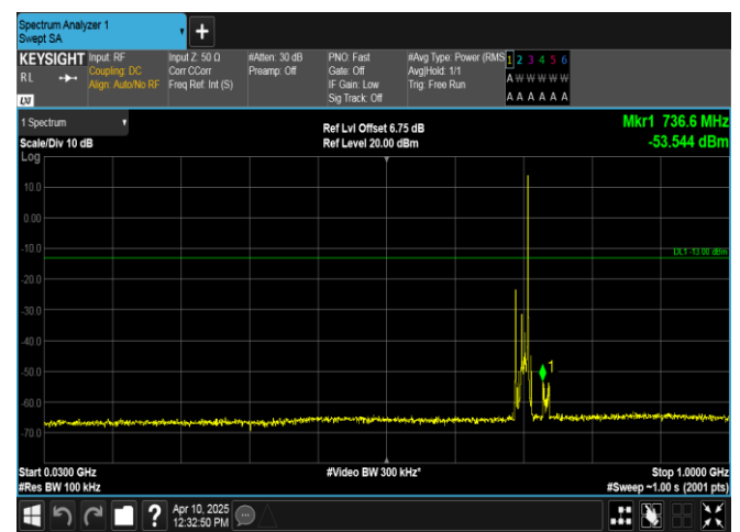
Band12-10MHz-QPSK-23130-1RB#49-30~1000-PASS
