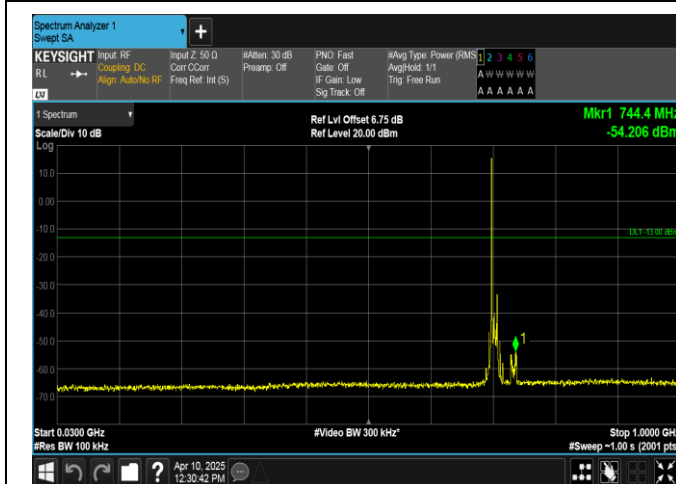
Band12-10MHz-QPSK-23130-1RB#0-30~1000-PASS
