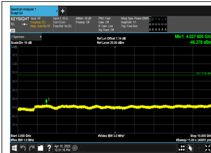
Band12-10MHz-QPSK-23130-1RB#0-3000~10000-PASS
