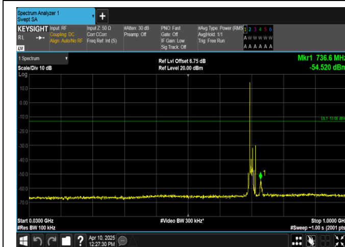
Band12-10MHz-16QAM-23095-1RB#0-30~1000-PASS
