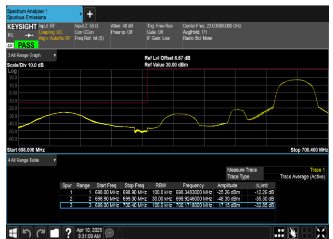
Band12-1.4MHz-16QAM-23017-1RB#5-PASS
