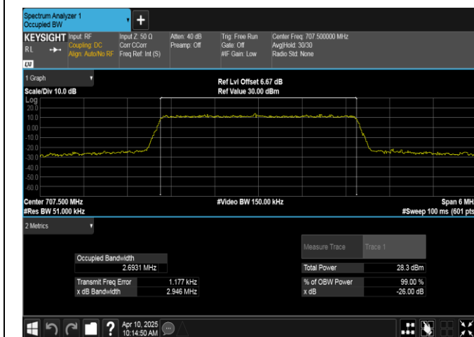
Band12-3MHz-16QAM-23095-15RB#0-PASS
