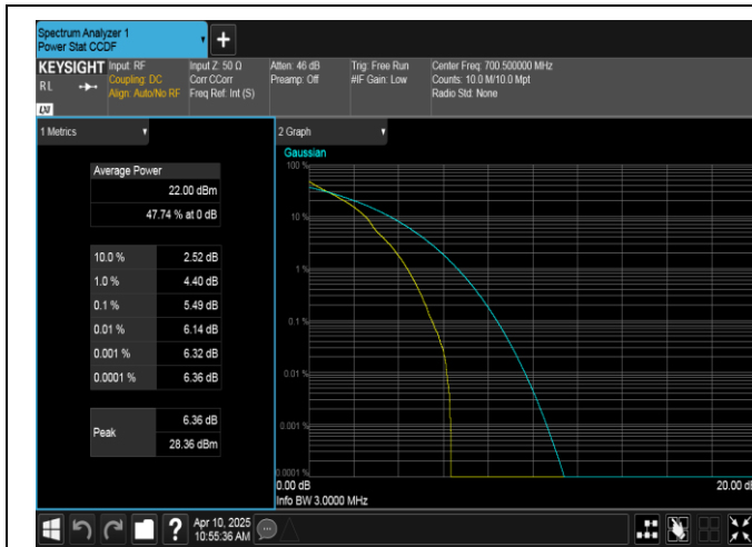
Band12-3MHz-QPSK-23025-1RB#0-PASS
