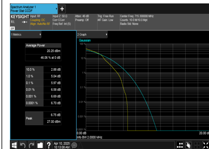
Band12-1.4MHz-16QAM-23173-1RB#0-PASS
