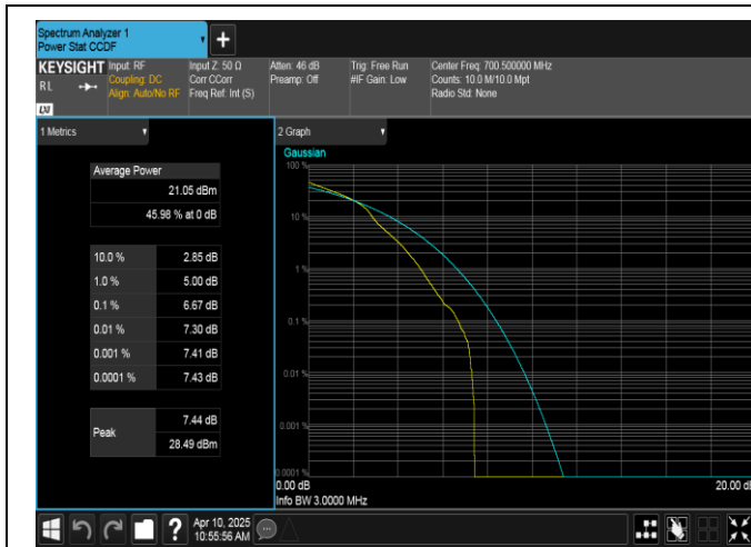
Band12-3MHz-16QAM-23025-1RB#0-PASS
