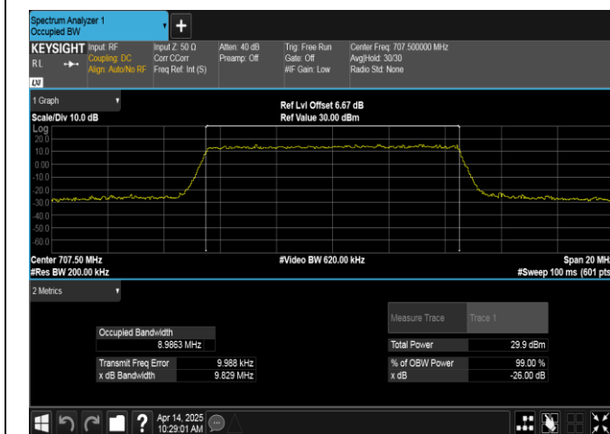
Band12-10MHz-16QAM-23095-50RB#0-PASS
