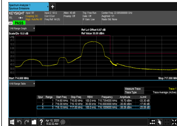
Band12-1.4MHz-QPSK-23173-1RB#5-PASS
