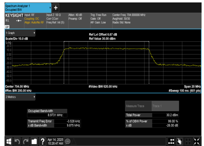
Band12-10MHz-16QAM-23060-50RB#0-PASS
