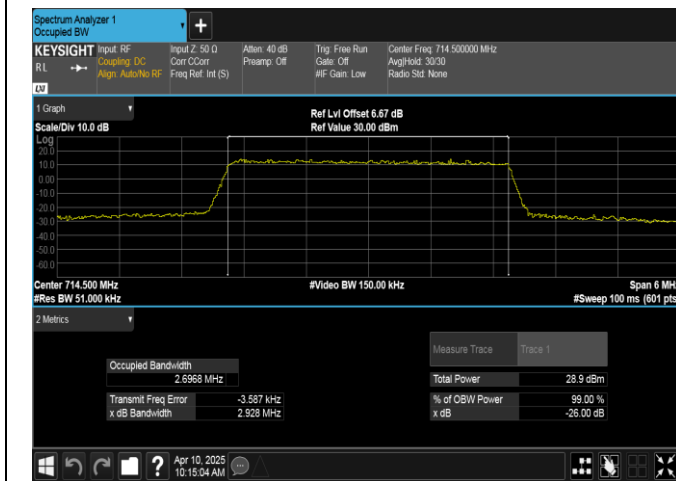
Band12-3MHz-QPSK-23165-15RB#0-PASS
