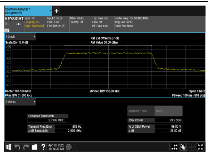
Band12-3MHz-QPSK-23095-15RB#0-PASS
