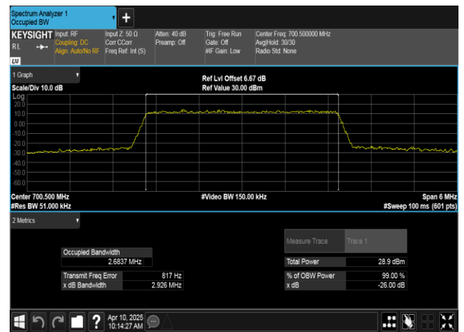
Band12-3MHz-16QAM-23025-15RB#0-PASS
