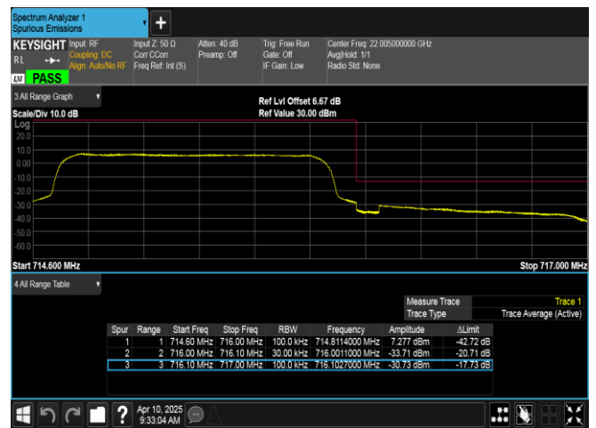
Band12-1.4MHz-QPSK-23173-6RB#0-PASS
