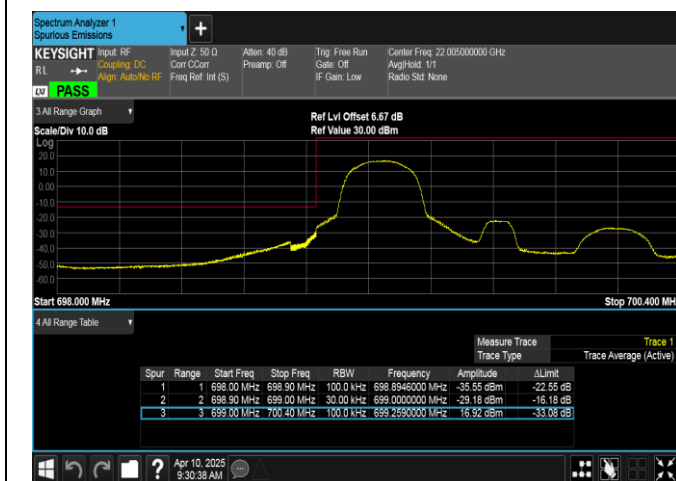
Band12-1.4MHz-16QAM-23017-1RB#0-PASS
