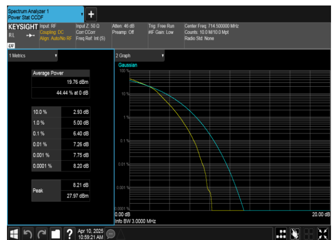
Band12-3MHz-16QAM-23165-15RB#0-PASS
