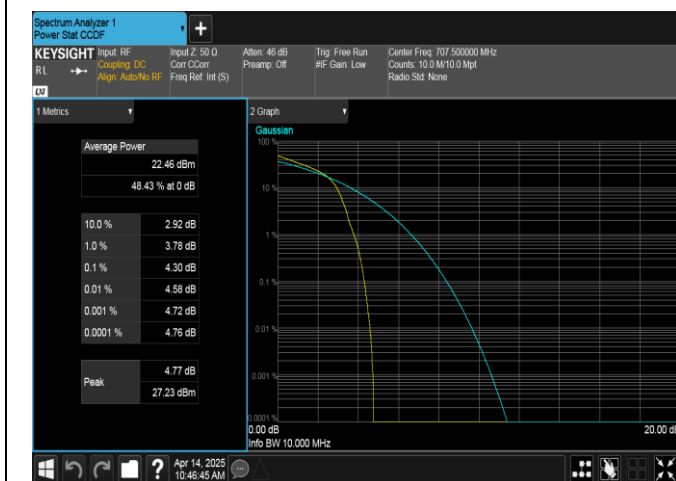
Band12-10MHz-16QAM-23095-1RB#0-PASS
