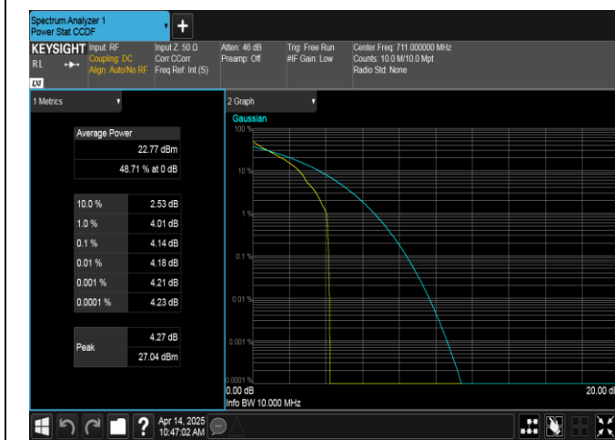
Band12-10MHz-QPSK-23130-1RB#0-PASS
