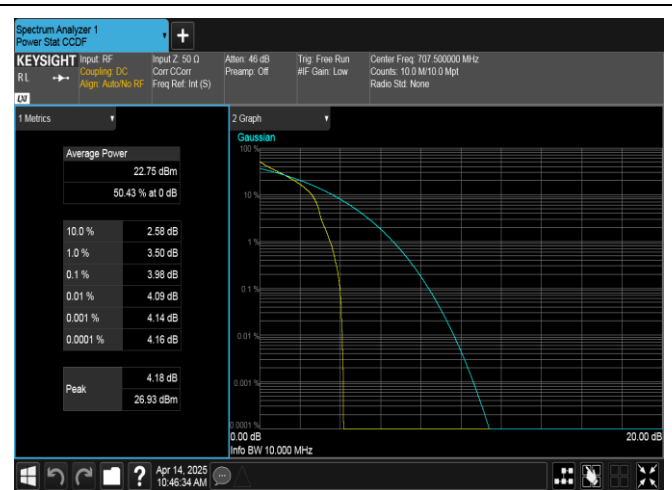
Band12-10MHz-QPSK-23095-1RB#0-PASS
