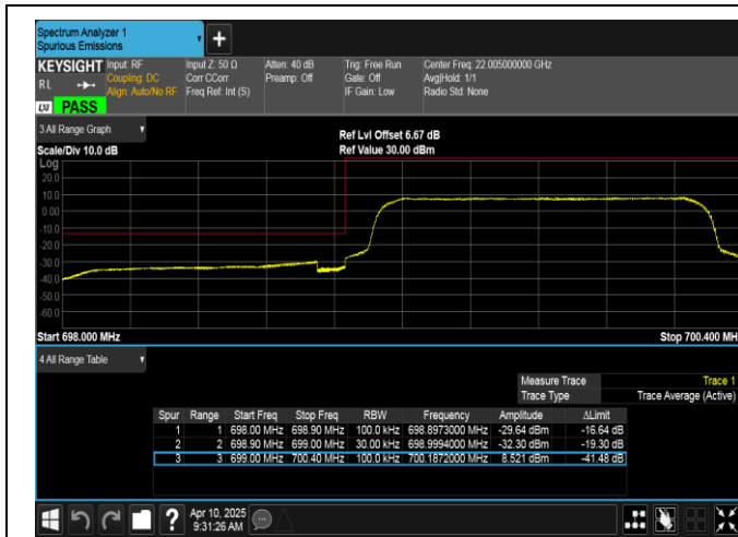
Band12-1.4MHz-QPSK-23017-6RB#0-PASS
