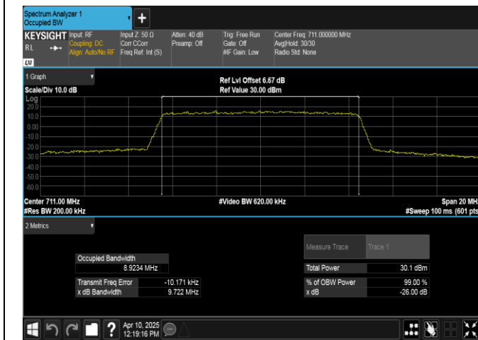
Band12-10MHz-QPSK-23130-50RB#0-PASS
