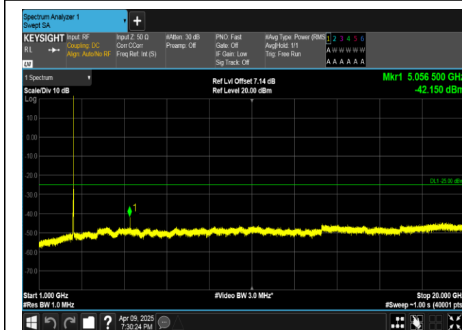
Band7-15MHz-QPSK-21100-1RB#0-1000~20000-PASS
