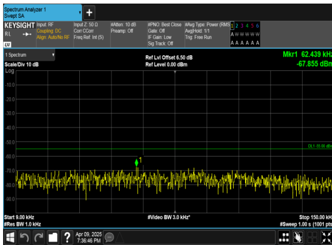
Band7-15MHz-16QAM-21375-1RB#74-0.009~0.15-PASS
