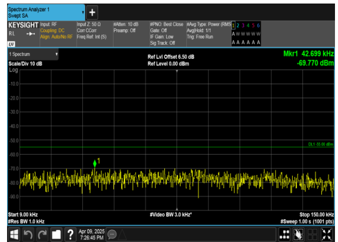
Band7-15MHz-16QAM-20825-1RB#0-0.009~0.15-PASS
