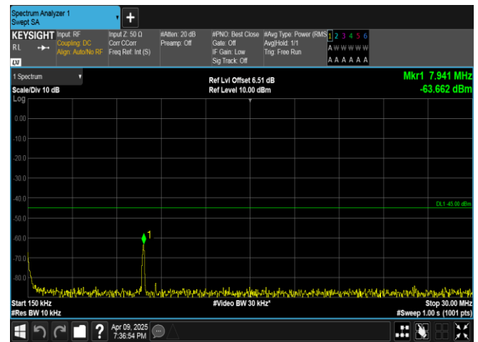
Band7-15MHz-16QAM-21375-1RB#74-0.15~30-PASS
