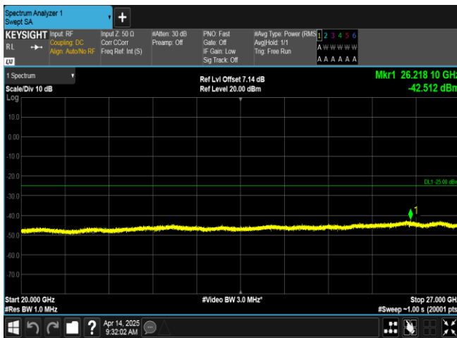
Band7-15MHz-QPSK-21375-75RB#0-20000~27000-PASS
