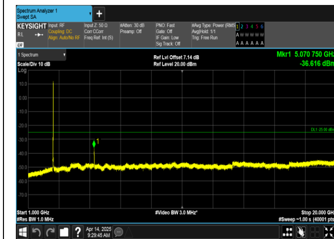
Band7-15MHz-QPSK-21100-75RB#0-1000~20000-PASS
