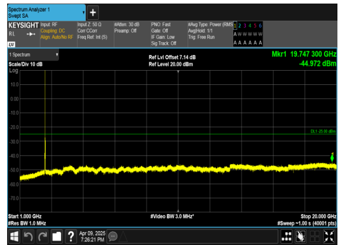
Band7-15MHz-QPSK-20825-1RB#0-1000~20000-PASS
