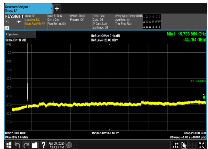
Band7-15MHz-16QAM-20825-1RB#74-1000~20000-PASS
