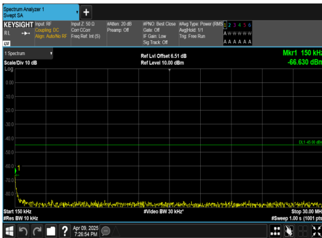
Band7-15MHz-16QAM-20825-1RB#0-0.15~30-PASS
