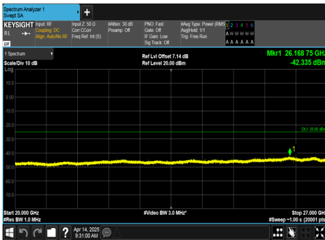
Band7-15MHz-16QAM-21100-75RB#0-20000~27000-PASS
