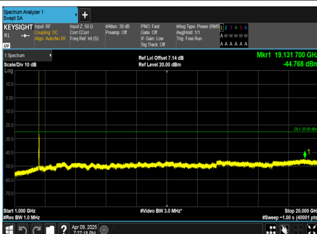
Band7-15MHz-16QAM-20825-1RB#0-1000~20000-PASS
