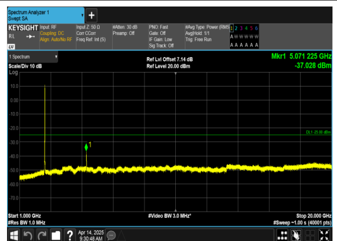
Band7-15MHz-16QAM-21100-75RB#0-1000~20000-PASS
