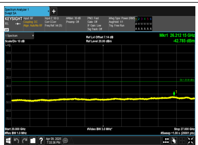
Band7-15MHz-16QAM-21100-1RB#74-20000~27000-PASS
