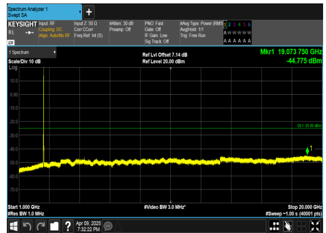
Band7-15MHz-QPSK-21100-1RB#74-1000~20000-PASS
