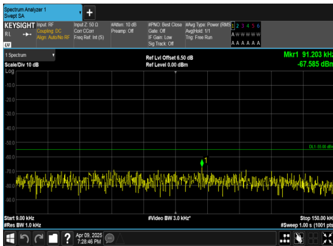
Band7-15MHz-16QAM-20825-1RB#74-0.009~0.15-PASS
