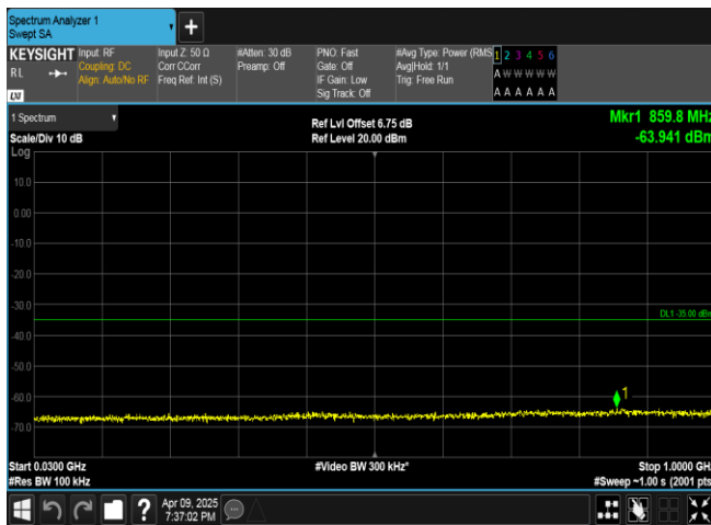
Band7-15MHz-16QAM-21375-1RB#74-30~1000-PASS
