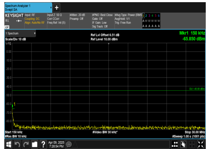
Band7-15MHz-16QAM-20825-1RB#74-0.15~30-PASS
