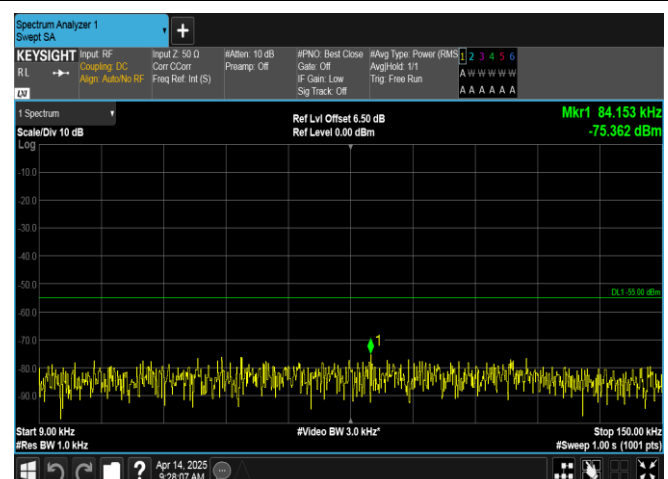
Band7-15MHz-16QAM-20825-75RB#0-0.009~0.15-PASS
