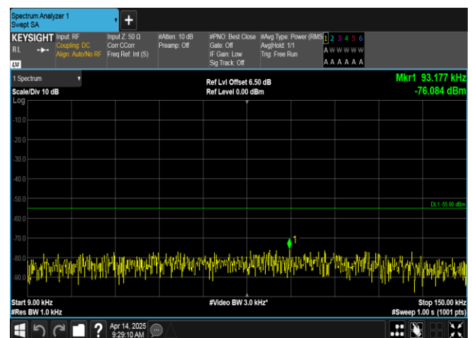
Band7-15MHz-QPSK-21100-75RB#0-0.009~0.15-PASS
