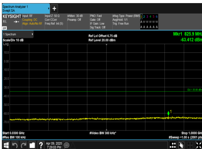
Band7-15MHz-16QAM-20825-1RB#74-30~1000-PASS
