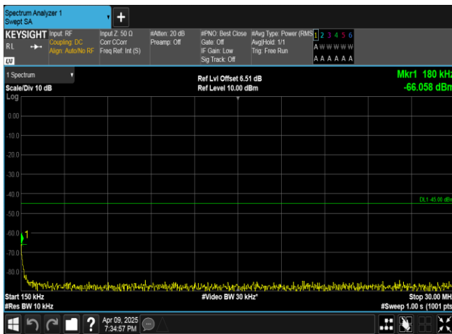
Band7-15MHz-16QAM-21375-1RB#0-0.15~30-PASS
