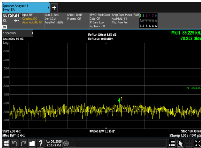
Band7-15MHz-QPSK-21100-1RB#74-0.009~0.15-PASS
