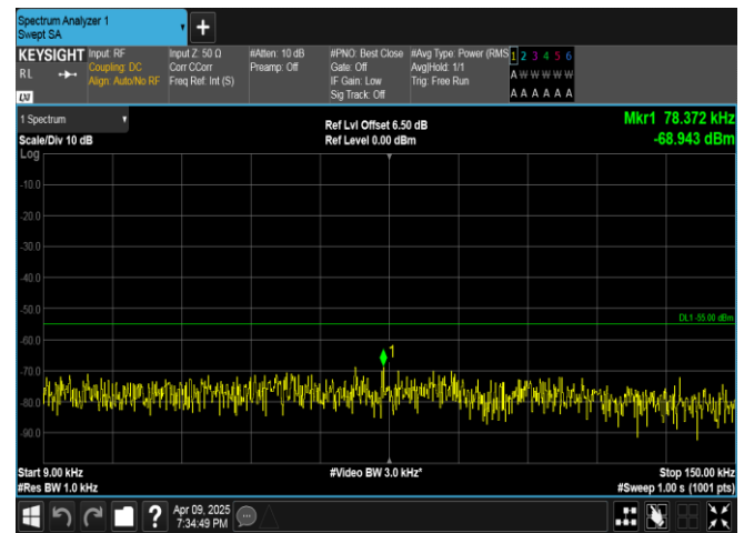
Band7-15MHz-16QAM-21375-1RB#0-0.009~0.15-PASS
