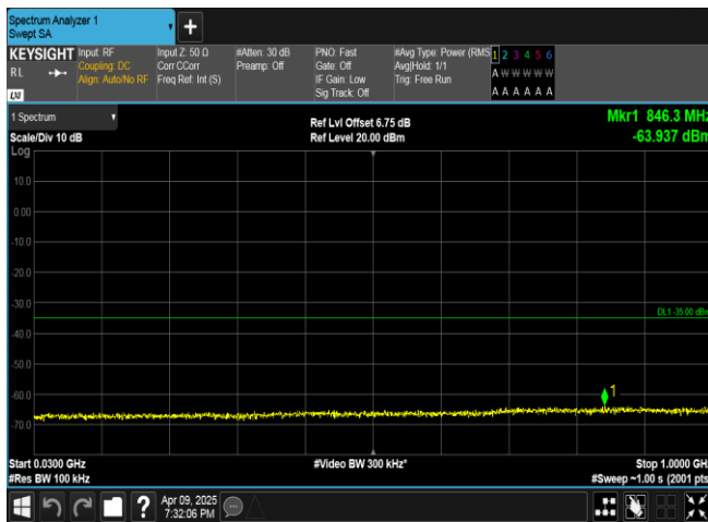
Band7-15MHz-QPSK-21100-1RB#74-30~1000-PASS
