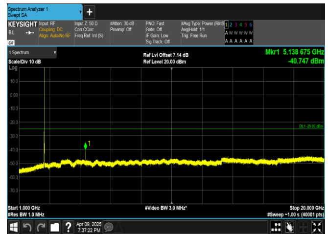
Band7-15MHz-16QAM-21375-1RB#74-1000~20000-PASS
