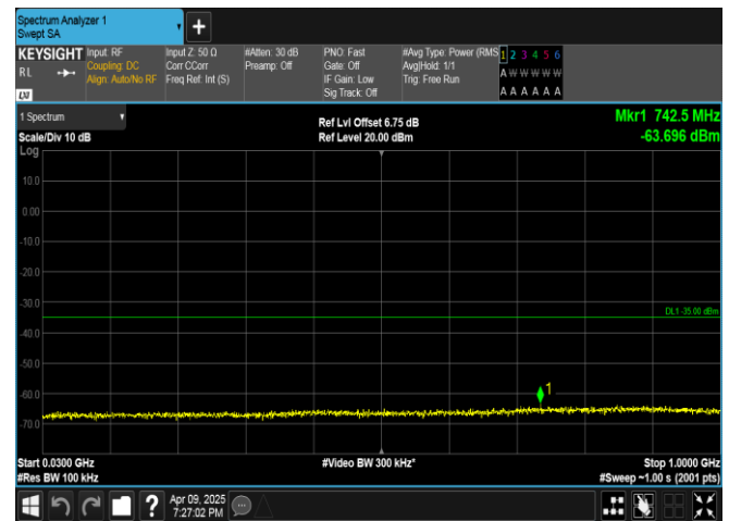
Band7-15MHz-16QAM-20825-1RB#0-30~1000-PASS
