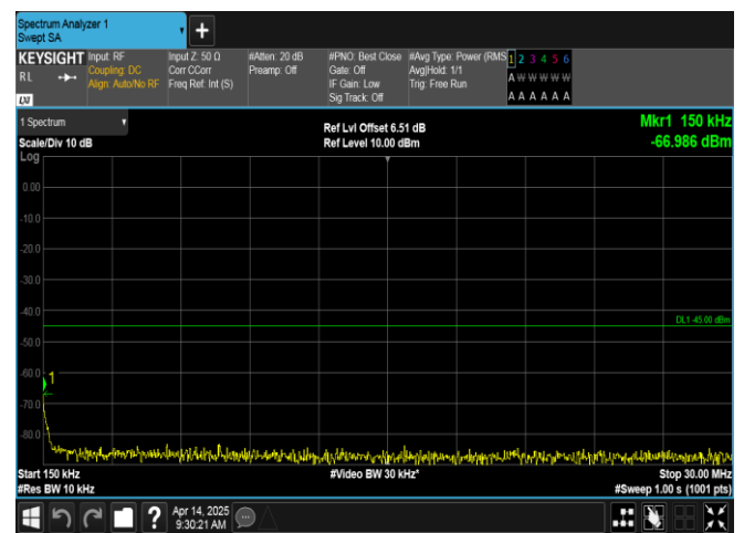
Band7-15MHz-16QAM-21100-75RB#0-0.15~30-PASS
