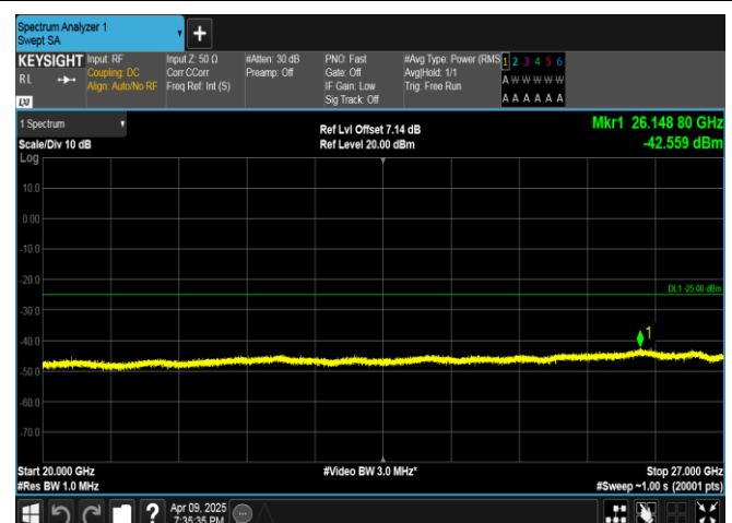
Band7-15MHz-16QAM-21375-1RB#0-20000~27000-PASS
