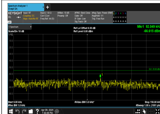
Band7-15MHz-16QAM-21100-1RB#0-0.009~0.15-PASS
