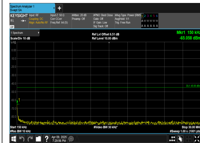
Band7-15MHz-QPSK-21100-1RB#0-0.15~30-PASS
