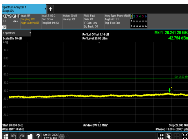
Band7-15MHz-16QAM-21375-1RB#74-20000~27000-PASS
