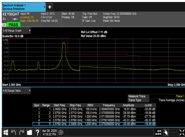
Band7-5MHz-QPSK-21425-1RB#24-PASS
