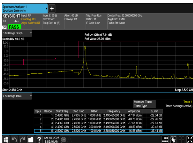
Band7-20MHz-QPSK-20850-1RB#0-PASS
