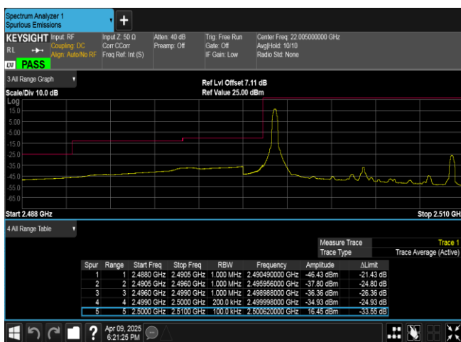
Band7-10MHz-QPSK-20800-1RB#0-PASS
