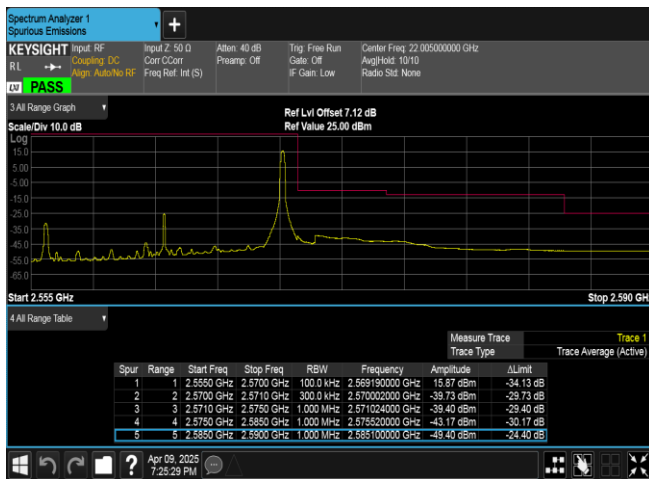
Band7-15MHz-16QAM-21375-1RB#74-PASS
