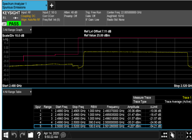
Band7-20MHz-QPSK-20850-100RB#0-PASS
