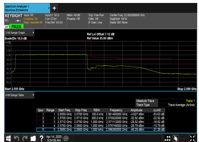
Band7-15MHz-QPSK-21375-75RB#0-PASS
