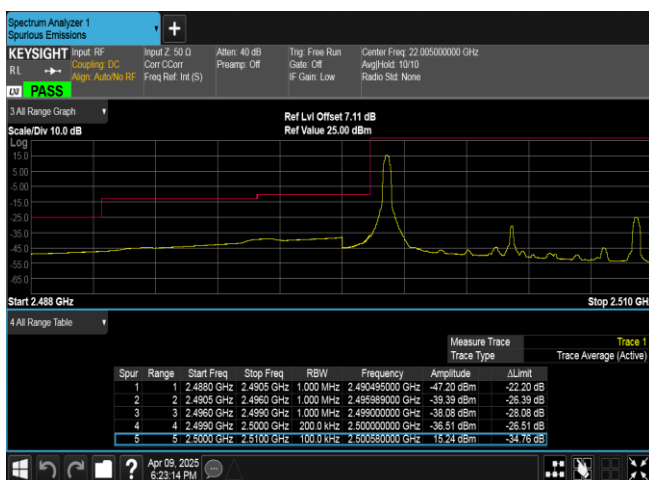
Band7-10MHz-16QAM-20800-1RB#0-PASS
