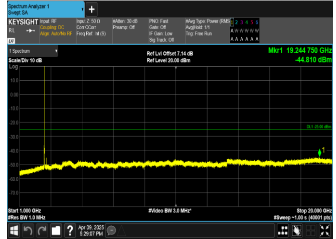
Band7-5MHz-QPSK-20775-1RB#0-1000~20000-PASS
