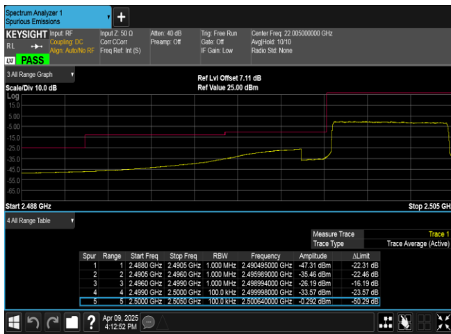
Band7-5MHz-16QAM-20775-25RB#0-PASS
