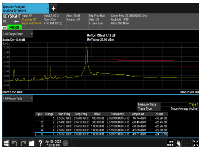
Band7-15MHz-QPSK-21375-1RB#74-PASS
