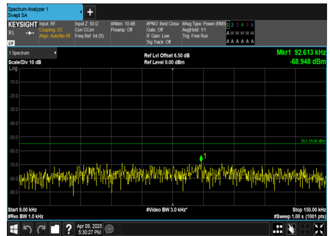
Band7-5MHz-QPSK-20775-1RB#24-0.009~0.15-PASS
