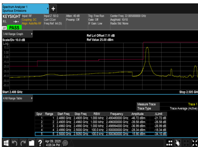
Band7-5MHz-16QAM-20775-1RB#0-PASS
