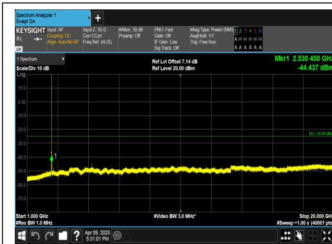
Band7-5MHz-QPSK-20775-1RB#24-1000~20000-PASS
