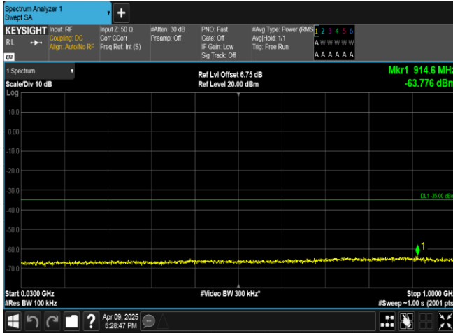
Band7-5MHz-QPSK-20775-1RB#0-30~1000-PASS
