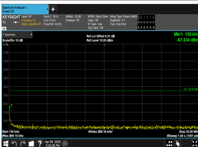
Band7-5MHz-QPSK-20775-1RB#24-0.15~30-PASS
