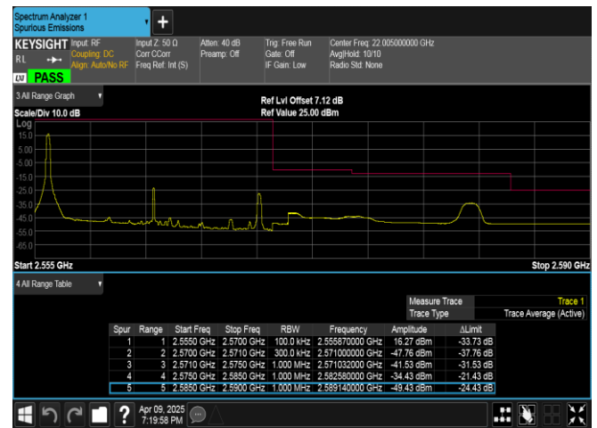
Band7-15MHz-QPSK-21375-1RB#0-PASS
