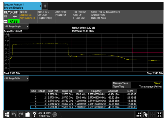
Band7-10MHz-QPSK-21400-50RB#0-PASS
