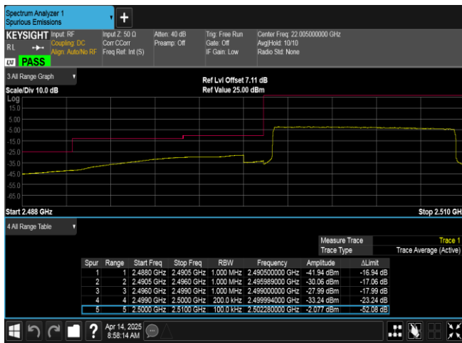
Band7-10MHz-16QAM-20800-50RB#0-PASS
