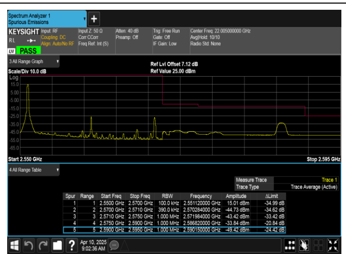
Band7-20MHz-16QAM-21350-1RB#0-PASS
