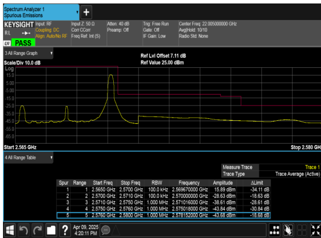
Band7-5MHz-16QAM-21425-1RB#24-PASS
