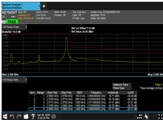
Band7-10MHz-QPSK-21400-1RB#49-PASS
