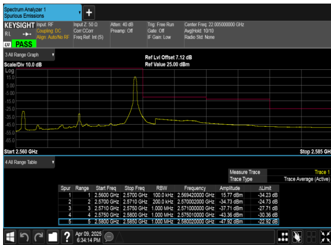
Band7-10MHz-16QAM-21400-1RB#49-PASS
