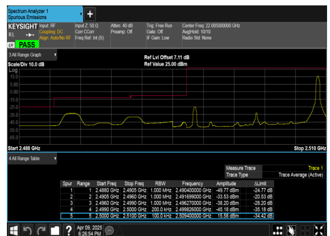
Band7-10MHz-16QAM-20800-1RB#49-PASS
