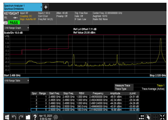
Band7-20MHz-16QAM-20850-1RB#99-PASS
