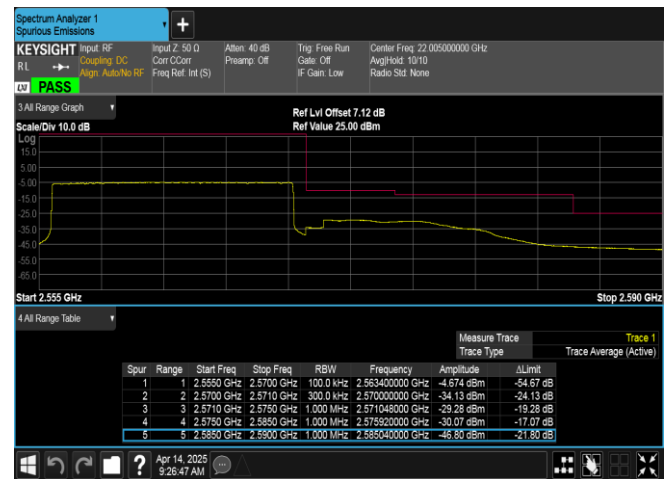
Band7-15MHz-16QAM-21375-75RB#0-PASS
