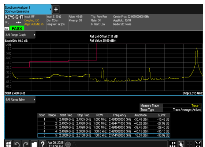
Band7-15MHz-16QAM-20825-1RB#74-PASS
