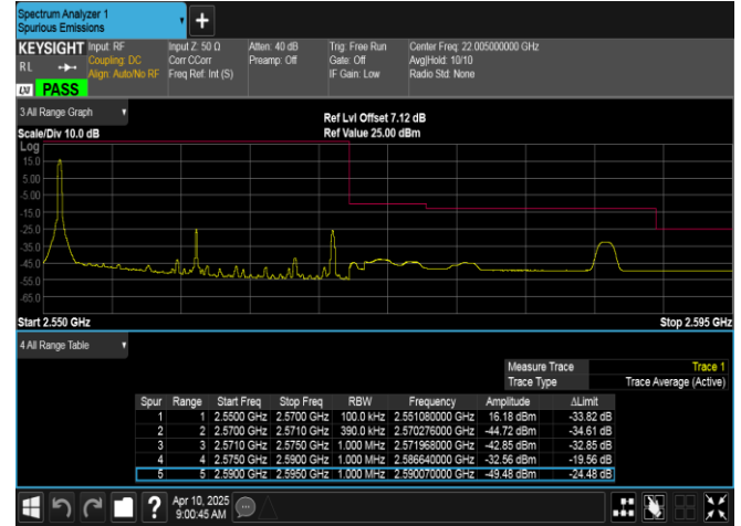
Band7-20MHz-QPSK-21350-1RB#0-PASS
