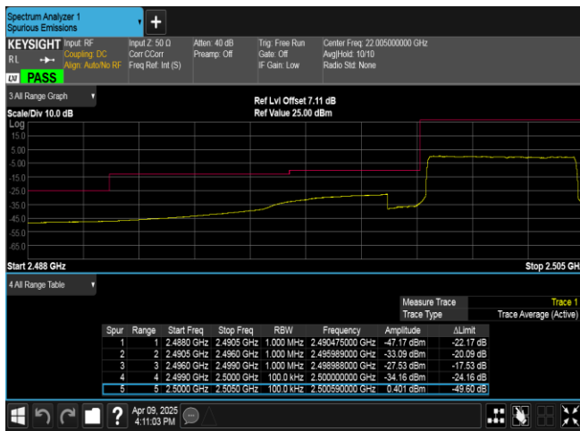
Band7-5MHz-QPSK-20775-25RB#0-PASS
