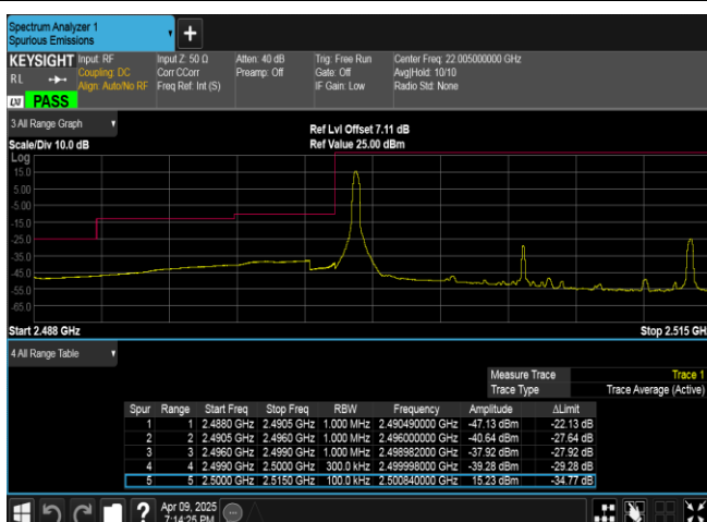
Band7-15MHz-16QAM-20825-1RB#0-PASS
