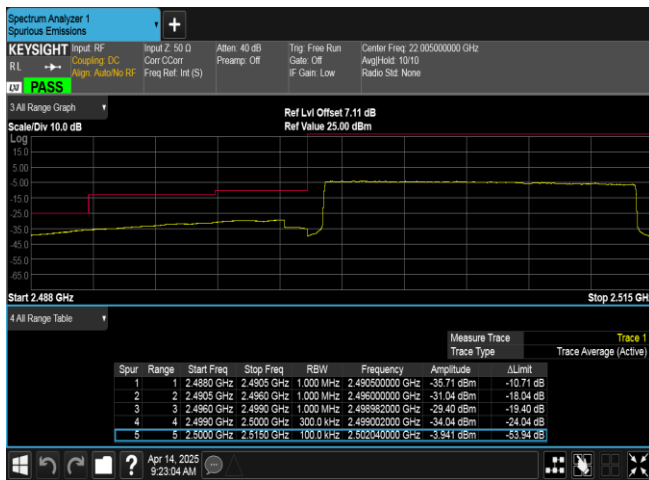
Band7-15MHz-16QAM-20825-75RB#0-PASS
