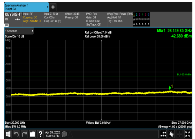
Band7-5MHz-QPSK-20775-1RB#24-20000~27000-PASS
