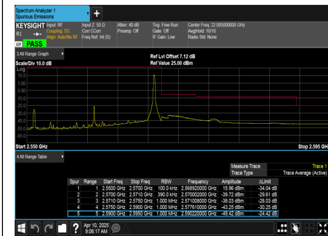
Band7-20MHz-16QAM-21350-1RB#99-PASS
