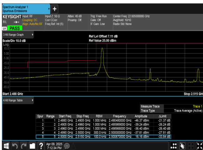
Band7-15MHz-QPSK-20825-1RB#0-PASS
