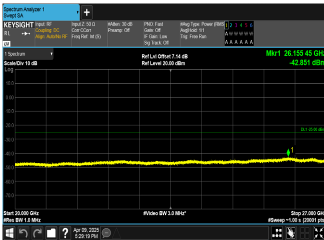
Band7-5MHz-QPSK-20775-1RB#0-20000~27000-PASS
