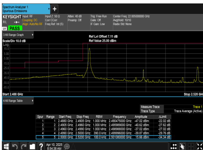
Band7-20MHz-16QAM-20850-1RB#0-PASS
