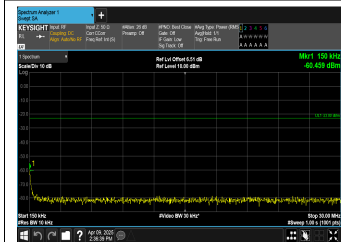
Band5-5MHz-QPSK-20625-1RB#24-0.15~30-PASS
