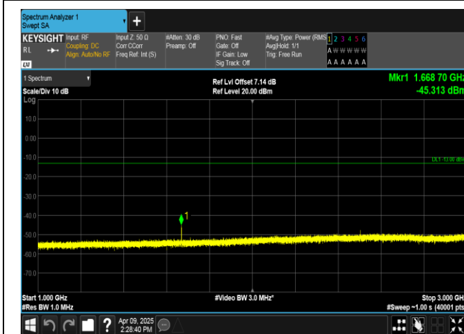
Band5-5MHz-QPSK-20525-1RB#0-1000~3000-PASS
