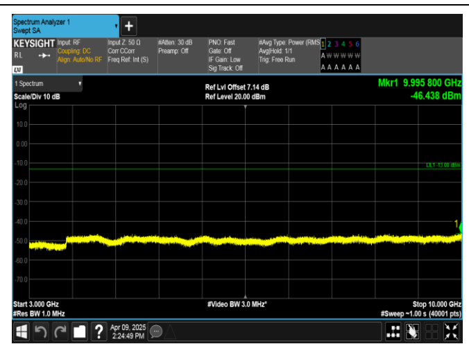
Band5-5MHz-QPSK-20425-1RB#24-3000~10000-PASS
