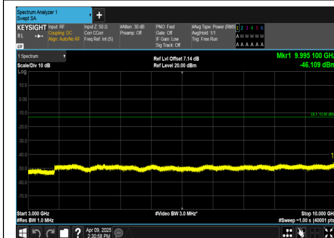
Band5-5MHz-QPSK-20525-1RB#24-3000~10000-PASS
