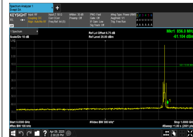
Band5-5MHz-QPSK-20525-1RB#24-30~1000-PASS
