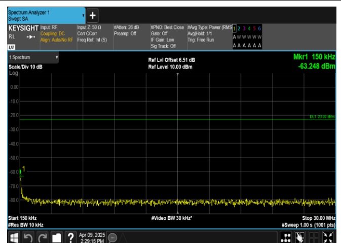
Band5-5MHz-16QAM-20525-1RB#0-0.15~30-PASS
