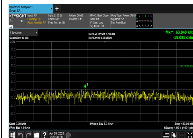
Band5-5MHz-16QAM-20525-1RB#0-0.009~0.15-PASS
