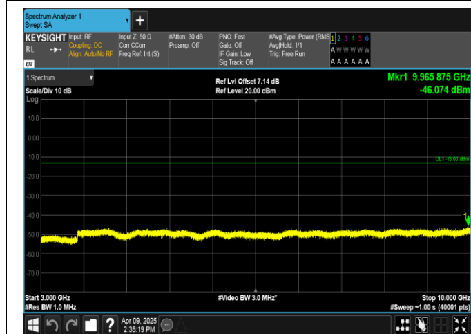
Band5-5MHz-QPSK-20625-1RB#0-3000~10000-PASS
