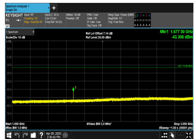
Band5-5MHz-QPSK-20525-1RB#24-1000~3000-PASS
