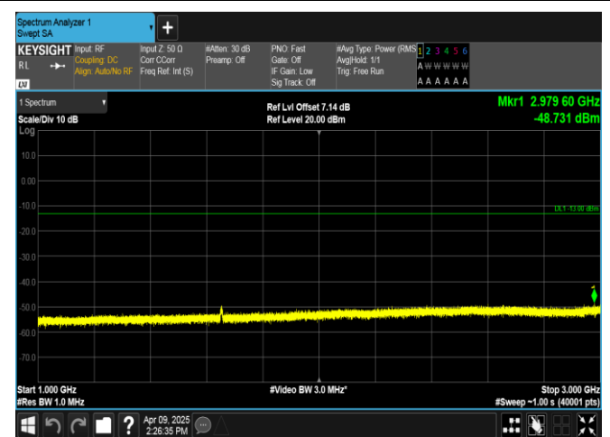
Band5-5MHz-QPSK-20425-25RB#0-1000~3000-PASS
