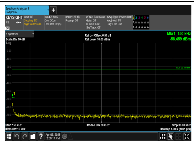
Band5-5MHz-QPSK-20525-1RB#24-0.15~30-PASS
