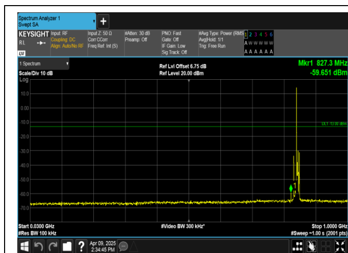
Band5-5MHz-QPSK-20625-1RB#0-30~1000-PASS
