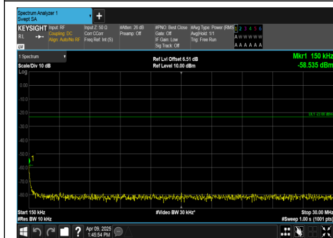
Band5-3MHz-QPSK-20415-1RB#14-0.15~30-PASS
