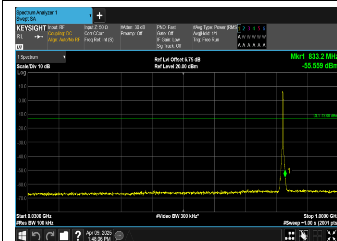
Band5-3MHz-QPSK-20415-15RB#0-30~1000-PASS
