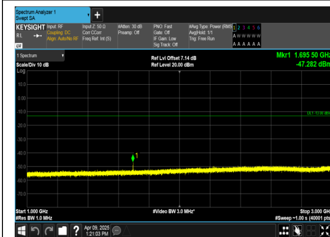
Band5-1.4MHz-16QAM-20643-1RB#0-1000~3000-PASS
