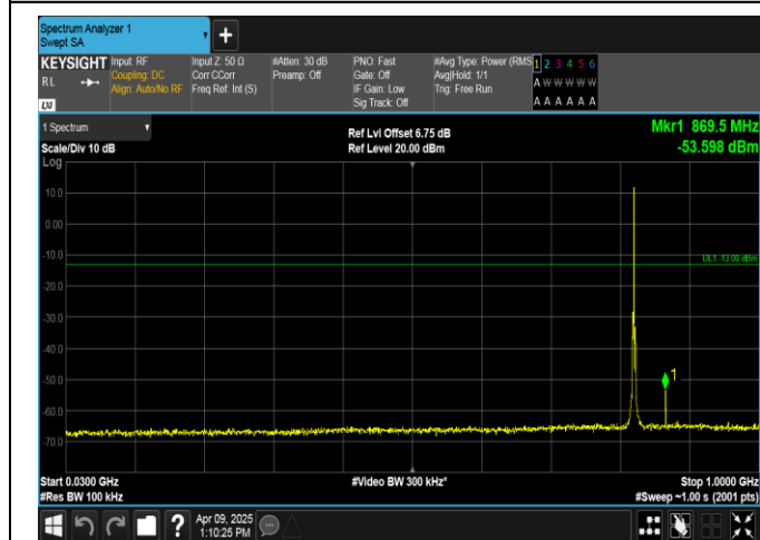
Band5-1.4MHz-16QAM-20407-1RB#5-30~1000-PASS
