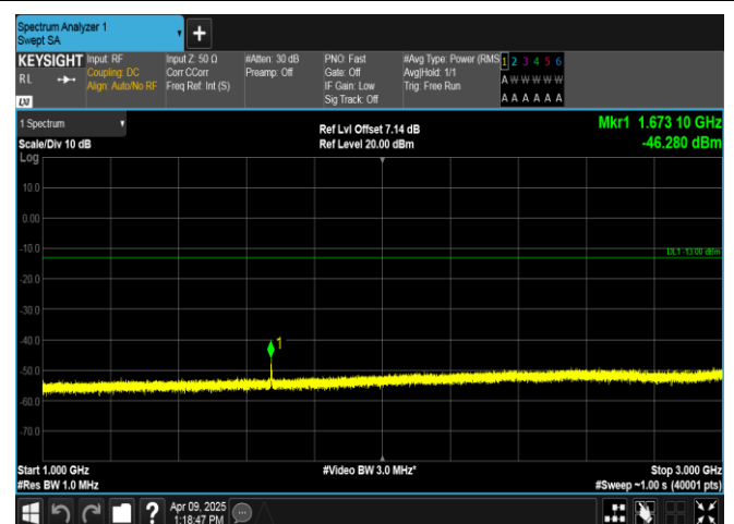
Band5-1.4MHz-16QAM-20525-6RB#0-1000~3000-PASS
