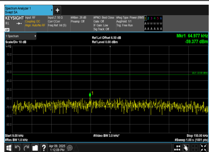
Band5-1.4MHz-16QAM-20407-6RB#0-0.009~0.15-PASS
