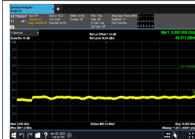
Band5-3MHz-QPSK-20415-1RB#0-3000~10000-PASS
