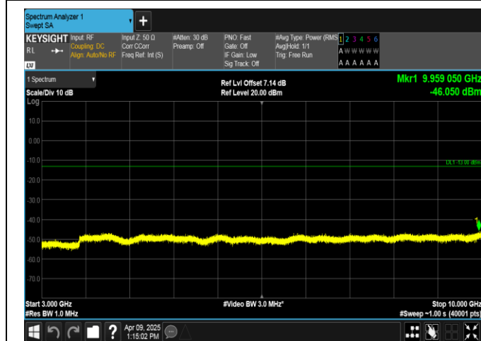
Band5-1.4MHz-16QAM-20525-1RB#0-3000~10000-PASS
