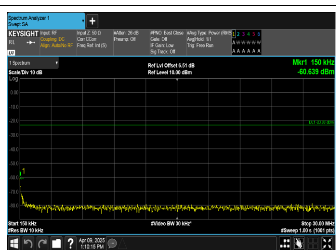
Band5-1.4MHz-16QAM-20407-1RB#5-0.15~30-PASS
