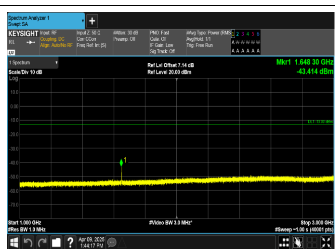
Band5-3MHz-QPSK-20415-1RB#0-1000~3000-PASS
