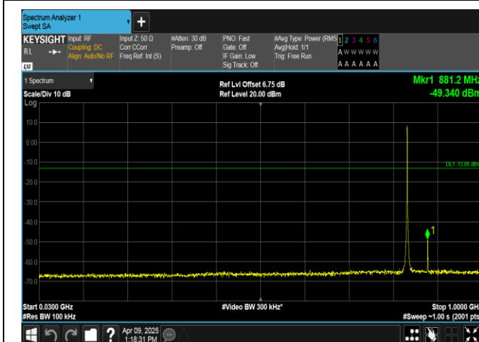
Band5-1.4MHz-16QAM-20525-6RB#0-30~1000-PASS
