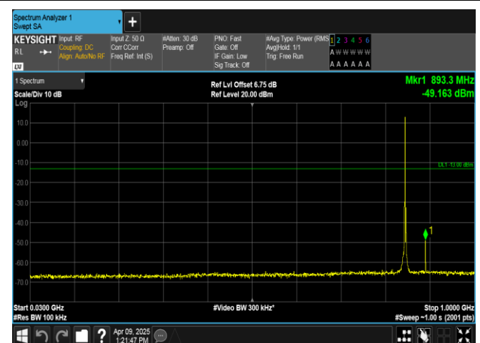
Band5-1.4MHz-QPSK-20643-1RB#5-30~1000-PASS
