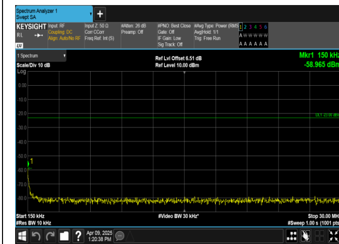
Band5-1.4MHz-16QAM-20643-1RB#0-0.15~30-PASS
