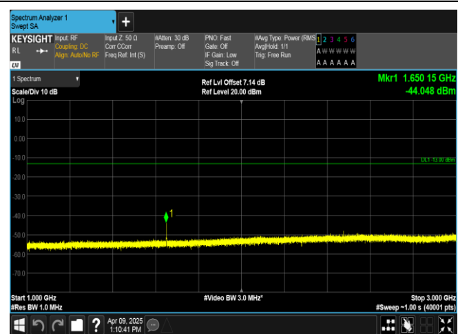
Band5-1.4MHz-16QAM-20407-1RB#5-1000~3000-PASS
