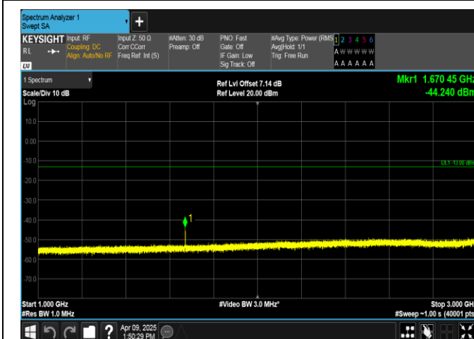
Band5-3MHz-QPSK-20525-1RB#0-1000~3000-PASS
