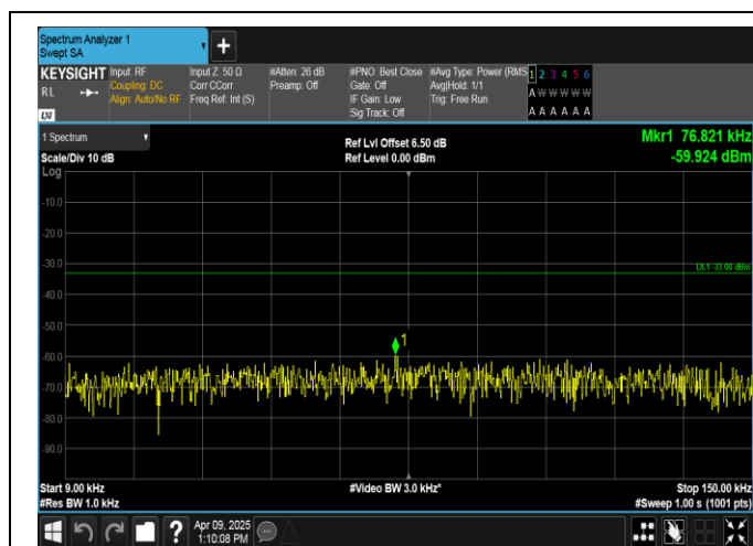
Band5-1.4MHz-16QAM-20407-1RB#5-0.009~0.15-PASS
