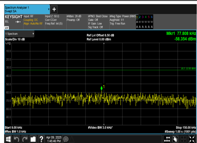
Band5-3MHz-QPSK-20415-1RB#14-0.009~0.15-PASS
