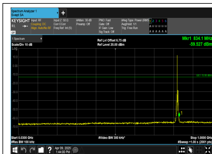
Band5-3MHz-QPSK-20415-1RB#0-30~1000-PASS
