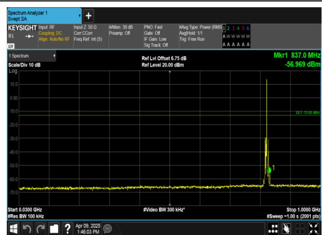
Band5-3MHz-QPSK-20415-1RB#14-30~1000-PASS
