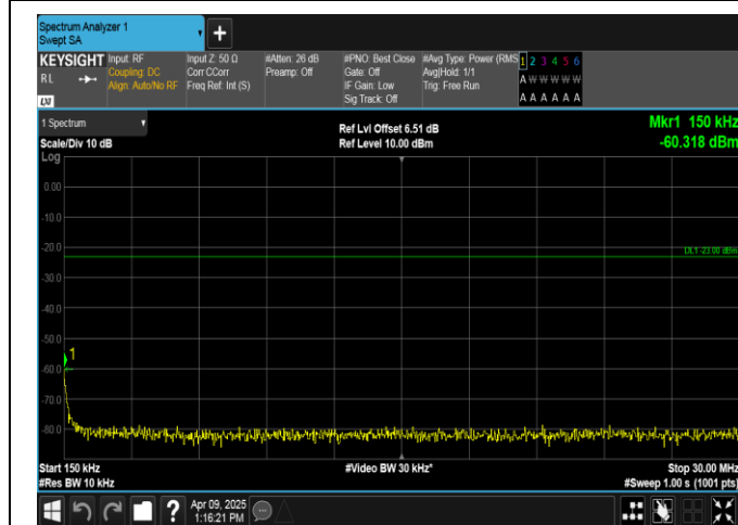
Band5-1.4MHz-16QAM-20525-1RB#5-0.15~30-PASS
