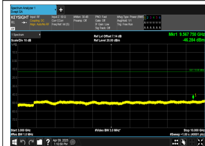
Band5-1.4MHz-16QAM-20407-1RB#5-3000~10000-PASS
