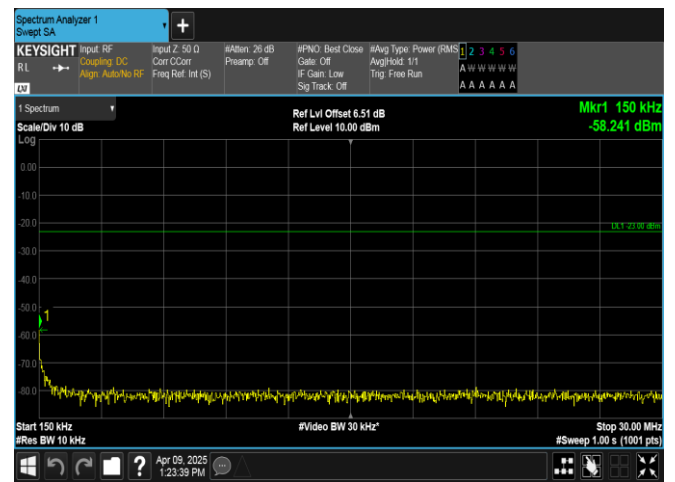
Band5-1.4MHz-QPSK-20643-6RB#0-0.15~30-PASS
