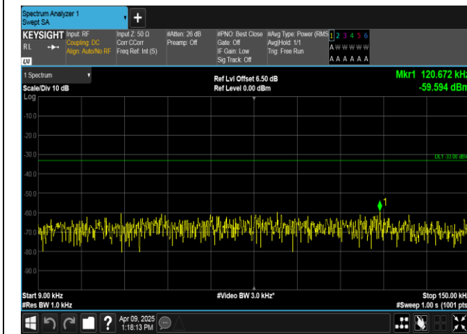
Band5-1.4MHz-16QAM-20525-6RB#0-0.009~0.15-PASS
