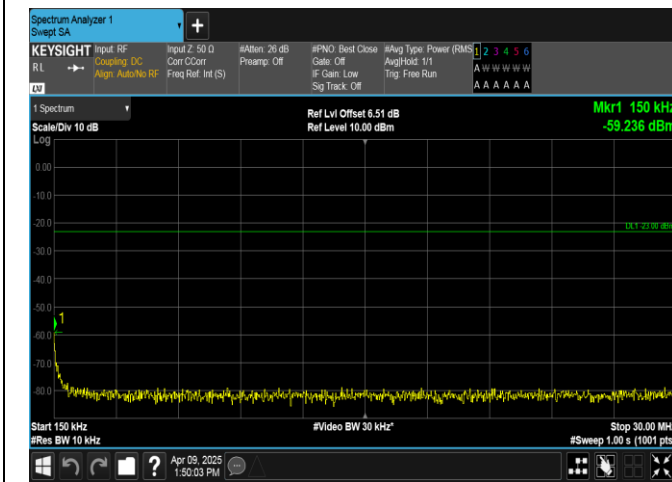
Band5-3MHz-QPSK-20525-1RB#0-0.15~30-PASS
