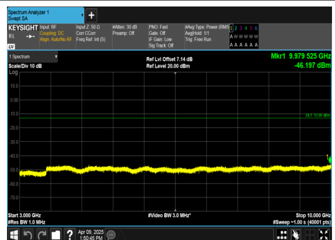
Band5-3MHz-QPSK-20525-1RB#0-3000~10000-PASS
