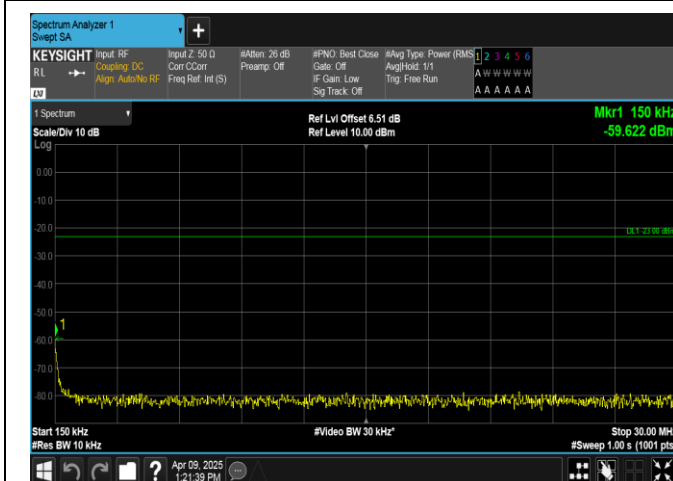
Band5-1.4MHz-QPSK-20643-1RB#5-0.15~30-PASS
