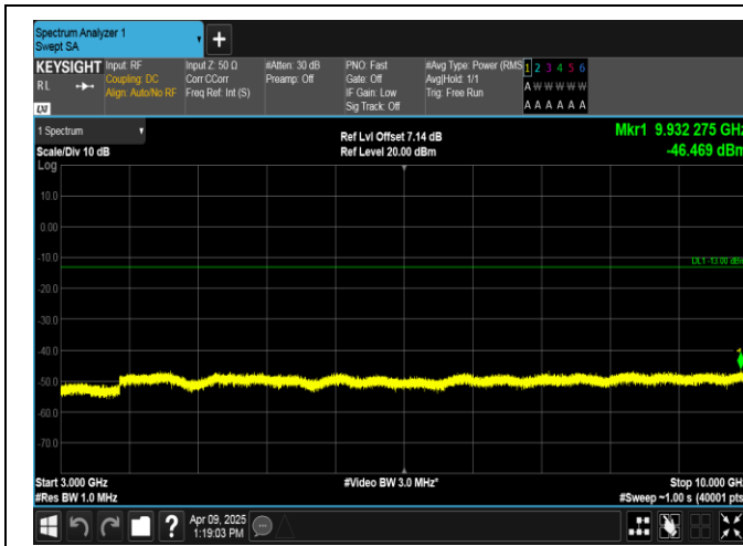
Band5-1.4MHz-16QAM-20525-6RB#0-3000~10000-PASS
