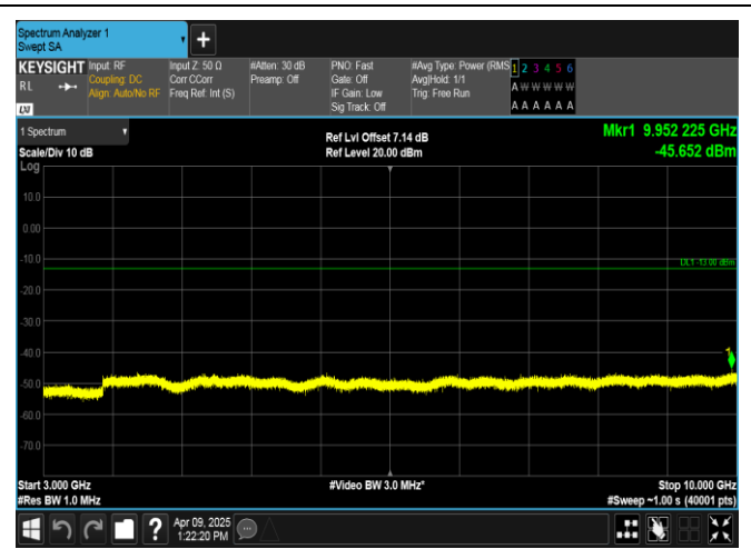
Band5-1.4MHz-QPSK-20643-1RB#5-3000~10000-PASS
