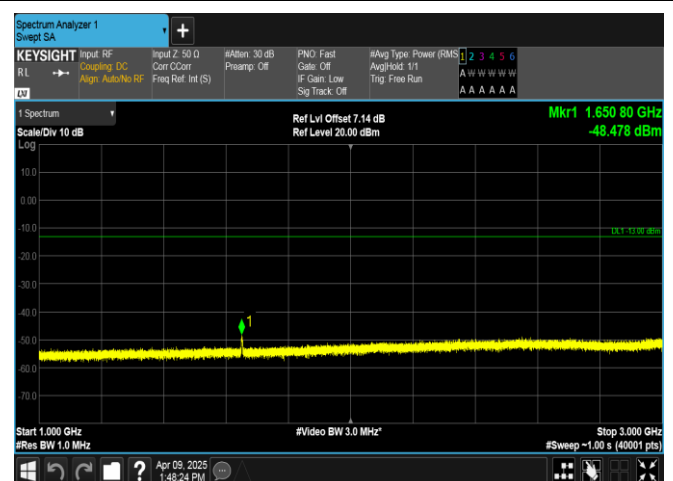
Band5-3MHz-QPSK-20415-15RB#0-1000~3000-PASS
