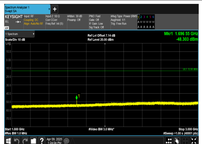
Band5-1.4MHz-QPSK-20643-6RB#0-1000~3000-PASS
