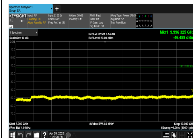
Band5-1.4MHz-16QAM-20643-1RB#5-3000~10000-PASS
