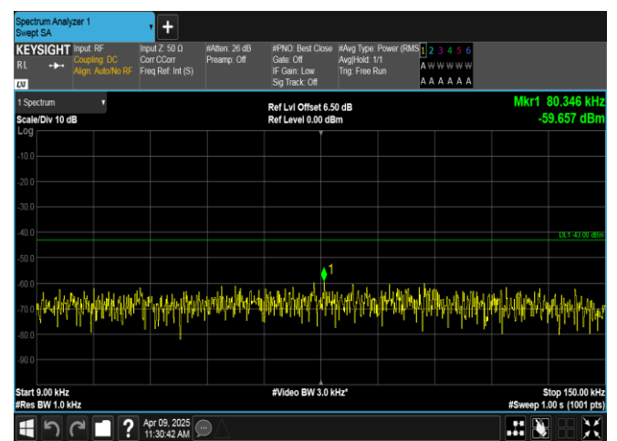
Band4-15MHz-QPSK-20175-1RB#0-0.009~0.15-PASS
