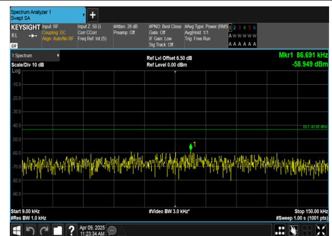
Band4-15MHz-QPSK-20025-1RB#74-0.009~0.15-PASS
