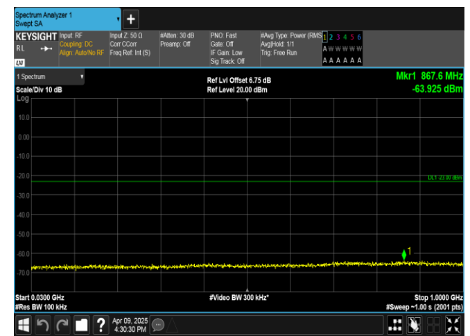
Band4-10MHz-16QAM-20350-50RB#0-30~1000-PASS
