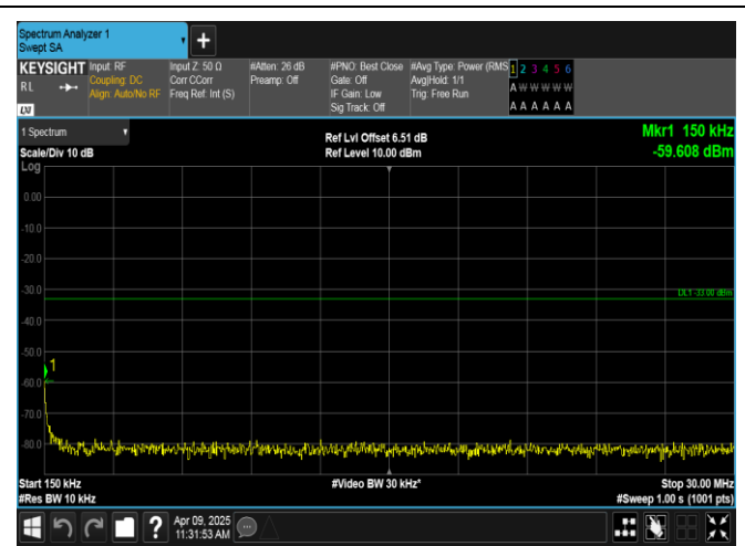
Band4-15MHz-16QAM-20175-1RB#0-0.15~30-PASS
