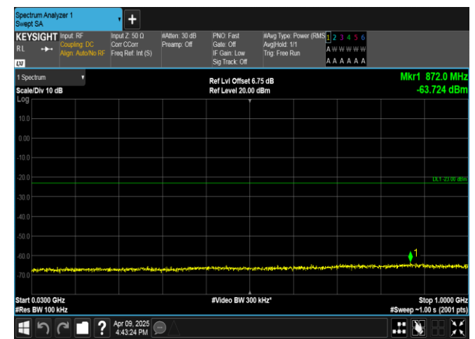
Band4-15MHz-16QAM-20025-75RB#0-30~1000-PASS
