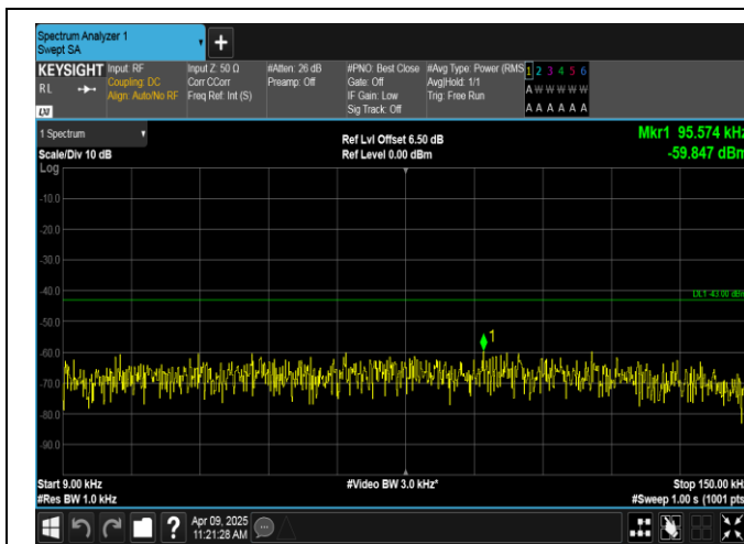
Band4-15MHz-QPSK-20025-1RB#0-0.009~0.15-PASS
