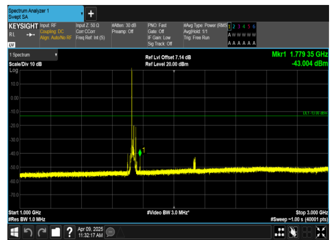
Band4-15MHz-16QAM-20175-1RB#0-1000~3000-PASS
