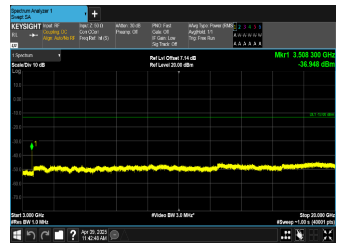
Band4-15MHz-QPSK-20325-1RB#74-3000~20000-PASS
