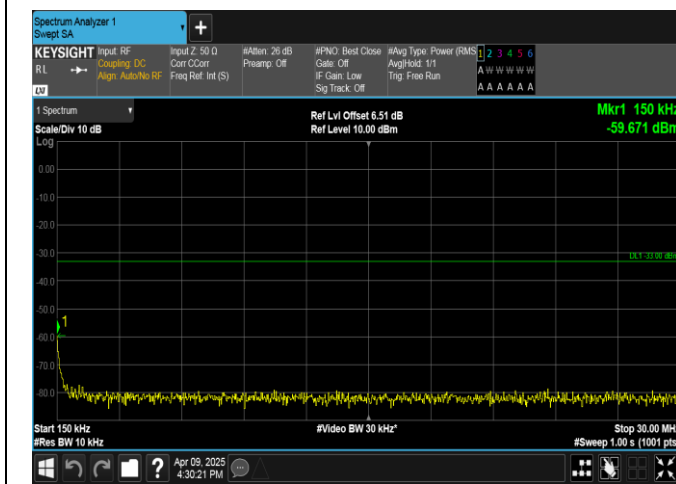
Band4-10MHz-16QAM-20350-50RB#0-0.15~30-PASS
