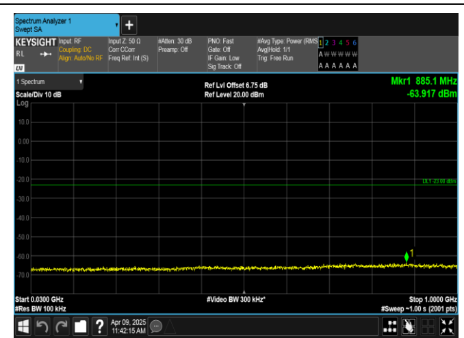
Band4-15MHz-QPSK-20325-1RB#74-30~1000-PASS
