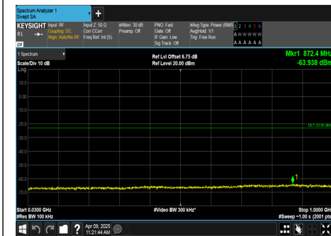
Band4-15MHz-QPSK-20025-1RB#0-30~1000-PASS
