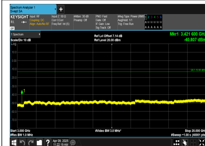
Band4-15MHz-QPSK-20025-1RB#0-3000~20000-PASS
