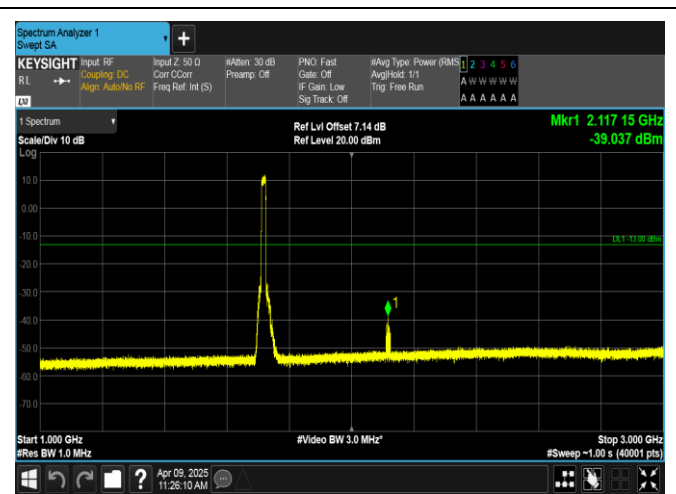
Band4-15MHz-QPSK-20025-75RB#0-1000~3000-PASS
