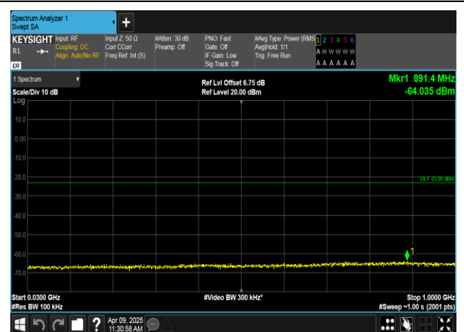
Band4-15MHz-QPSK-20175-1RB#0-30~1000-PASS
