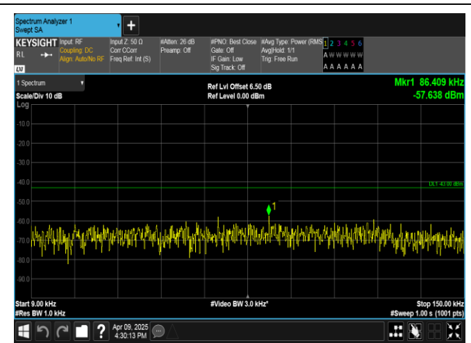
Band4-10MHz-16QAM-20350-50RB#0-0.009~0.15-PASS
