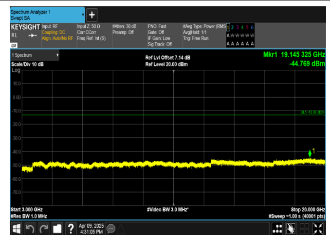
Band4-10MHz-16QAM-20350-50RB#0-3000~20000-PASS
