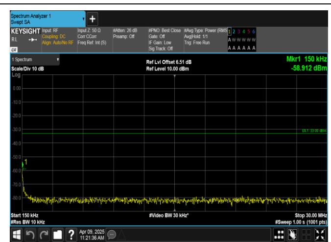
Band4-15MHz-QPSK-20025-1RB#0-0.15~30-PASS
