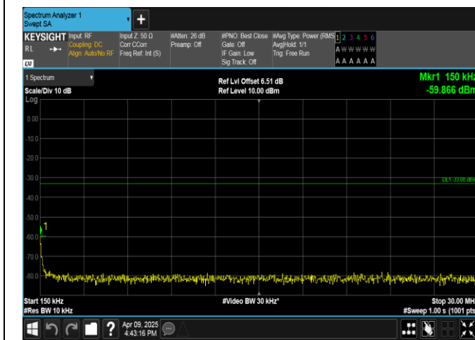
Band4-15MHz-16QAM-20025-75RB#0-0.15~30-PASS
