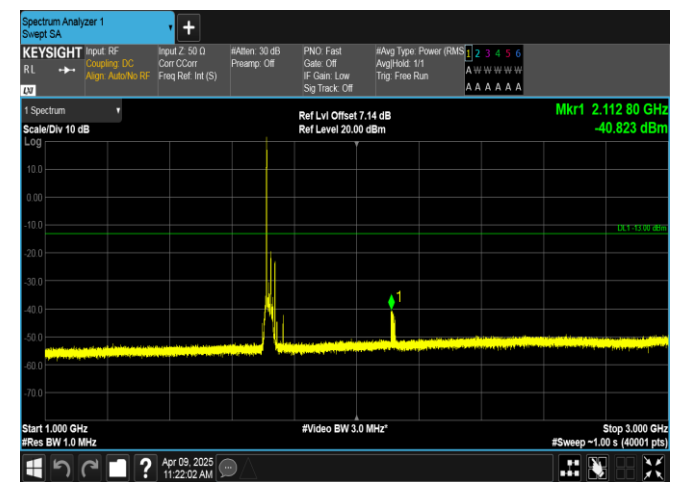
Band4-15MHz-QPSK-20025-1RB#0-1000~3000-PASS
